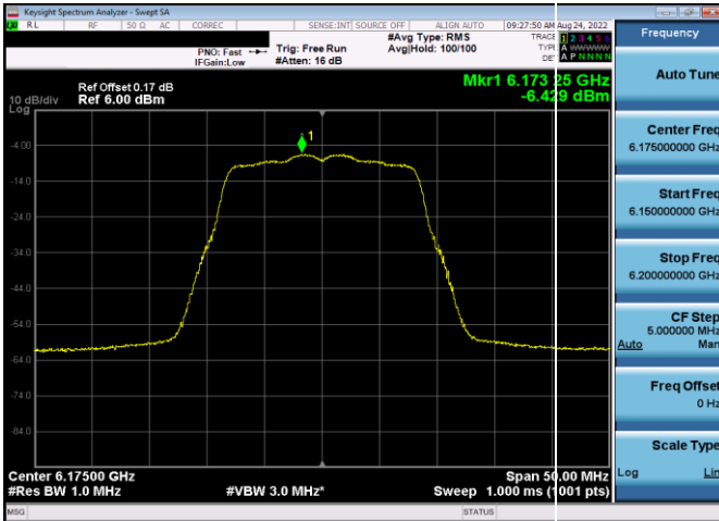
Plot 7-141. Power Spectral Density Plot Antenna 5b (20MHz 802.11a (UNII Band 5) – Ch. 45, MCS4)
