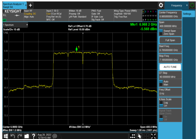
Plot 7-204. Power Spectral Density Plot Antenna 4a (160MHz 802.11ax (UNII Band 8) – Ch. 207, MCS2)
