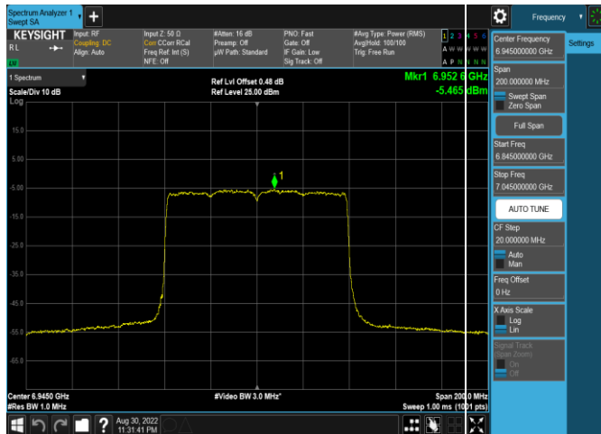
Plot 7-203. Power Spectral Density Plot Antenna 4a (80MHz 802.11ax (UNII Band 8) – Ch. 199, MCS2)
