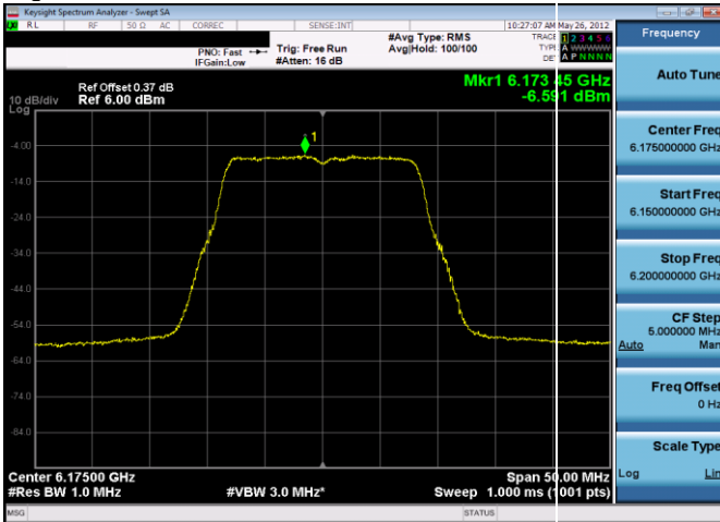
Plot 7-225. Power Spectral Density Plot Antenna 4a (20MHz 802.11a (UNII Band 5) – Ch. 45, MCS11)
