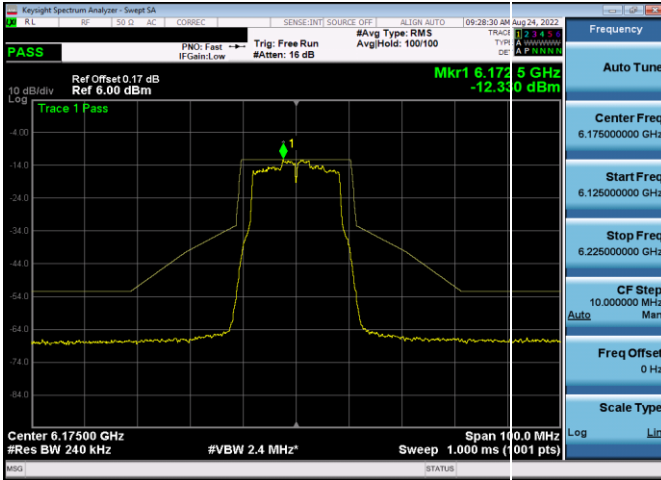
Plot 7-345. In-Band Emission Plot Antenna 5b (20MHz 802.11a (UNII Band 5) – Ch. 45, MCS2)
