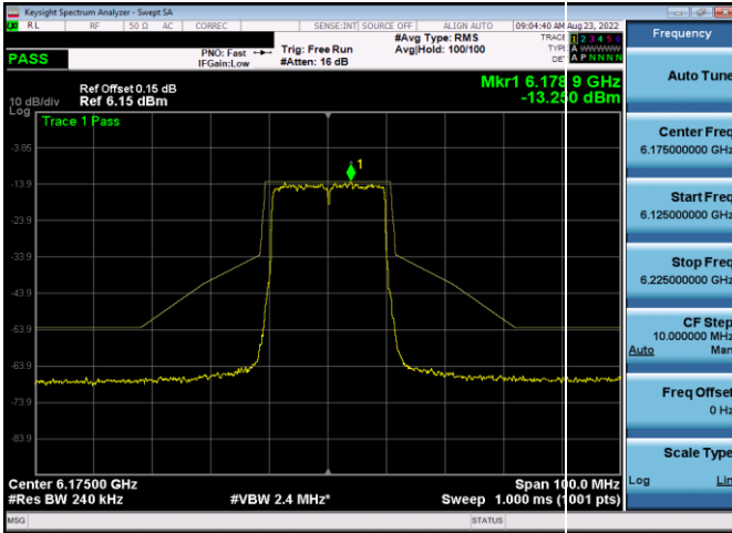
Plot 7-346. In-Band Emission Plot Antenna 5b (20MHz 802.11ax (UNII Band 5) – Ch. 45, MCS2)
