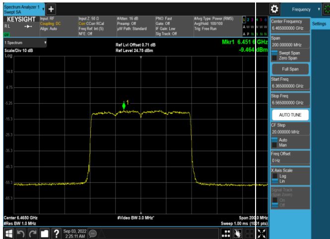
Plot 7-294. Power Spectral Density Plot SDM Antenna 4a (80MHz 802.11ax (UNII Band 6) – Ch. 103, MCS4)
