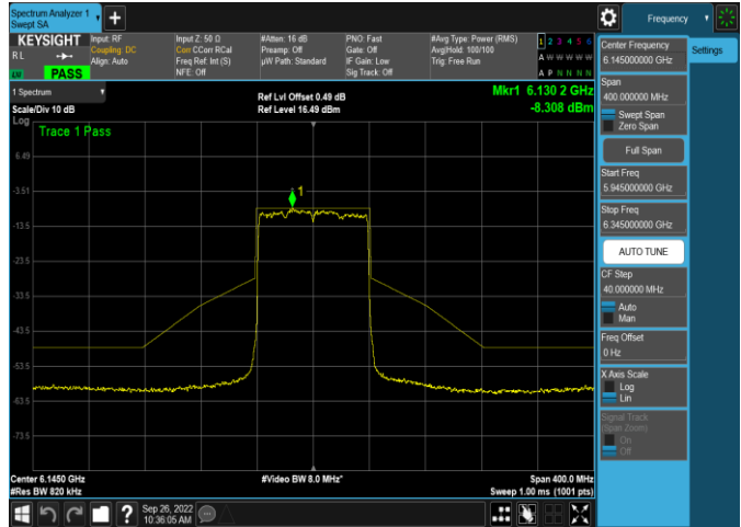
Plot 7-348. In-Band Emission Plot Antenna 5b (80MHz 802.11ax (UNII Band 5) – Ch. 39, MCS2)
