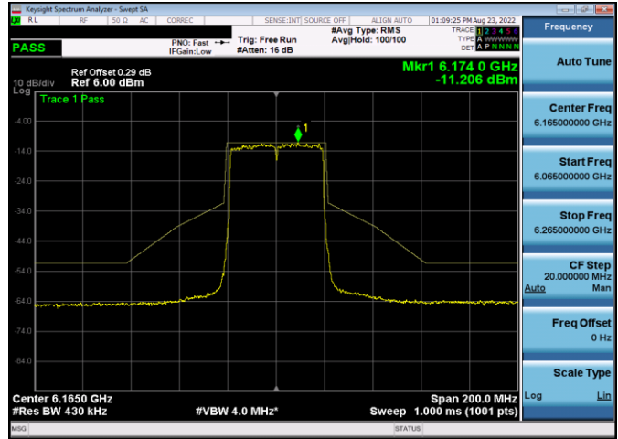
Plot 7-347. In-Band Emission Plot Antenna 5b (40MHz 802.11ax (UNII Band 5) – Ch. 43, MCS2)
