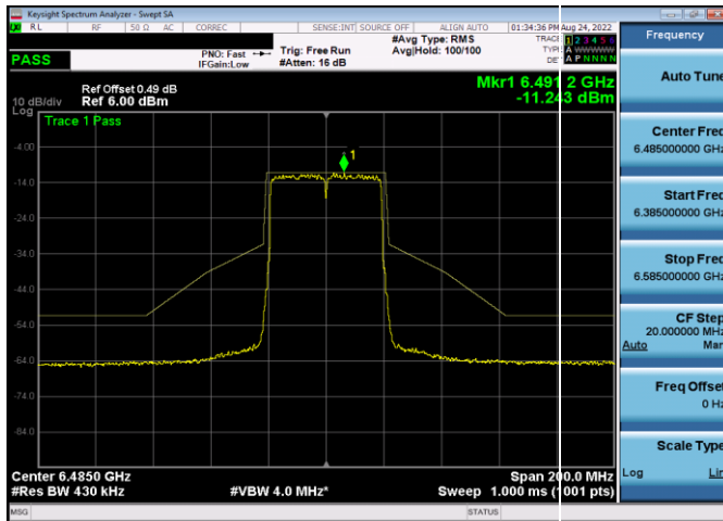
Plot 7-372. In-Band Emission Plot Antenna 5b (40MHz 802.11ax (UNII Band 6) – Ch. 107, MCS4)
