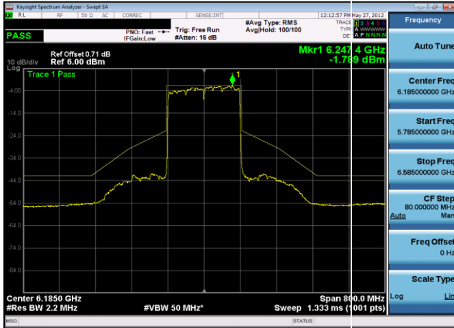
Plot 7-349. In-Band Emission Plot Antenna 5b (160MHz 802.11ax (UNII Band 5) – Ch. 47, MCS2)
