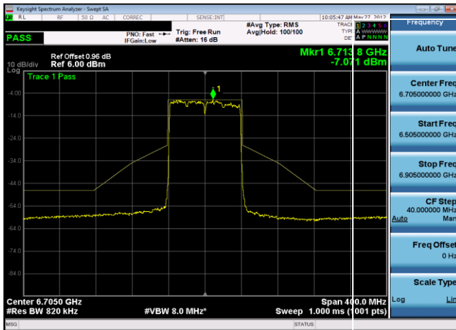
Plot 7-394. In-Band Emission Plot Antenna 5b (80MHz 802.11ax (UNII Band 7) – Ch. 151, MCS11)
