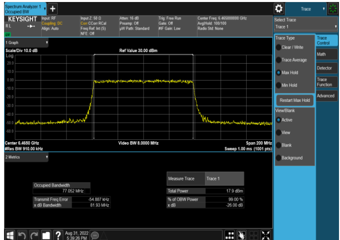
Plot 7-26. 26dB & 99% Bandwidth Plot Antenna 5b (80MHz 802.11ax RU96 (UNII Band 6) – Ch. 103)
