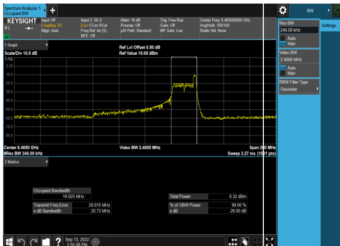
Plot 7-27. 26dB & 99% Bandwidth Plot Antenna 5b (80MHz 802.11ax RU26 (UNII Band 6) – Ch. 103)
