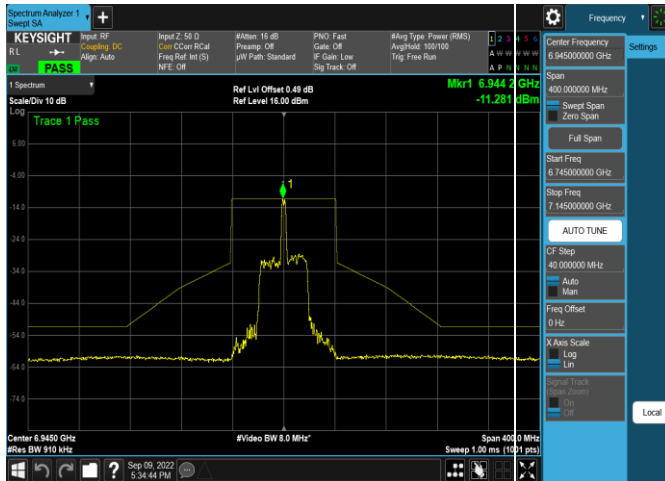
Plot 7-627. In-Band Emission Plot SDM Antenna 5b (80MHz 802.11ax RU26 (UNII Band 8) – Ch. 199)
