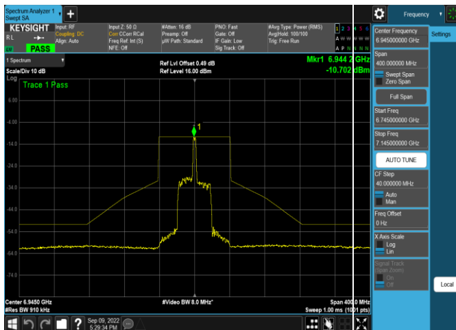
Plot 7-628. In-Band Emission Plot SDM Antenna 4a (80MHz 802.11ax RU26 (UNII Band 8) – Ch. 199)
