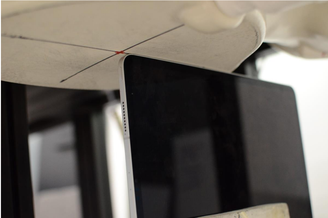
Figure G-7 SAR Test Setup Photo – Right Edge at 0 mm – Antenna 4A
