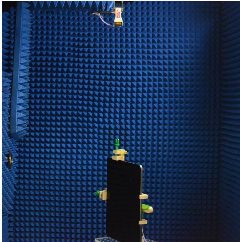
Test Setup Photo 7 – Radiated Power Test Setup (Figure 7-1)
