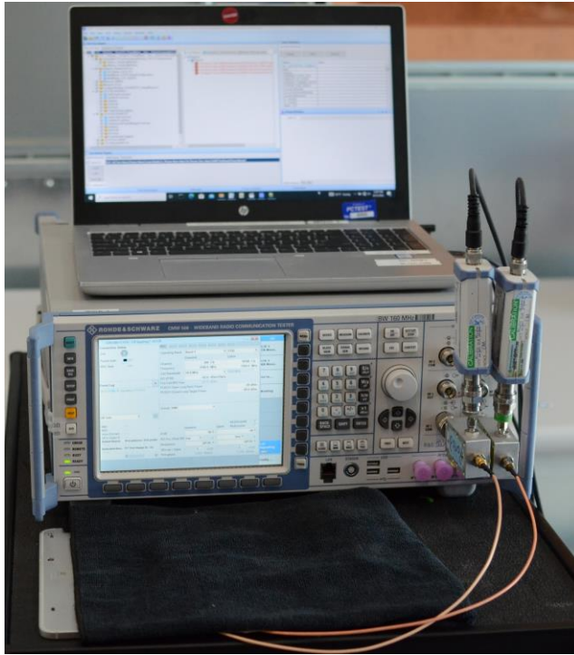
Test Setup Photo 5 – Conducted Test Setup (Figure 6-1c)
