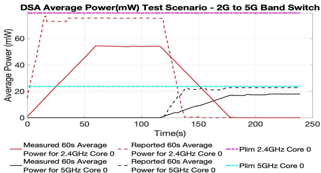
Figure F - 10 60 Sec Average SAR Utilization vs. Time during Band Switch
