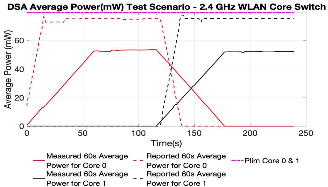
Figure F - 2 60 Sec Average Power vs. Time, 2.4 GHz
