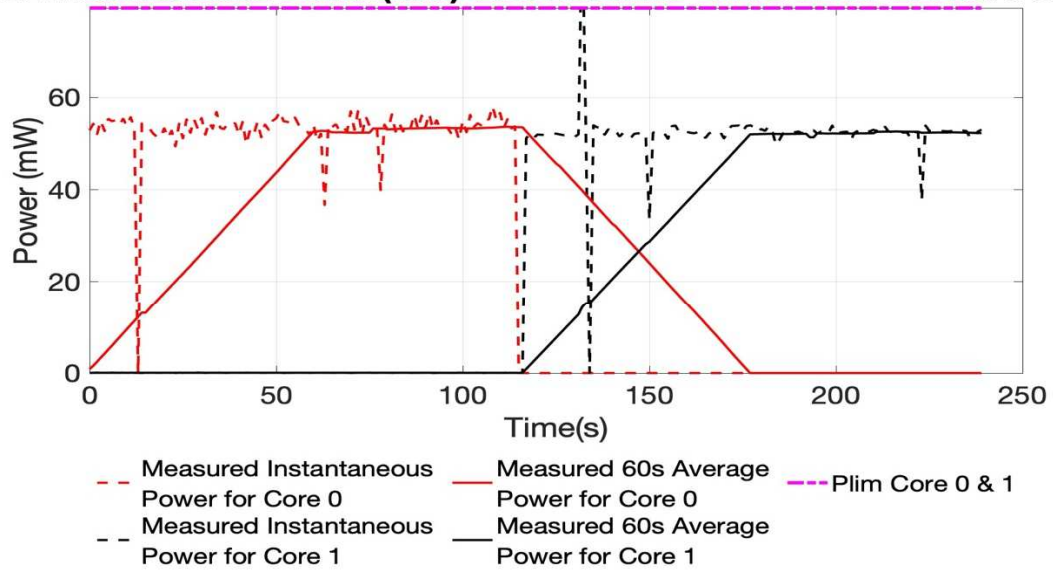
Figure F - 3 60 Sec Instantaneous Power vs. Time, 2.4 GHz
