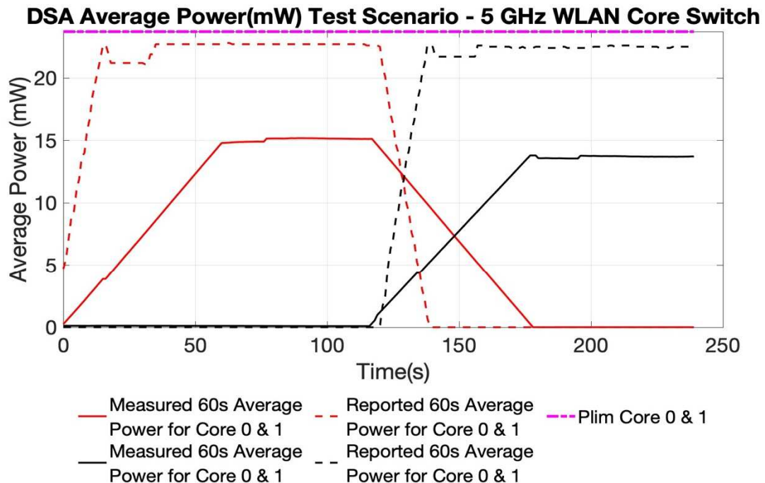
Figure F - 4 60 Sec Average SAR Utilization vs. Time, 5 GHz
