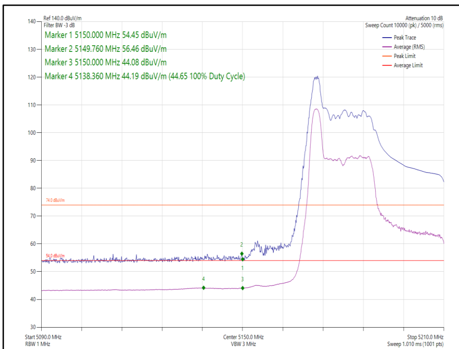
Figure 33 - 802.11ax HE40, Core 0, 26-0 - 5190 MHz Band Edge Frequency 5150 MHz
