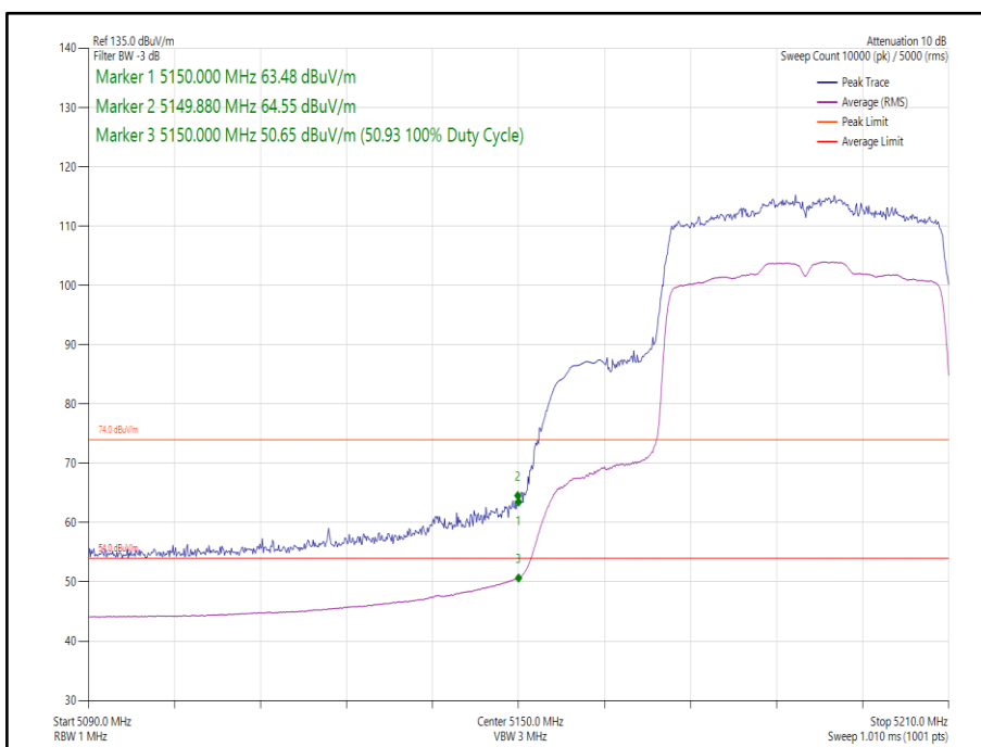
Figure 32 - 802.11ax HE40, Core 0, SU - 5190 MHz Band Edge Frequency 5150 MHz
