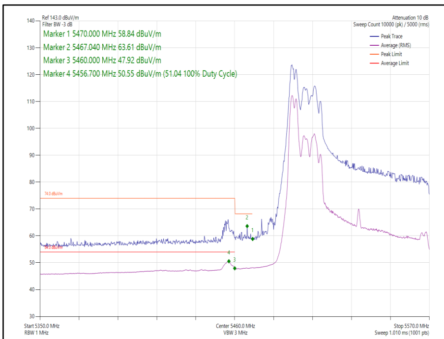
Figure 303 - 802.11ax HE80 CDD, Cores 0-1, 52-37- 5530 MHz Band Edge Frequency 5470 MHz
