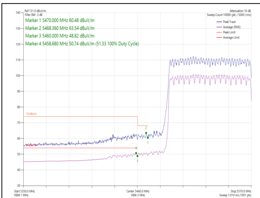
Figure 302 - 802.11ax HE80 CDD, Cores 0-1, SU - 5530 MHz Band Edge Frequency 5470 MHz
