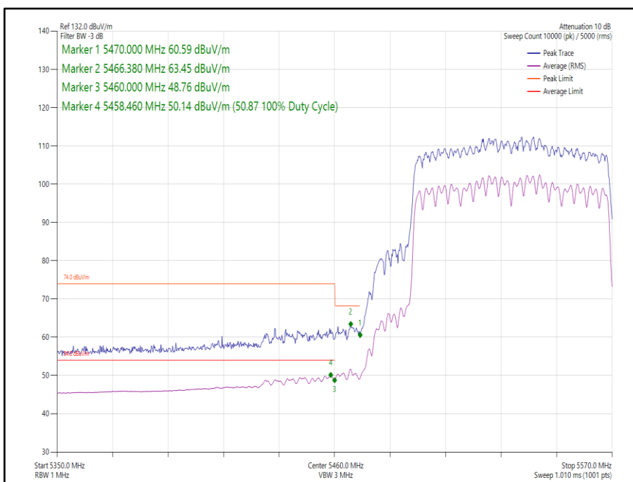
Figure 300 - 802.11ac VHT80 CDD, Cores 0-1 - 5530 MHz Band Edge Frequency 5470 MHz
