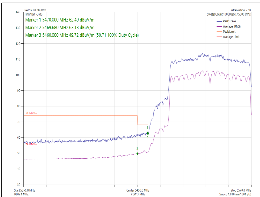
Figure 301 - 802.11ac VHT80 SDM, Cores 0-1 - 5530 MHz Band Edge Frequency 5470 MHz
