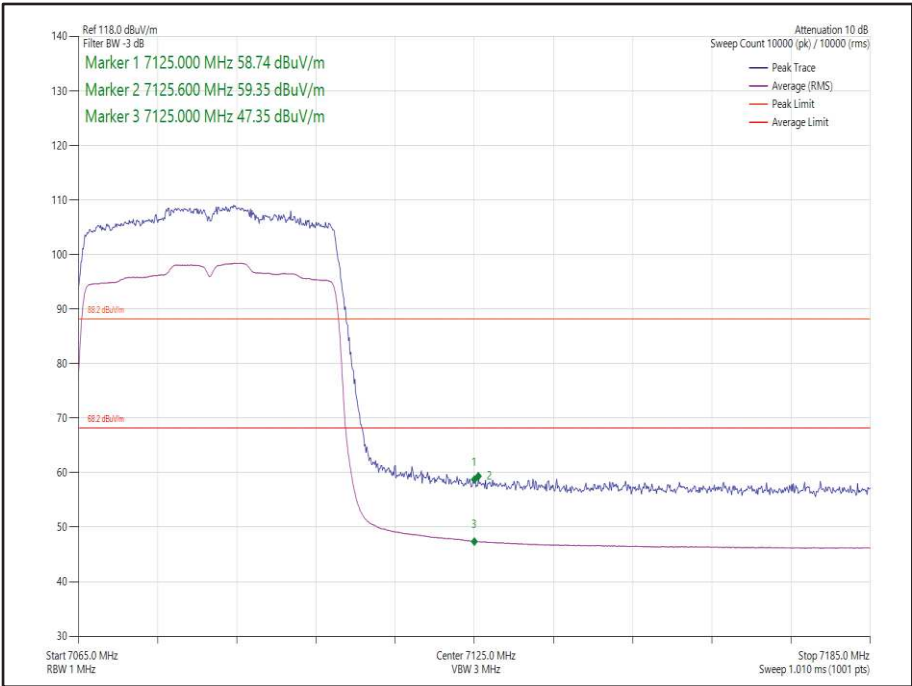
Figure 44 - 802.11ax HE40, Core 0, SU - 7085 MHz Band Edge Frequency 7125 MHz
