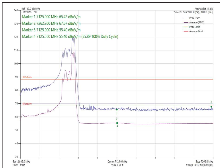
Figure 63 - 802.11ax HE80 CDD, Cores 0-1, 52-52 - 7025 MHz Band Edge Frequency 7125 MHz
