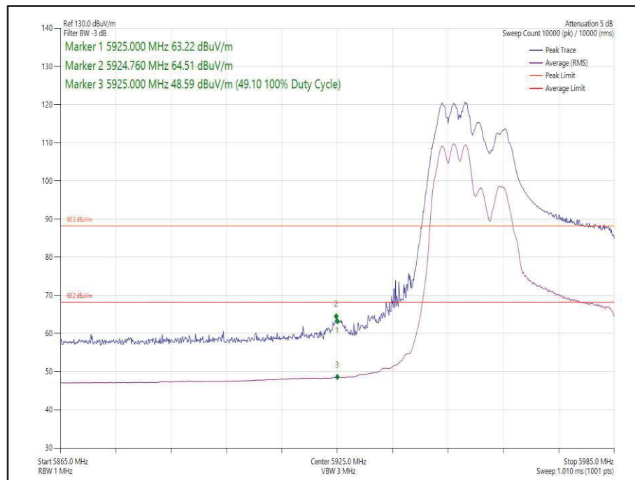
Figure 47 - 802.11ax HE40 CDD, Cores 0-1, 106-53 - 5965 MHz Band Edge Frequency 5925 MHz
