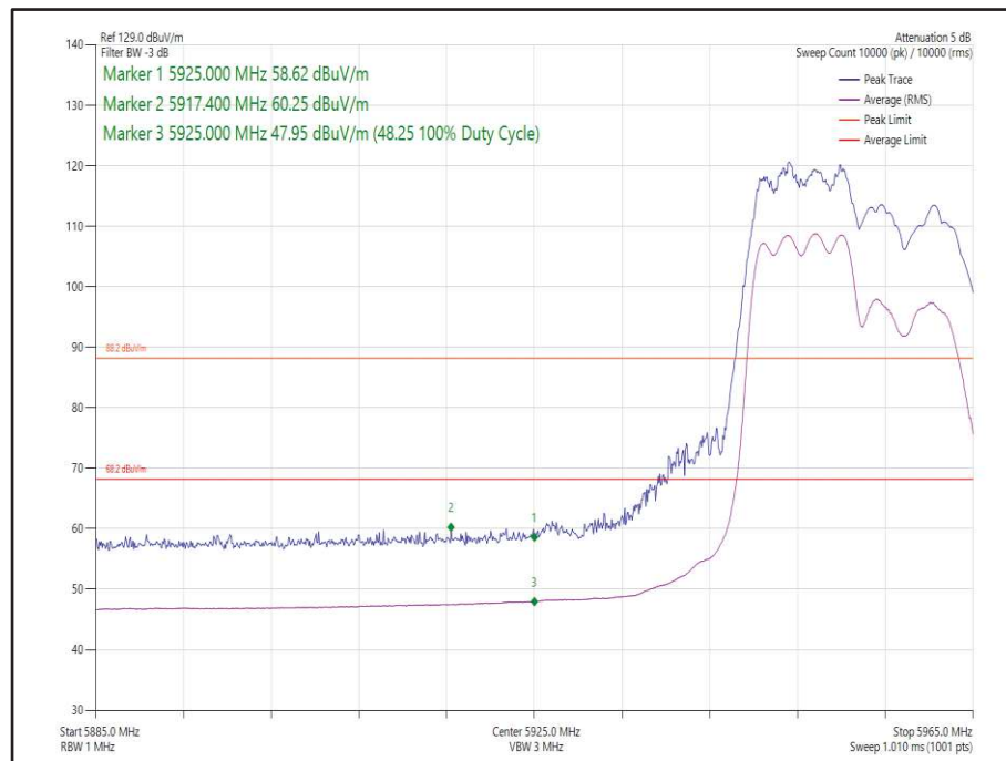
Figure 37 - 802.11ax HE20 CDD, Cores 0-1 106-53 - 5955 MHz Band Edge Frequency 5925 MHz
