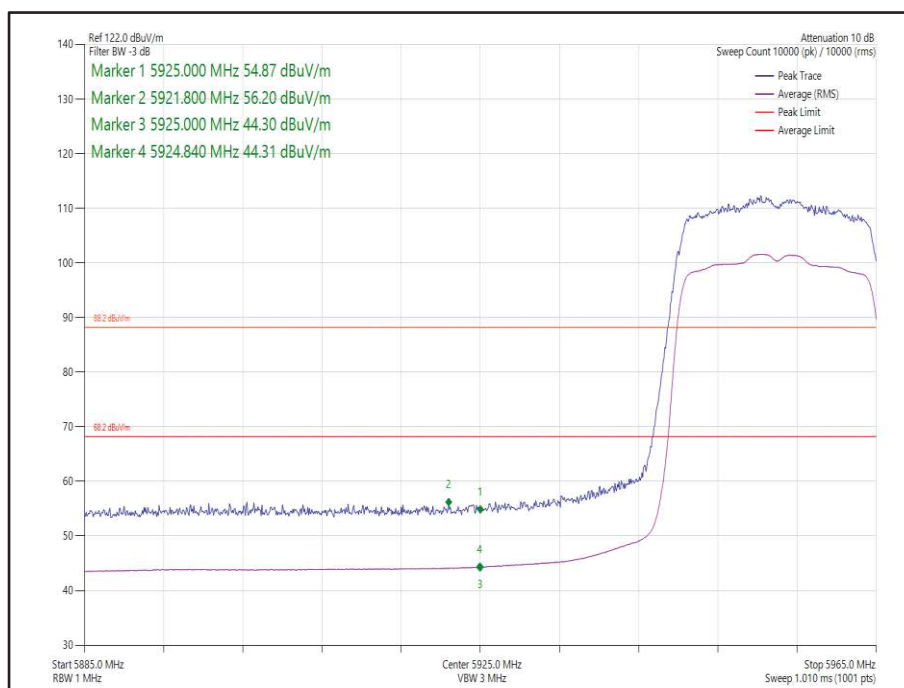
Figure 32- 802.11ax HE20, Core 1, SU - 5955 MHz, Band Edge Frequency 5925 MHz
