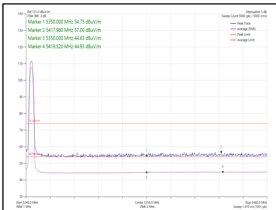
Figure 19 - Static - \pi/4 DQPSK/4-DH5 - 5245 MHz - Band Edge Frequency 5350 MHz
