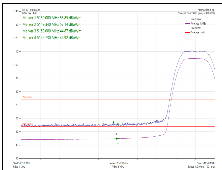
Figure 18 - Static - \pi/4 DQPSK/8-DH5 - 5162 MHz - Band Edge Frequency 5150 MHz
