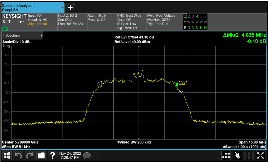
Figure 53 - Core 0 (A) 5789 MHz (CH64) 99% Bandwidth
