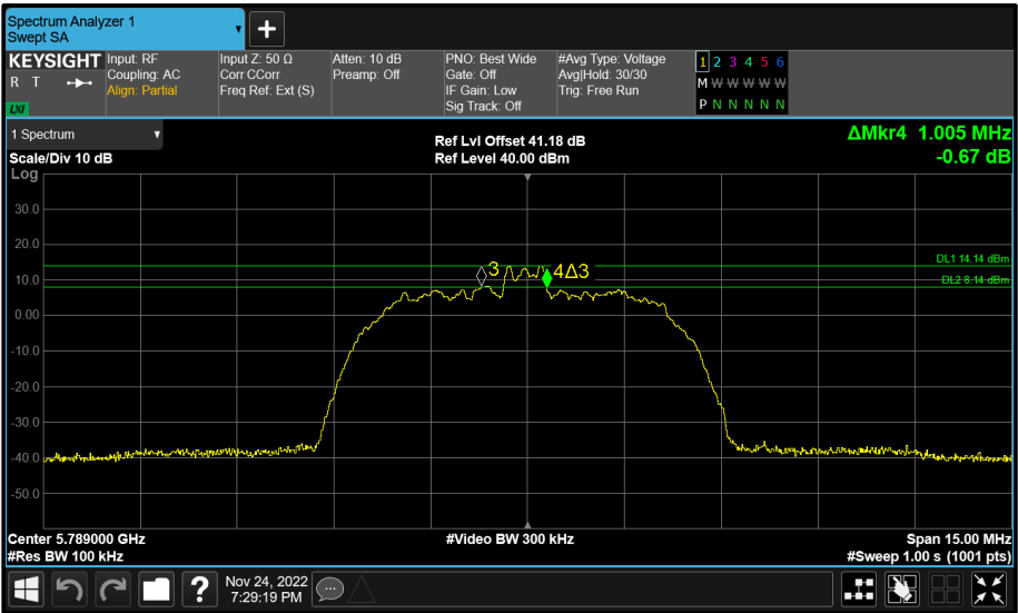
Figure 54 - Core 0 (A) 5789 MHz (CH64) 6 dB Bandwidth
