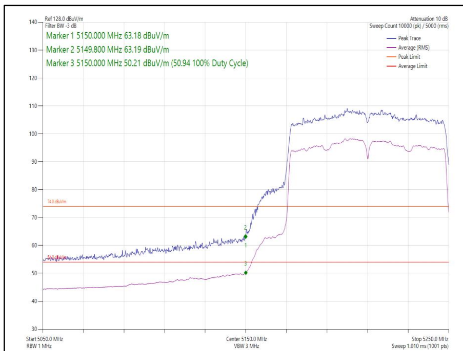
Figure 58 - 802.11ac VHT80, Core 0 - 5210 MHz, Band Edge Frequency 5150 MHz
