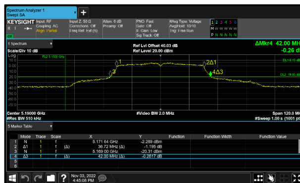
Figure 175 - 802.11n HT40 Maximum 99% OBW
