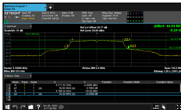
Figure 147 - 802.11n HT40 Maximum 99% OBW
