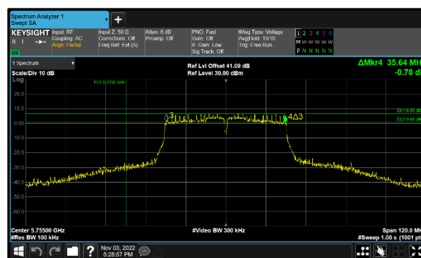
Figure 191 - 802.11n HT40 Maximum 6 dB EBW
