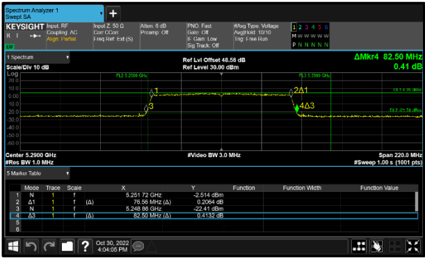
Figure 205 - 802.11ac VHT80 Maximum 99% OBW
