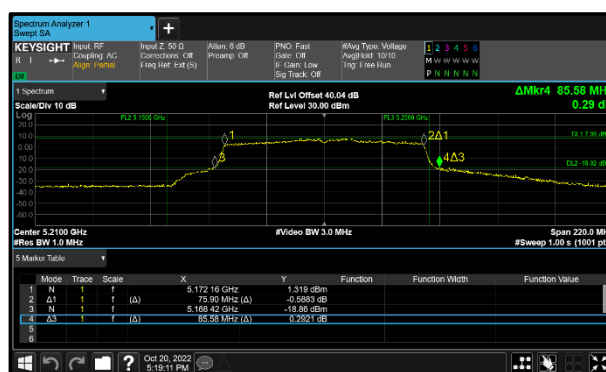
Figure 149 - 802.11ac VHT80 Maximum 99% OBW
