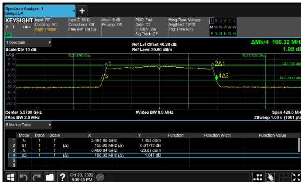
Figure 128 - 802.11ax HE160 SU Minimum 99% OBW
