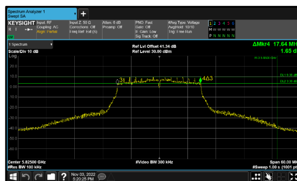
Figure 189 - 802.11n HT20 Maximum 6 dB EBW
