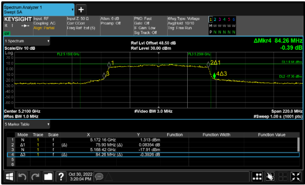
Figure 204 - 802.11ac VHT80 Minimum 99% OBW
