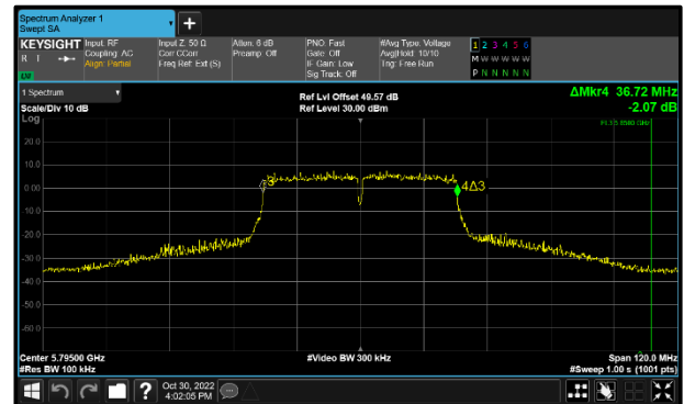
Figure 209 - 802.11n HT40 Maximum 6 dB EBW
