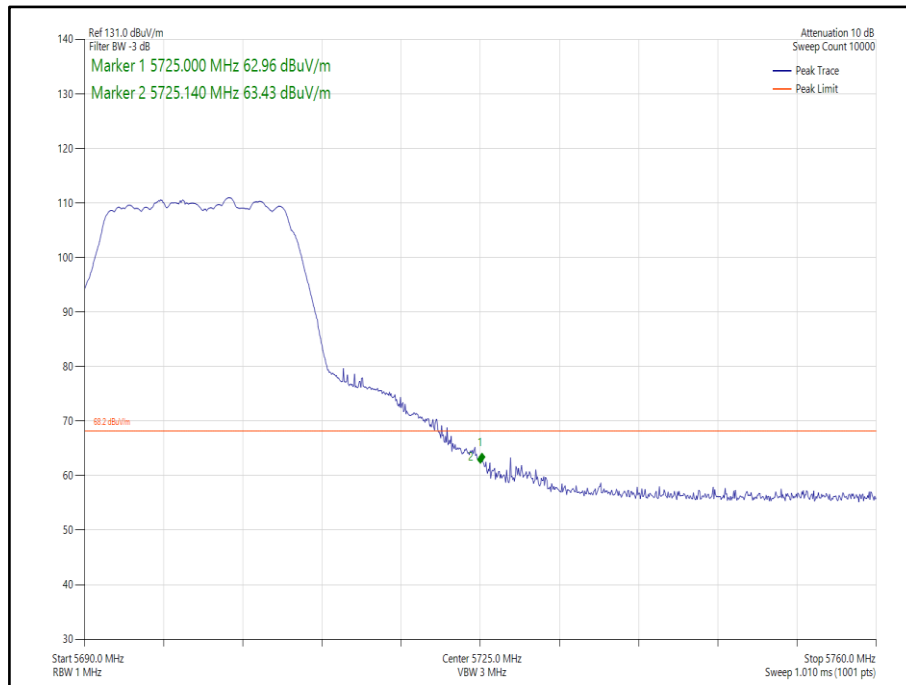
Figure 216 - 802.11a, Core 0 - 5700 MHz, Band Edge Frequency 5725 MHz
