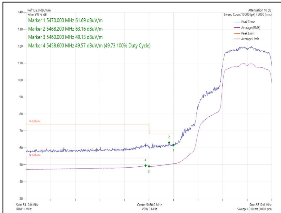
Figure 214- 802.11ax HE20, Core 0, SU - 5500 MHz, Band Edge Frequency 5470 MHz
