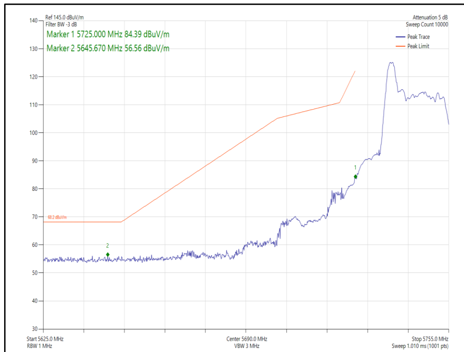
Figure 223- 802.11ax HE20, Core 0, 26-0 - 5745 MHz, Band Edge Frequency 5725 MHz
