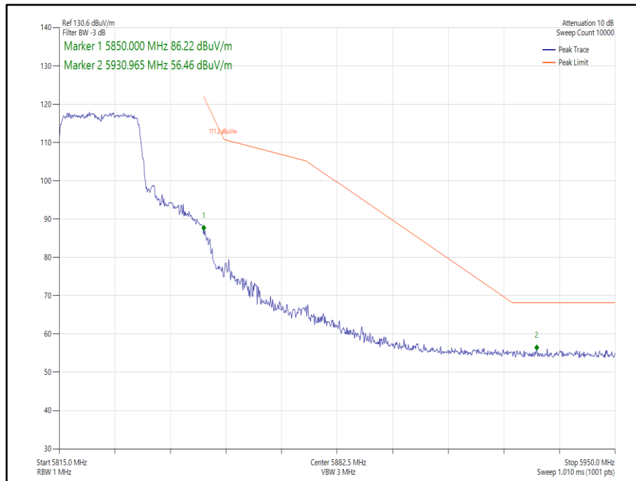
Figure 226- 802.11ax HE20, Core 0, SU - 5825 MHz, Band Edge Frequency 5850 MHz
