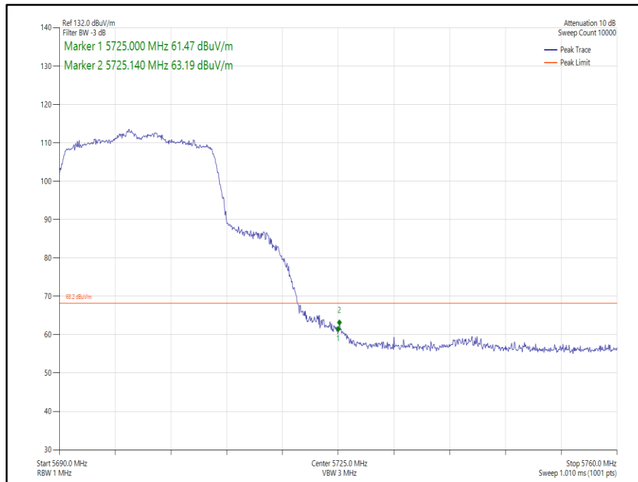
Figure 218- 802.11ax HE20, Core 0, SU - 5700 MHz, Band Edge Frequency 5725 MHz
