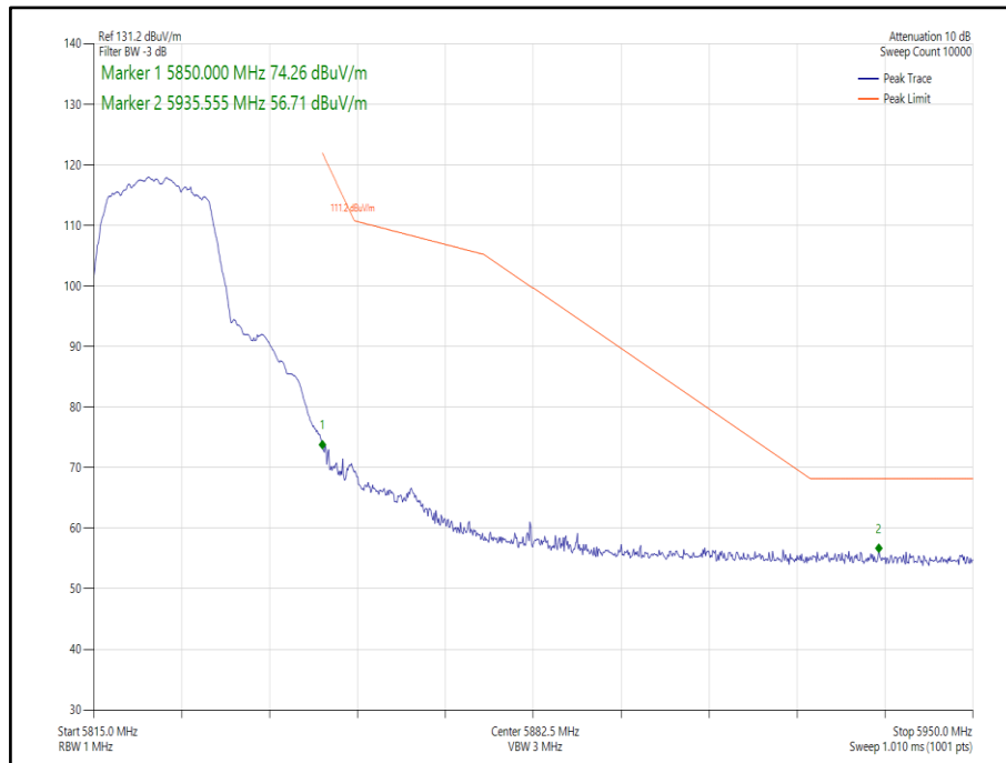
Figure 224 - 802.11a, Core 0, - 5825 MHz, Band Edge Frequency 5850 MHz
