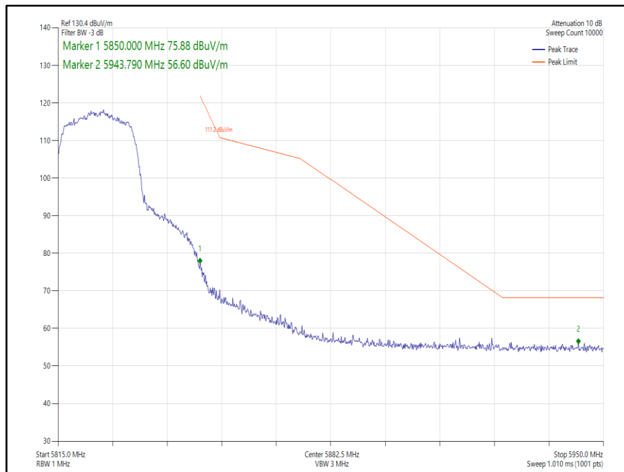
Figure 225 - 802.11n HT20, Core 0, - 5825 MHz, Band Edge Frequency 5850 MHz
