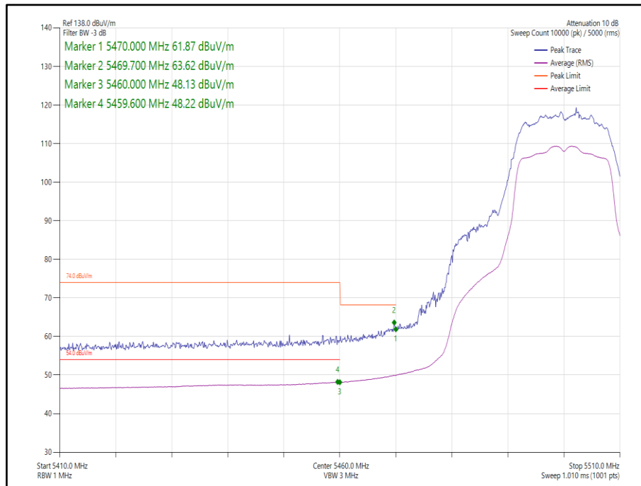
Figure 212 - 802.11a, Core 0 - 5500 MHz, Band Edge Frequency 5470 MHz
