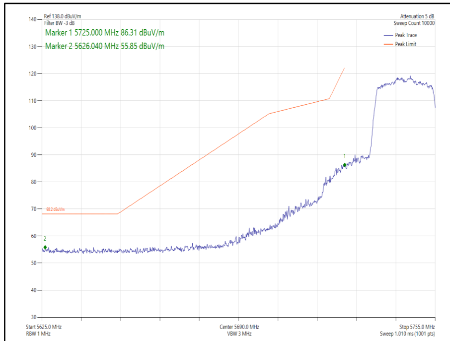
Figure 222- 802.11ax HE20, Core 0, SU - 5745 MHz, Band Edge Frequency 5725 MHz
