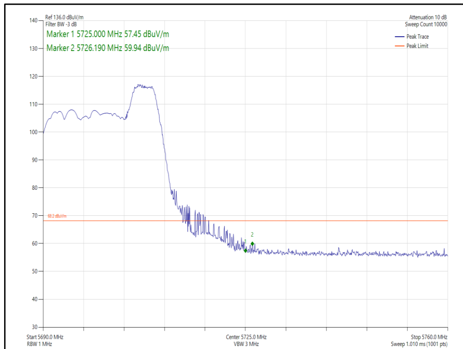
Figure 219- 802.11ax HE20, Core 0, 52-40 - 5700 MHz, Band Edge Frequency 5725 MHz
