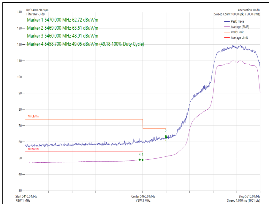
Figure 213 - 802.11n HT20, Core 0 - 5500 MHz, Band Edge Frequency 5470 MHz
