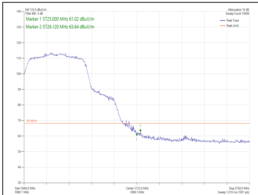
Figure 217 - 802.11n HT20, Core 0 - 5700 MHz, Band Edge Frequency 5725 MHz
