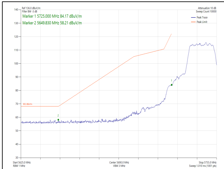
Figure 220 - 802.11a, Core 0- 5745 MHz, Band Edge Frequency 5725 MHz
