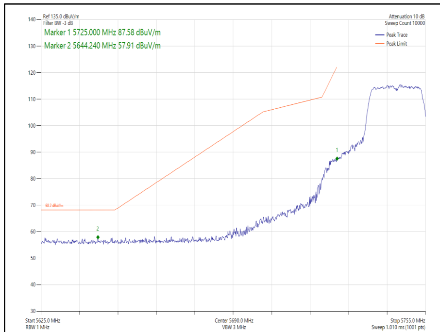
Figure 221 - 802.11n HT20, Core 0- 5745 MHz, Band Edge Frequency 5725 MHz
