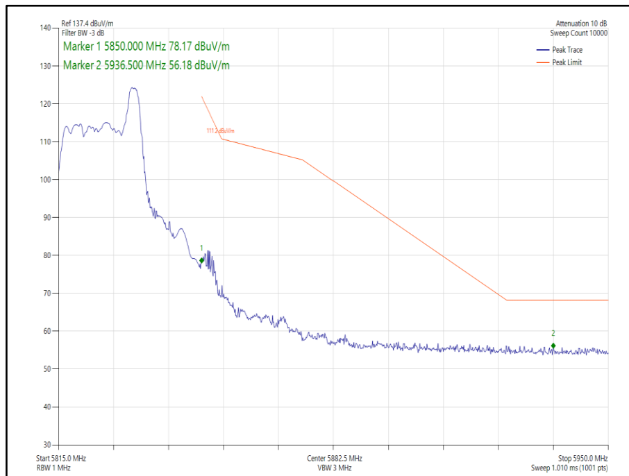
Figure 227- 802.11ax HE20, Core 0, 26-8 - 5825 MHz, Band Edge Frequency 5850 MHz
