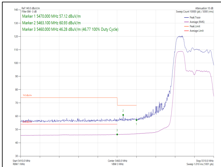
Figure 215- 802.11ax HE20, Core 0, 52-37 - 5500 MHz, Band Edge Frequency 5470 MHz
