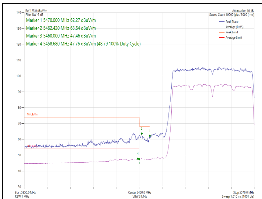
Figure 288 - 802.11ac VHT80 Core 0 - 5530 MHz, Band Edge Frequency 5470 MHz
