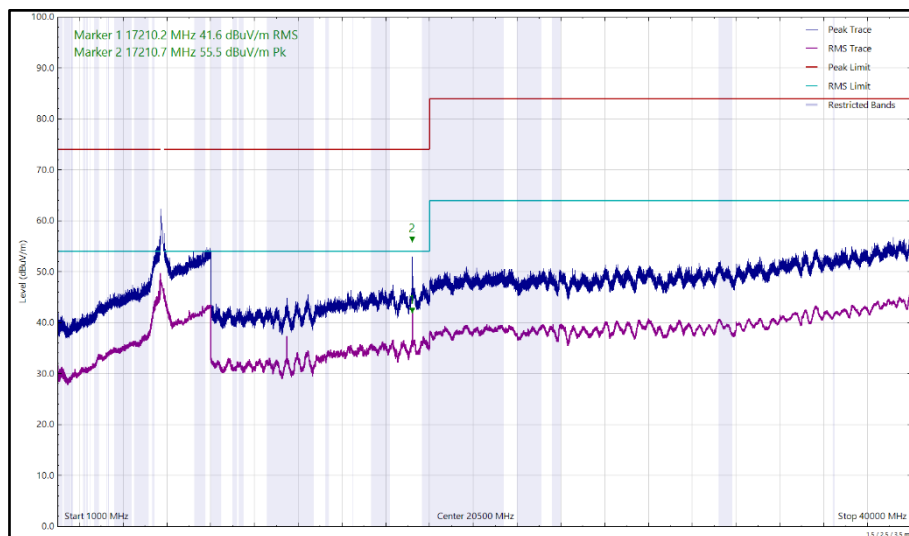
Figure 402 - U-NII-3 - 5745 MHz (CH149), HE20, RU26-0, CDD, Core 0 + Core 1, 1 GHz to 40 GHz, Vertical
