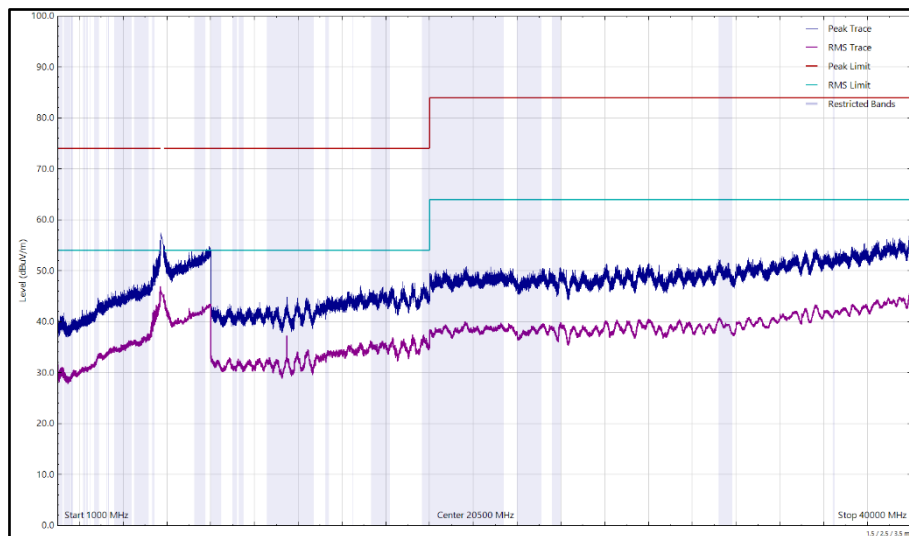
Figure 401 - U-NII-3 - 5745 MHz (CH149), HE20, RU26-0, CDD, Core 0 + Core 1, 1 GHz to 40 GHz, Horizontal
