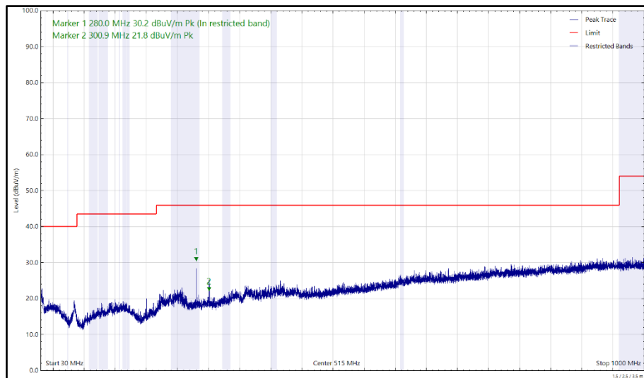
Figure 403 - U-NII-3 - 5825 MHz (CH165), HE20, RU26-0, CDD, Core 0 + Core 1, 30 MHz to 1 GHz, Horizontal (Peak)
