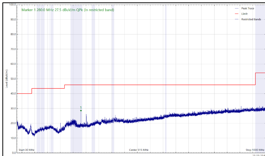
Figure 375 - U-NII-1 - 5180 MHz (CH36), VHT20, CDD, Core 0 + Core 1, 30 MHz to 1 GHz, Horizontal (Peak)
