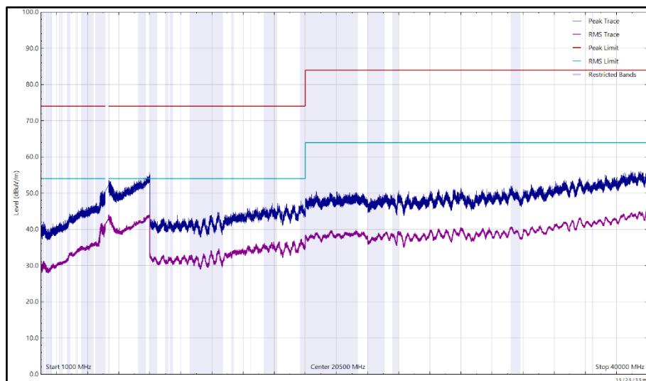
Figure 376 - U-NII-1 - 5180 MHz (CH36), VHT20, CDD, Core 0 + Core 1, 1 GHz to 40 GHz, Horizontal
