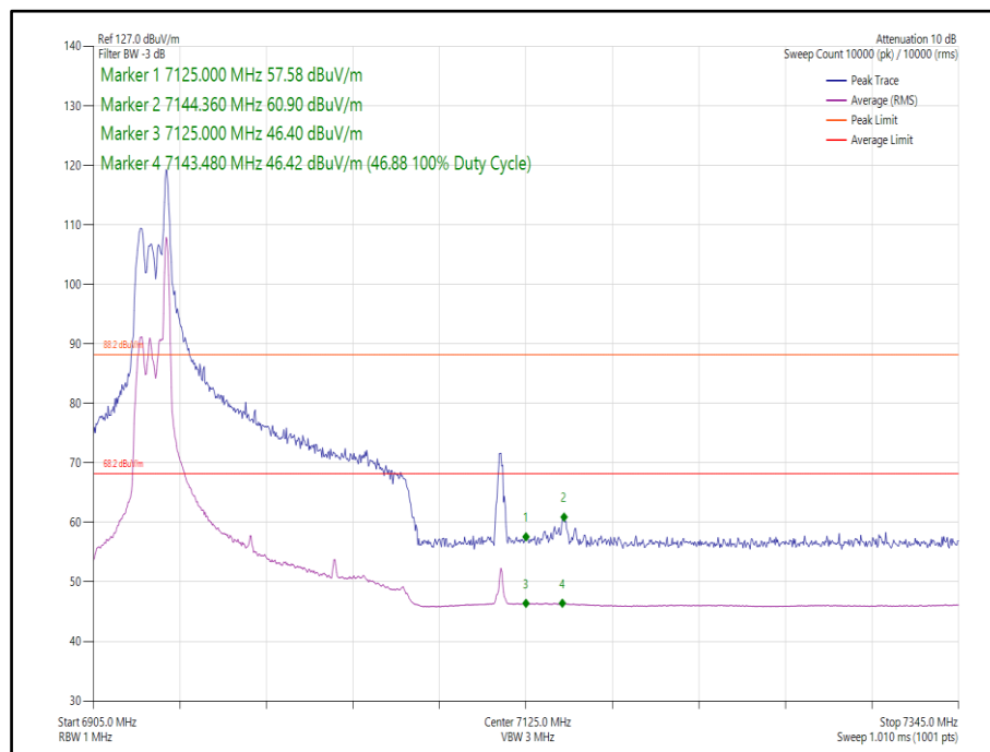
Figure 77 - 802.11ax HE160 SDM, Cores 0-1, 26-17 - 6985 MHz Band Edge Frequency 7125 MHz
