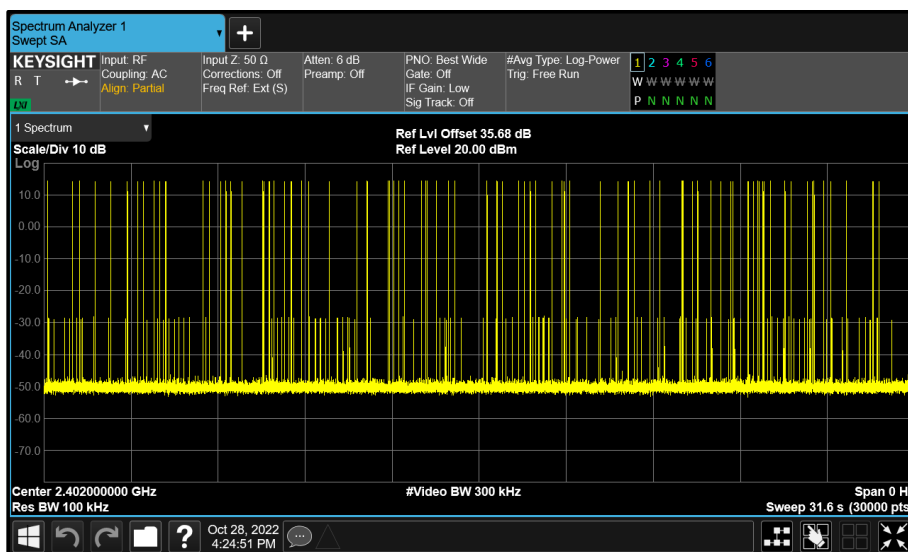
Figure 29 - \pi/4 DQPSK - 2402 MHz Accumulated Transmit Time
