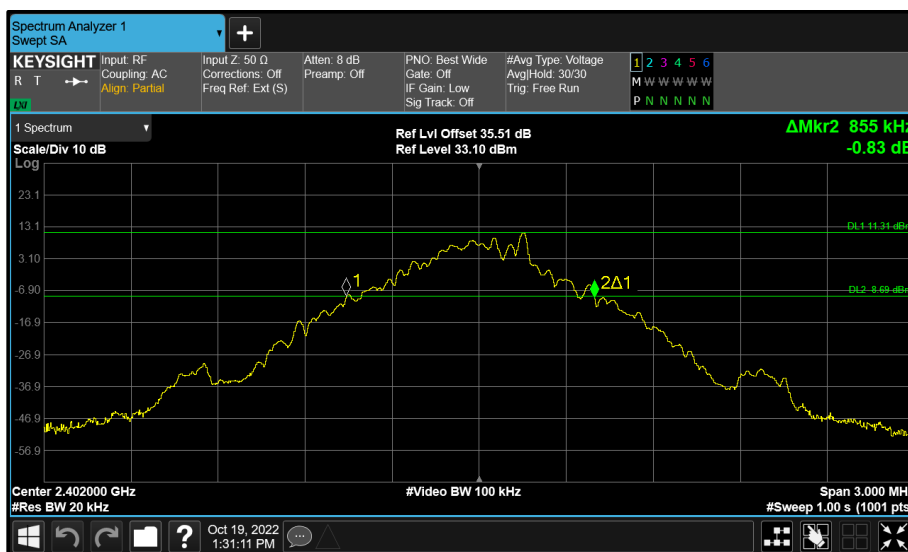
Figure 76 - Core 2 (C) 2402 MHz (CH0) 20 dB Bandwidth
