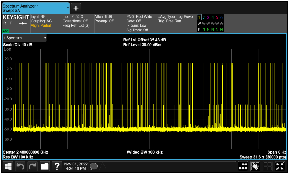
Figure 28 - \pi/4 DQPSK - 2480 MHz Accumulated Transmit Time
