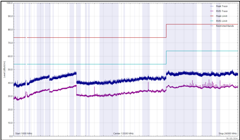
Figure 99 - 2412 MHz (CH1), HT20, CDD, Core 0 + Core 1, 1 GHz to 26 GHz, Vertical
