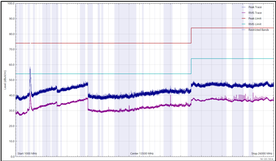
Figure 69 - 2437 MHz (CH6), 802.11b, Core 1, 1 GHz to 26 GHz, Horizontal
