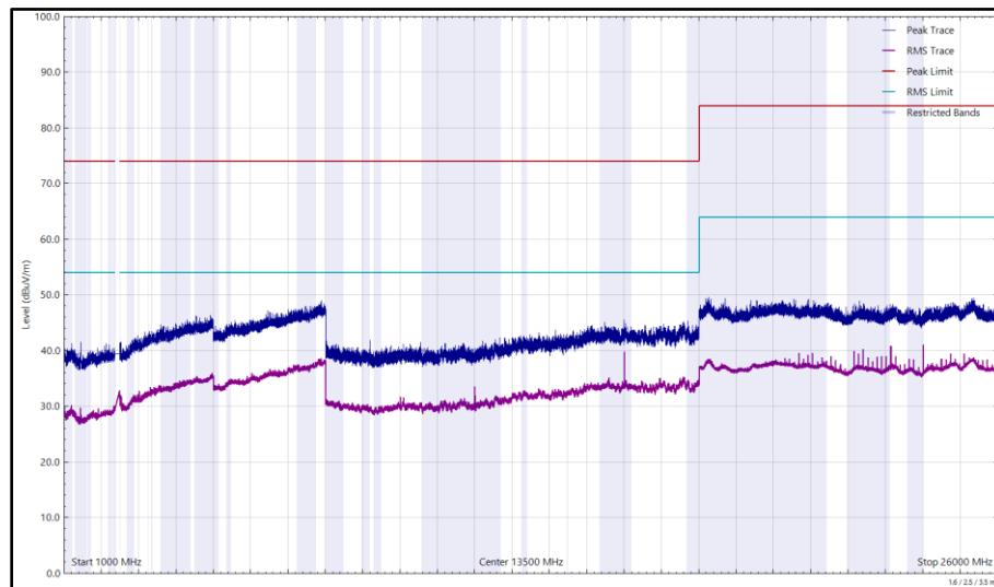
Figure 75 - 2412 MHz (CH1), 802.11g, Core 0, 1 GHz to 26 GHz, Vertical
