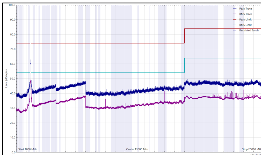
Figure 101 - 2437 MHz (CH6), HT20, CDD, Core 0 + Core 1, 1 GHz to 26 GHz, Horizontal
