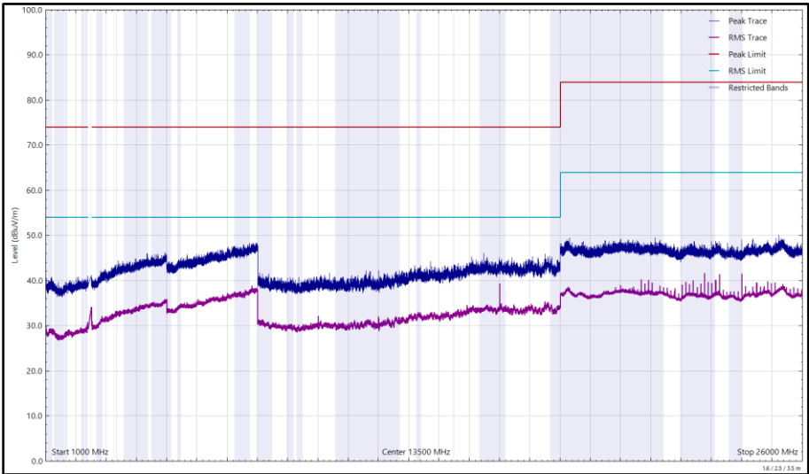
Figure 65 - 2472 MHz (CH13), 802.11b, Core 0, 1 GHz to 26 GHz, Vertical
