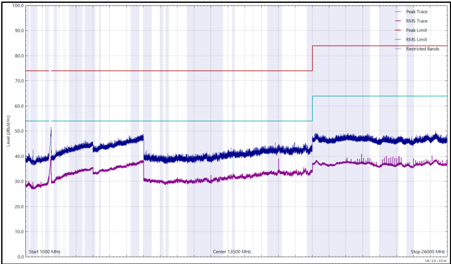
Figure 81 - 2472 MHz (CH13), 802.11g, Core 0, 1 GHz to 26 GHz, Vertical
