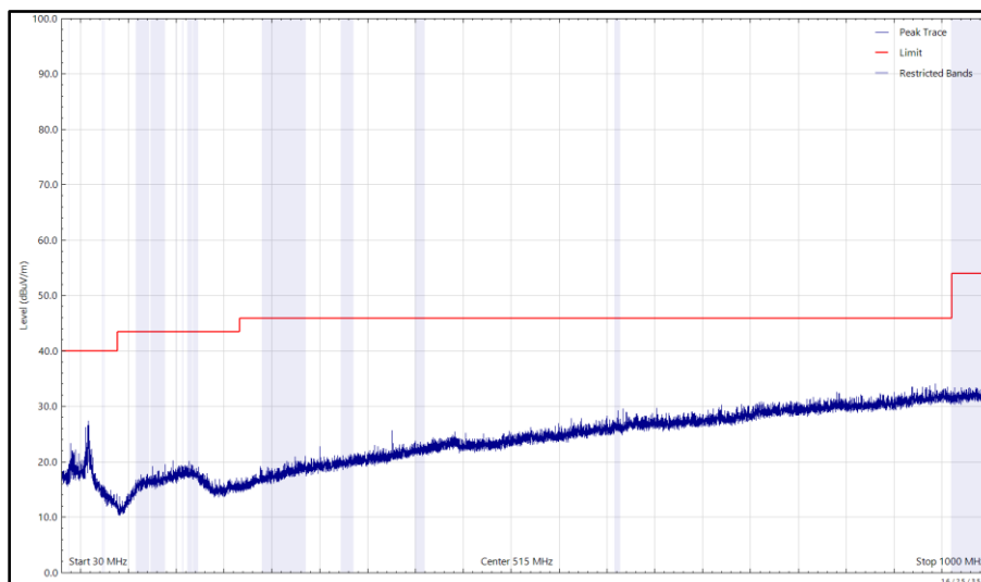
Figure 100 - 2437 MHz (CH6), HT20, CDD, Core 0 + Core 1, 30 MHz to 1 GHz, Horizontal (Peak)
