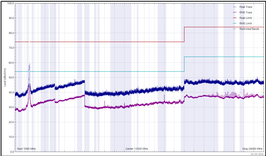
Figure 77 - 2437 MHz (CH6), 802.11g, Core 0, 1 GHz to 26 GHz, Horizontal
