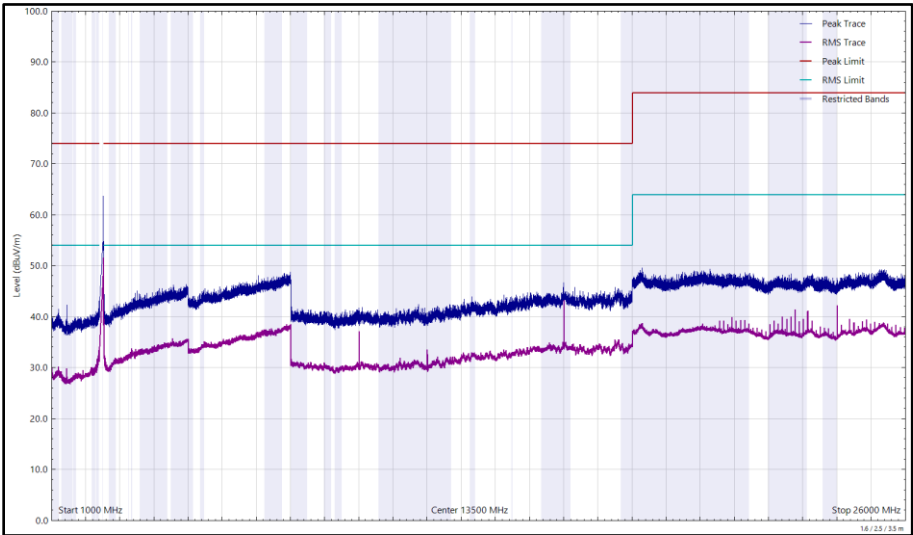
Figure 105 - 2472 MHz (CH13), HT20, CDD, Core 0 + Core 1, 1 GHz to 26 GHz, Vertical
