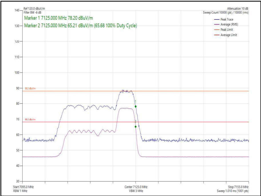
Figure 44 - 802.11ax, HE20, RU52-40, SISO, Core 1 - 7115 MHz, Band Edge Frequency 7125 MHz
