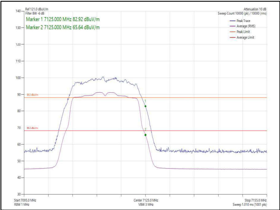
Figure 40 - 802.11a, SISO, Core 1 - 7115 MHz, Band Edge Frequency 7125 MHz
