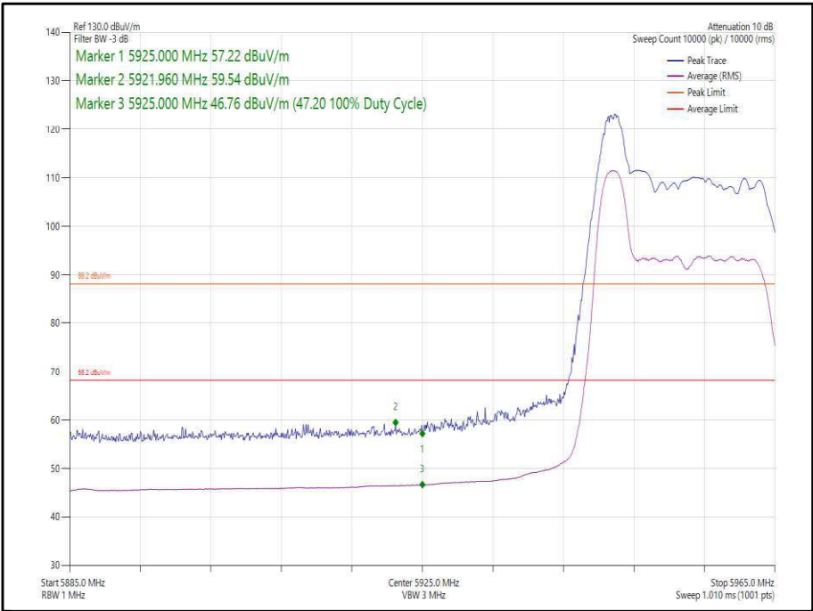
Figure 38 - 802.11ax, HE20, RU26-0, SISO, Core 1 - 5955 MHz, Band Edge Frequency 5925 MHz
