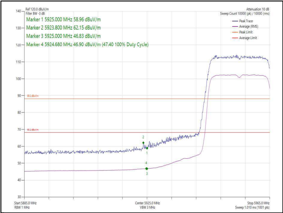
Figure 37 - 802.11ax, HE20, SU, SISO, Core 1 - 5955 MHz, Band Edge Frequency 5925 MHz
