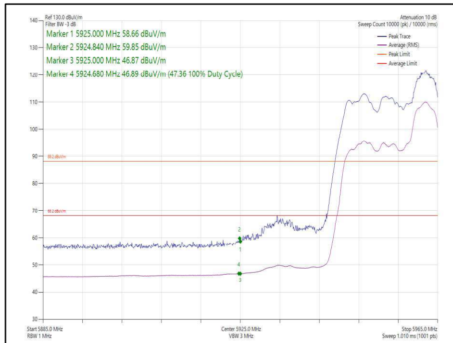
Figure 52 - 802.11ax, HE20, RU52-40, SDM, Core 0-1 - 5955 MHz, Band Edge Frequency 5925 MHz
