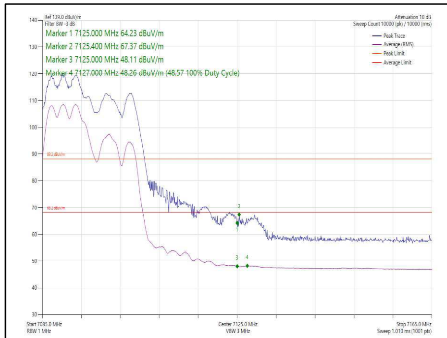
Figure 48 - 802.11ax, HE20, RU106-53, CDD, Core 0-1 - 7095 MHz, Band Edge Frequency 7125 MHz
