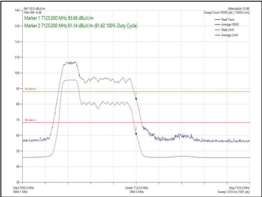
Figure 35 - 802.11ax, HE20, RU52-37, SISO, Core 0 - 7115 MHz, Band Edge Frequency 7125 MHz
