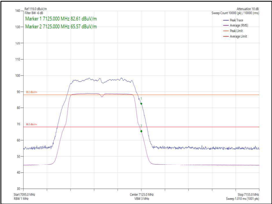
Figure 31 - 802.11a, SISO, Core 0 - 7115 MHz, Band Edge Frequency 7125 MHz
