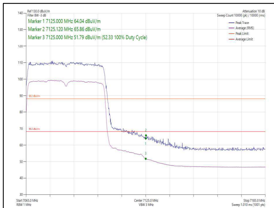
Figure 63 - 802.11ax, HE40, SU, SISO, Core 1 - 7085 MHz, Band Edge Frequency 7125 MHz
