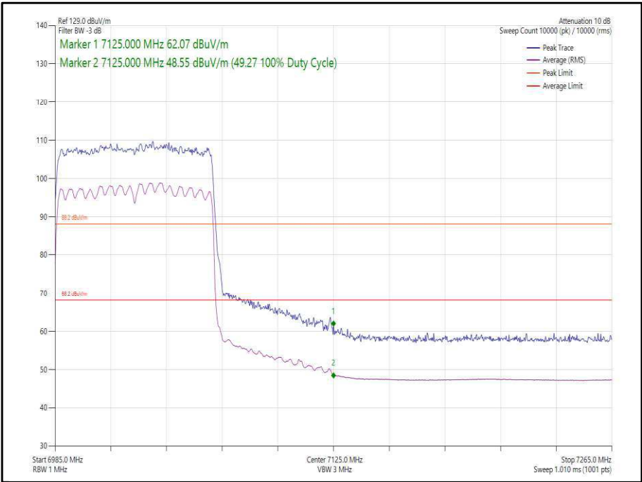
Figure 87 - 802.11ax, HE80, SU2, SDM, Core 0-1 - 7025 MHz, Band Edge Frequency 7125 MHz
