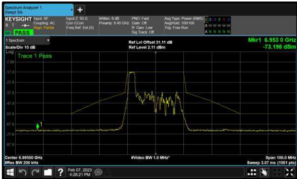
Figure 126 – D (Core 1) 802.11ax HE20 RU26 6995 MHz (CH209)
