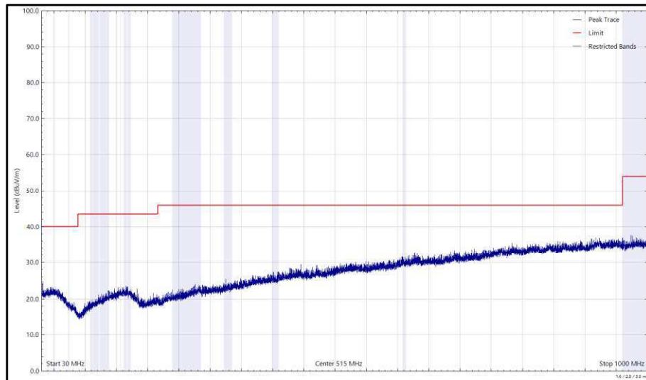
Figure 151 - U-NII-7 - 6695 MHz (CH149), HE20, SU, CDD, Core 0 + Core 1, 30 MHz to 1 GHz, Horizontal (Peak)
