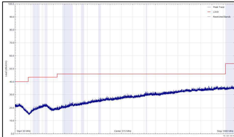
Figure 143 - U-NII-6 - 6475 MHz (CH105), HE20, SU, CDD, Core 0 + Core 1, 30 MHz to 1 GHz, Horizontal (Peak)
