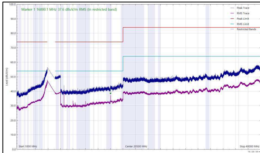
Figure 139 - U-NII-5 - 6415 MHz (CH93), HE20, SU, CDD, Core 0 + Core 1, 1 GHz to 40 GHz, Horizontal
