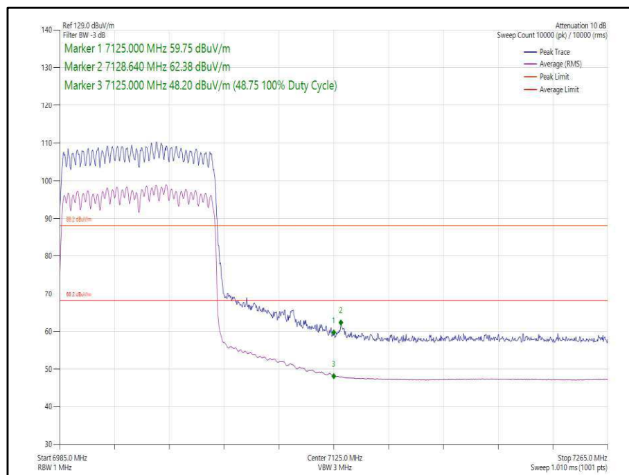
Figure 83 - 802.11ax, HE80, SU, CDD, Core 0-1 - 7025 MHz, Band Edge Frequency 7125 MHz
