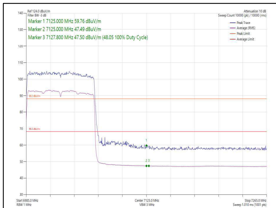
Figure 75 - 802.11ax, HE80, SU, SISO, Core 0 - 7025 MHz, Band Edge Frequency 7125 MHz
