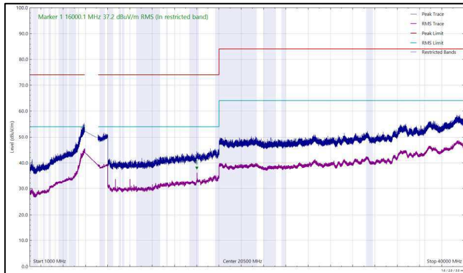
Figure 147 - U-NII-6 - 6515 MHz (CH113), HE20, SU, CDD, Core 0 + Core 1, 1 GHz to 40 GHz, Horizontal
