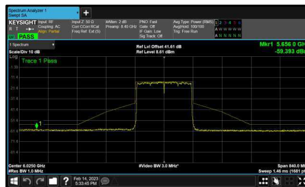
Figure 124 – A (Core 0) 802.11ax HE160 SU 6025 MHz (CH15)
