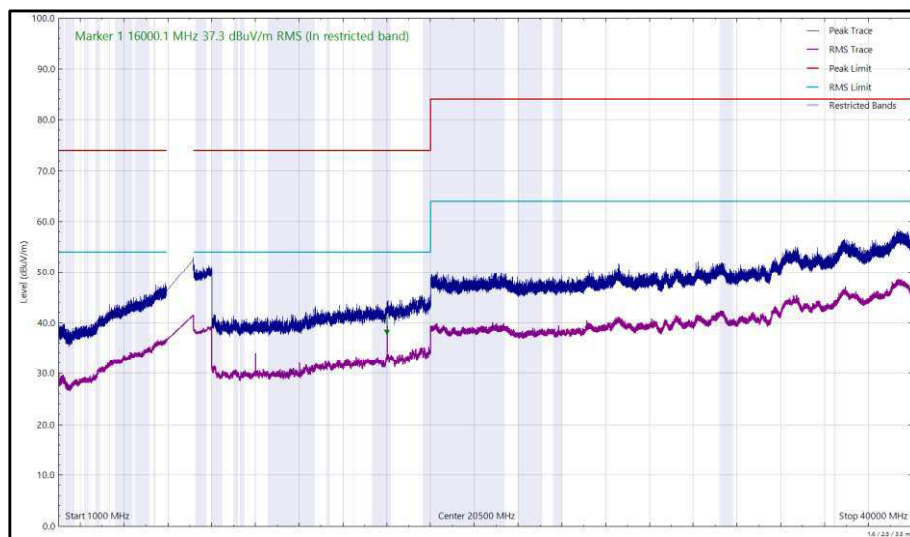
Figure 156 - U-NII-7 - 6855 MHz (CH181), HE20, SU, CDD, Core 0 + Core 1, 1 GHz to 40 GHz, Vertical
