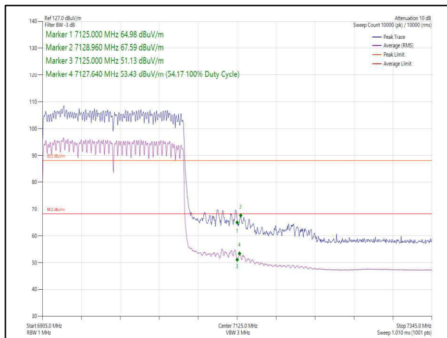
Figure 101 - 802.11ax, HE160, SU, CDD, Core 0-1 - 6985 MHz, Band Edge Frequency 7125 MHz
