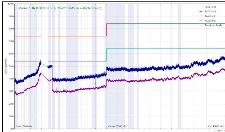
Figure 149 - U-NII-7 - 6535 MHz (CH117), HE20, SU, CDD, Core 0 + Core 1, 1 GHz to 40 GHz, Horizontal
