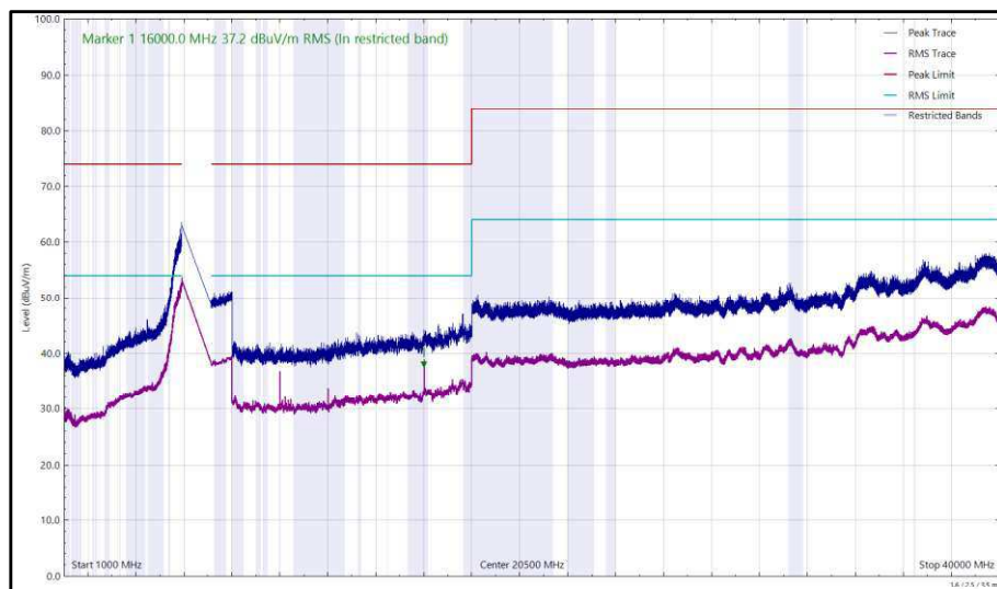
Figure 133 - U-NII-5 - 5955 MHz (CH1), HE20, SU, CDD, Core 0 + Core 1, 1 GHz to 40 GHz, Horizontal
