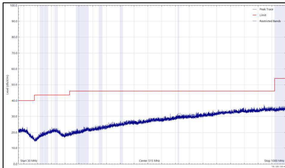
Figure 135 - U-NII-5 - 6175 MHz (CH45), HE20, SU, CDD, Core 0 + Core 1, 30 MHz to 1 GHz, Horizontal (Peak)
