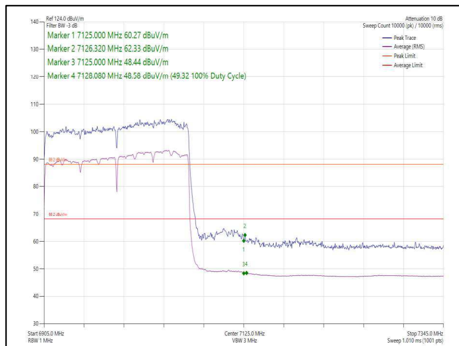
Figure 97 - 802.11ax, HE160, SU, SISO, Core 1 - 6985 MHz, Band Edge Frequency 7125 MHz
