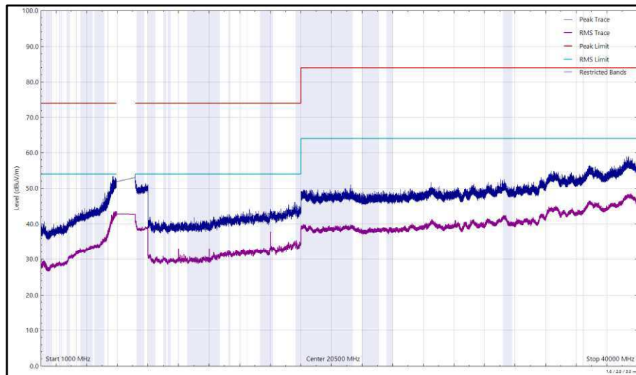
Figure 155 - U-NII-7 - 6855 MHz (CH181), HE20, SU, CDD, Core 0 + Core 1, 1 GHz to 40 GHz, Horizontal
