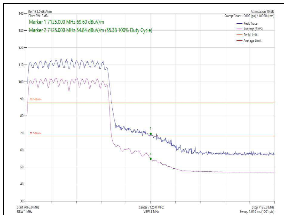
Figure 67 - 802.11ax, HE40, SU, CDD, Core 0-1 - 7085 MHz, Band Edge Frequency 7125 MHz
