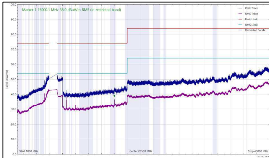
Figure 157 - U-NII-8 - 6895 MHz (CH189), HE20, SU, CDD, Core 0 + Core 1, 1 GHz to 40 GHz, Horizontal
