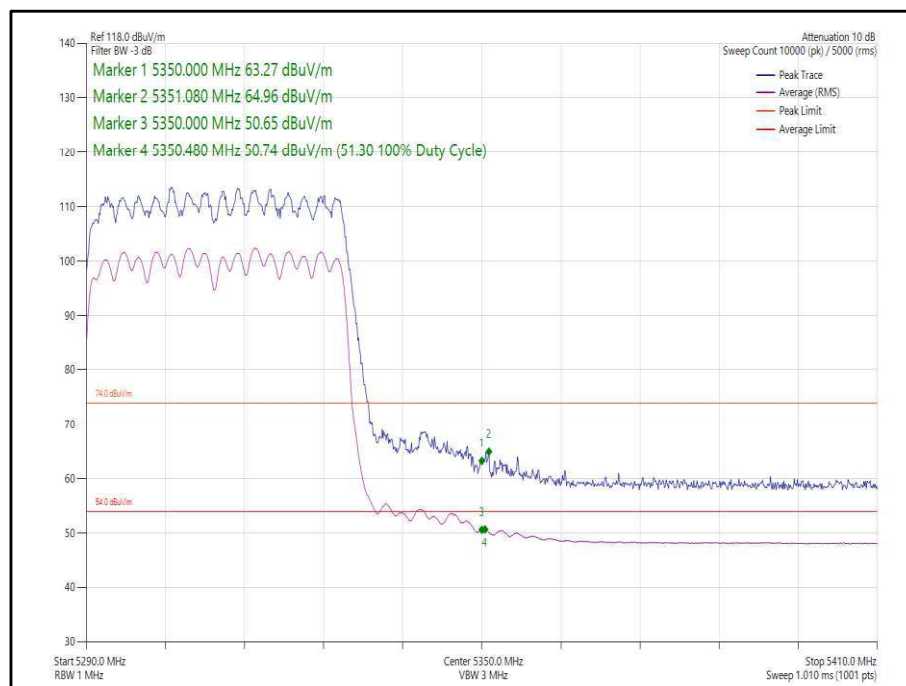
Figure 71 - 802.11ax, HE40, SU, CDD, Core 0-1 - 5310 MHz, Band Edge Frequency 5350 MHz
