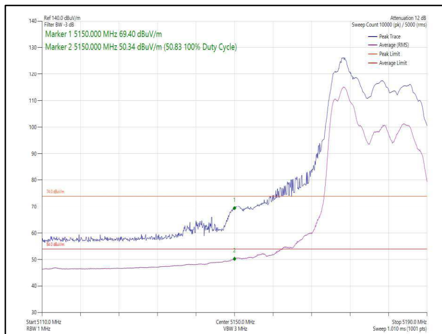
Figure 27 - 802.11ax, HE20, RU 52-37, CDD, Core 0-1 - 5180 MHz, Band Edge Frequency 5150 MHz
