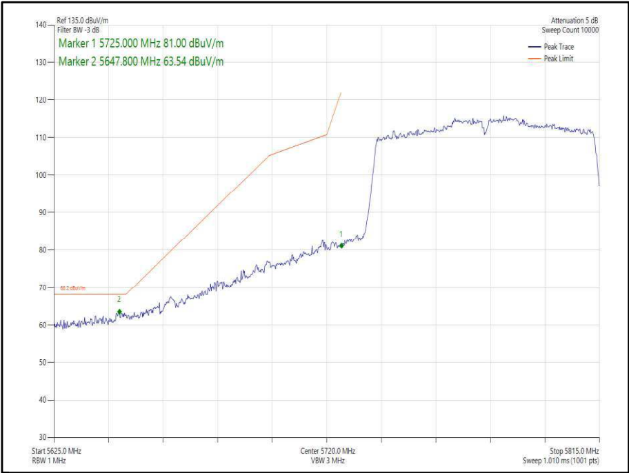
Figure 404 - 802.11ac, VHT80, SISO, Core 1 - 5775 MHz, Band Edge Frequency 5725 MHz
