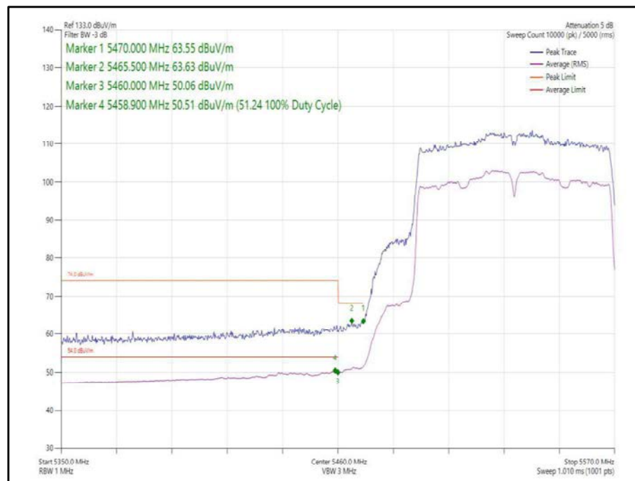
Figure 401 - 802.11ac, VHT80, SISO, Core 1 - 5530 MHz, Band Edge Frequency 5470 MHz
