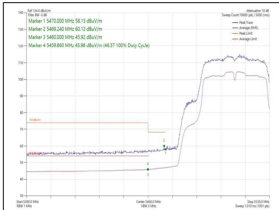
Figure 381 - 802.11n, HT40, TxBF, Core 0-1 - 5510 MHz, Band Edge Frequency 5470 MHz
