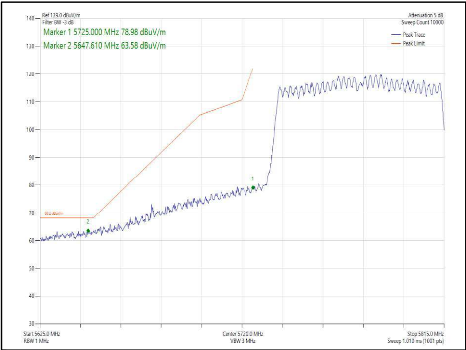
Figure 417 - 802.11ax, HE80, SU, CDD, Core 0-1 - 5775 MHz, Band Edge Frequency 5725 MHz
