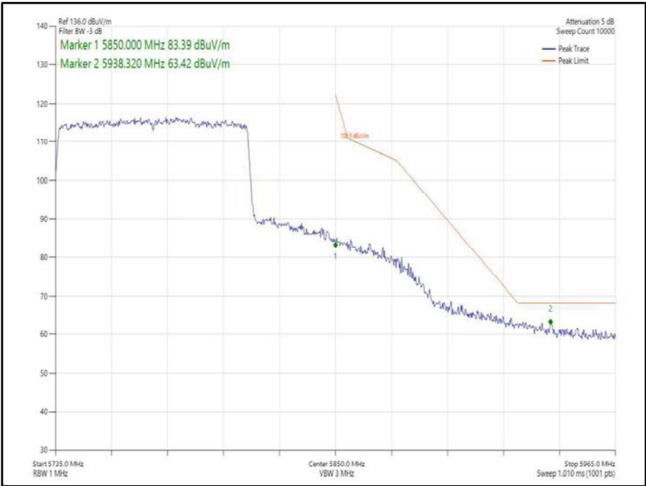
Figure 399 - 802.11ax, HE80, SU, SISO, Core 0 - 5775 MHz, Band Edge Frequency 5850 MHz
