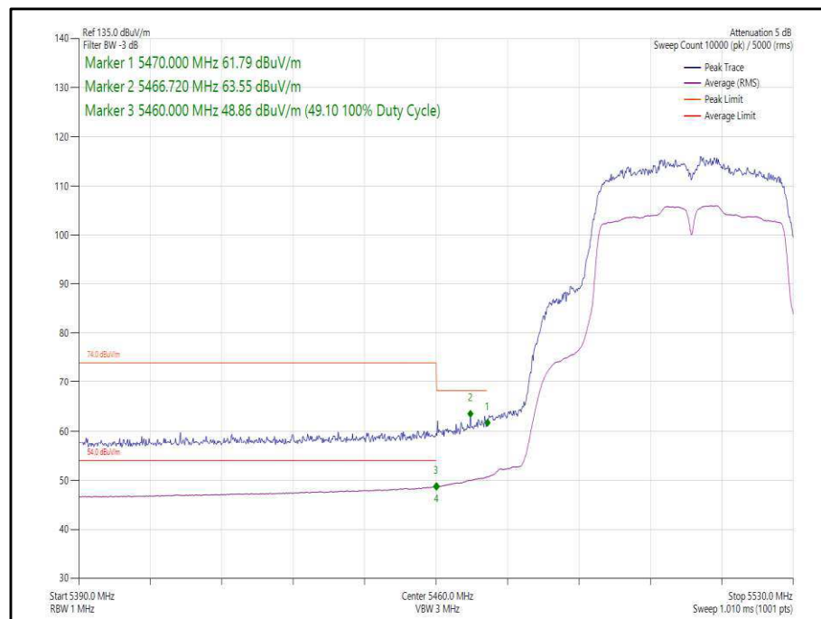
Figure 345 - 802.11n, HT40, SISO, Core 1 - 5510 MHz, Band Edge Frequency 5470 MHz
