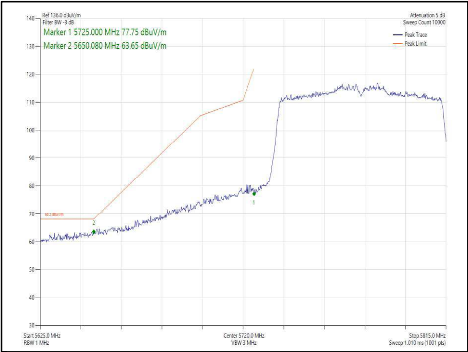
Figure 392 - 802.11ac, VHT80, SISO, Core 0 - 5775 MHz, Band Edge Frequency 5725 MHz
