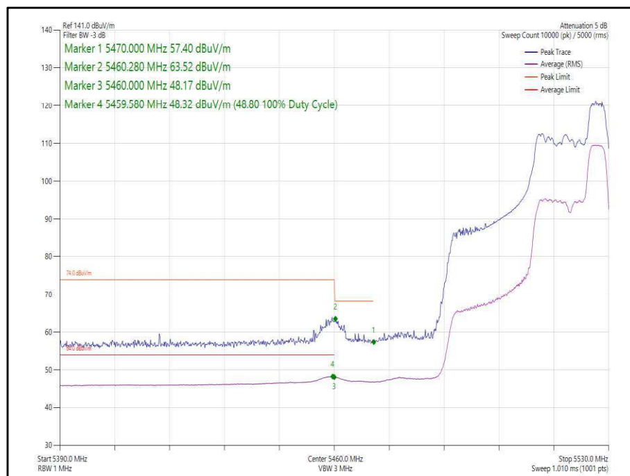
Figure 347 - 802.11ax, HE40, RU 52-44, SISO, Core 1 - 5510 MHz, Band Edge Frequency 5470 MHz
