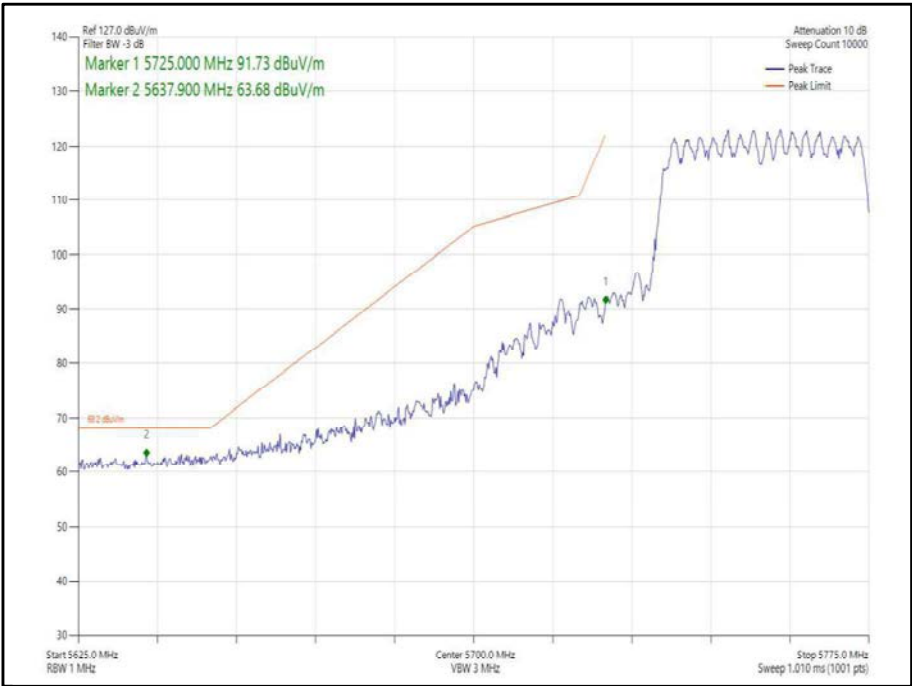
Figure 361 - 802.11ax, HE40, SU, CDD, Core 0-1 - 5755 MHz, Band Edge Frequency 5725 MHz
