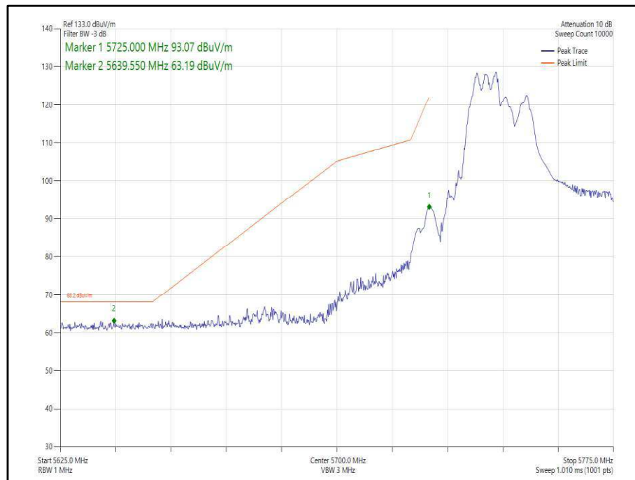
Figure 362 - 802.11ax, HE40, RU 106-53, CDD, Core 0-1 - 5755 MHz, Band Edge Frequency 5725 MHz
