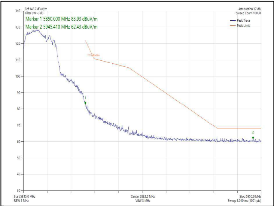
Figure 331 - 802.11n, HT20 TxBF, Core 0-1 - 5825 MHz, Band Edge Frequency 5850 MHz
