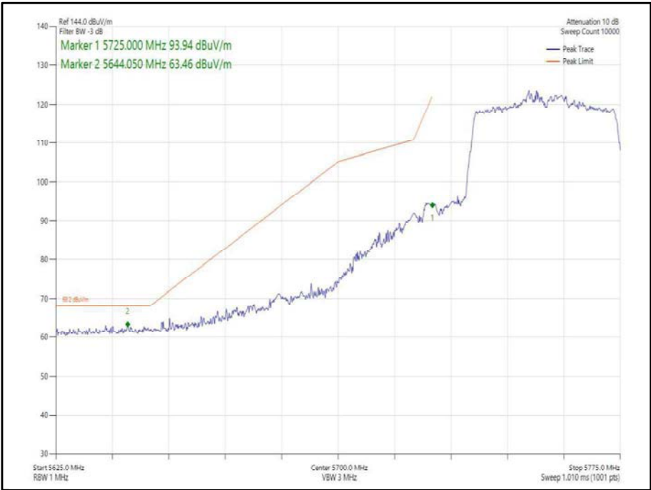
Figure 373 - 802.11ax, HE40, SU, SDM, Core 0-1 - 5755 MHz, Band Edge Frequency 5725 MHz
