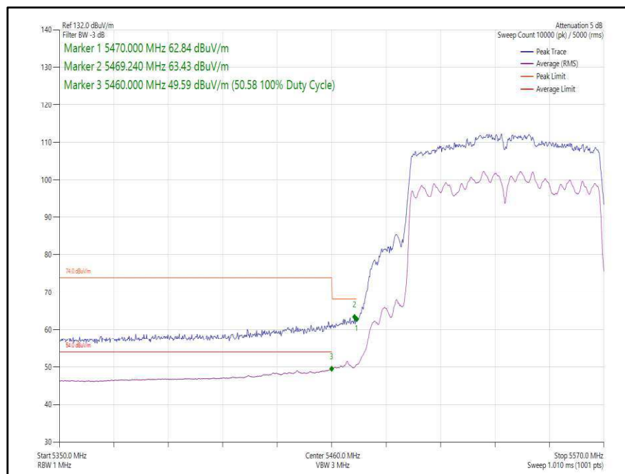
Figure 428 - 802.11ac, VHT80, SDM, Core 0-1 - 5530 MHz, Band Edge Frequency 5470 MHz
