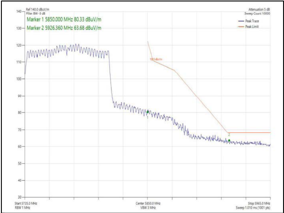
Figure 426 - 802.11ax, HE80, SU, CDD, Core 0-1 - 5775 MHz, Band Edge Frequency 5850 MHz
