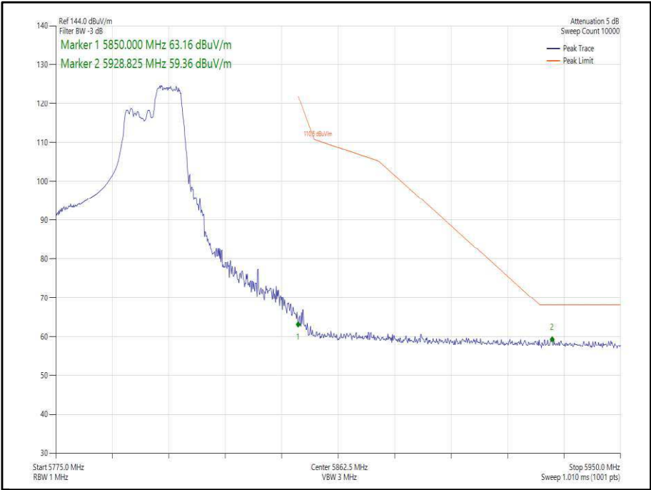
Figure 344 - 802.11ax, HE40, RU 106-56, SISO, Core 0 - 5795 MHz, Band Edge Frequency 5850 MHz
