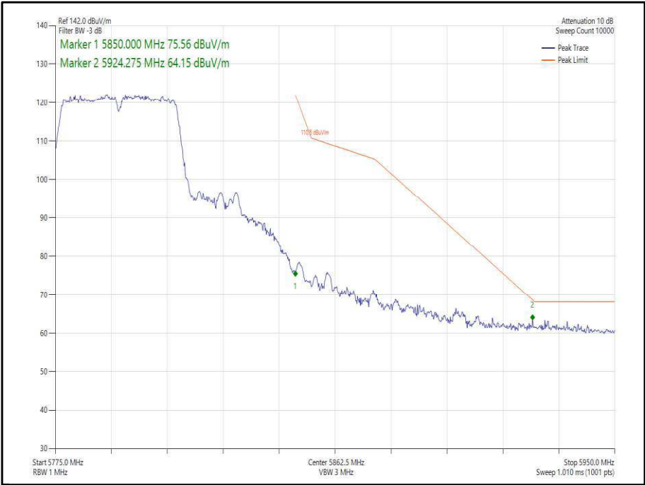
Figure 378 - 802.11n, HT40, SDM, Core 0-1 - 5795 MHz, Band Edge Frequency 5850 MHz
