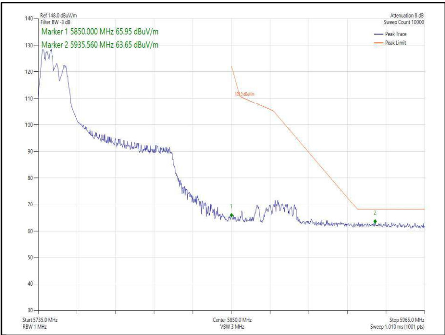
Figure 427 - 802.11ax, HE80, RU 106-60, CDD, Core 0-1 - 5775 MHz, Band Edge Frequency 5850 MHz
