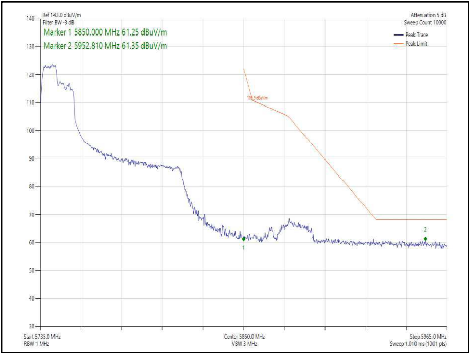
Figure 412 - 802.11ax, HE80, RU 106-53, SISO, Core 1 - 5775 MHz, Band Edge Frequency 5850 MHz
