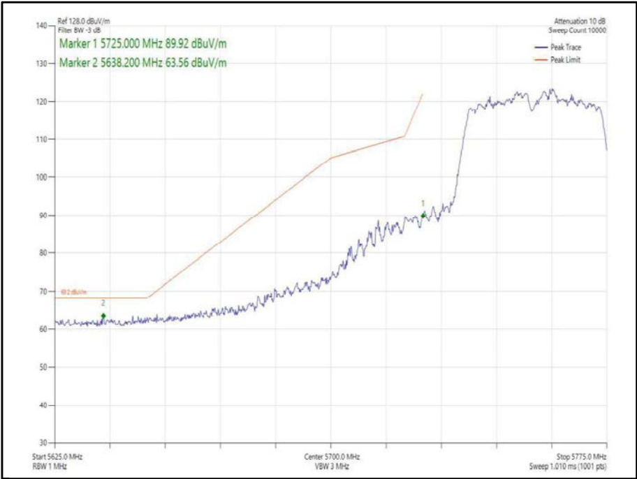
Figure 360 - 802.11n, HT40, CDD, Core 0-1 - 5755 MHz, Band Edge Frequency 5725 MHz
