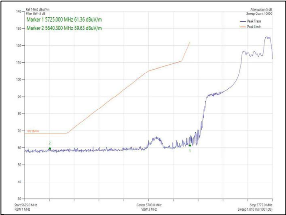
Figure 338 - 802.11ax, HE40, RU 52-44, SISO, Core 0 - 5755 MHz, Band Edge Frequency 5725 MHz
