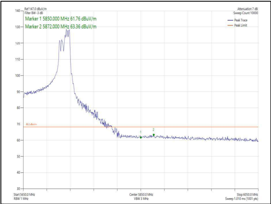
Figure 425 - 802.11ax, HE80, RU 106-60, CDD, Core 0-1 - 5690 MHz, Band Edge Frequency 5850 MHz
