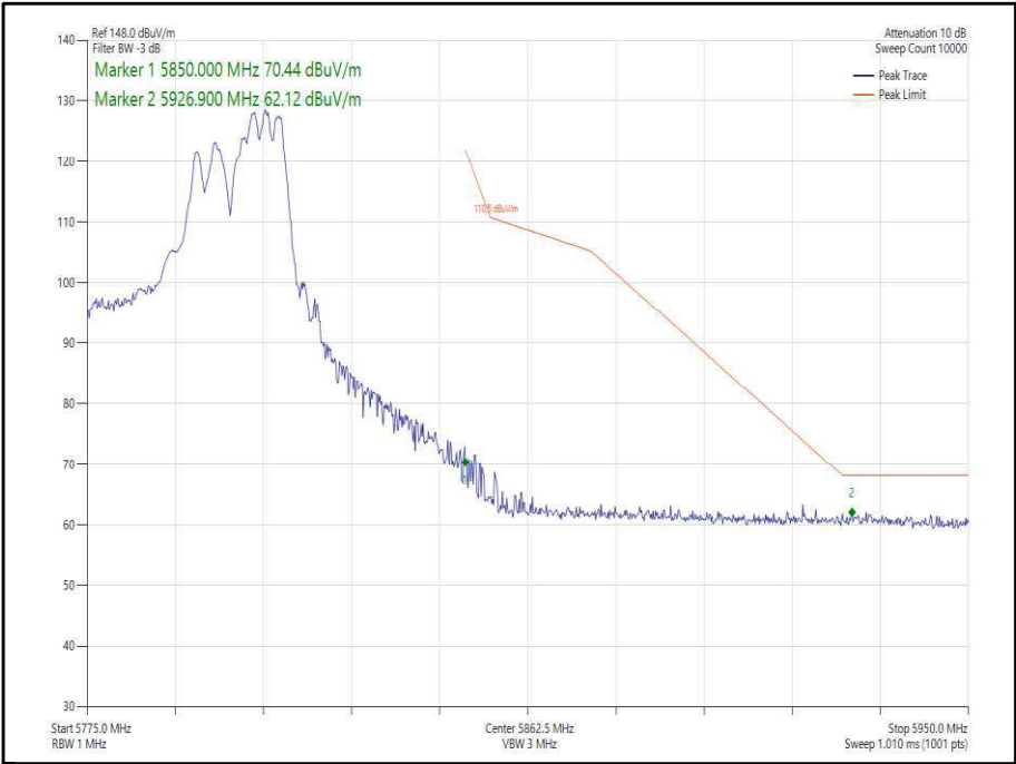
Figure 380 - 802.11ax, HE40, RU 106-56, SDM, Core 0-1 - 5795 MHz, Band Edge Frequency 5850 MHz
