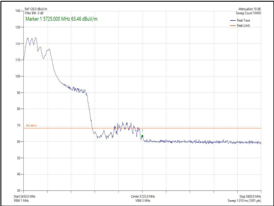
Figure 365 - 802.11ax, HE40, RU 106-53, CDD, Core 0-1 - 5670 MHz, Band Edge Frequency 5725 MHz
