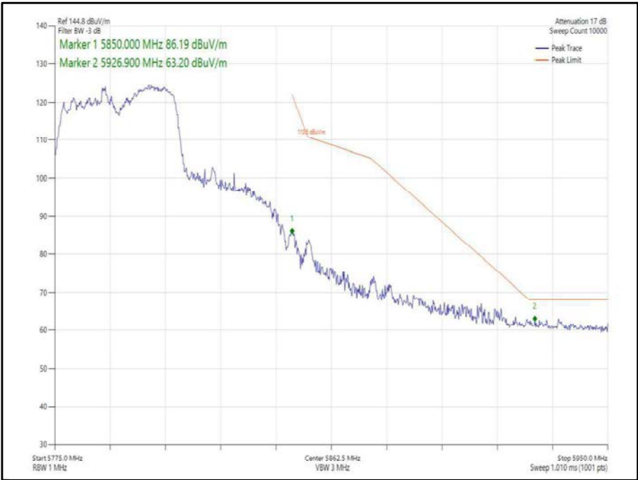
Figure 387 - 802.11n, HT40, TxBF, Core 0-1 - 5795 MHz, Band Edge Frequency 5850 MHz
