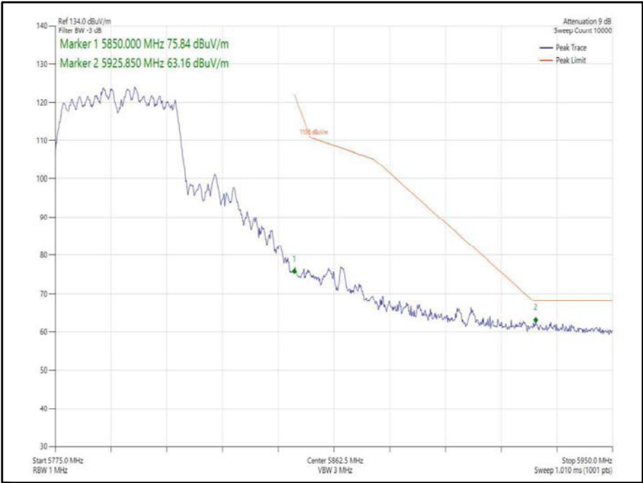
Figure 366 - 802.11n, HT40, CDD, Core 0-1 - 5795 MHz, Band Edge Frequency 5850 MHz
