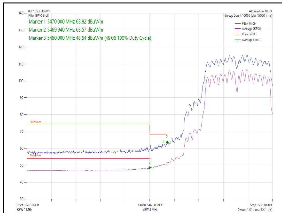
Figure 357 - 802.11n, HT40, CDD, Core 0-1 - 5510 MHz, Band Edge Frequency 5470 MHz
