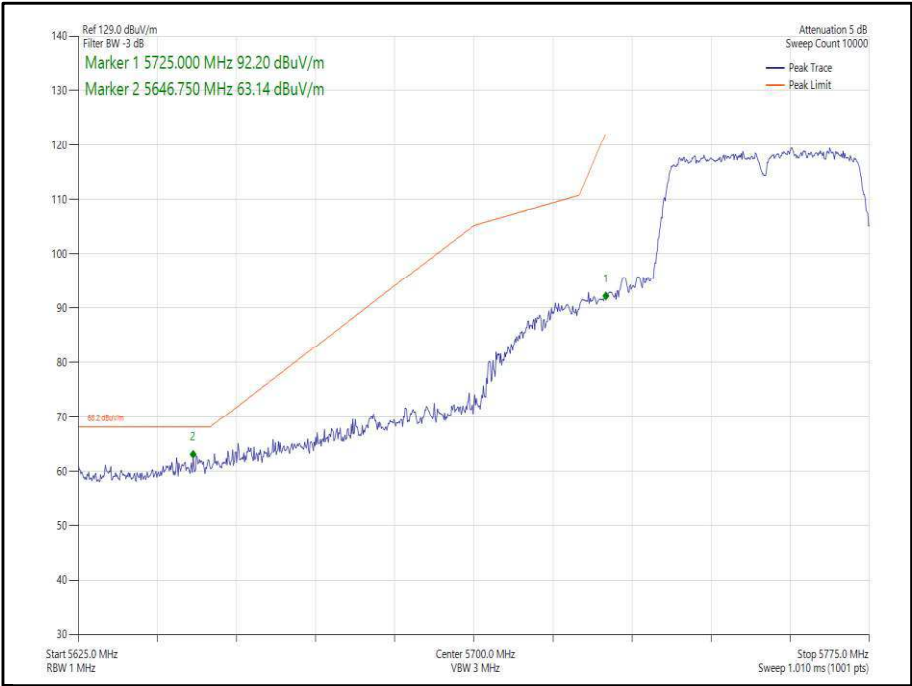
Figure 348 - 802.11n, HT40, SISO, Core 1 - 5755 MHz, Band Edge Frequency 5725 MHz
