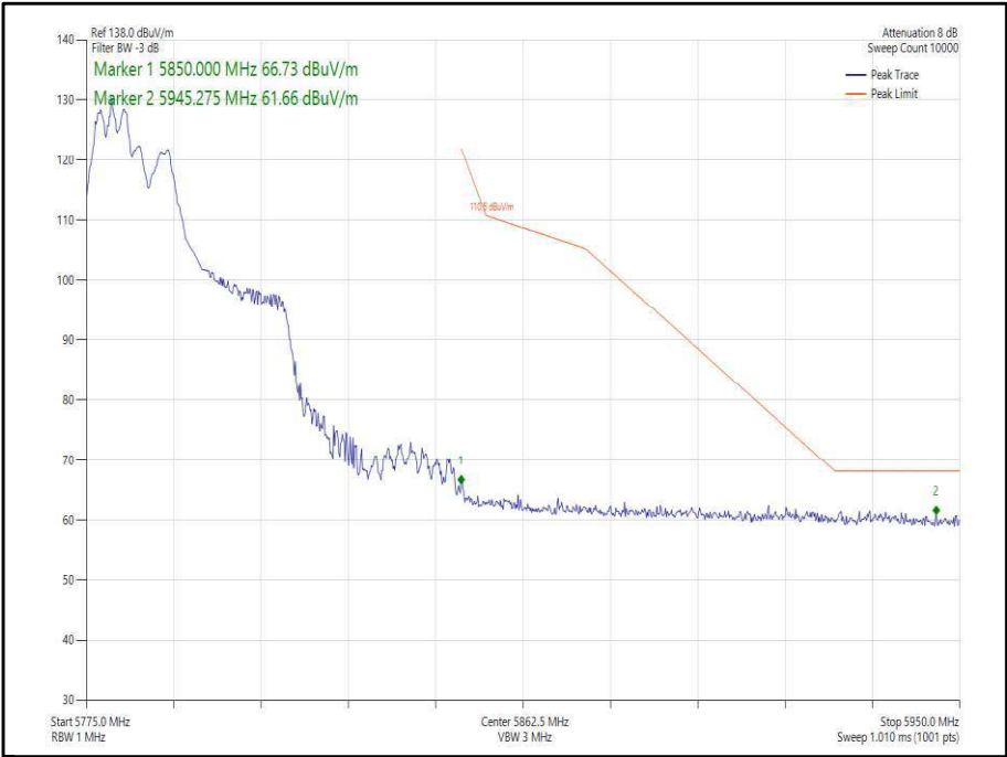
Figure 368 - 802.11ax, HE40, RU 106-53, CDD, Core 0-1 - 5795 MHz, Band Edge Frequency 5850 MHz
