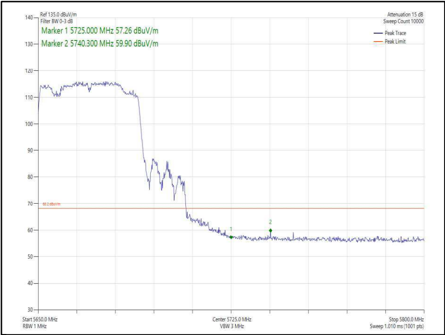
Figure 386 - 802.11ax, HE40, SU, TxBF, Core 0-1 - 5670 MHz, Band Edge Frequency 5725 MHz
