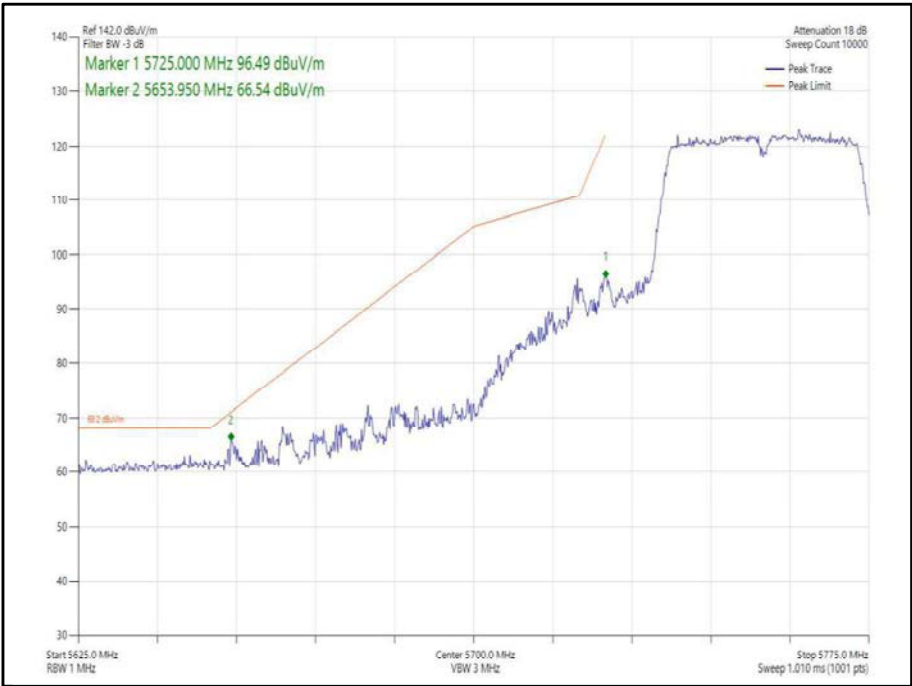
Figure 383 - 802.11ac, VHT40, TxBF, Core 0-1 - 5755 MHz, Band Edge Frequency 5725 MHz
