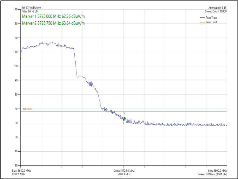
Figure 352 - 802.11ax, HE40, SU, SISO, Core 1 - 5670 MHz, Band Edge Frequency 5725 MHz
