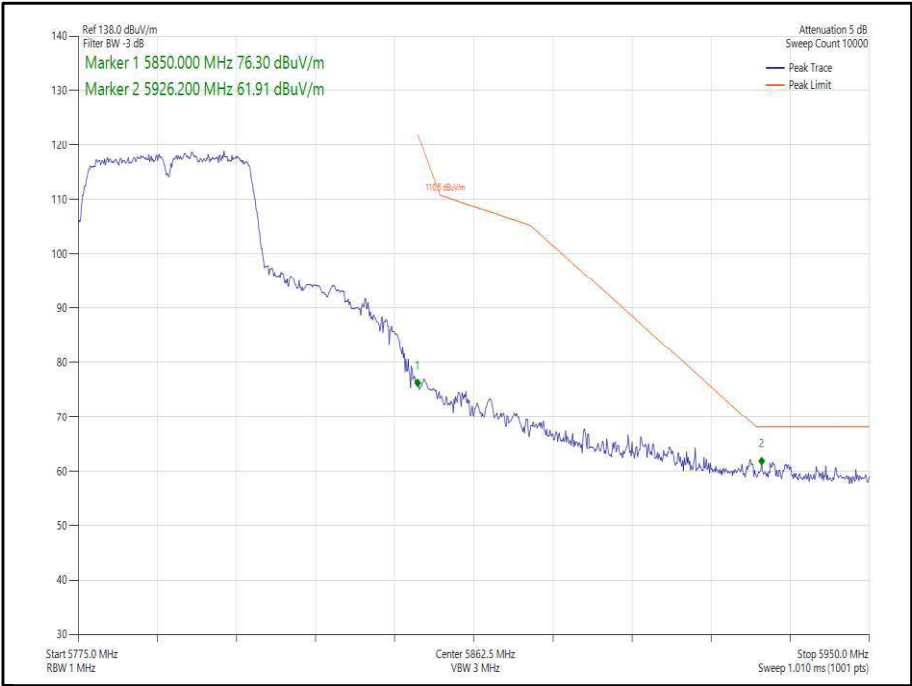
Figure 354 - 802.11n, HT40, SISO, Core 1 - 5795 MHz, Band Edge Frequency 5850 MHz
