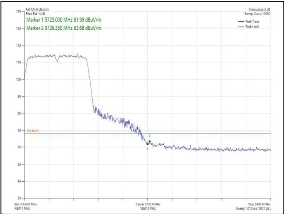
Figure 351 - 802.11n, HT40, SISO, Core 1 - 5670 MHz, Band Edge Frequency 5725 MHz
