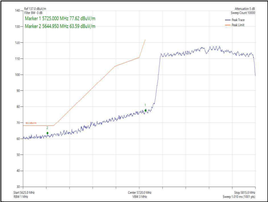
Figure 416 - 802.11ac, VHT80, CDD, Core 0-1 - 5775 MHz, Band Edge Frequency 5725 MHz
