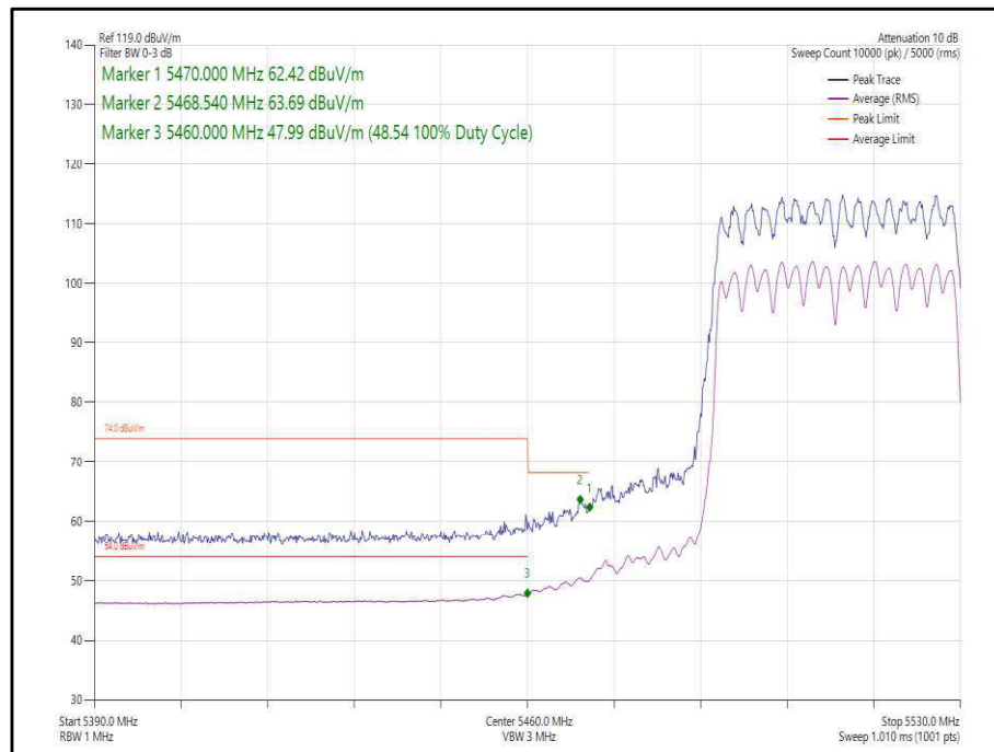
Figure 358 - 802.11ax, HE40, SU, CDD, Core 0-1 - 5510 MHz, Band Edge Frequency 5470 MHz
