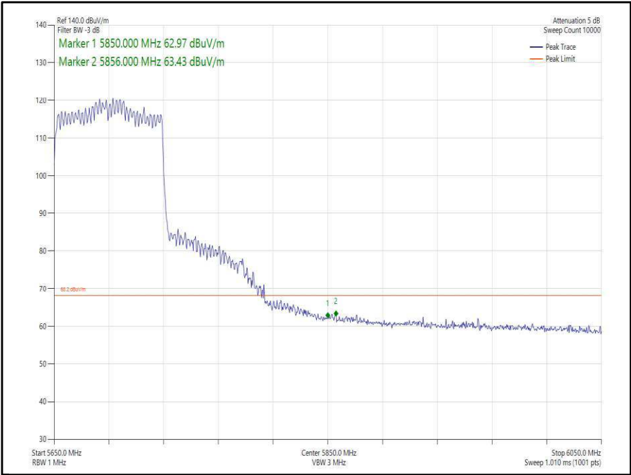
Figure 424 - 802.11ax, HE80, SU, CDD, Core 0-1 - 5690 MHz, Band Edge Frequency 5850 MHz
