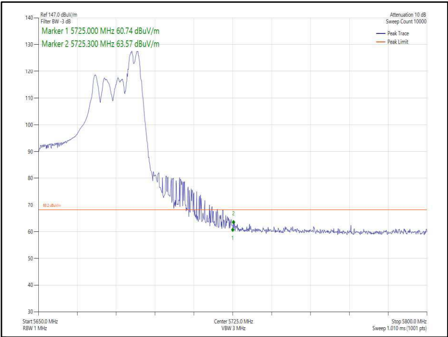
Figure 377 - 802.11ax, HE40, RU 52-44, SDM, Core 0-1 - 5670 MHz, Band Edge Frequency 5725 MHz
