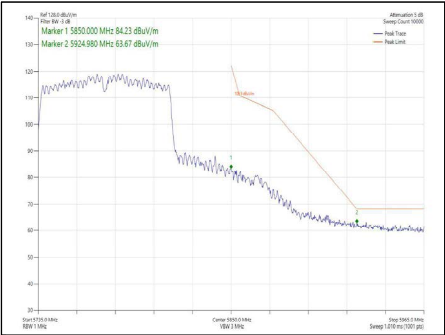
Figure 423 - 802.11ac, VHT80, CDD, Core 0-1 - 5775 MHz, Band Edge Frequency 5850 MHz
