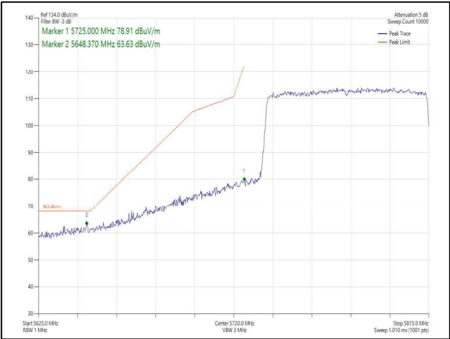
Figure 405 - 802.11ax, HE80, SU, SISO, Core 1 - 5775 MHz, Band Edge Frequency 5725 MHz
