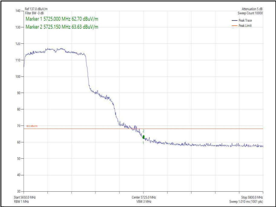
Figure 340 - 802.11ax, HE40, SU, SISO, Core 0 - 5670 MHz, Band Edge Frequency 5725 MHz
