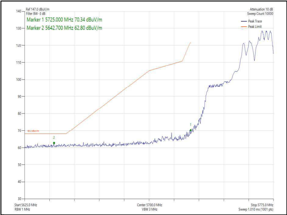
Figure 374 - 802.11ax, HE40, RU 106-56, SDM, Core 0-1 - 5755 MHz, Band Edge Frequency 5725 MHz
