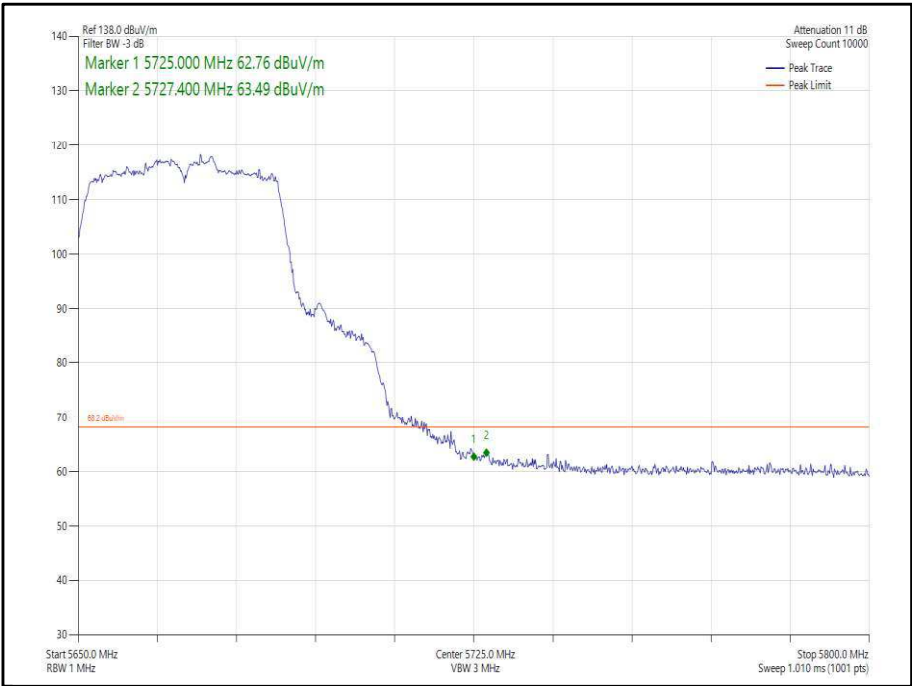
Figure 375 - 802.11n, HT40, SDM, Core 0-1 - 5670 MHz, Band Edge Frequency 5725 MHz
