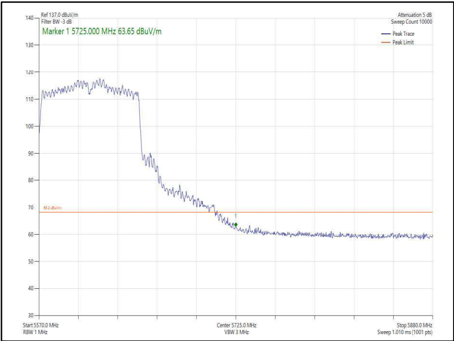
Figure 419 - 802.11ac, VHT80, CDD, Core 0-1 - 5610 MHz, Band Edge Frequency 5725 MHz
