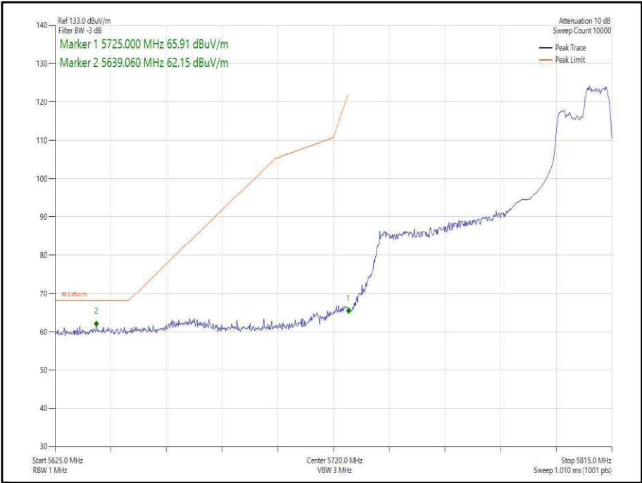
Figure 394 - 802.11ax, HE80, RU 106-60, SISO, Core 0 - 5775 MHz, Band Edge Frequency 5725 MHz
