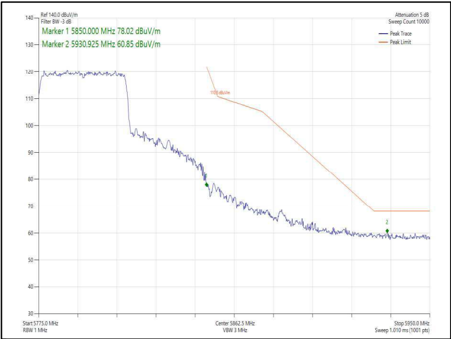
Figure 343 - 802.11ax, HE40, SU, SISO, Core 0 - 5795 MHz, Band Edge Frequency 5850 MHz
