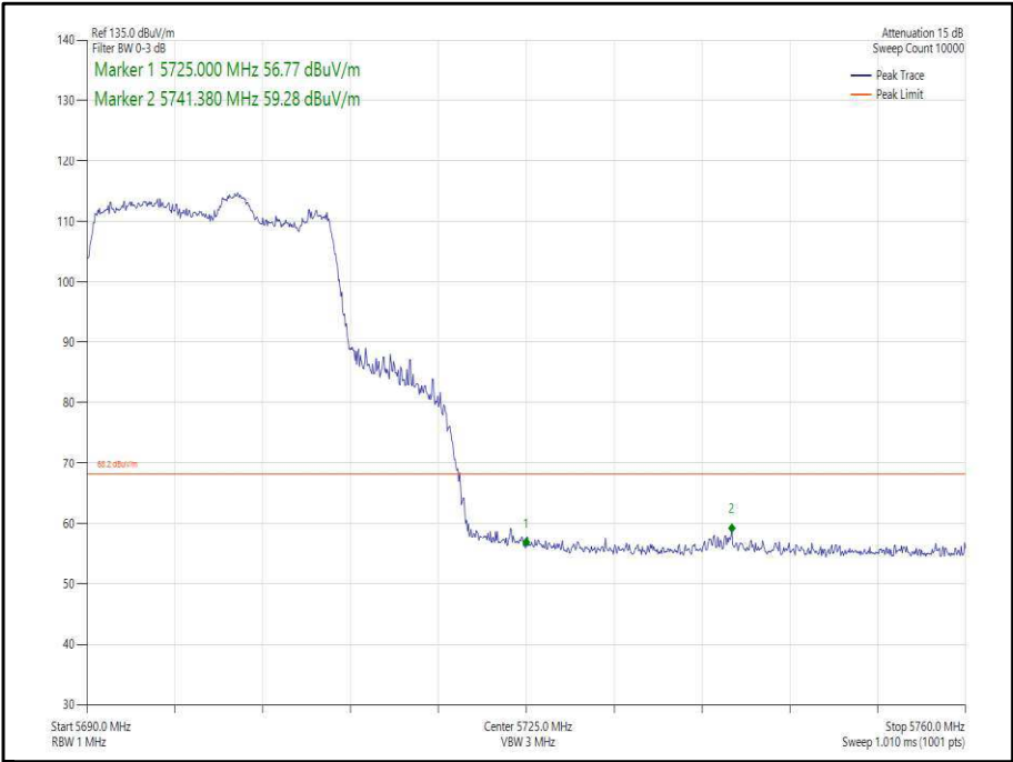
Figure 330 - 802.11ax, HE20, SU, TxBF, Core 0-1 - 5700 MHz, Band Edge Frequency 5725 MHz
