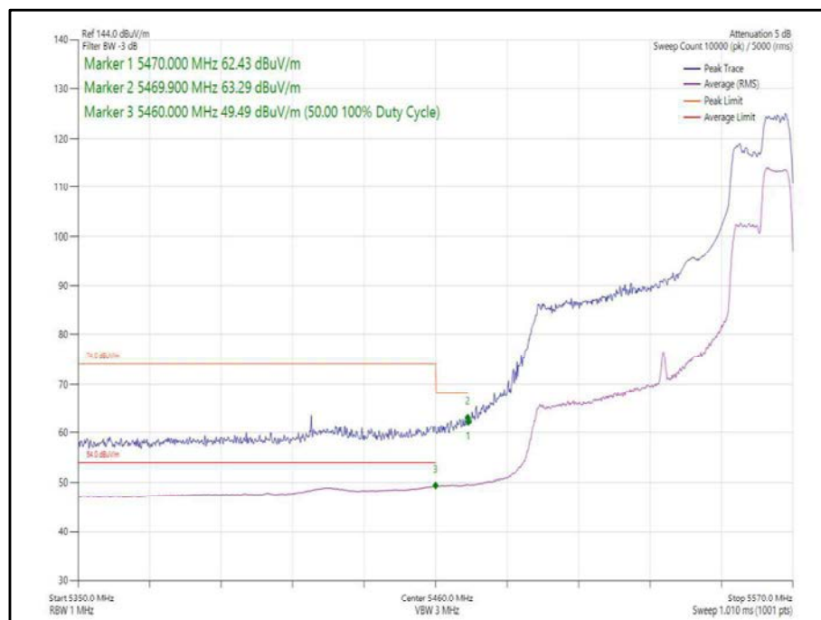
Figure 391 - 802.11ax, HE80, RU 106-60, SISO, Core 0 - 5530 MHz, Band Edge Frequency 5470 MHz
