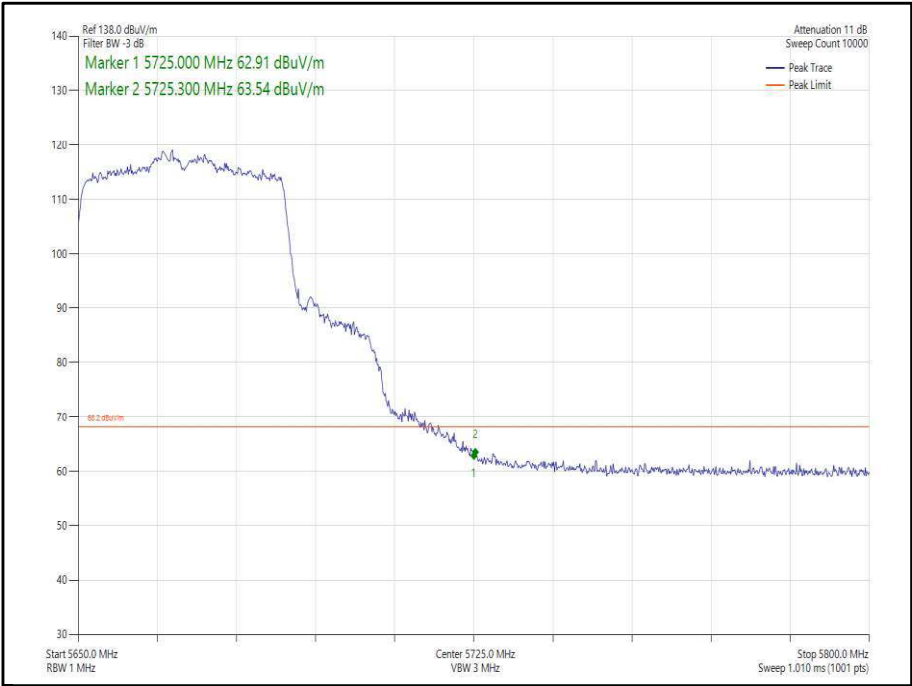
Figure 376 - 802.11ax, HE40, SU, SDM, Core 0-1 - 5670 MHz, Band Edge Frequency 5725 MHz
