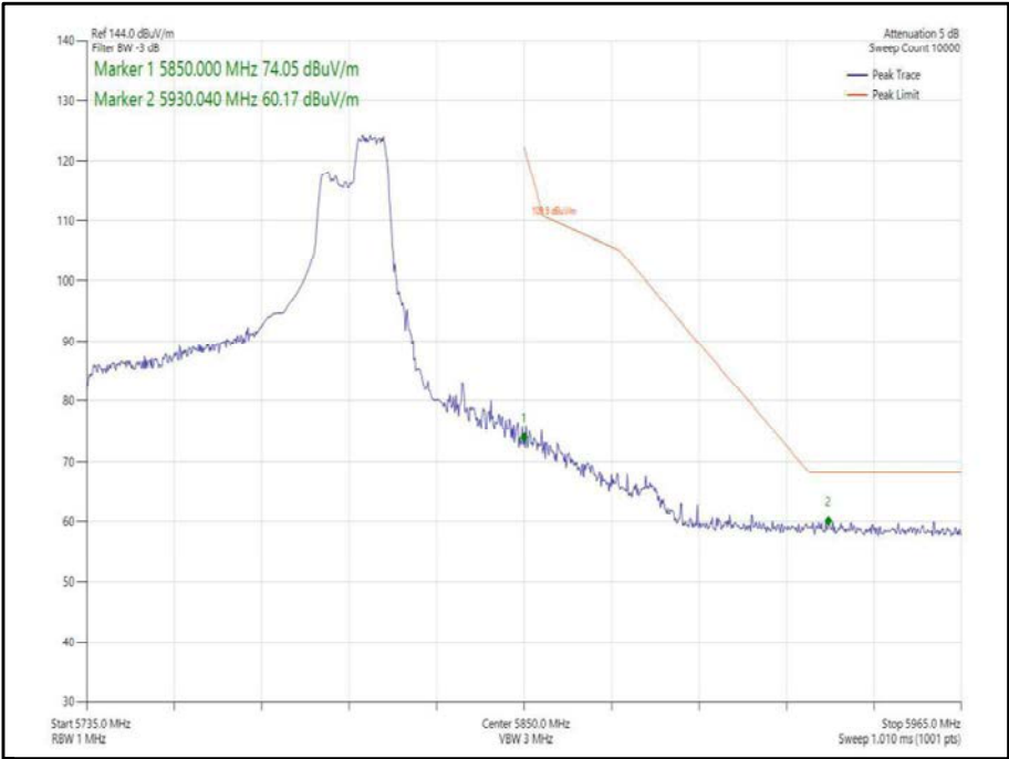
Figure 400 - 802.11ax, HE80, RU 106-60, SISO, Core 0 - 5775 MHz, Band Edge Frequency 5850 MHz
