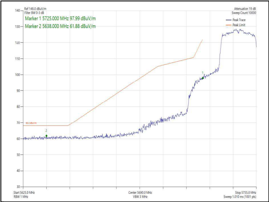
Figure 328 - 802.11ax, HE20, SU, TxBF, Core 0-1 - 5745 MHz, Band Edge Frequency 5725 MHz
