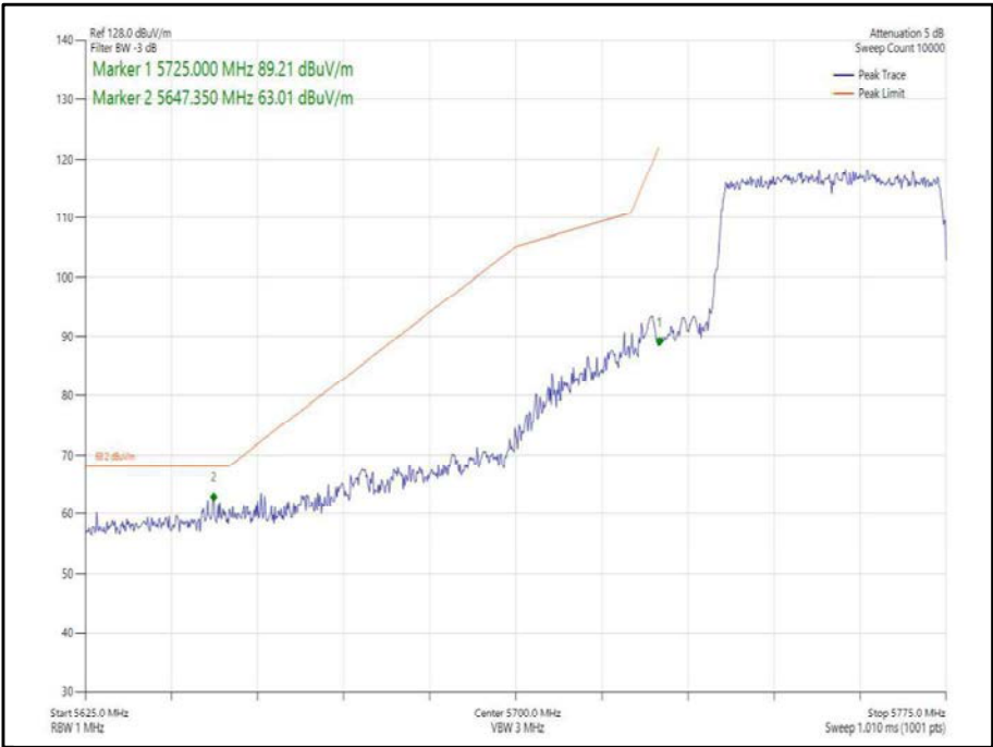
Figure 349 - 802.11ax, HE40, SU, SISO, Core 1 - 5755 MHz, Band Edge Frequency 5725 MHz
