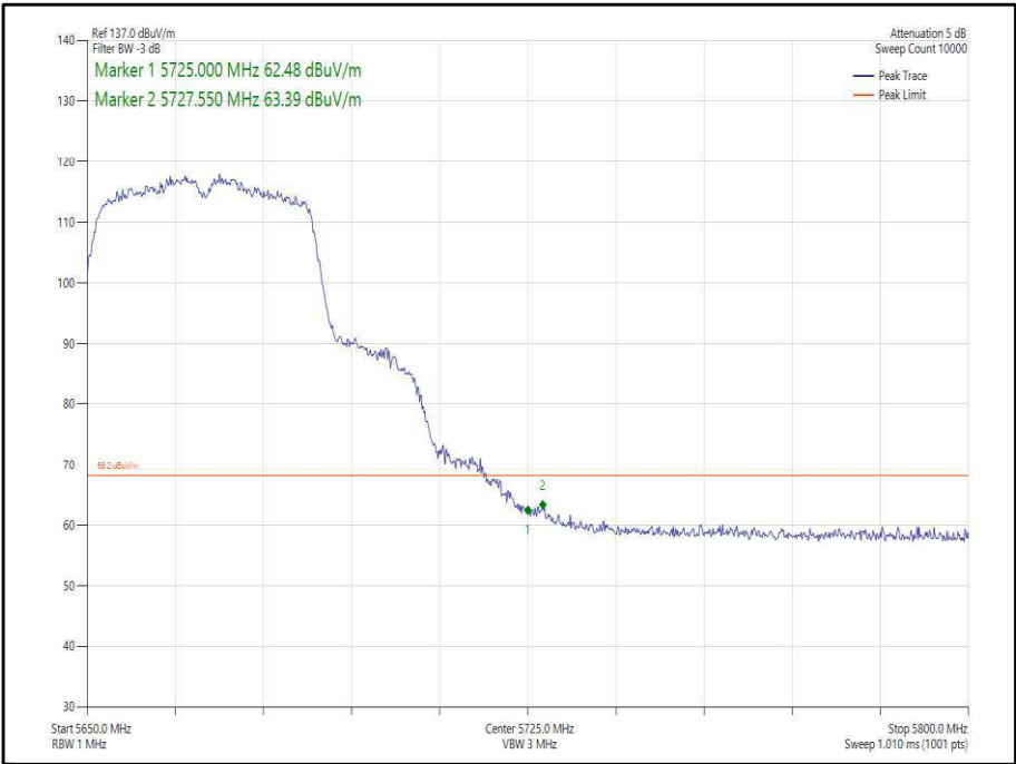
Figure 339 - 802.11n, HT40, SISO, Core 0 - 5670 MHz, Band Edge Frequency 5725 MHz
