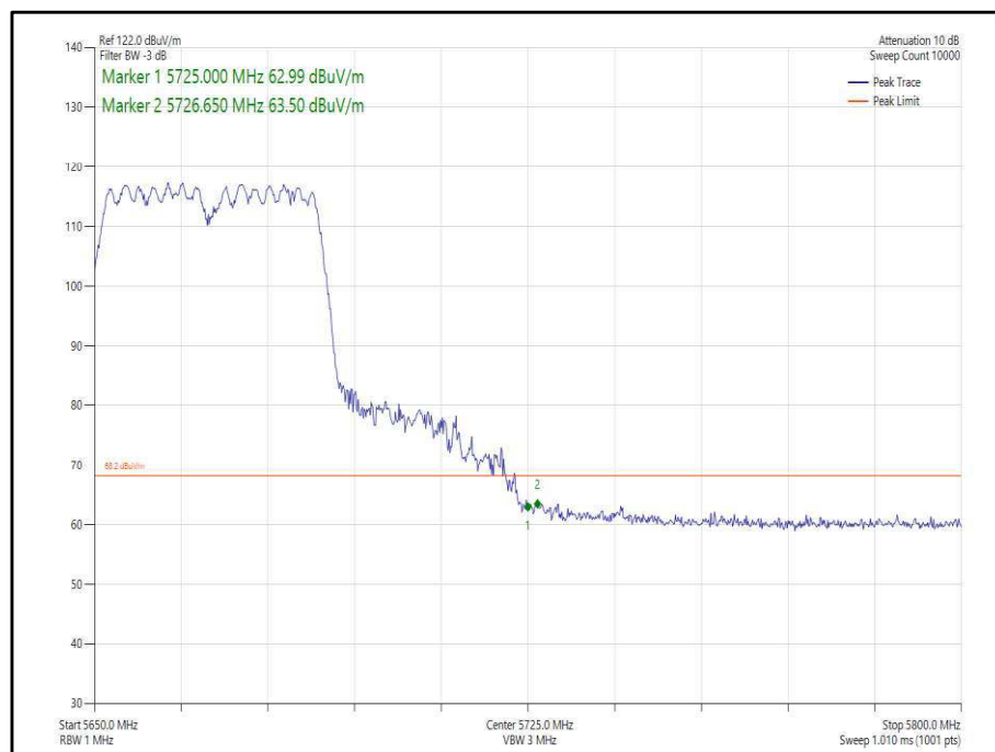
Figure 363 - 802.11n, HT40, CDD, Core 0-1 - 5670 MHz, Band Edge Frequency 5725 MHz
