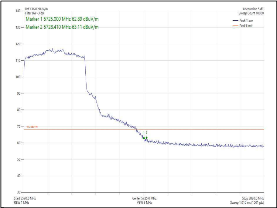
Figure 396 - 802.11ax, HE80, SU, SISO, Core 0 - 5610 MHz, Band Edge Frequency 5725 MHz
