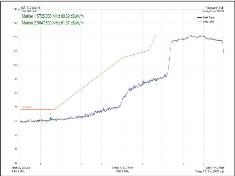
Figure 336 - 802.11n, HT40, SISO, Core 0 - 5755 MHz, Band Edge Frequency 5725 MHz
