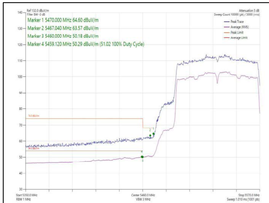
Figure 389 - 802.11ac, VHT80, SISO, Core 0 - 5530 MHz, Band Edge Frequency 5470 MHz
