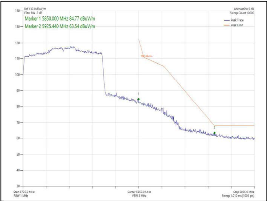
Figure 411 - 802.11ax, HE80, SU, SISO, Core 1 - 5775 MHz, Band Edge Frequency 5850 MHz
