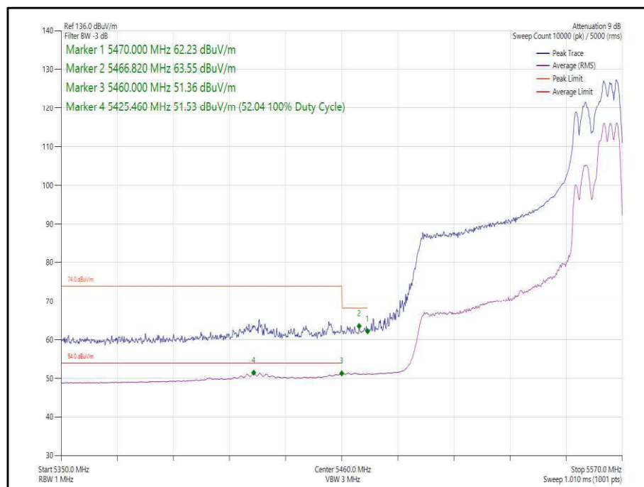
Figure 415 - 802.11ax, HE80, RU 106-60, CDD, Core 0-1 - 5530 MHz, Band Edge Frequency 5470 MHz
