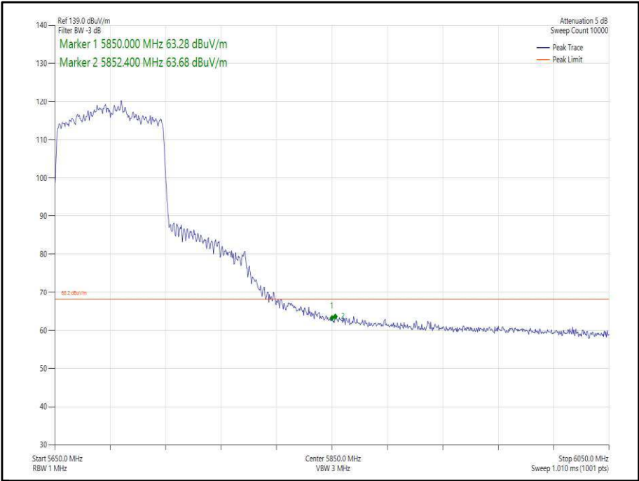
Figure 422 - 802.11ac, VHT80, CDD, Core 0-1 - 5690 MHz, Band Edge Frequency 5850 MHz
