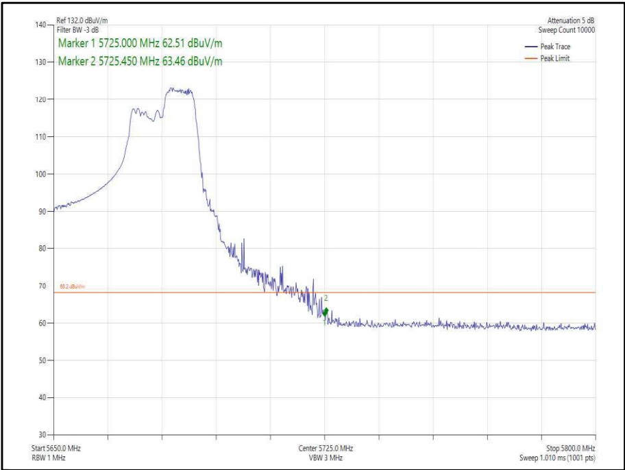
Figure 353 - 802.11ax, HE40, RU 106-56, SISO, Core 1 - 5670 MHz, Band Edge Frequency 5725 MHz
