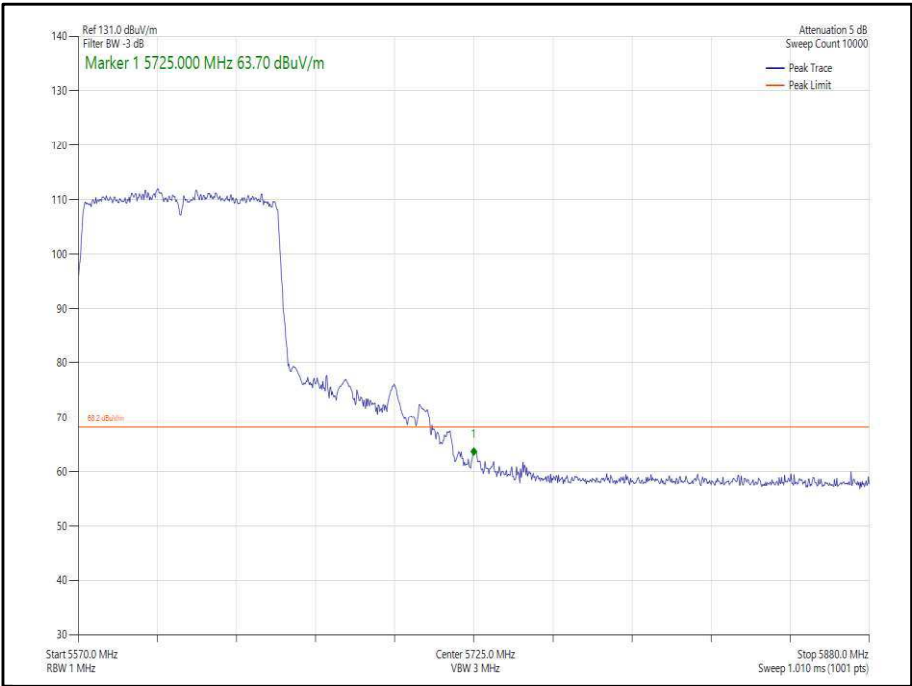
Figure 407 - 802.11ac, VHT80, SISO, Core 1 - 5610 MHz, Band Edge Frequency 5725 MHz
