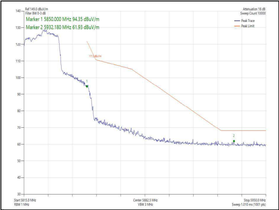
Figure 332 - 802.11ax, HE20, SU, TxBF, Core 0-1 - 5825 MHz, Band Edge Frequency 5850 MHz
