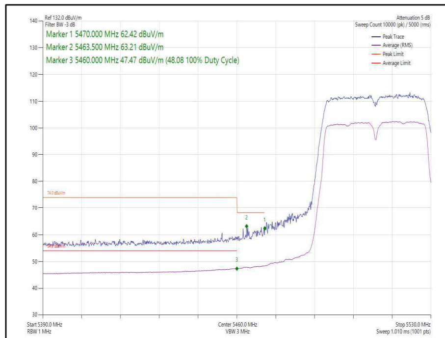
Figure 333 - 802.11n, HT40, SISO, Core 0 - 5510 MHz, Band Edge Frequency 5470 MHz
