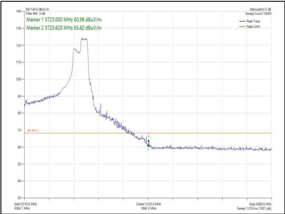
Figure 409 - 802.11ax, HE80, RU 106-60, SISO, Core 1 - 5610 MHz, Band Edge Frequency 5725 MHz
