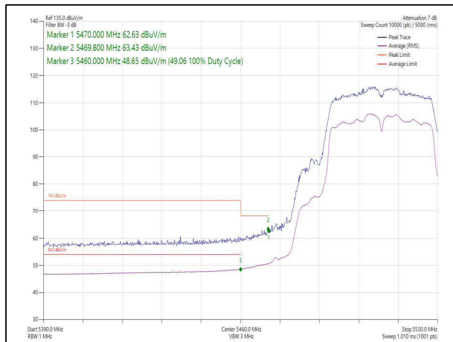
Figure 369 - 802.11n, HT40, SDM, Core 0-1 - 5510 MHz, Band Edge Frequency 5470 MHz
