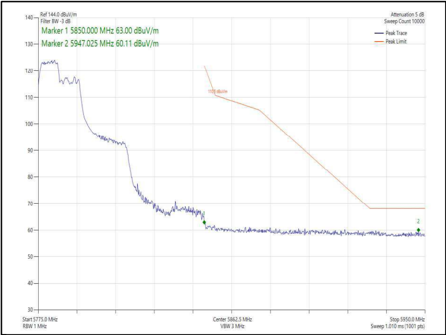
Figure 356 - 802.11ax, HE40, RU 106-53, SISO, Core 1 - 5795 MHz, Band Edge Frequency 5850 MHz
