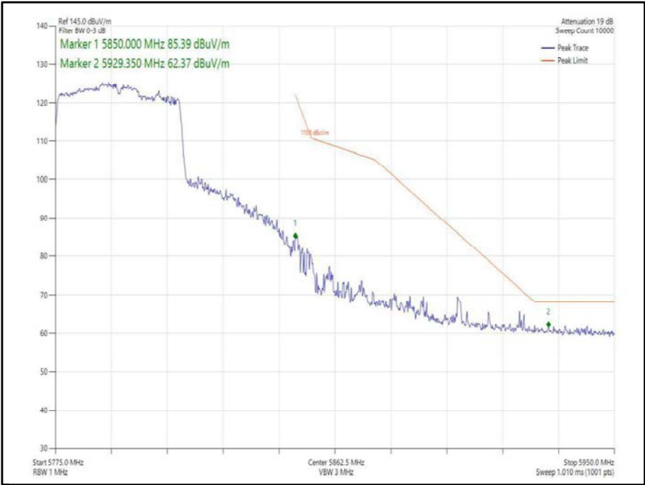
Figure 388 - 802.11ax, HE40, SU, TxBF, Core 0-1 - 5795 MHz, Band Edge Frequency 5850 MHz
