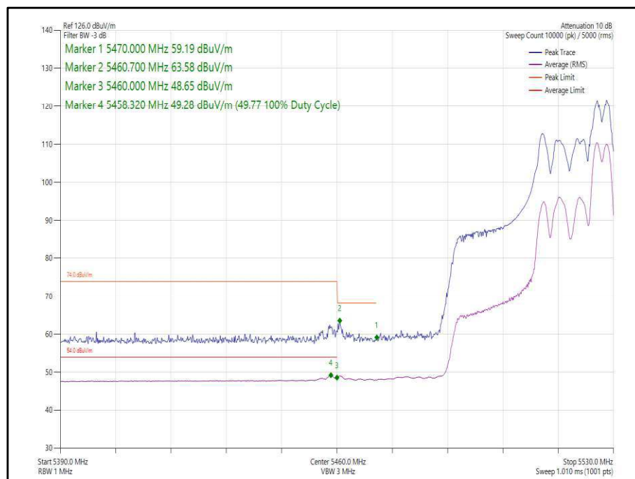
Figure 359 - 802.11ax, HE40, RU 52-44, CDD, Core 0-1 - 5510 MHz, Band Edge Frequency 5470 MHz
