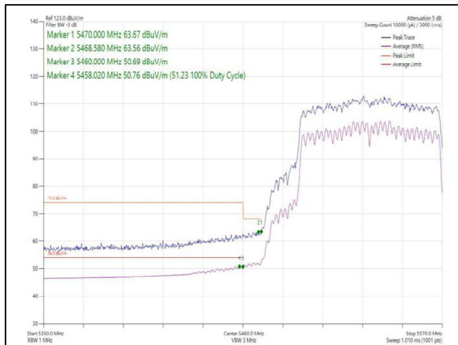
Figure 413 - 802.11ac, VHT80, CDD, Core 0-1 - 5530 MHz, Band Edge Frequency 5470 MHz
