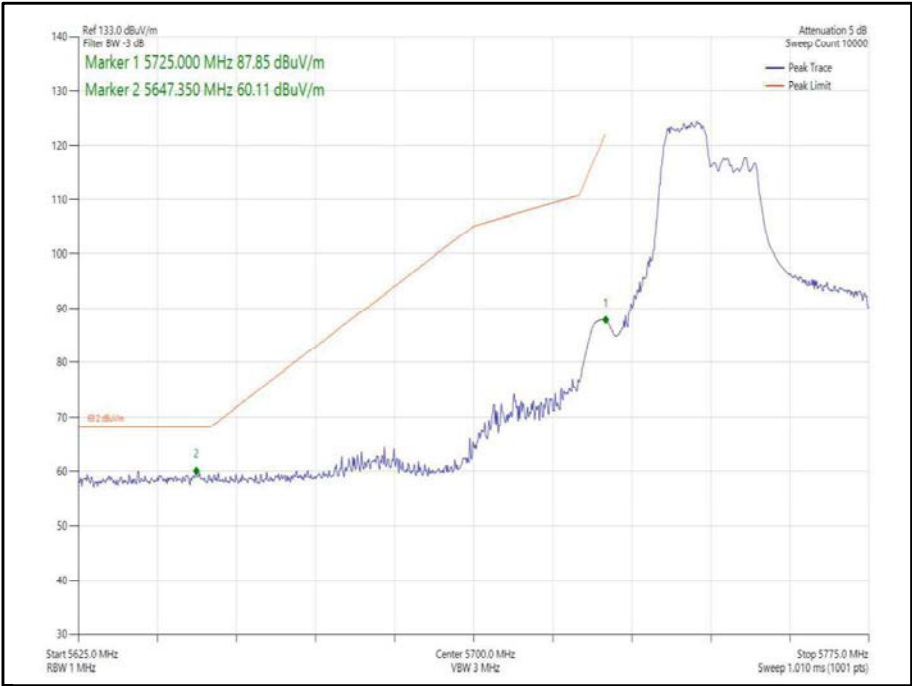
Figure 350 - 802.11ax, HE40, RU 106-53, SISO, Core 1 - 5755 MHz, Band Edge Frequency 5725 MHz
