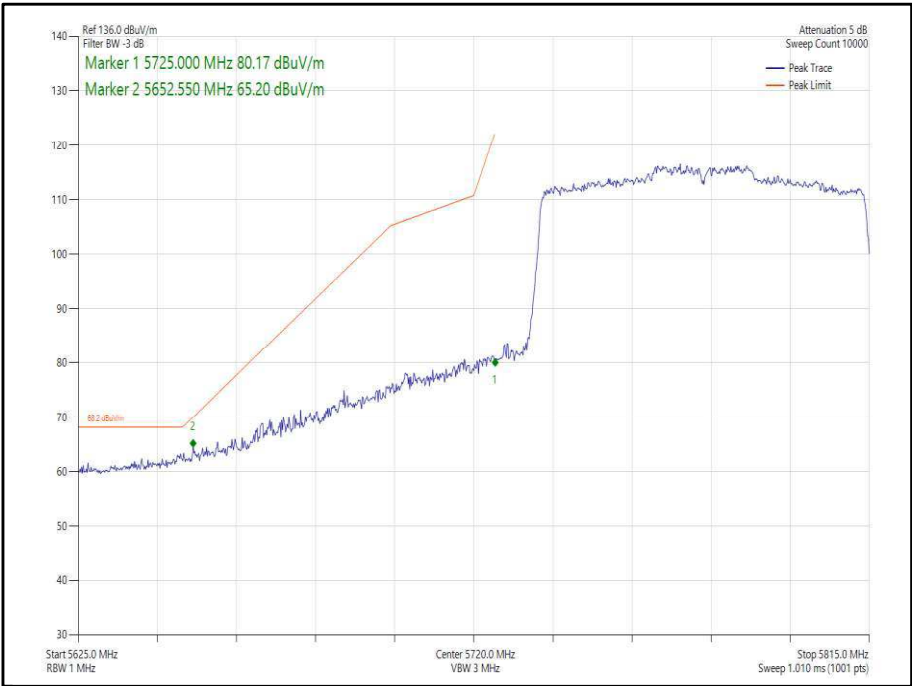
Figure 393 - 802.11ax, HE80, SU, SISO, Core 0 - 5775 MHz, Band Edge Frequency 5725 MHz
