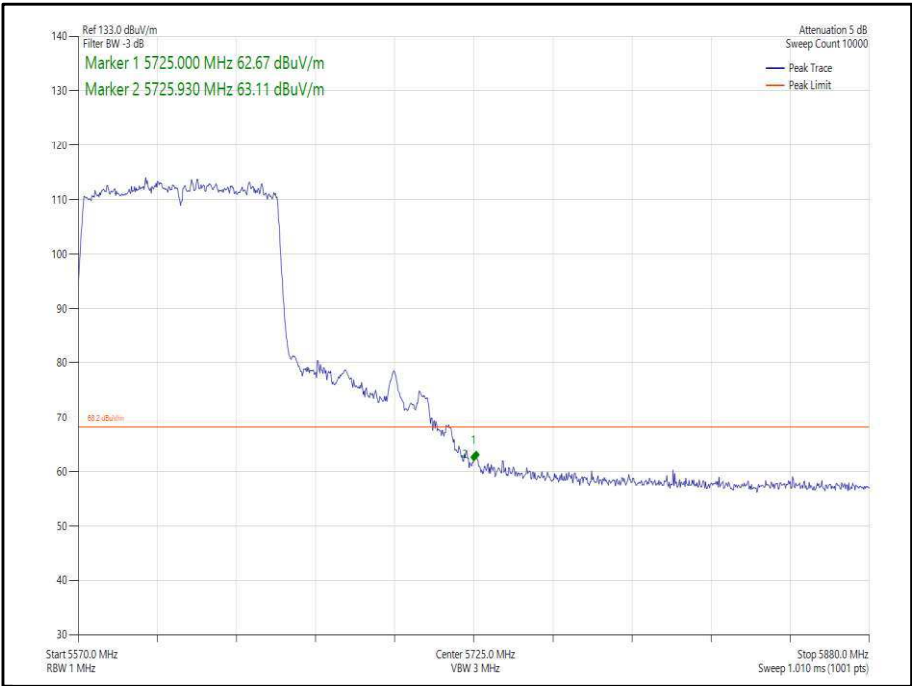
Figure 395 - 802.11ac, VHT80, SISO, Core 0 - 5610 MHz, Band Edge Frequency 5725 MHz
