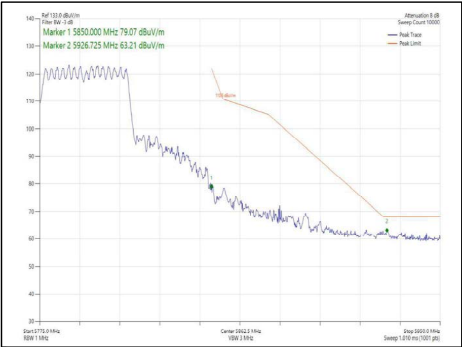
Figure 367 - 802.11ax, HE40, SU, CDD, Core 0-1 - 5795 MHz, Band Edge Frequency 5850 MHz
