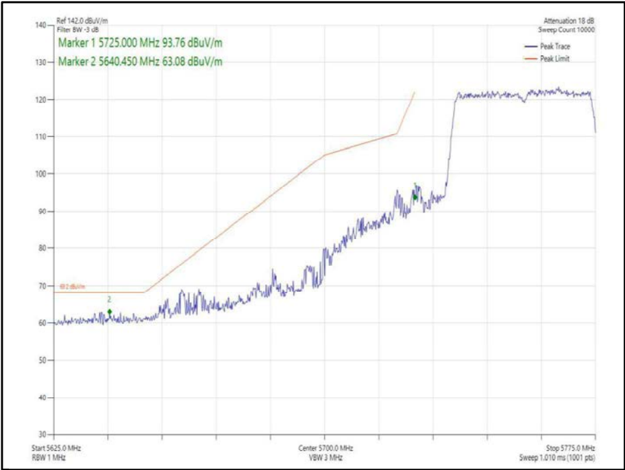
Figure 384 - 802.11ax, HE40, SU, TxBF, Core 0-1 - 5755 MHz, Band Edge Frequency 5725 MHz
