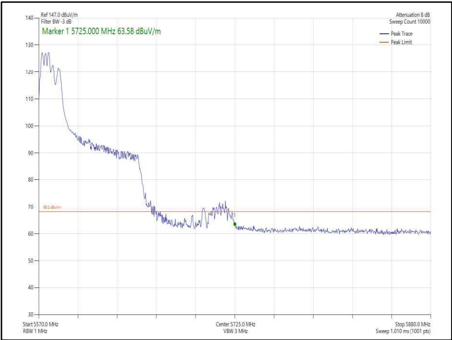
Figure 421 - 802.11ax, HE80, RU 106-53, CDD, Core 0-1 - 5610 MHz, Band Edge Frequency 5725 MHz
