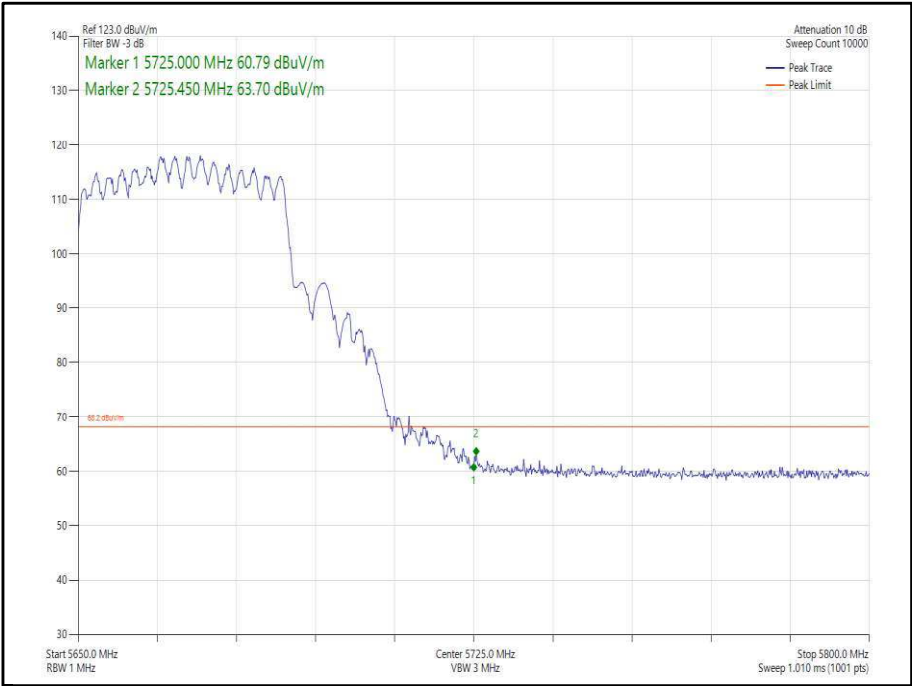
Figure 364 - 802.11ax, HE40, SU, CDD, Core 0-1 - 5670 MHz, Band Edge Frequency 5725 MHz
