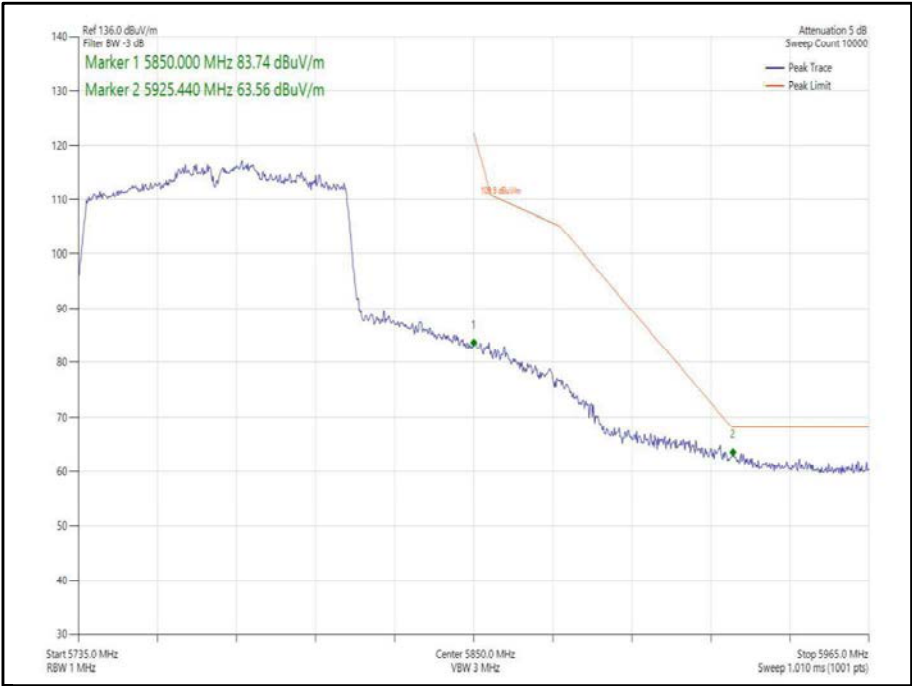
Figure 410 - 802.11ac, VHT80, SISO, Core 1 - 5775 MHz, Band Edge Frequency 5850 MHz
