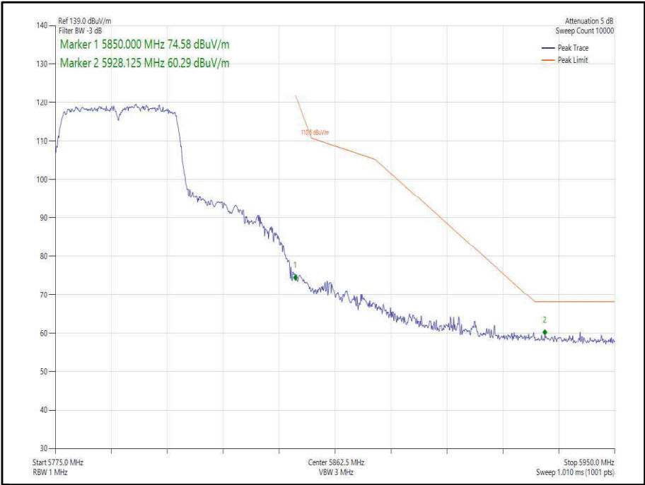
Figure 342 - 802.11n, HT40, SISO, Core 0 - 5795 MHz, Band Edge Frequency 5850 MHz
