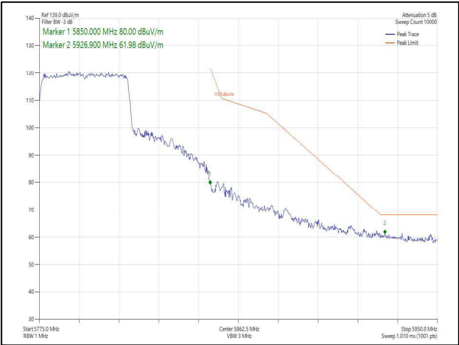
Figure 355 - 802.11ax, HE40, SU, SISO, Core 1 - 5795 MHz, Band Edge Frequency 5850 MHz
