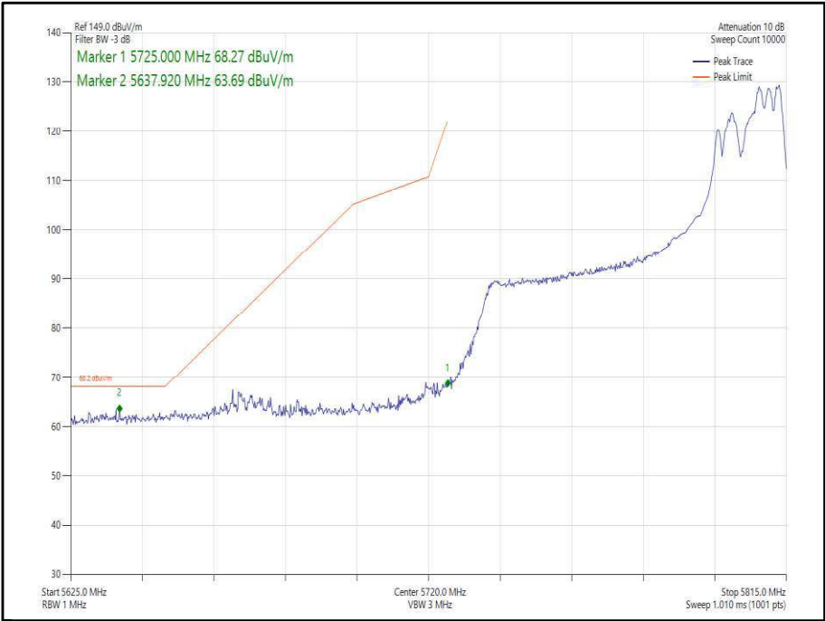
Figure 418 - 802.11ax, HE80, RU 106-60, CDD, Core 0-1 - 5775 MHz, Band Edge Frequency 5725 MHz
