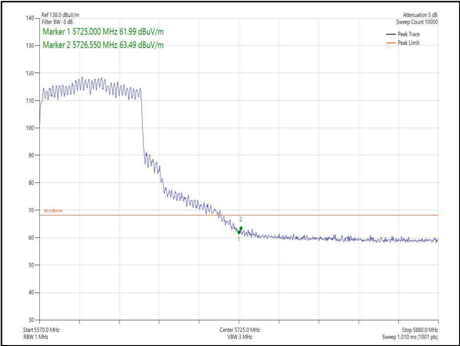
Figure 420 - 802.11ax, HE80, SU, CDD, Core 0-1 - 5610 MHz, Band Edge Frequency 5725 MHz
