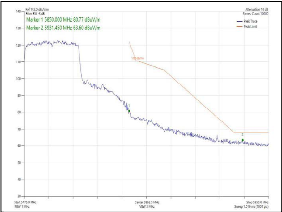
Figure 379 - 802.11ax, HE40, SU, SDM, Core 0-1 - 5795 MHz, Band Edge Frequency 5850 MHz
