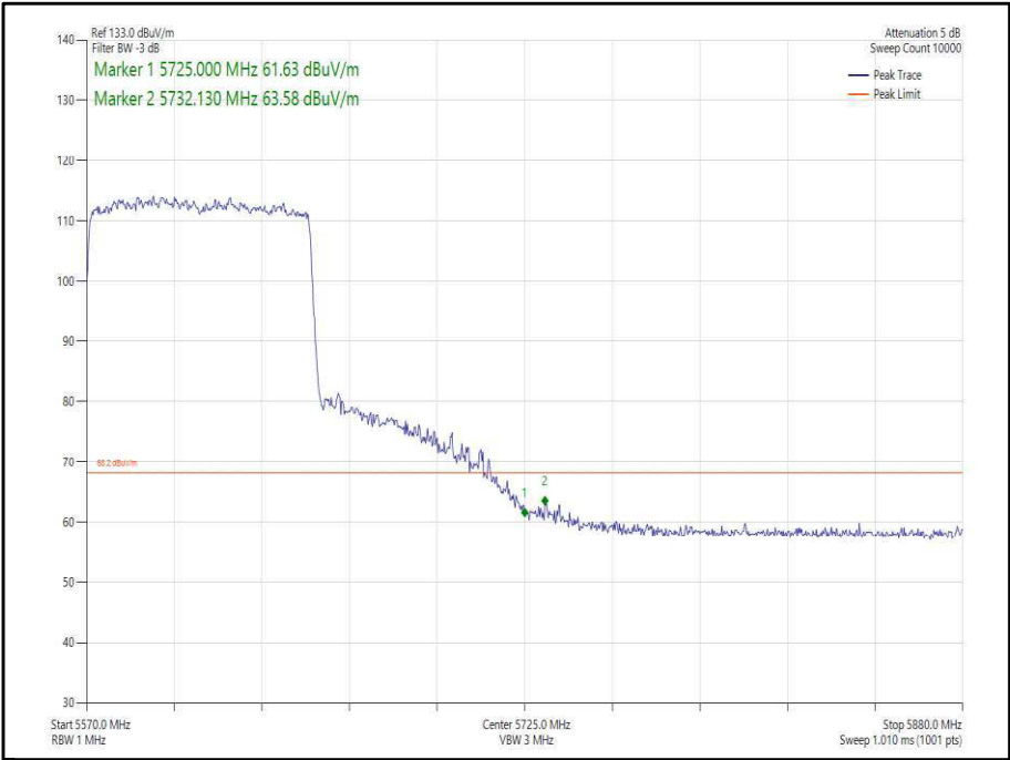
Figure 408 - 802.11ax, HE80, SU, SISO, Core 1 - 5610 MHz, Band Edge Frequency 5725 MHz
