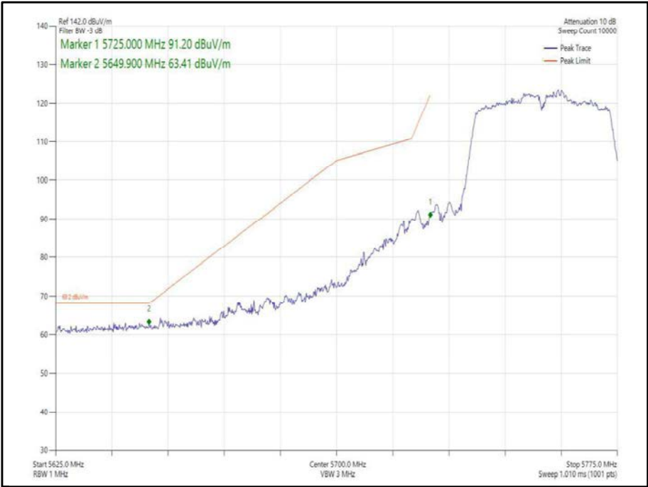
Figure 372 - 802.11n, HT40, SDM, Core 0-1 - 5755 MHz, Band Edge Frequency 5725 MHz
