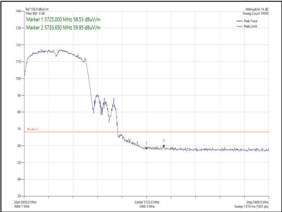
Figure 385 - 802.11n, HT40, TxBF, Core 0-1 - 5670 MHz, Band Edge Frequency 5725 MHz
