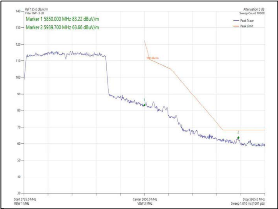
Figure 398 - 802.11ac, VHT80, SISO, Core 0 - 5775 MHz, Band Edge Frequency 5850 MHz
