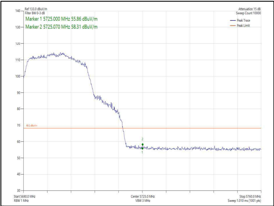
Figure 329 - 802.11ac, VHT20 TxBF, Core 0-1 - 5700 MHz, Band Edge Frequency 5725 MHz
