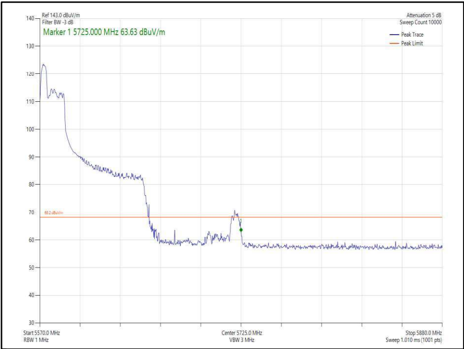
Figure 397 - 802.11ax, HE80, RU 52-37, SISO, Core 0 - 5610 MHz, Band Edge Frequency 5725 MHz
