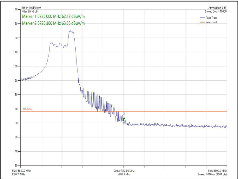
Figure 341 - 802.11ax, HE40, RU 52-44, SISO, Core 0 - 5670 MHz, Band Edge Frequency 5725 MHz
