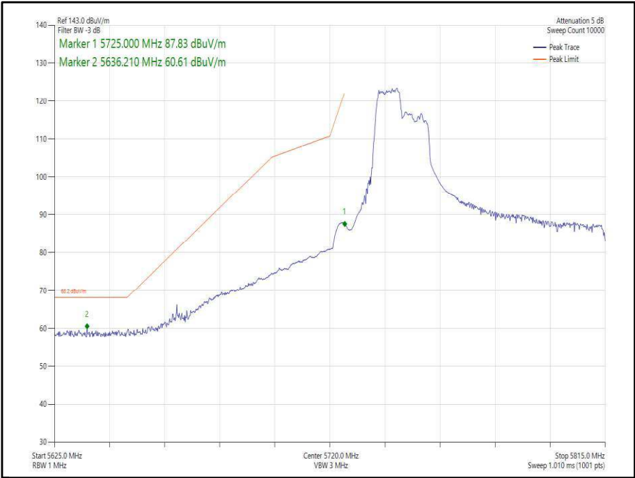
Figure 406 - 802.11ax, HE80, RU 106-53, SISO, Core 1 - 5775 MHz, Band Edge Frequency 5725 MHz
