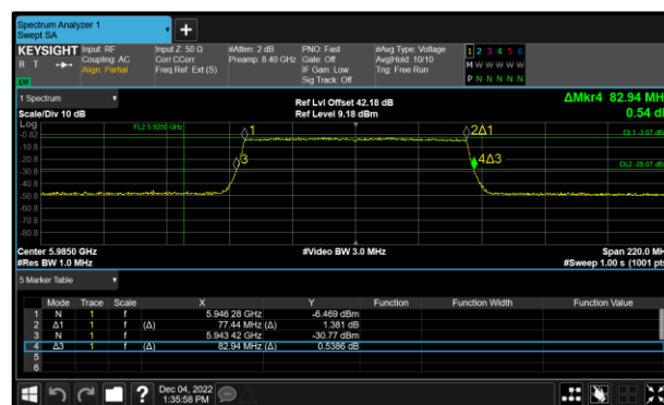
Figure 30 - 802.11ax HE80 SU Maximum 99% OBW
