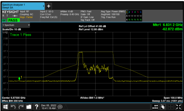
Figure 96 - B (Core 1) 802.11ax HE20 RU26 6875 MHz (CH185)
