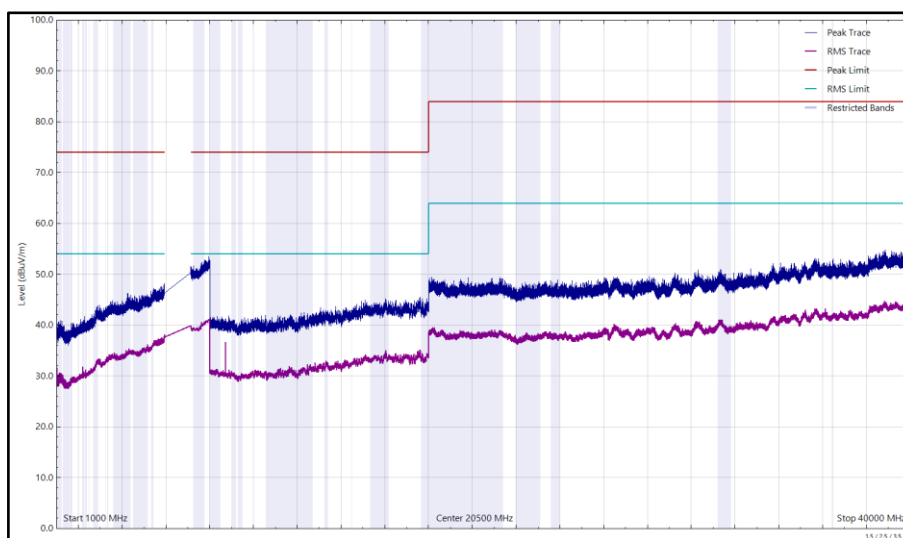
Figure 117 - U-NII-7 - 6535 MHz (CH117-6E), HE20, SU, CDD, Core 0 + Core 1, 1 GHz to 40 GHz, Horizontal
