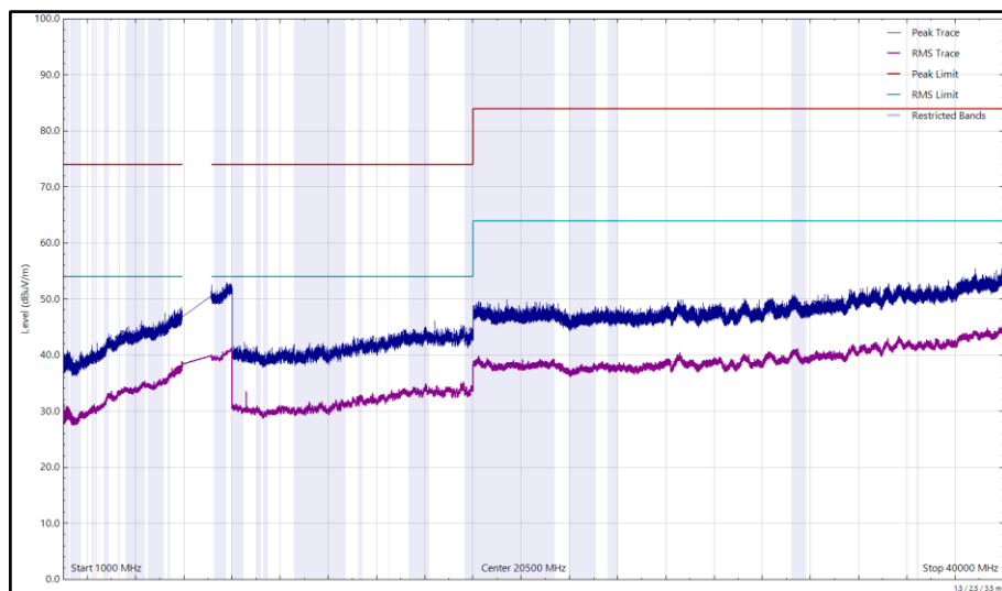
Figure 110 - U-NII-6 - 6435 MHz (CH97-6E), HE20, SU, CDD, Core 0 + Core 1, 1 GHz to 40 GHz, Vertical
