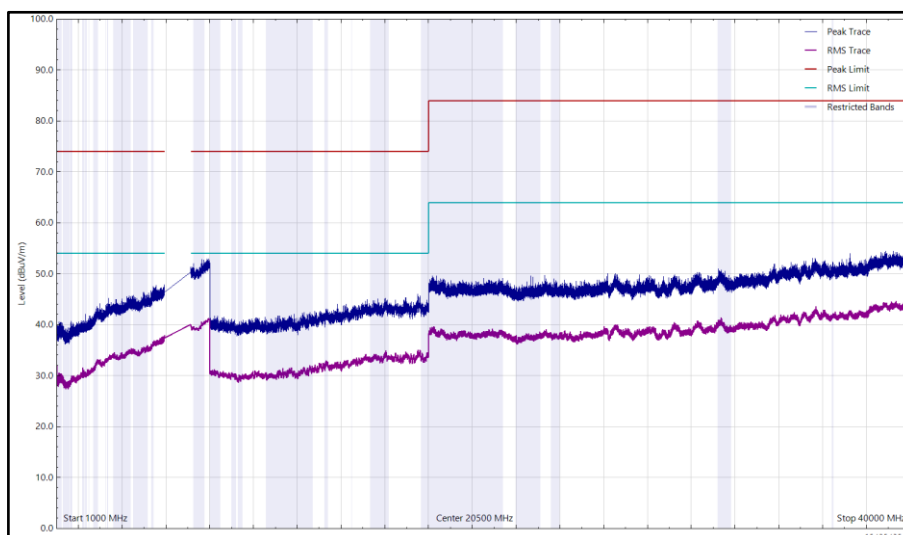
Figure 120 - U-NII-7 - 6695 MHz (CH149-6E), HE20, SU, CDD, Core 0 + Core 1, 1 GHz to 40 GHz, Horizontal
