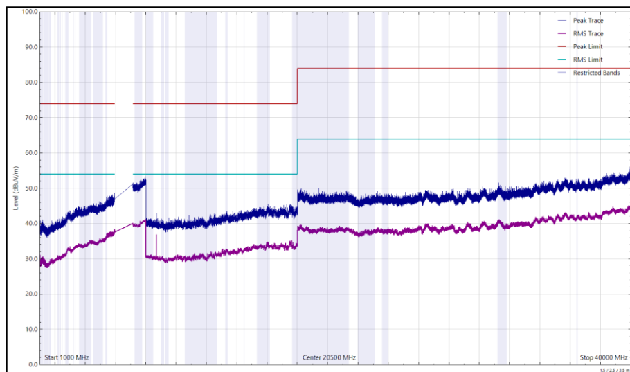
Figure 116 - U-NII-6 - 6515 MHz (CH113-6E), HE20, SU, CDD, Core 0 + Core 1, 1 GHz to 40 GHz, Vertical
