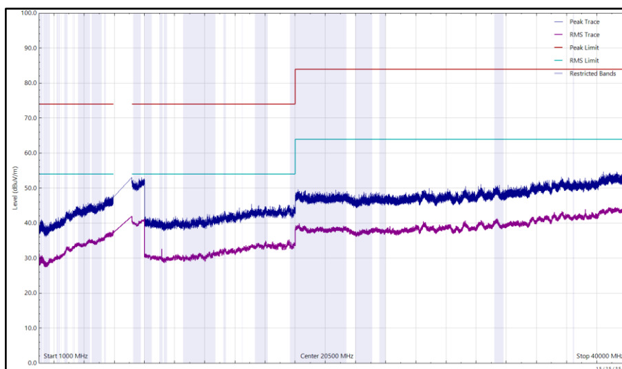
Figure 124 - U-NII-7 - 6855 MHz (CH181-6E), HE20, SU, CDD, Core 0 + Core 1, 1 GHz to 40 GHz, Vertical
