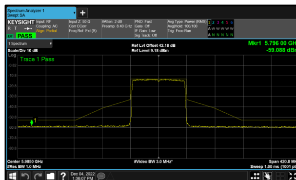
Figure 99 - A (Core 0) 802.11ax HE80 SU 5985 MHz (CH7)
