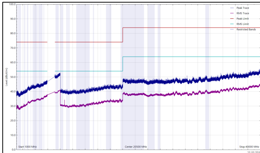
Figure 115 - U-NII-6 - 6515 MHz (CH113-6E), HE20, SU, CDD, Core 0 + Core 1, 1 GHz to 40 GHz, Horizontal
