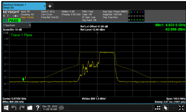
Figure 95 - B (Core 1) 802.11ax HE20 RU106 6875 MHz (CH185)
