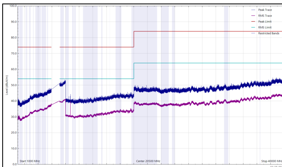
Figure 118 - U-NII-7 - 6535 MHz (CH117-6E), HE20, SU, CDD, Core 0 + Core 1, 1 GHz to 40 GHz, Vertical
