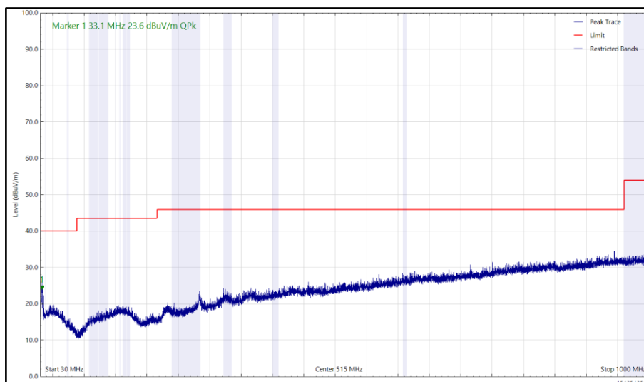
Figure 119 - U-NII-7 - 6695 MHz (CH149-6E), HE20, SU, CDD, Core 0 + Core 1, 30 MHz to 1 GHz, Horizontal (Peak)
