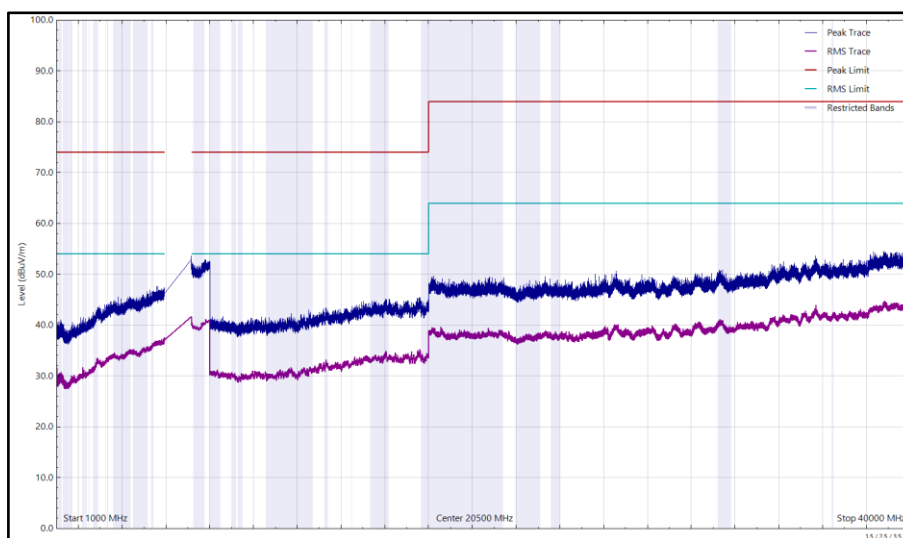
Figure 123 - U-NII-7 - 6855 MHz (CH181-6E), HE20, SU, CDD, Core 0 + Core 1, 1 GHz to 40 GHz, Horizontal
