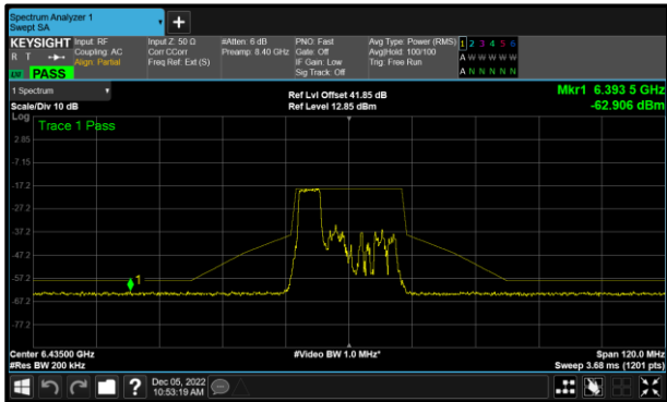
Figure 97 - A (Core 0) 802.11ax HE20 RU52 6435 MHz (CH97)
