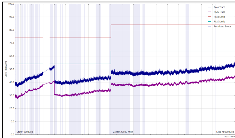
Figure 109 - U-NII-6 - 6435 MHz (CH97-6E), HE20, SU, CDD, Core 0 + Core 1, 1 GHz to 40 GHz, Horizontal
