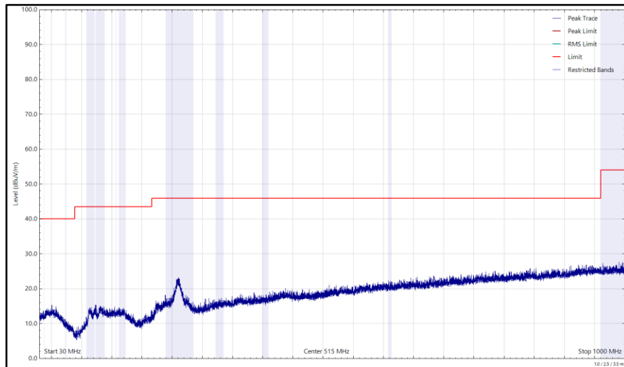
Figure 98 - 2437 MHz (CH6), HE20, RU26-0, Core 0 + Core 1, 30 MHz to 1 GHz, Horizontal
