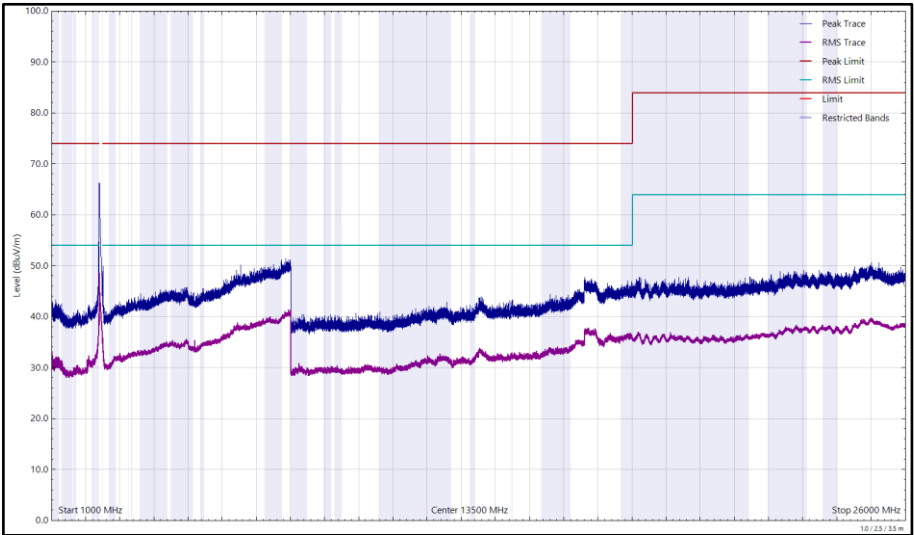
Figure 101 - 2437 MHz (CH6), HE20, RU26-0, Core 0 + Core 1, 1 GHz to 26 GHz, Vertical
