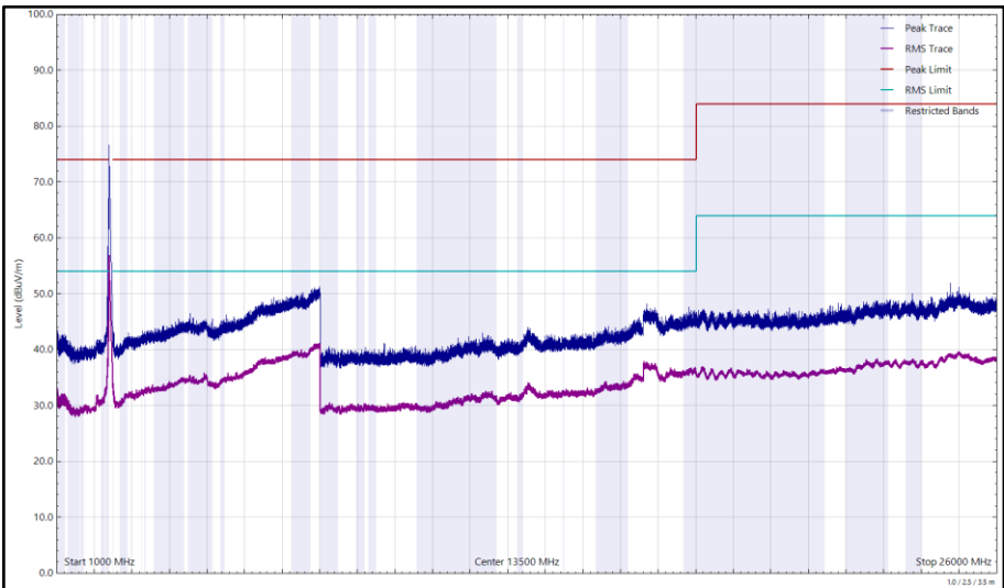
Figure 97 - 2412 MHz (CH1), HE20, RU26-0, Core 0 + Core 1, 1 GHz to 26 GHz, Vertical
