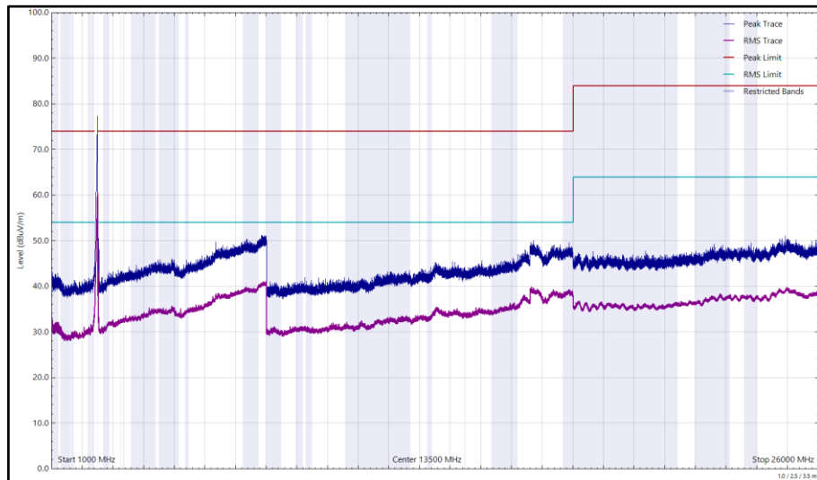
Figure 102 - 2472 MHz (CH13), HE20, RU26-0, Core 0 + Core 1, 1 GHz to 26 GHz, Horizontal
