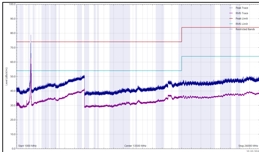
Figure 103 - 2472 MHz (CH13), HE20, RU26-0, Core 0 + Core 1, 1 GHz to 26 GHz, Vertical
