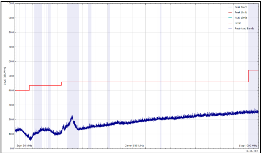
Figure 100 - 2437 MHz (CH6), HE20, RU26-0, Core 0 + Core 1, 30 MHz to 1 GHz, Vertical
