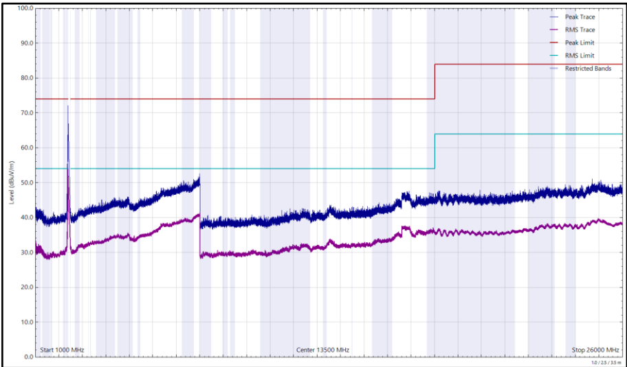
Figure 96 - 2412 MHz (CH1), HE20, RU26-0, Core 0 + Core 1, 1 GHz to 26 GHz, Horizontal
