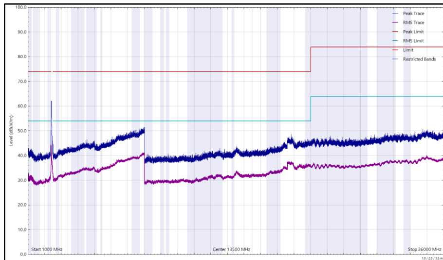
Figure 99 - 2437 MHz (CH6), HE20, RU26-0, Core 0 + Core 1, 1 GHz to 26 GHz, Horizontal
