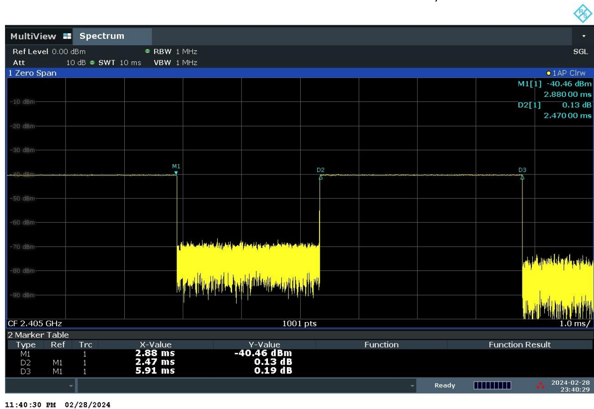
Figure 7-8 802.15.4 Transmission Plot – Antenna WF7/WF8/WF9, Variant 1
