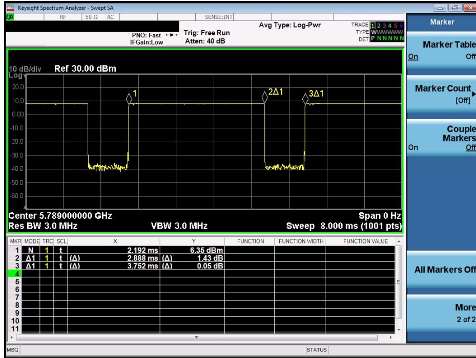
Equation 7-19 NB UNII 3 (BDR) Duty Cycle Calculation – Antenna WF7, Variant 2
