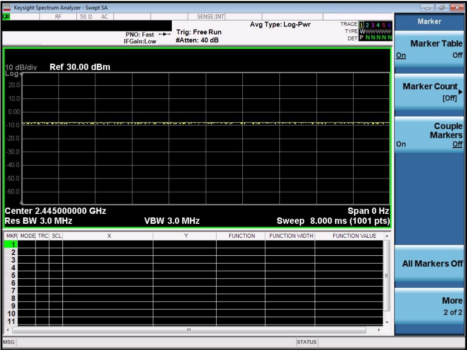
Figure 7-10 802.15.4 Transmission Plot – Antenna WF7/WF8/WF9, Variants 1/2
