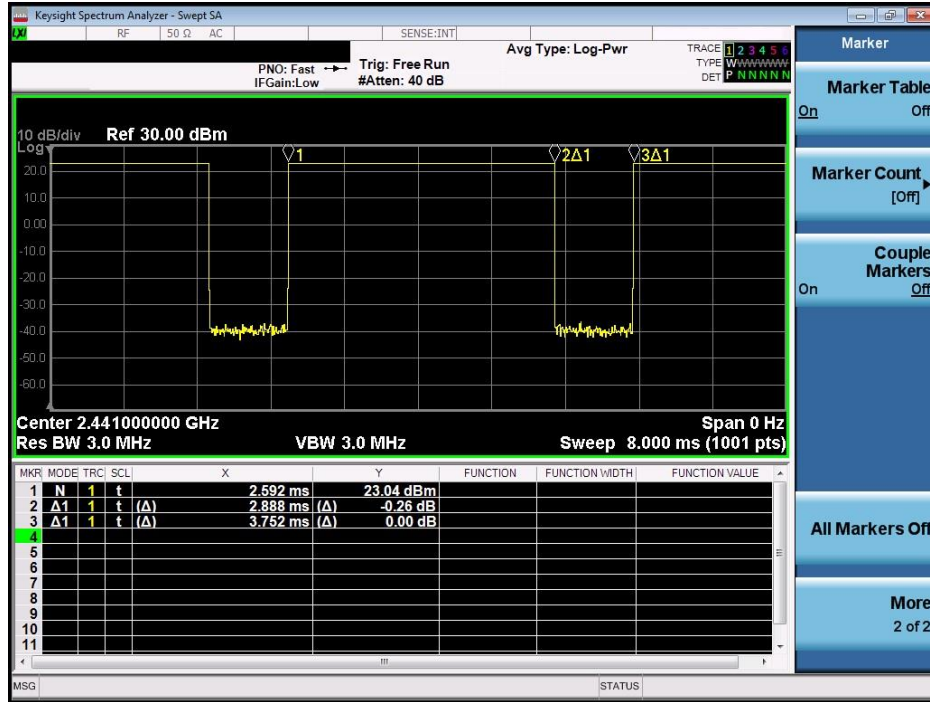
Equation 7-2 Bluetooth Duty Cycle Calculation – Antenna WF7, Variant 2
