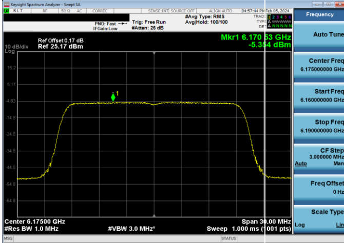
Plot 7-182. Power Spectral Density Plot LPI Antenna WF5B (20MHz 802.11ax (UNII Band 5) – Ch. 45, MCS2)
