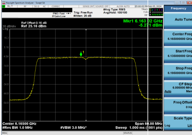
Plot 7-183. Power Spectral Density Plot LPI Antenna WF5B (40MHz 802.11ax (UNII Band 5) – Ch. 43, MCS2)
