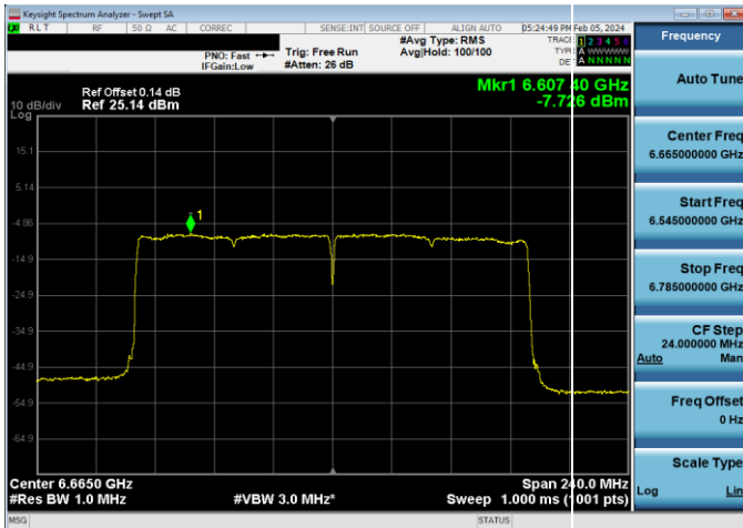
Plot 7-195. Power Spectral Density Plot LPI Antenna WF5B (160MHz 802.11ax (UNII Band 7) – Ch. 143, MCS2)
