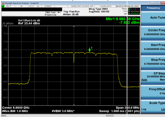
Plot 7-231. Power Spectral Density Plot LPI Antenna WF5B (160MHz 802.11ax (UNII Band 7) – Ch. 143, MCS11)
