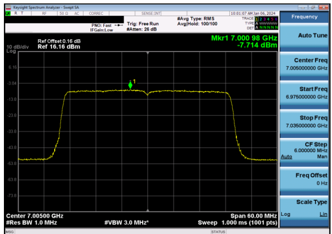
Plot 7-182. Power Spectral Density Plot LPI Antenna 5T LPI (40MHz 802.11ax (UNII Band 8) – Ch. 211, MCS4)
