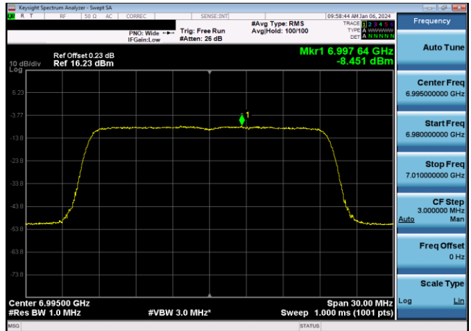
Plot 7-181. Power Spectral Density Plot LPI Antenna 5T LPI (20MHz 802.11ax (UNII Band 8) – Ch. 209, MCS4)
