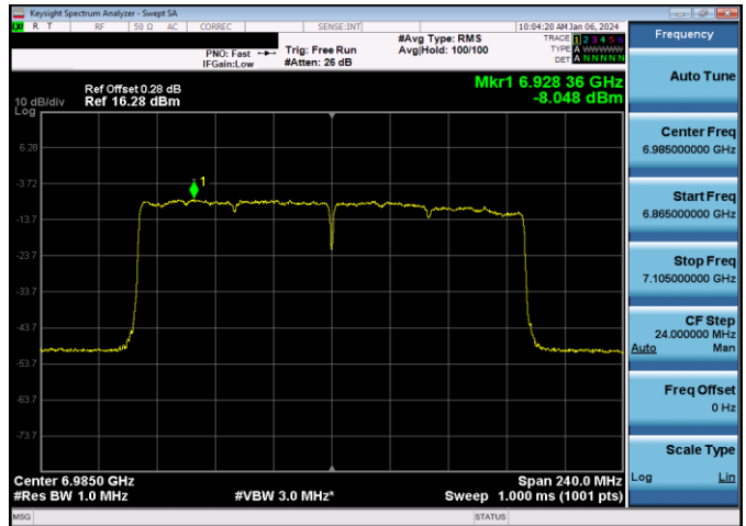
Plot 7-184. Power Spectral Density Plot LPI Antenna 5T LPI (160MHz 802.11ax (UNII Band 8) – Ch. 207, MCS4)
