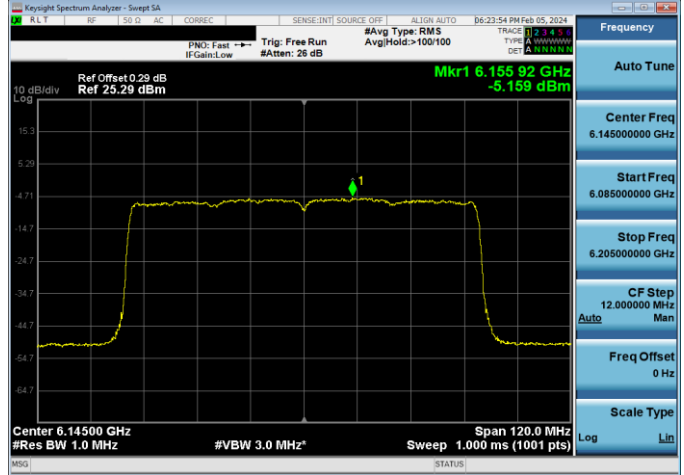
Plot 7-220. Power Spectral Density Plot LPI Antenna WF5B (80MHz 802.11ax (UNII Band 5) – Ch. 39, MCS11)
