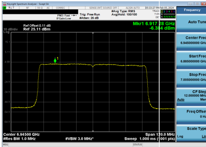
Plot 7-199. Power Spectral Density Plot LPI Antenna WF5B (80MHz 802.11ax (UNII Band 8) – Ch. 199, MCS2)
