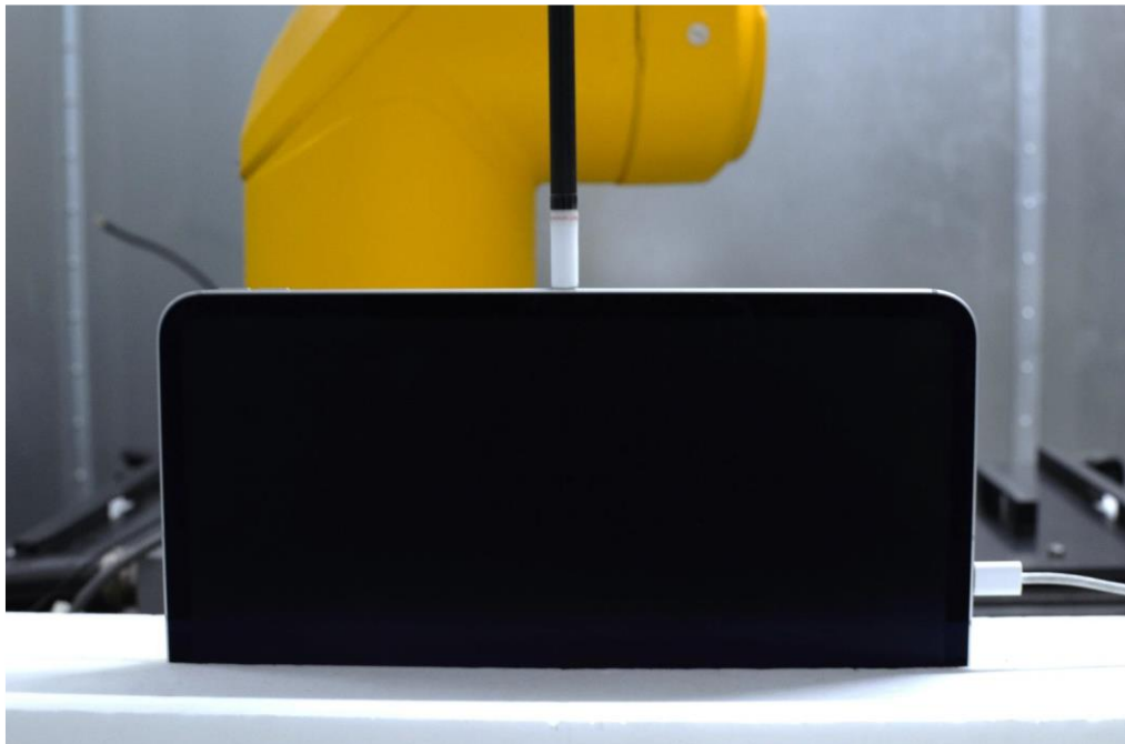
Near Field Power Density Test Setup Photo 18: Right Edge at 2mm – WF7/WF8/WF5B
