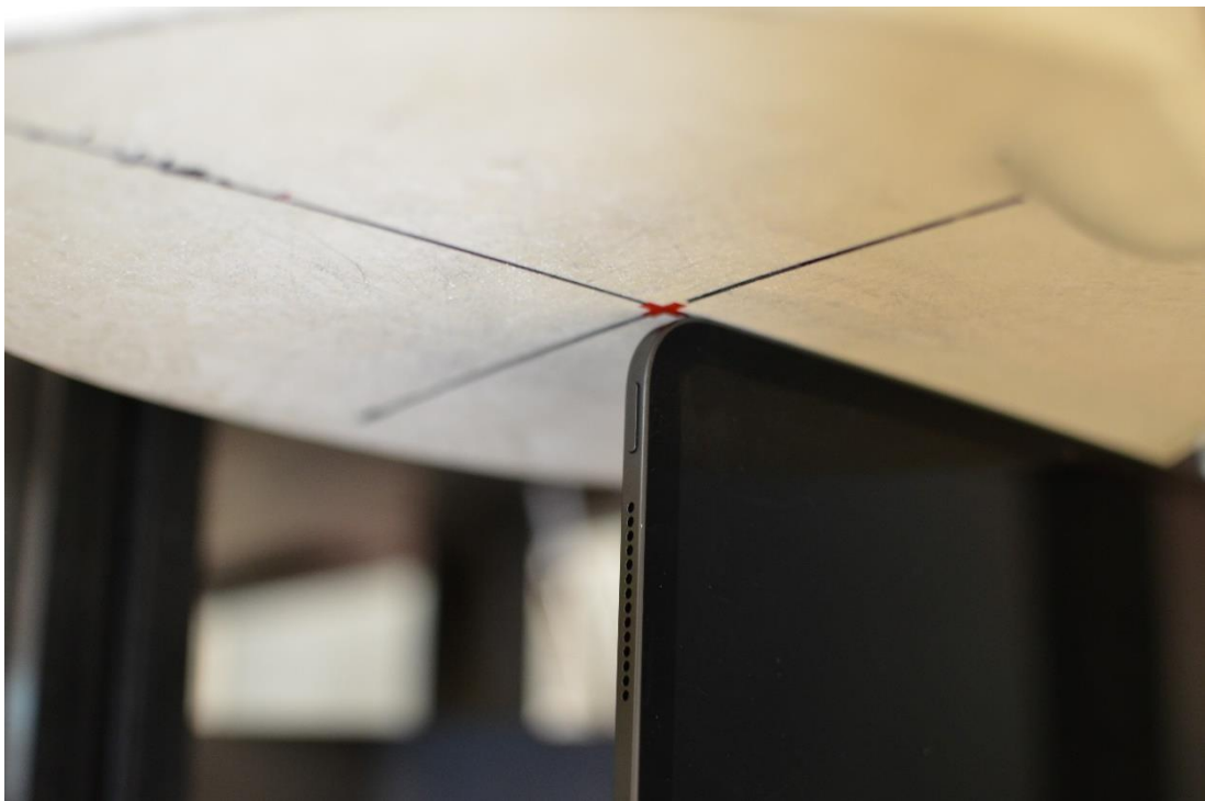
SAR Test Setup Photo 5: Right Edge at 0mm – Ant WF7/WF8/WF9
