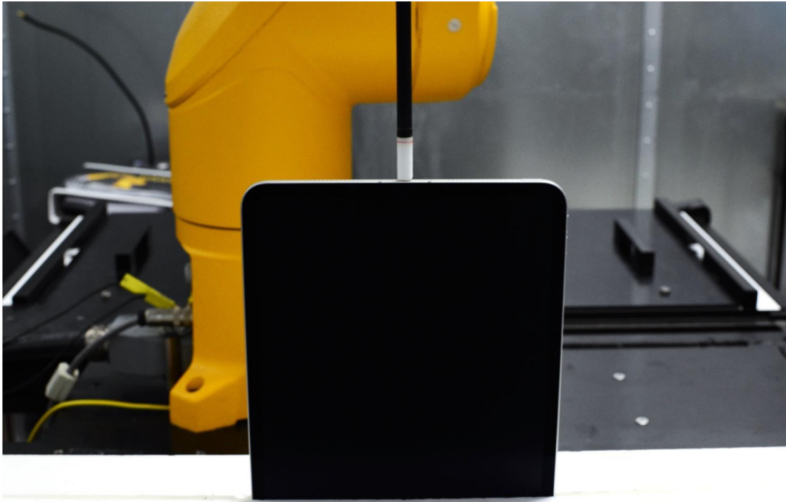
Near Field Power Density Test Setup Photo 15: Top Edge at 2mm – WF7/WF8/WF5B
