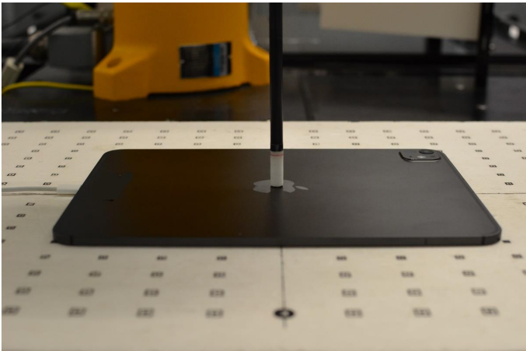
Near Field Power Density Test Setup Photo 14: Backside at 2mm – WF5B/WF7/WF8
