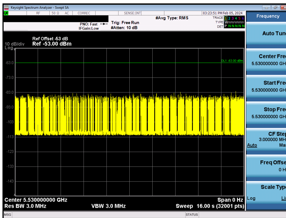
Figure 9-7. 5530MHz - Channel Loading - Mode 3 (80MHz)
