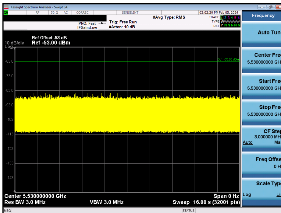
Figure 9-1. 5530MHz - Channel Loading - Mode 1 (80MHz)
