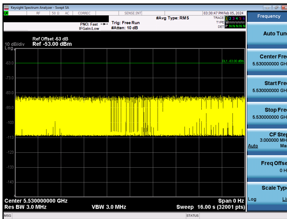
Figure 9-9. 5530 MHz - Channel Loading - Mode 4 (80MHz)
