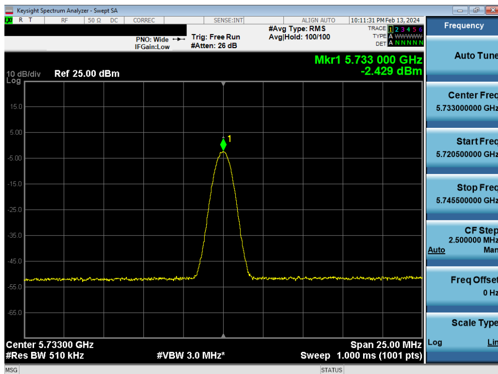
Plot 7-31. PSD Antenna 5b (BDR, iPA 5733MHz)
