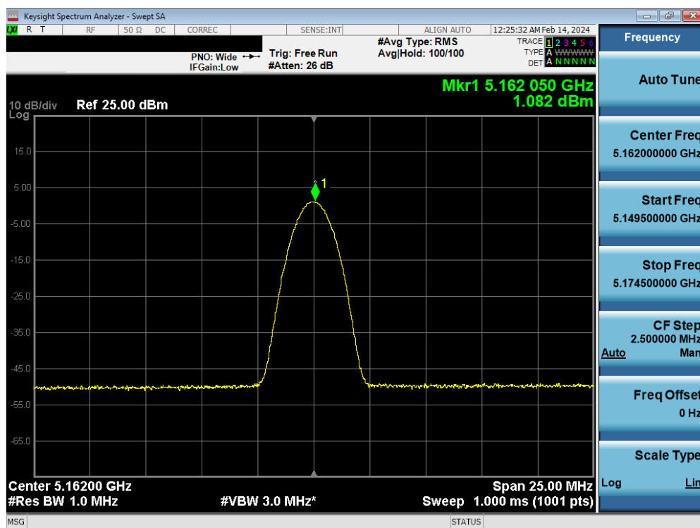
Plot 7-68. FCC/ISED PSD TxBF Antenna 4a (BDR, iPA – 5162MHz)
