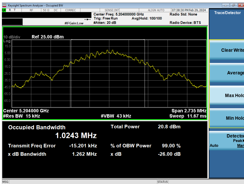
Plot 7-2. 26dB BW & 99% OBW Antenna 5b (BDR GFSK, ePA- 5204MHz)
