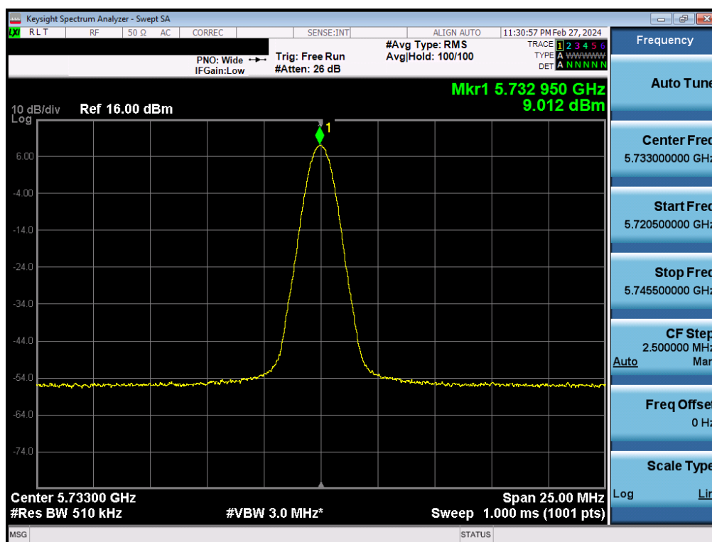
Plot 7-43. PSD Antenna 4a (BDR, ePA 5733MHz)
