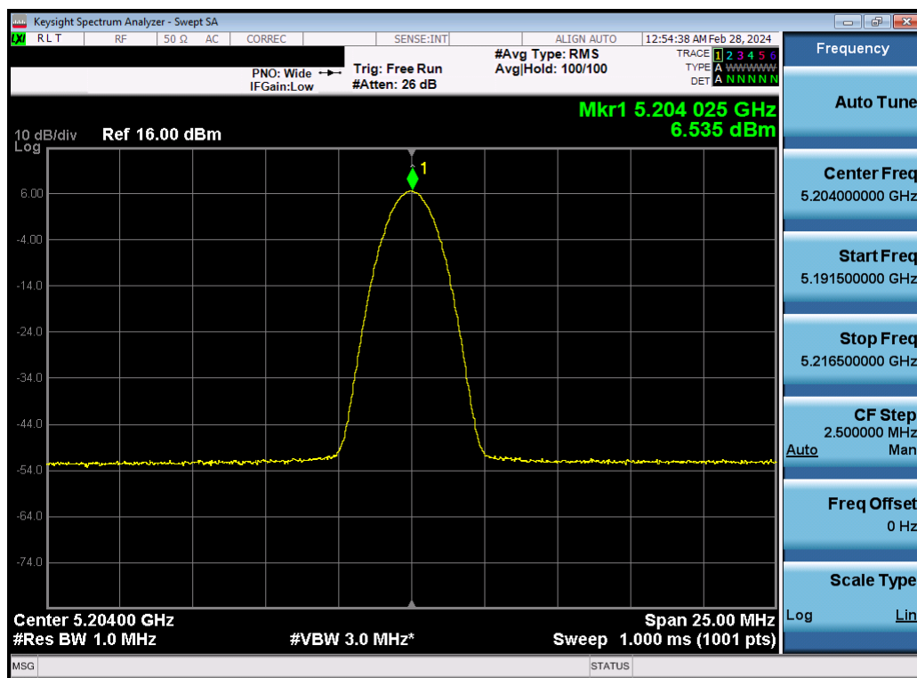
Plot 7-26. ISED PSD Antenna 5b (BDR, ePA – 5204MHz)
