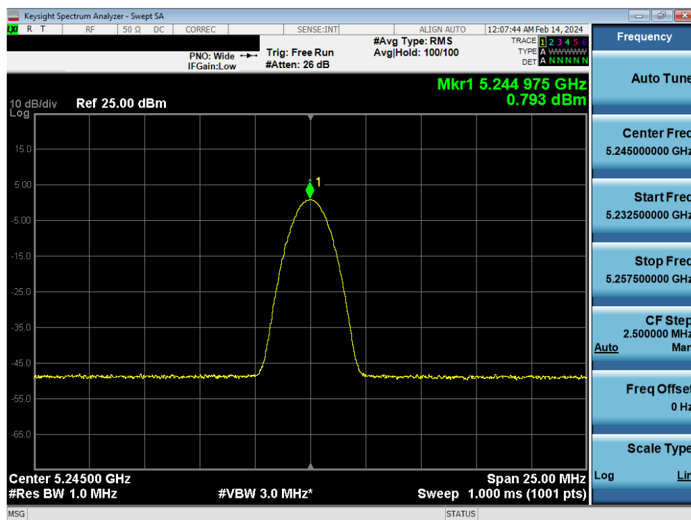
Plot 7-39. FCC/ISED PSD Antenna 4a (BDR, iPA– 5245MHz)
