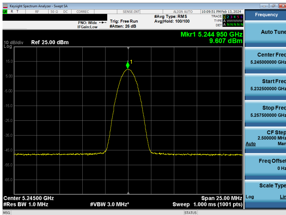
Plot 7-21. FCC PSD Antenna 5b (BDR, ePA- 5245MHz)
