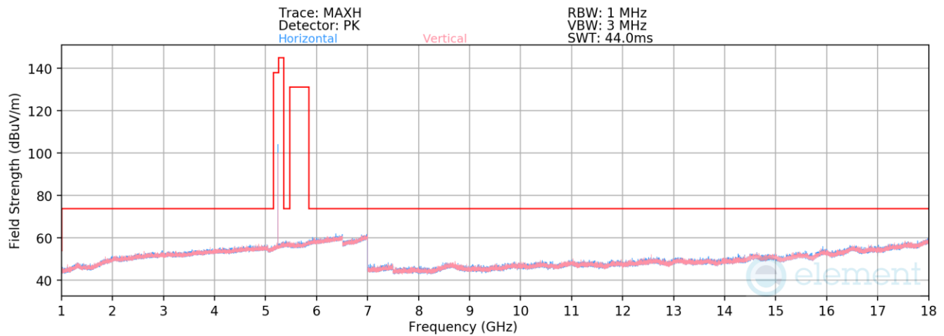
Plot 7-99. Radiated Spurious Emissions 1-18GHz Antenna 4a (BDR GFSK ePA - 5245MHz)
