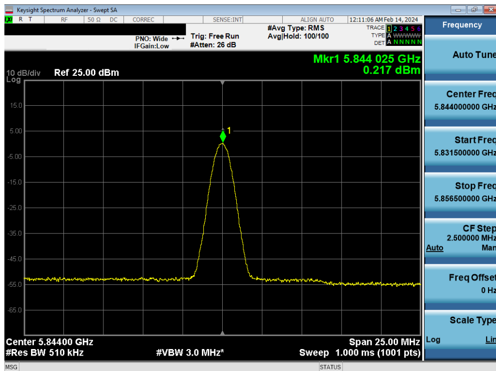
Plot 7-48. PSD Antenna 4a (BDR, iPA 5844MHz)
