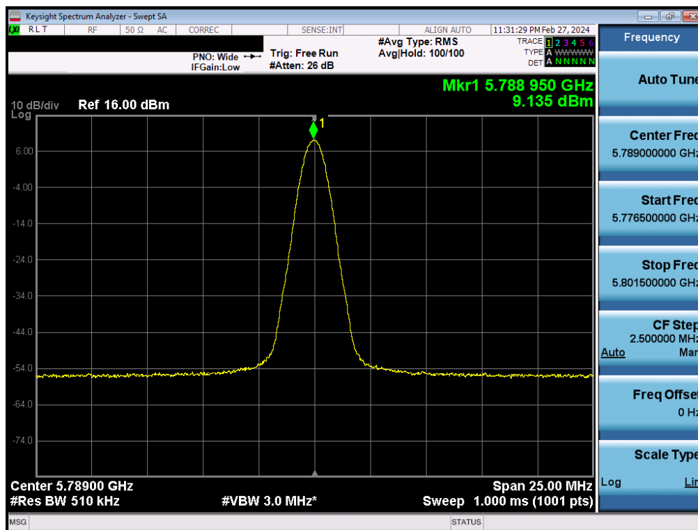
Plot 7-44. PSD Antenna 4a (BDR, ePA 5789MHz)
