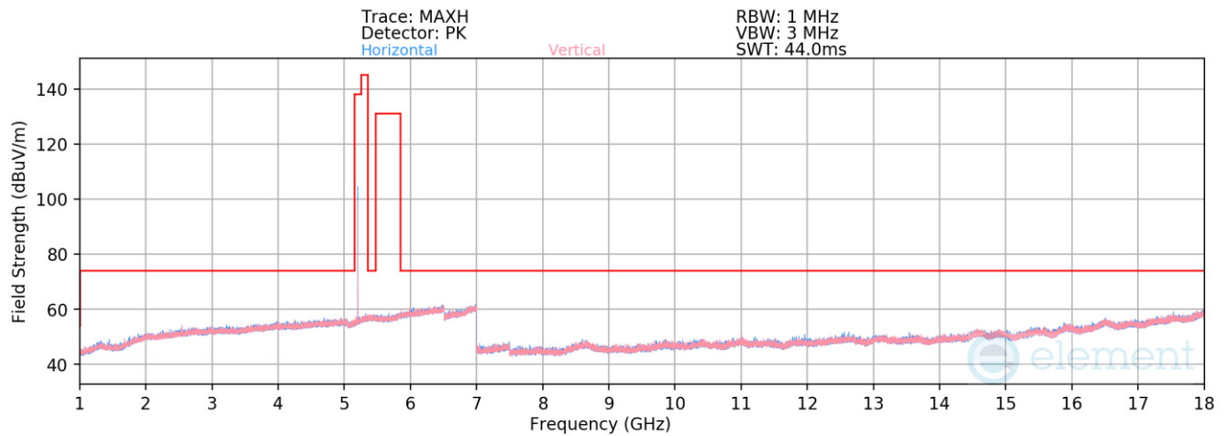
Plot 7-98. Radiated Spurious Emissions 1-18GHz Antenna 4a (BDR GFSK ePA – 5204MHz)
