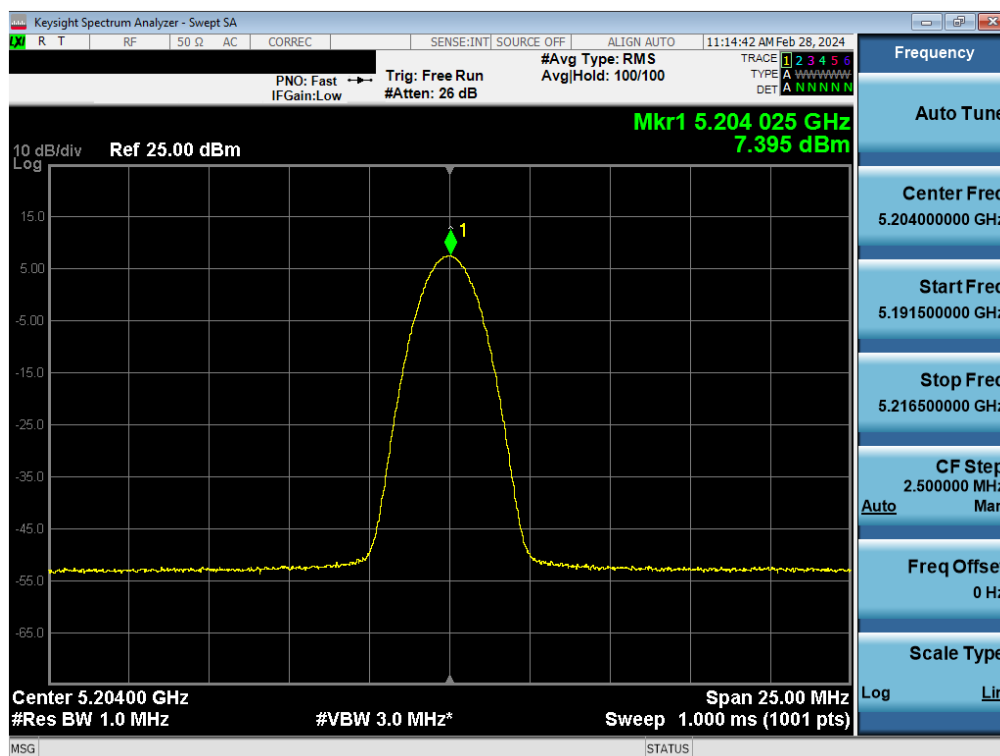
Plot 7-41. ISED PSD Antenna 4a (BDR, ePA – 5204MHz)
