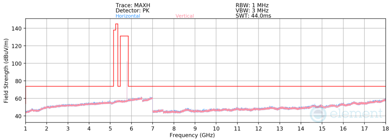
Plot 7-101. Radiated Spurious Emissions 1-18GHz Antenna 4a (BDR GFSK ePA - 5789MHz)
