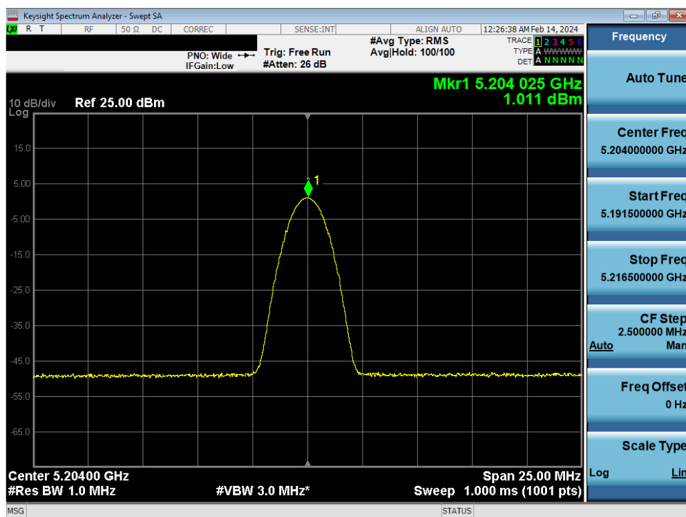
Plot 7-70. FCC/ISED PSD TxBF Antenna 4a (BDR, iPA – 5204MHz)
