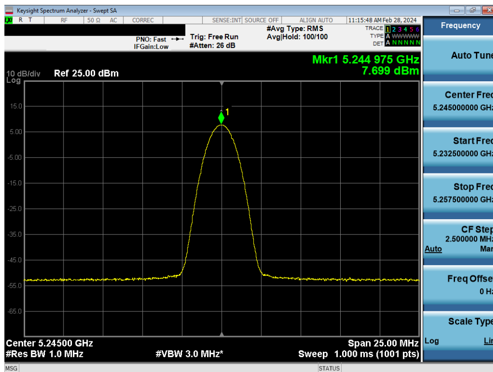
Plot 7-42. ISED PSD Antenna 4a (BDR, ePA- 5245MHz)
