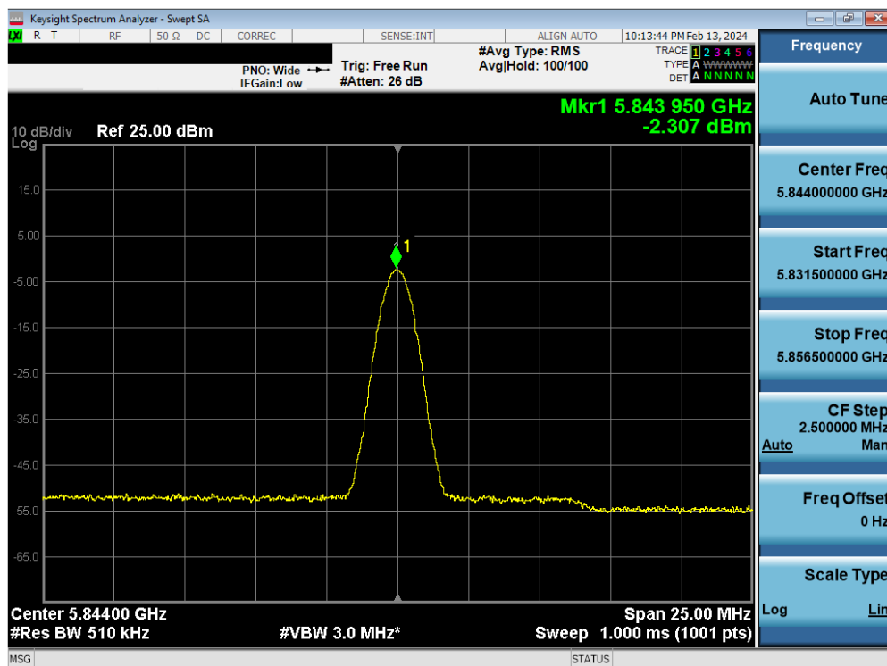
Plot 7-33. PSD Antenna 5b (BDR, iPA 5844MHz)
