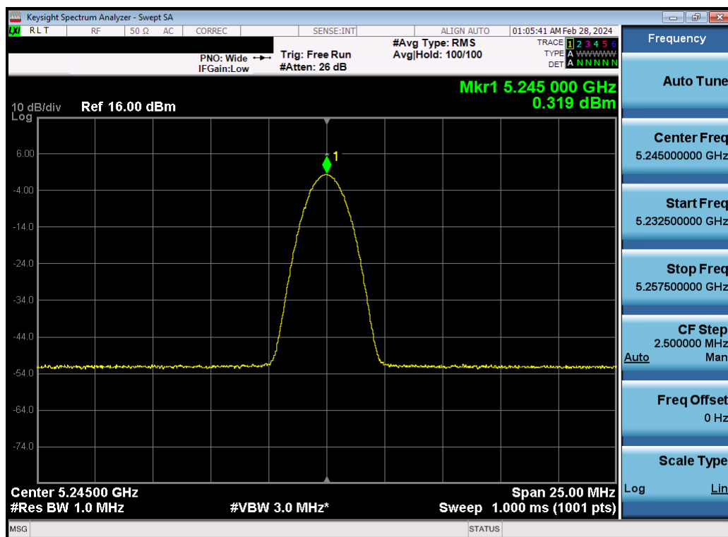
Plot 7-77. ISED PSD TxBF Antenna 5b (BDR, ePA– 5245MHz)
