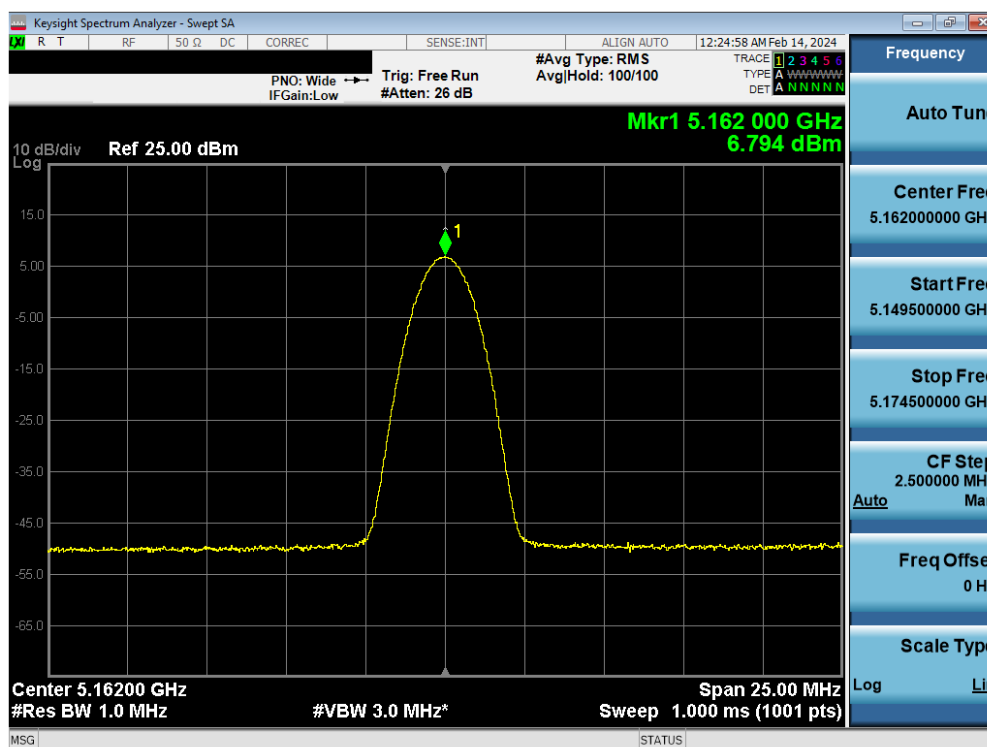
Plot 7-62. FCC PSD TxBF Antenna 4a (BDR, ePA – 5162MHz)
