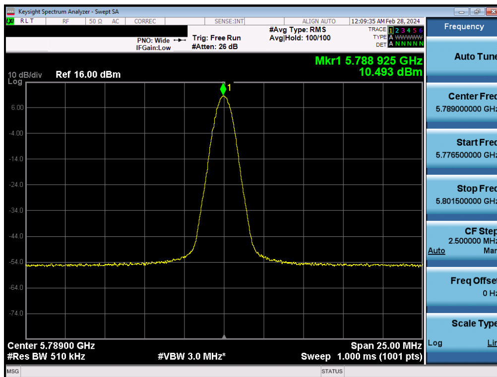
Plot 7-56. PSD Antenna 2a (BDR, ePA 5789MHz)
