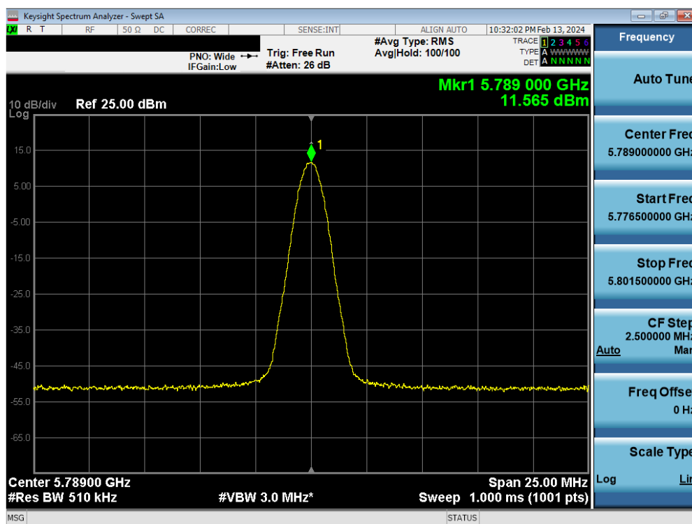
Plot 7-81. PSD TxBF Antenna 5b (BDR, ePA 5789MHz)
