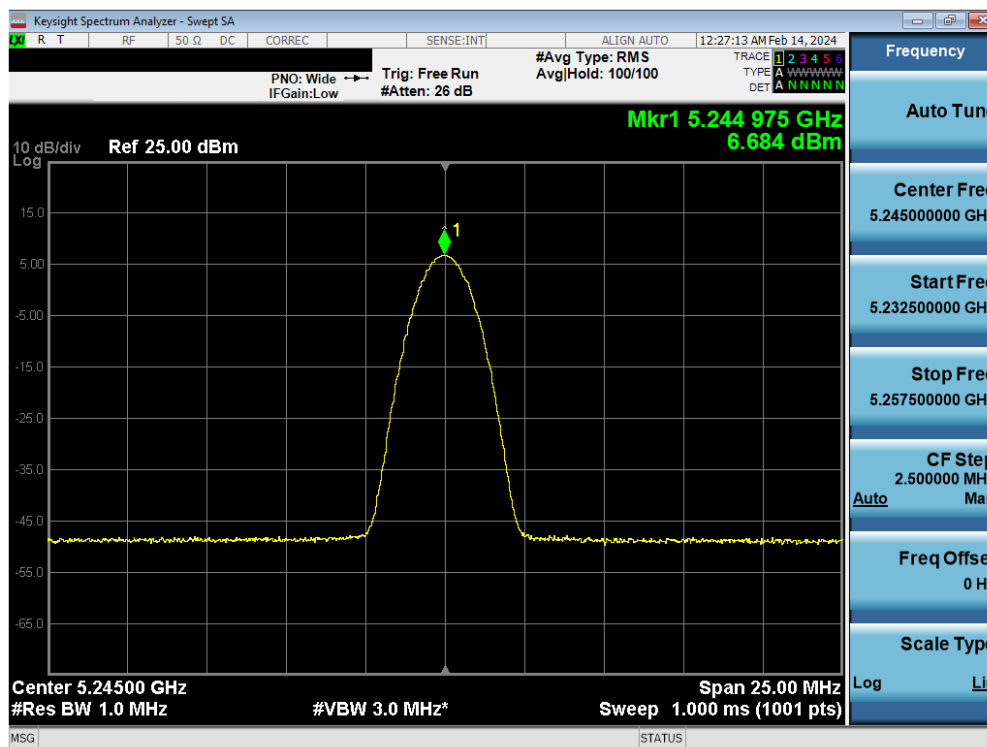
Plot 7-66. FCC PSD TxBF Antenna 4a (BDR, ePA- 5245MHz)
