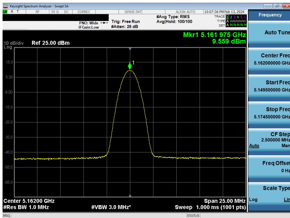
Plot 7-19. FCC PSD Antenna 5b (BDR, ePA – 5162MHz)
