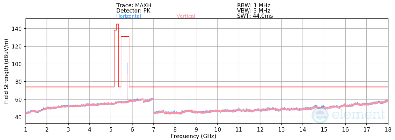
Plot 7-95. Radiated Spurious Emissions 1-18GHz Antenna 5b (BDR GFSK ePA- 5789MHz)
