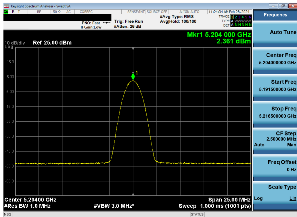
Plot 7-76. ISED PSD TxBF Antenna 4a (BDR, ePA – 5204MHz)
