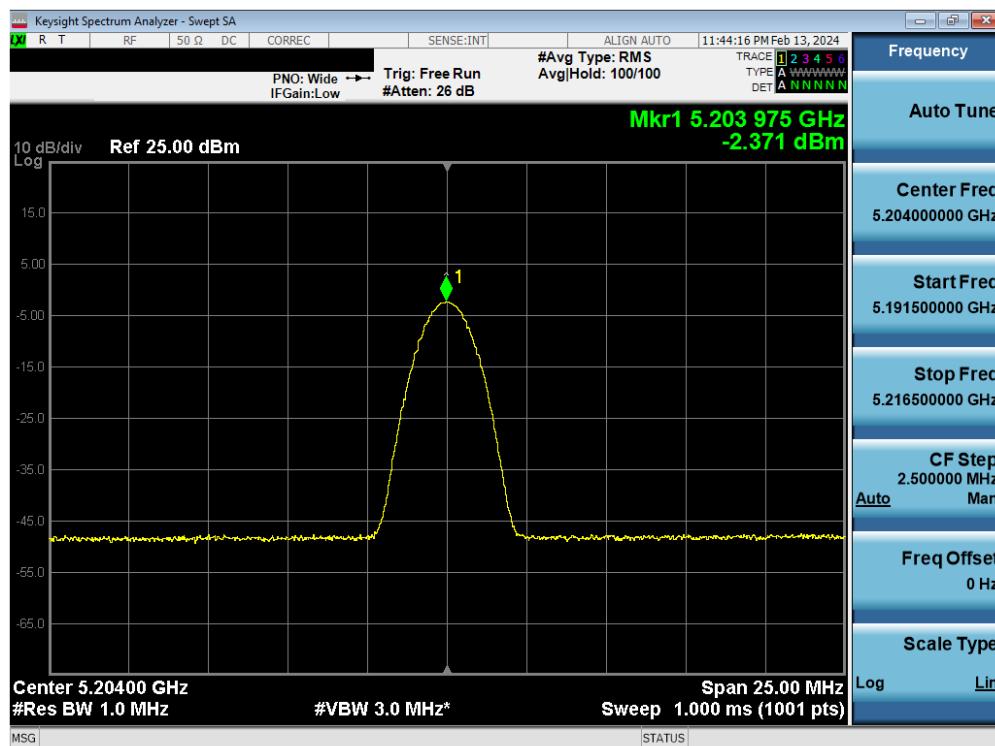
Plot 7-53. PSD Antenna 2a (BDR, iPA – 5204MHz)
