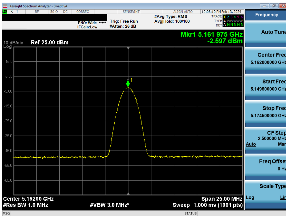
Plot 7-22. FCC/ISED PSD Antenna 5b (BDR, iPA - 5162MHz)
