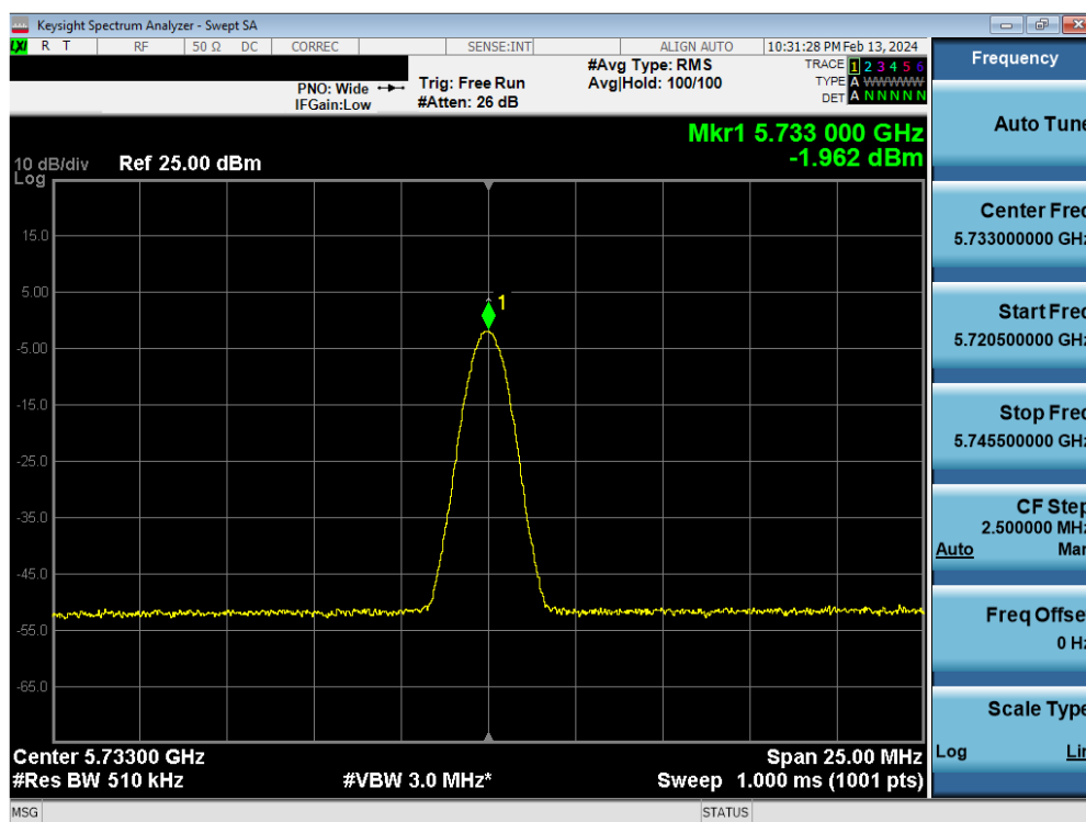
Plot 7-85. PSD TxBF Antenna 5b (BDR, iPA 5733MHz)
