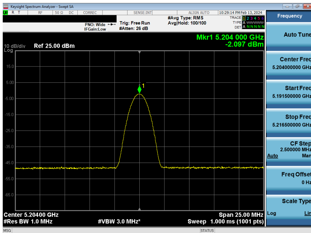
Plot 7-69. FCC/ISED PSD TxBF Antenna 5b (BDR, iPA – 5204MHz)
