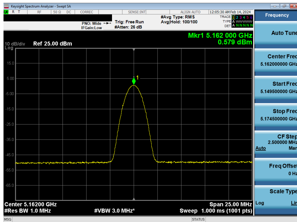
Plot 7-37. FCC/ISED PSD Antenna 4a (BDR, iPA – 5162MHz)
