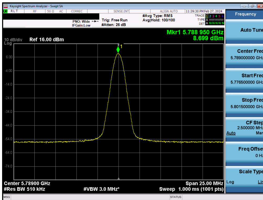
Plot 7-82. PSD TxBF Antenna 4a (BDR, ePA 5789MHz)
