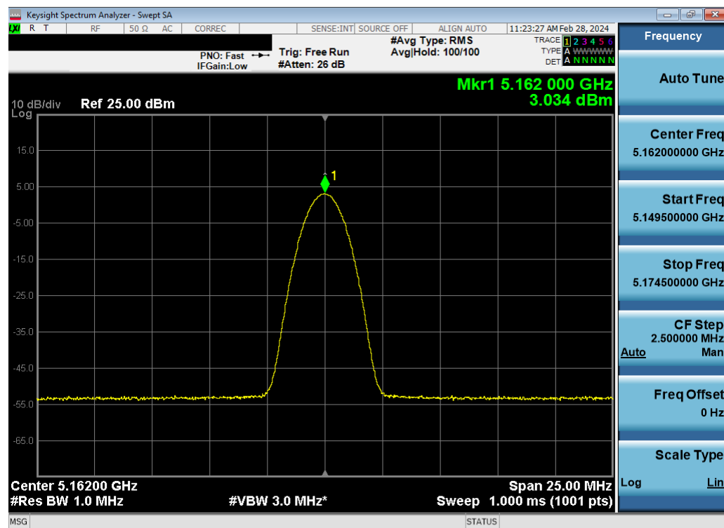
Plot 7-74. ISED PSD TxBF Antenna 4a (BDR, ePA – 5162MHz)
