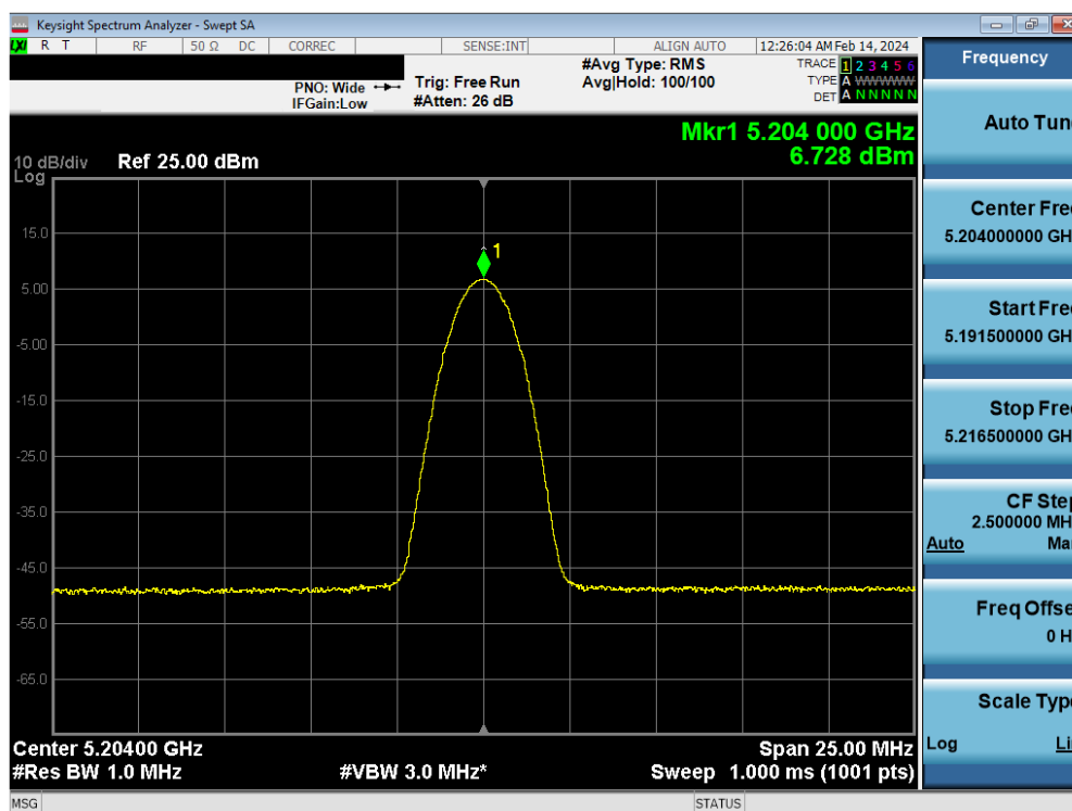
Plot 7-64. FCC PSD TxBF Antenna 4a (BDR, ePA – 5204MHz)
