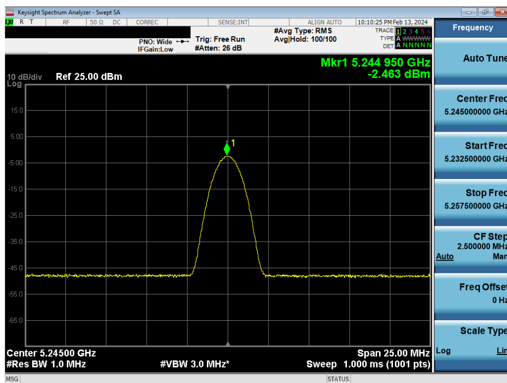
Plot 7-24. FCC/ISED PSD Antenna 5b (BDR, iPA– 5245MHz)
