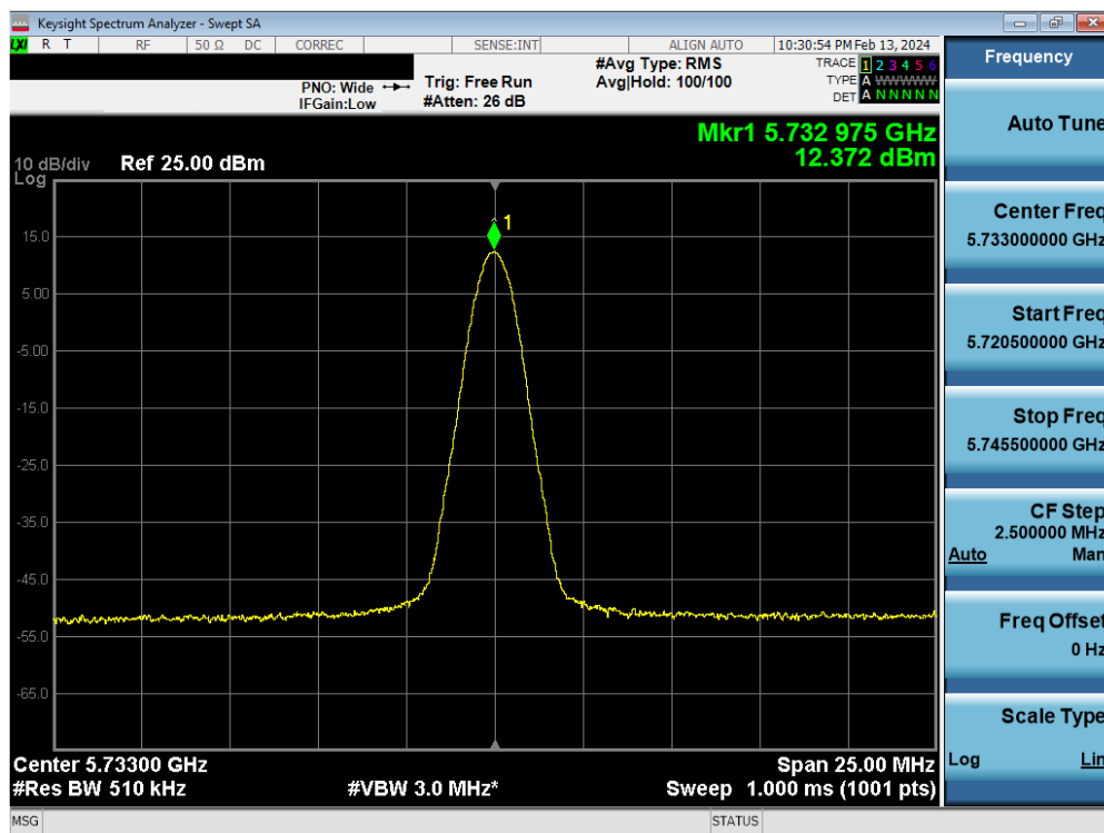
Plot 7-79. PSD TxBF Antenna 5b (BDR, ePA 5733MHz)
