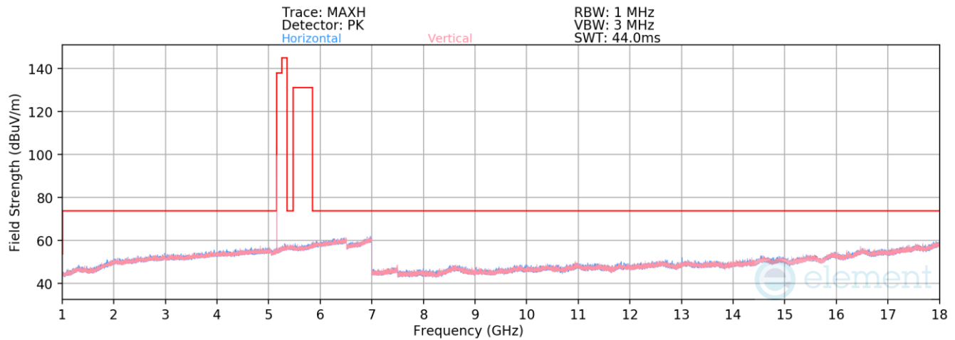
Plot 7-97. Radiated Spurious Emissions 1-18GHz Antenna 4a (BDR GFSK ePA – 5162MHz)
