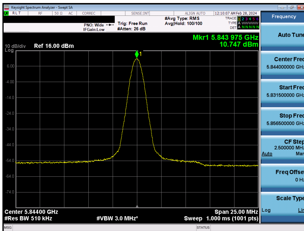
Plot 7-57. PSD Antenna 2a (BDR, ePA 5844MHz)
