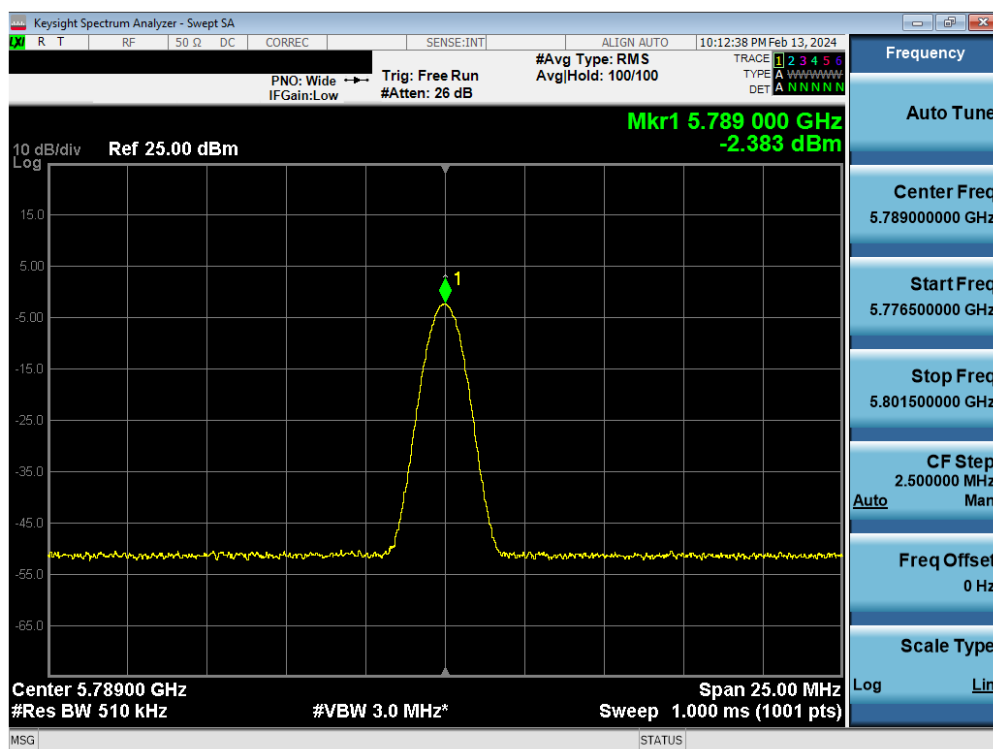
Plot 7-32. PSD Antenna 5b (BDR, iPA 5789MHz)
