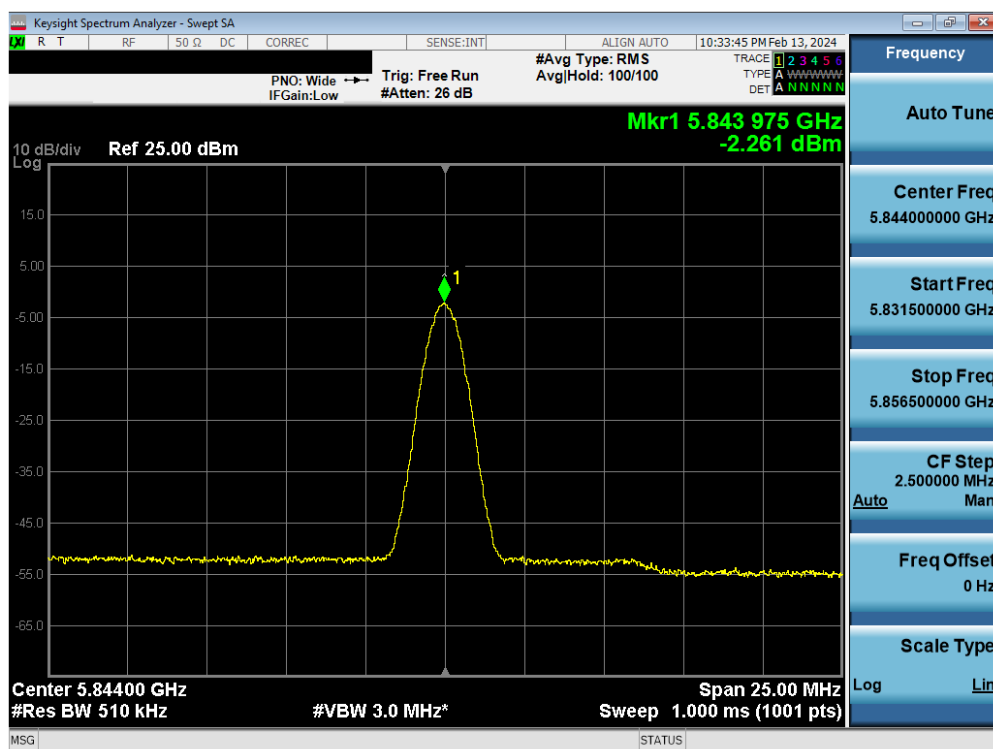
Plot 7-89. PSD TxBF Antenna 5b (BDR, iPA 5844MHz)
