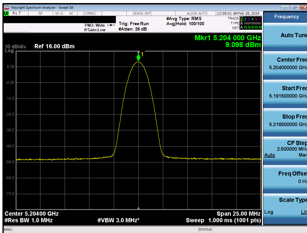
Plot 7-50. PSD Antenna 2a (BDR, ePA – 5204MHz)
