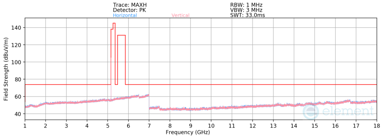
Plot 7-103. Radiated Spurious Emissions 1-18GHz Antenna 2a (BDR GFSK ePA – 5162MHz)
