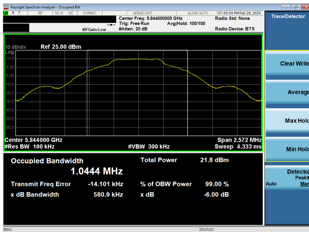
Plot 7-12. 6dB BW & 99% OBW Antenna 5b (BDR GFSK, 5844MHz)
