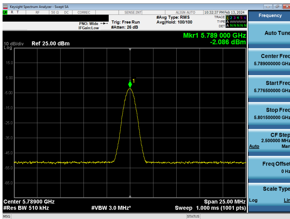
Plot 7-87. PSD TxBF Antenna 5b (BDR, iPA 5789MHz)
