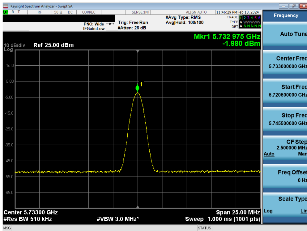
Plot 7-58. PSD Antenna 2a (BDR, iPA 5733MHz)
