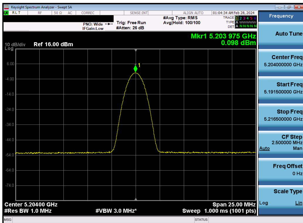
Plot 7-75. ISED PSD TxBF Antenna 5b (BDR, ePA – 5204MHz)
