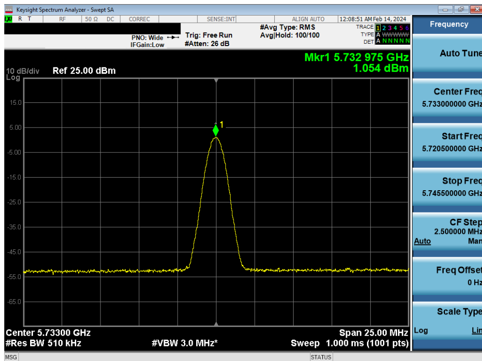
Plot 7-46. PSD Antenna 4a (BDR, iPA 5733MHz)
