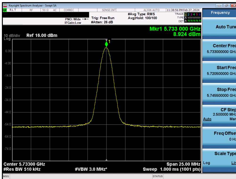
Plot 7-80. PSD TxBF Antenna 4a (BDR, ePA 5733MHz)
