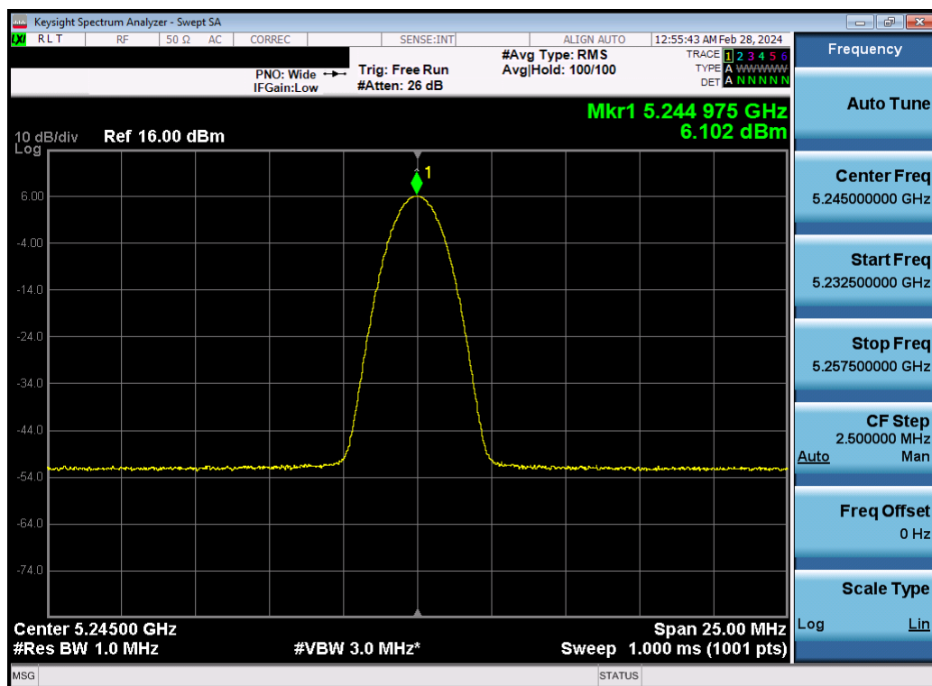
Plot 7-27. ISED PSD Antenna 5b (BDR, ePA- 5245MHz)
