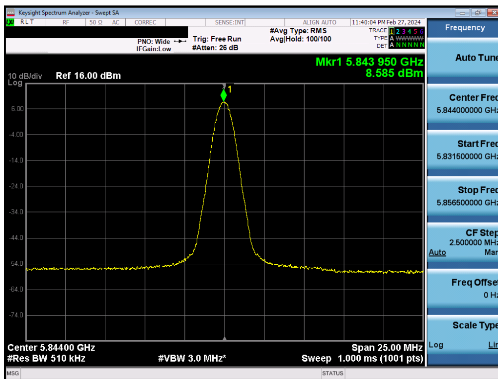
Plot 7-84. PSD TxBF Antenna 4a (BDR, ePA 5844MHz)
