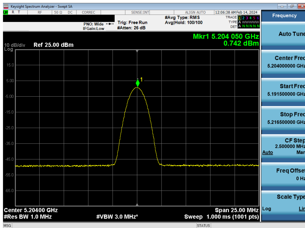
Plot 7-38. FCC/ISED PSD Antenna 4a (BDR, iPA – 5204MHz)
