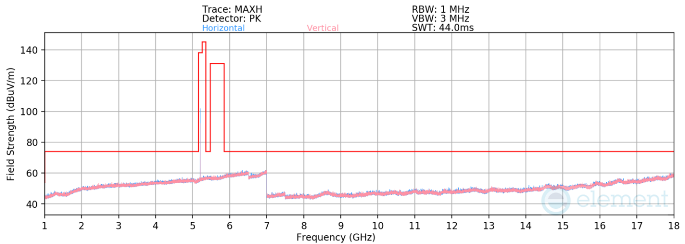
Plot 7-92. Radiated Spurious Emissions 1-18GHz Antenna 5b (BDR GFSK ePA – 5204MHz)
