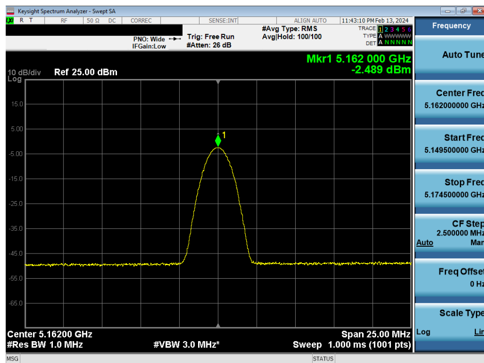
Plot 7-52. PSD Antenna 2a (BDR, iPA - 5162MHz)
