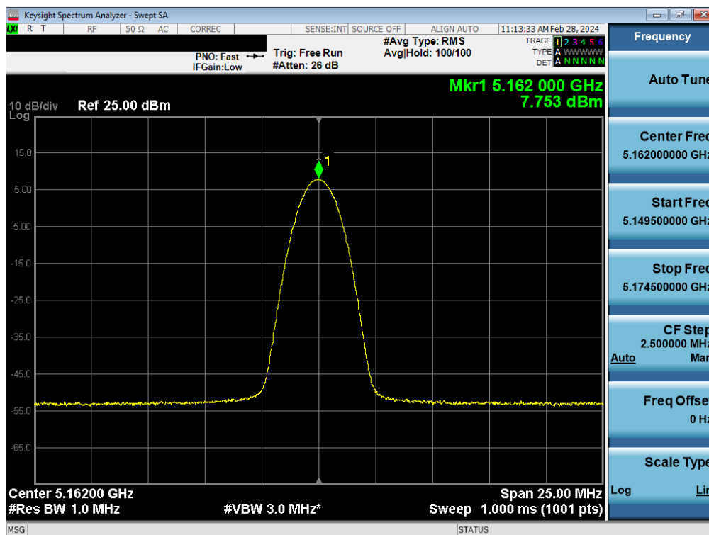
Plot 7-40. ISED PSD Antenna 4a (BDR, ePA – 5162MHz)
