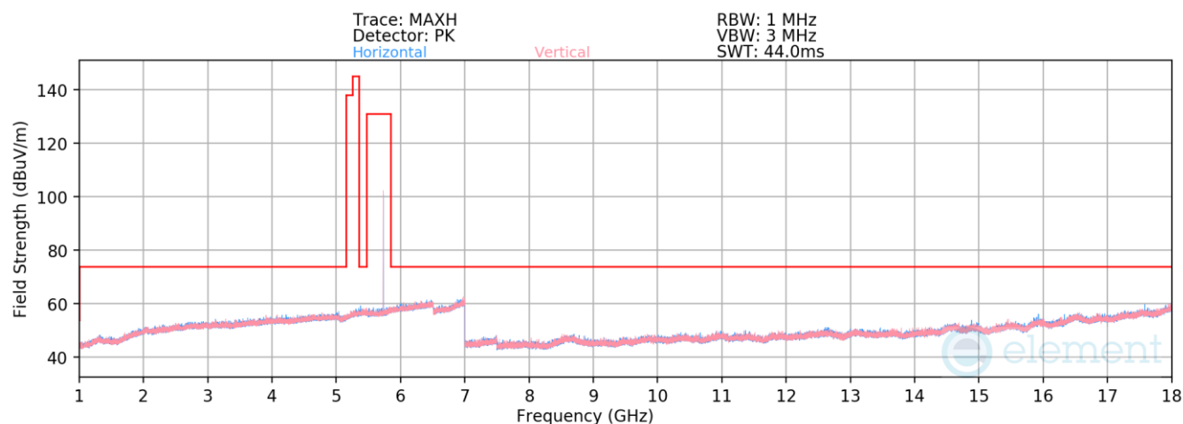
Plot 7-100. Radiated Spurious Emissions 1-18GHz Antenna 4a (BDR GFSK ePA – 5733MHz)
