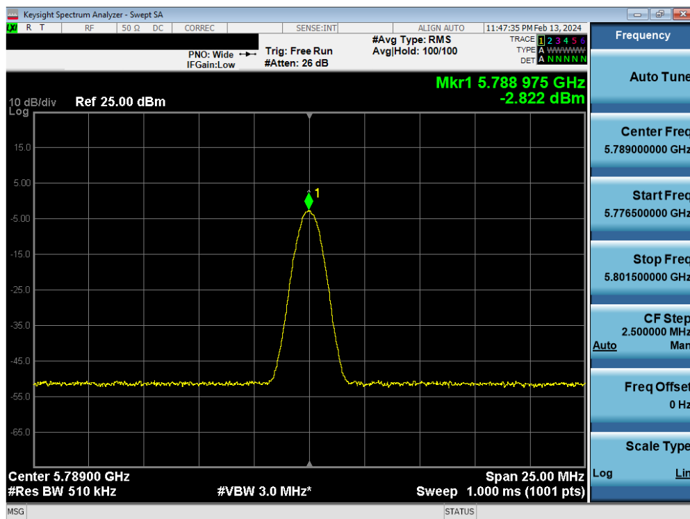
Plot 7-59. PSD Antenna 2a (BDR, iPA 5789MHz)
