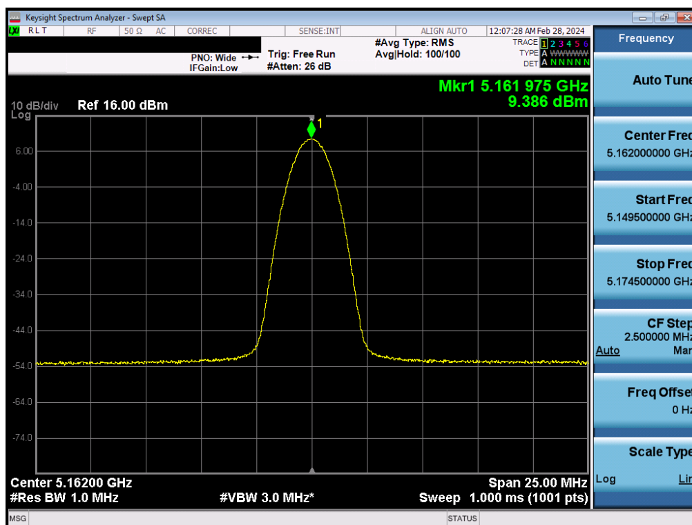
Plot 7-49. PSD Antenna 2a (BDR, ePA – 5162MHz)
