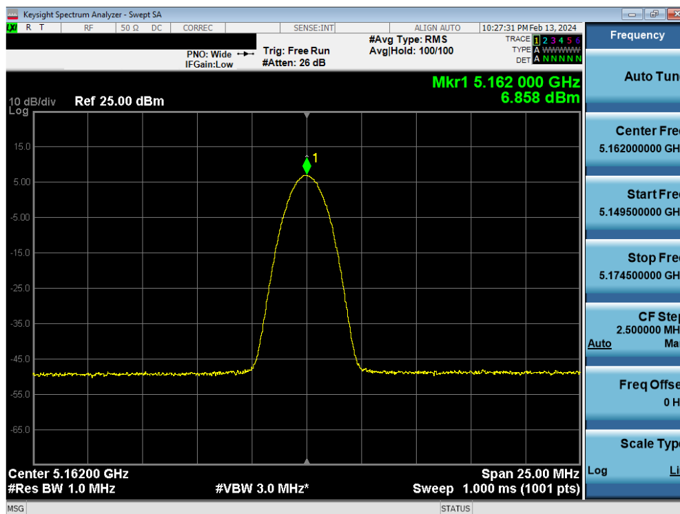
Plot 7-61. FCC PSD TxBF Antenna 5b (BDR, ePA – 5162MHz)
