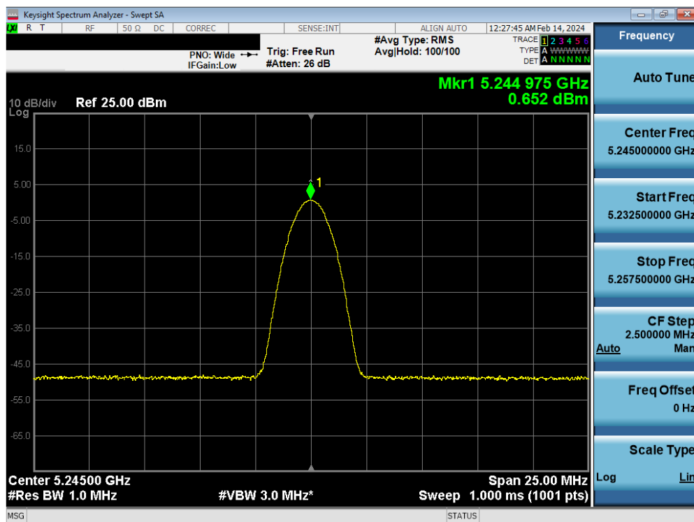
Plot 7-72. FCC/ISED PSD TxBF Antenna 4a (BDR, iPA- 5245MHz)
