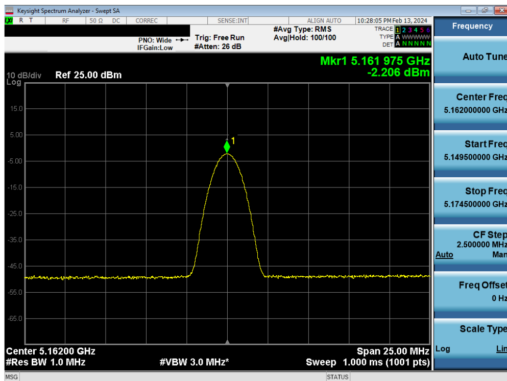
Plot 7-67. FCC/ISED PSD TxBF Antenna 5b (BDR, iPA – 5162MHz)
