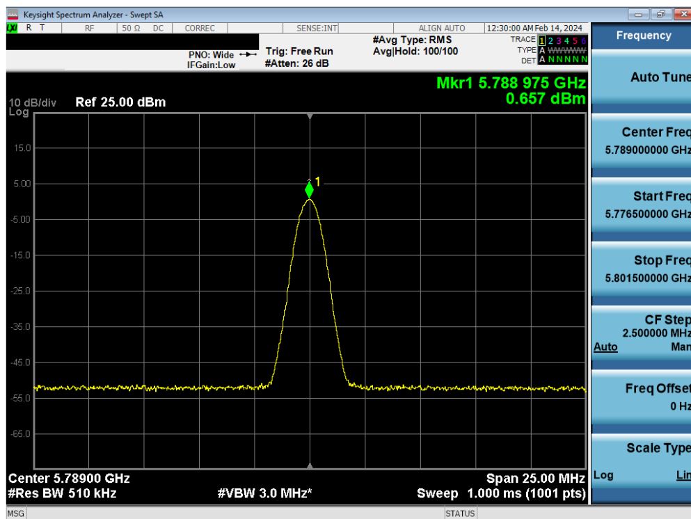
Plot 7-88. PSD TxBF Antenna 4a (BDR, iPA 5789MHz)
