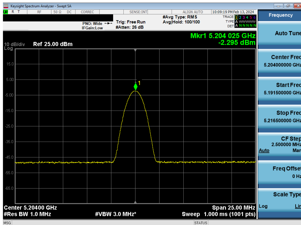
Plot 7-23. FCC/ISED PSD Antenna 5b (BDR, iPA – 5204MHz)
