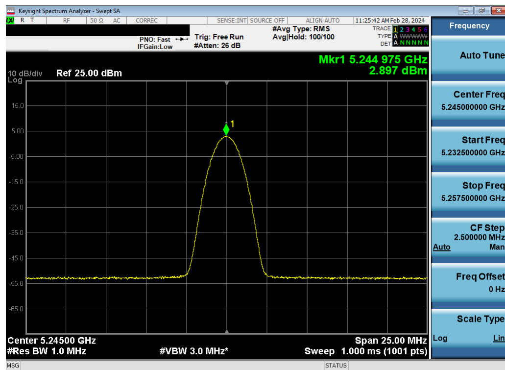
Plot 7-78. ISED PSD TxBF Antenna 4a (BDR, ePA– 5245MHz)
