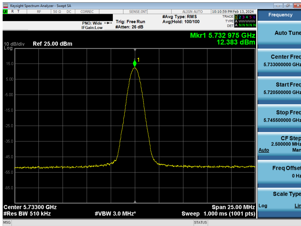
Plot 7-28. PSD Antenna 5b (BDR, ePA 5733MHz)
