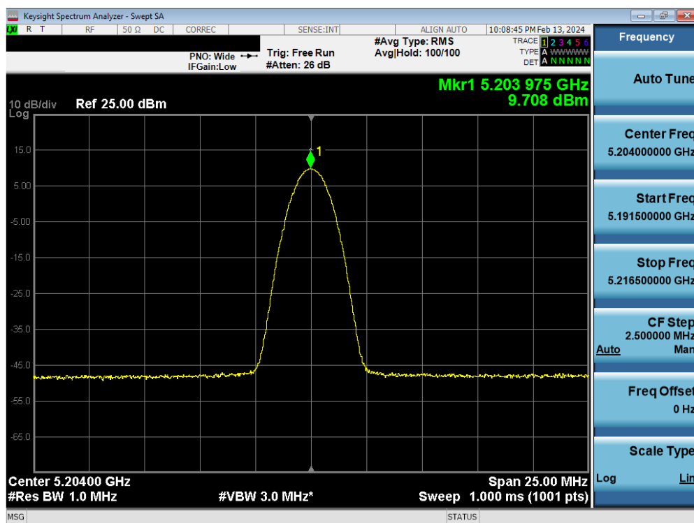
Plot 7-20. FCC PSD Antenna 5b (BDR, ePA – 5204MHz)
