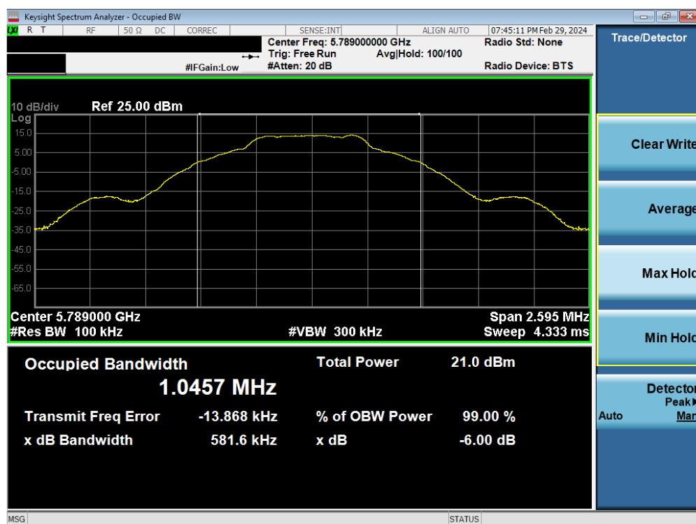
Plot 7-11. 6dB BW & 99% OBW Antenna 5b (BDR GFSK, 5789MHz)
