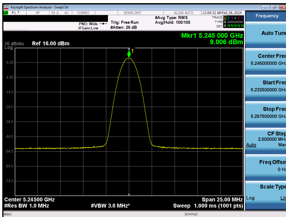
Plot 7-51. PSD Antenna 2a (BDR, ePA- 5245MHz)
