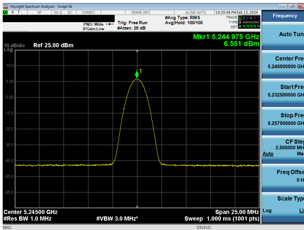
Plot 7-65. FCC PSD TxBF Antenna 5b (BDR, ePA- 5245MHz)
