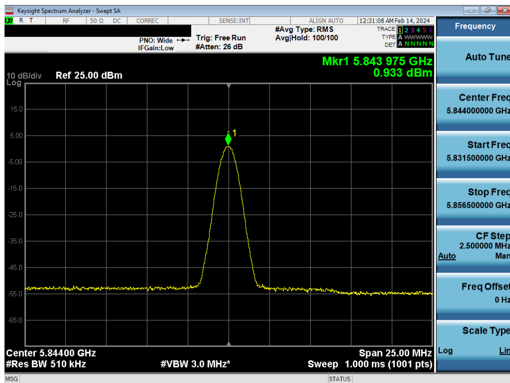
Plot 7-90. PSD TxBF Antenna 4a (BDR, iPA 5844MHz)
