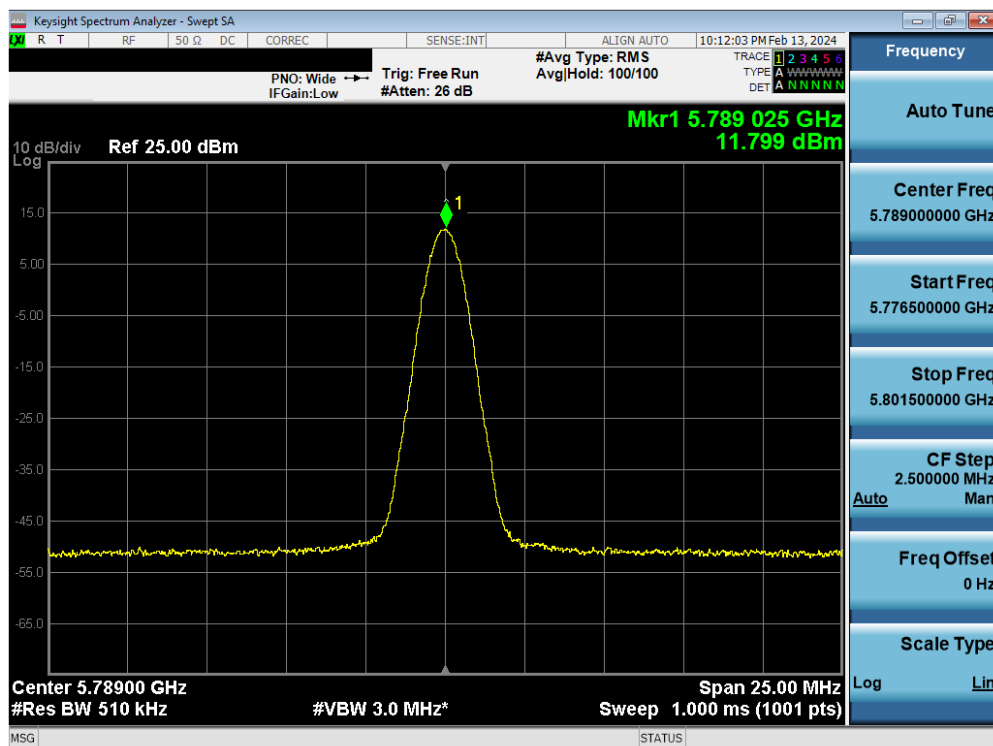
Plot 7-29. PSD Antenna 5b (BDR, ePA 5789MHz)
