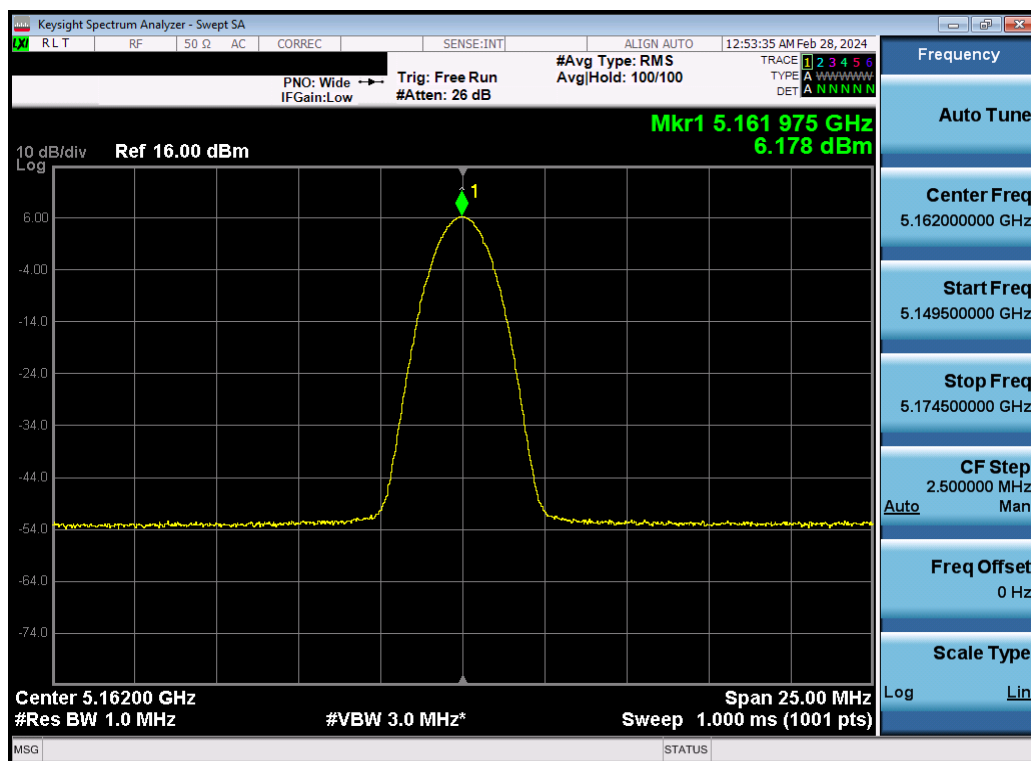
Plot 7-25. ISED PSD Antenna 5b (BDR, ePA – 5162MHz)
