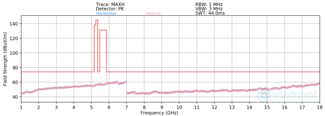
Plot 7-96. Radiated Spurious Emissions 1-18GHz Antenna 5b (BDR GFSK ePA- 5844MHz)
