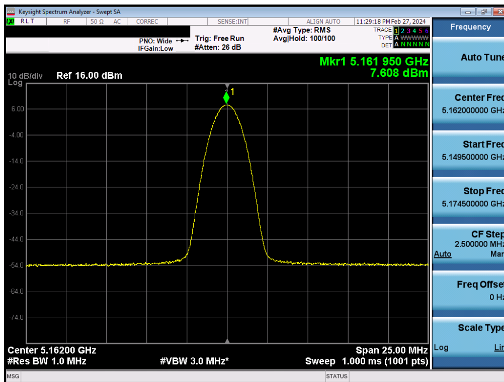
Plot 7-34. FCC PSD Antenna 4a (BDR, ePA – 5162MHz)
