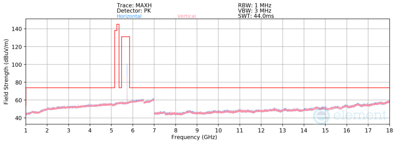
Plot 7-94. Radiated Spurious Emissions 1-18GHz Antenna 5b (BDR GFSK ePA – 5733MHz)
