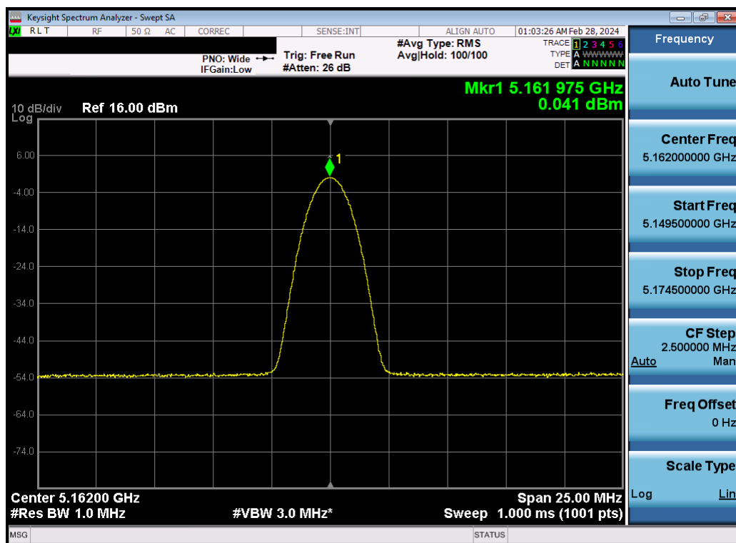
Plot 7-73. ISED PSD TxBF Antenna 5b (BDR, ePA – 5162MHz)
