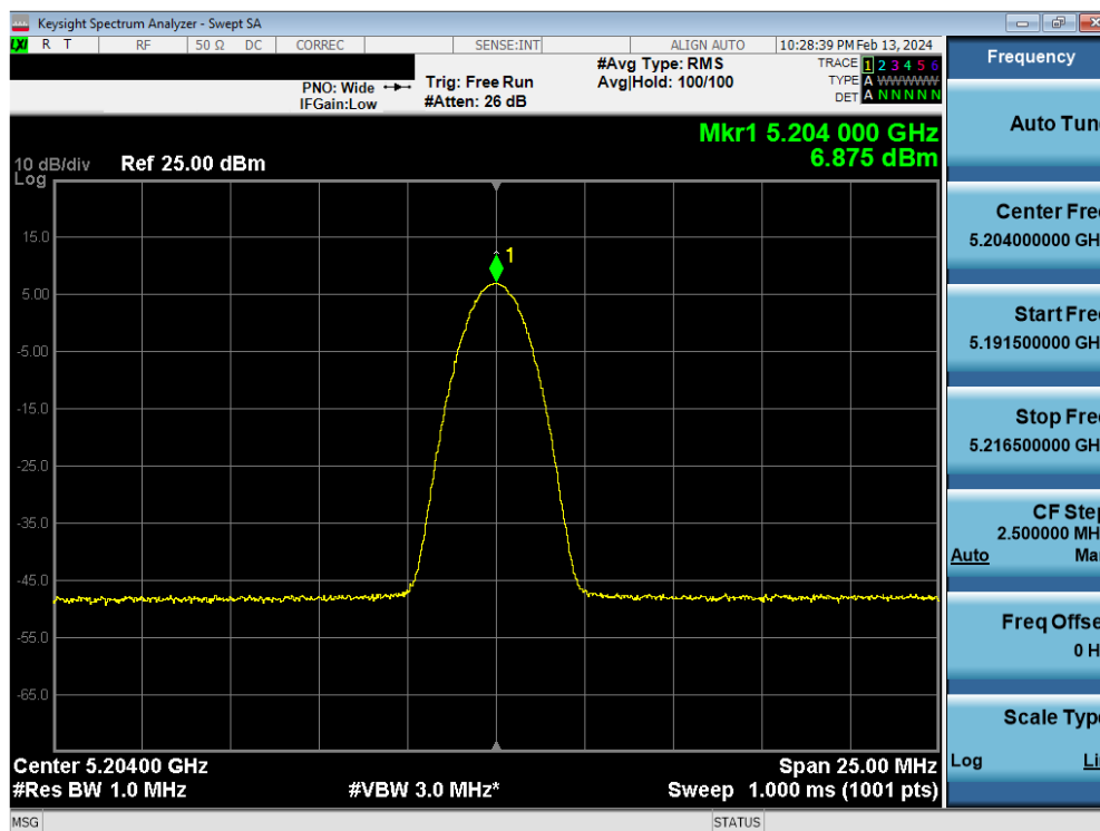
Plot 7-63. FCC PSD TxBF Antenna 5b (BDR, ePA – 5204MHz)
