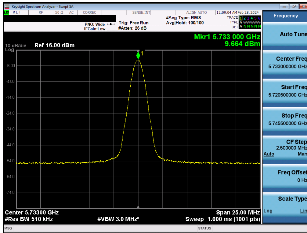
Plot 7-55. PSD Antenna 2a (BDR, ePA 5733MHz)
