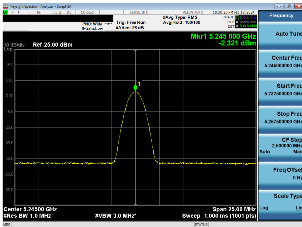
Plot 7-71. FCC/ISED PSD TxBF Antenna 5b (BDR, iPA- 5245MHz)
