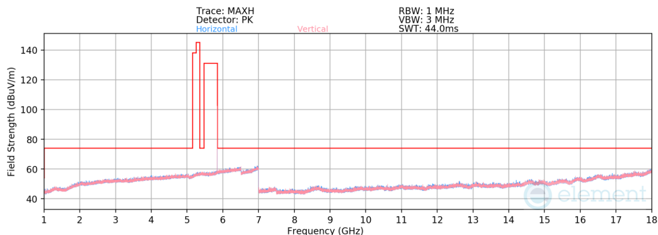
Plot 7-102. Radiated Spurious Emissions 1-18GHz Antenna 4a (BDR GFSK ePA – 5844MHz)
