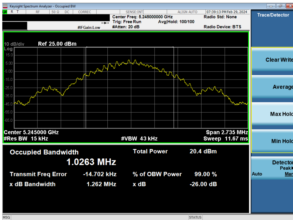
Plot 7-3. 26dB BW & 99% OBW Antenna 5b (BDR GFSK, ePA- 5245MHz)
