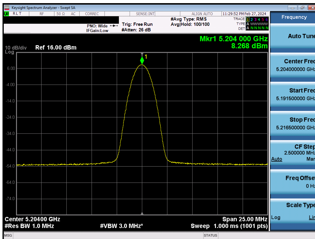
Plot 7-35. FCC PSD Antenna 4a (BDR, ePA – 5204MHz)
