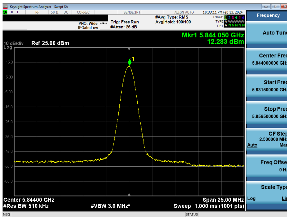
Plot 7-83. PSD TxBF Antenna 5b (BDR, ePA 5844MHz)
