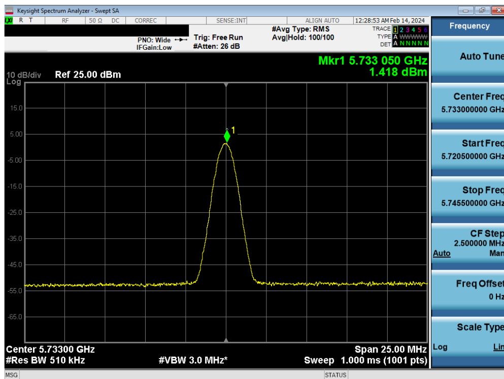
Plot 7-86. PSD TxBF Antenna 4a (BDR, iPA 5733MHz)
