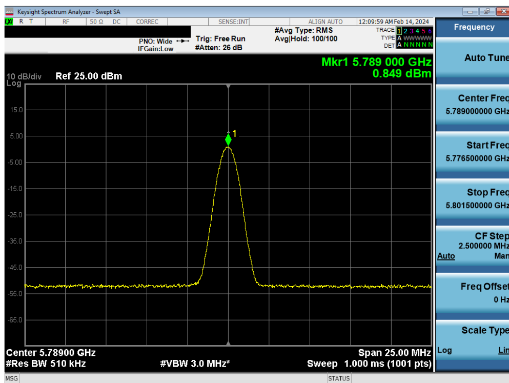
Plot 7-47. PSD Antenna 4a (BDR, iPA 5789MHz)
