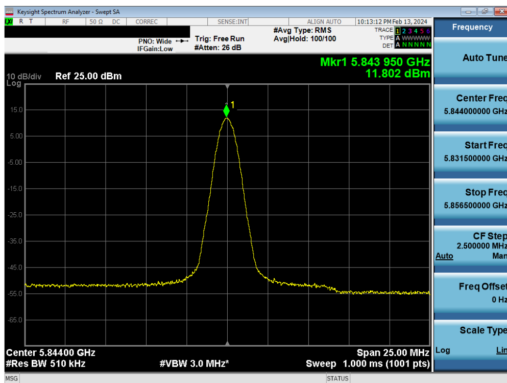
Plot 7-30. PSD Antenna 5b (BDR, ePA 5844MHz)
