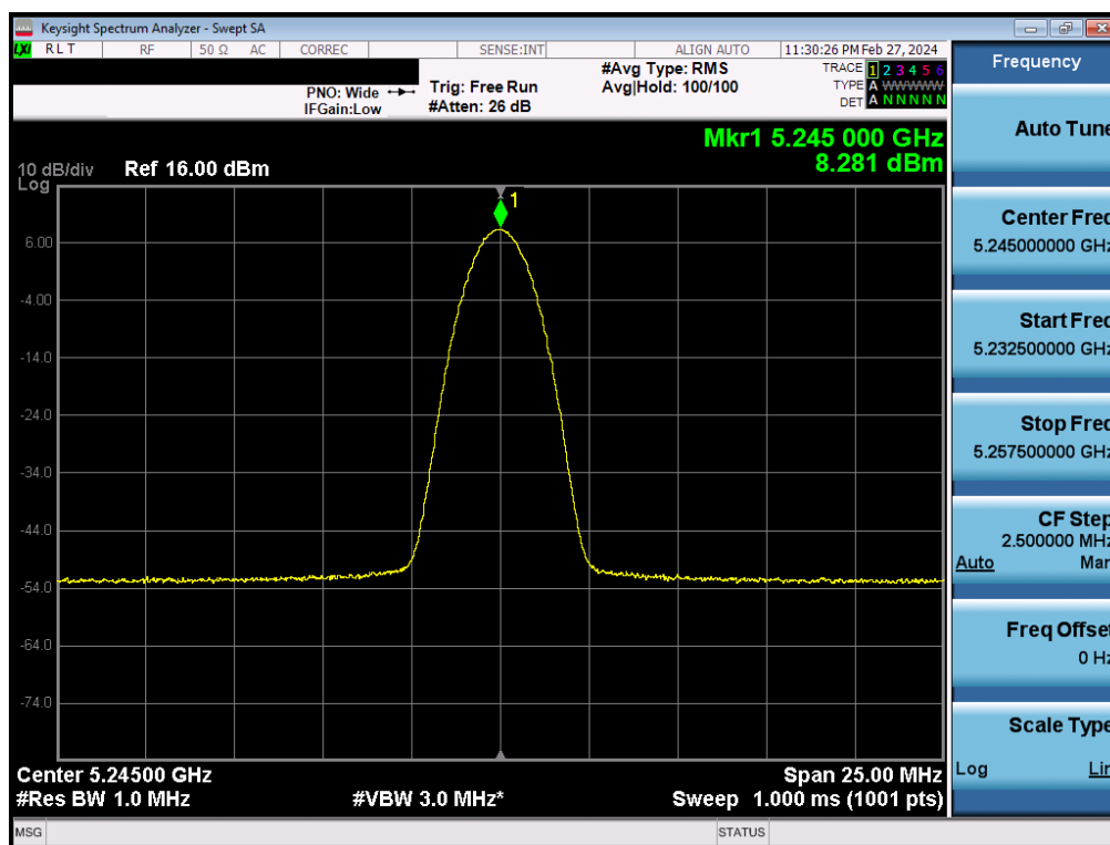
Plot 7-36. FCC PSD Antenna 4a (BDR, ePA– 5245MHz)
