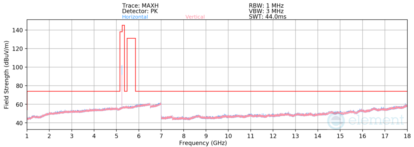
Plot 7-93. Radiated Spurious Emissions 1-18GHz Antenna 5b (BDR GFSK ePA - 5245MHz)
