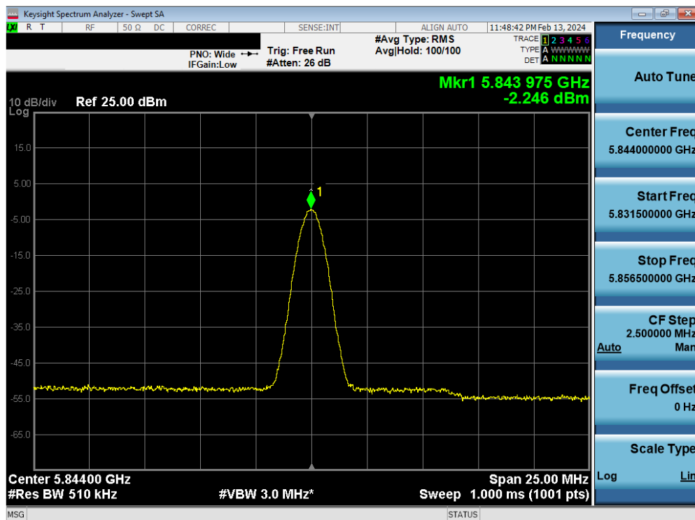
Plot 7-60. PSD Antenna 2a (BDR, iPA 5844MHz)
