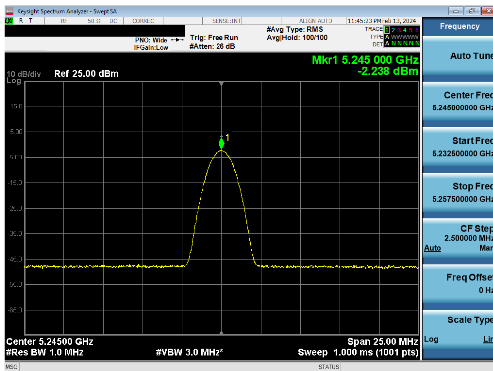
Plot 7-54. PSD Antenna 2a (BDR, iPA– 5245MHz)
