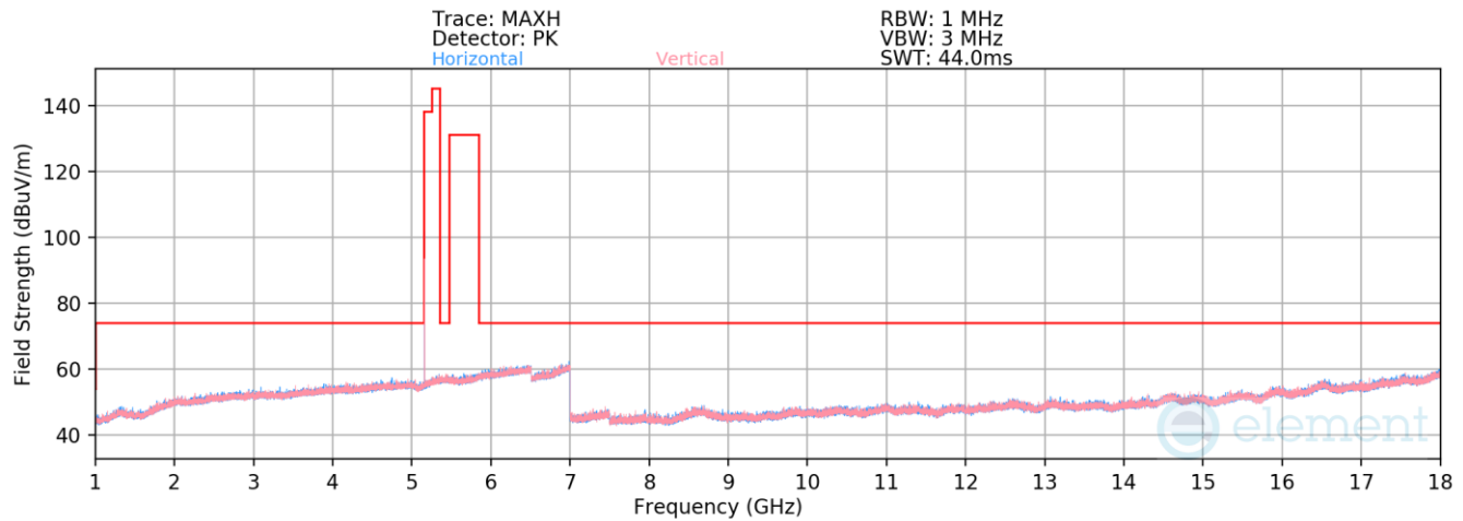
Plot 7-91. Radiated Spurious Emissions 1-18GHz Antenna 5b (BDR GFSK ePA – 5162MHz)
