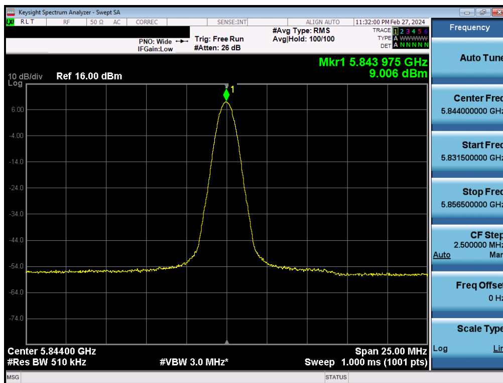
Plot 7-45. PSD Antenna 4a (BDR, ePA 5844MHz)
