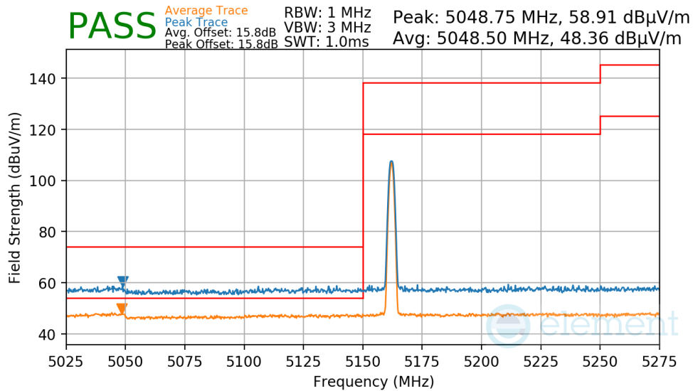
Plot 7-120. Radiated Lower Band Edge Measurement Antenna 4a
