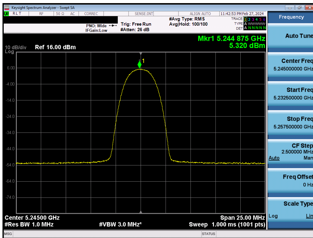
Plot 7-120. FCC PSD TxBF Antenna 4a (HDR4, ePA- 5245MHz)
