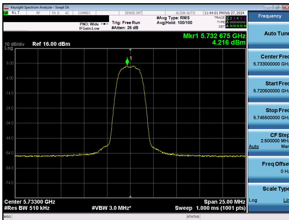
Plot 7-152. PSD TxBF Antenna 4a (HDR4, ePA 5733MHz)
