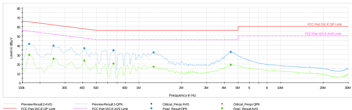
Plot 7-215. AC Line Conducted Plot TxBF (HDR4, ePA – 5245MHz) (L1) with AC/DC Adapter
