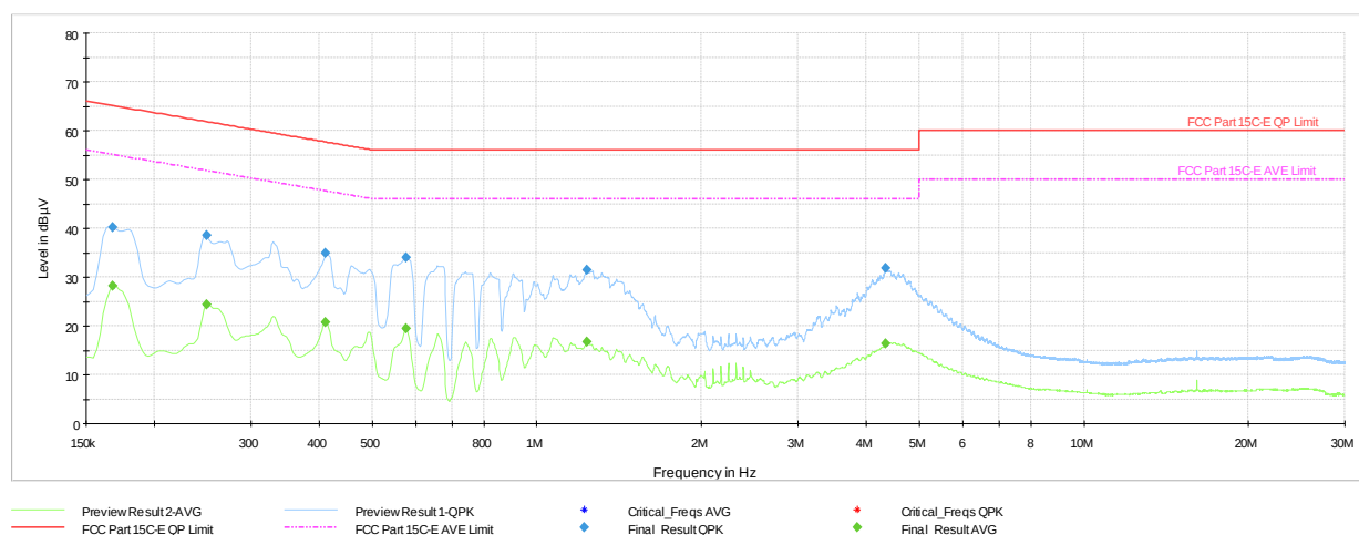
Plot 7-216. AC Line Conducted Plot TxBF (HDR4, ePA - 5245MHz) (N) with AC/DC Adapter
