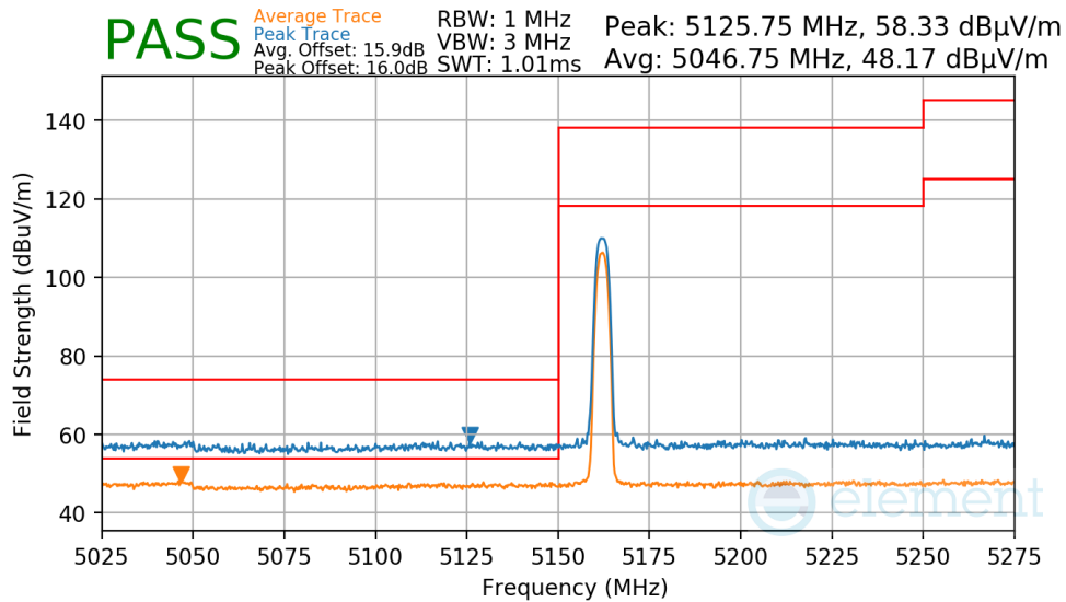
Plot 7-210. Radiated Lower Band Edge Measurement TxBF
