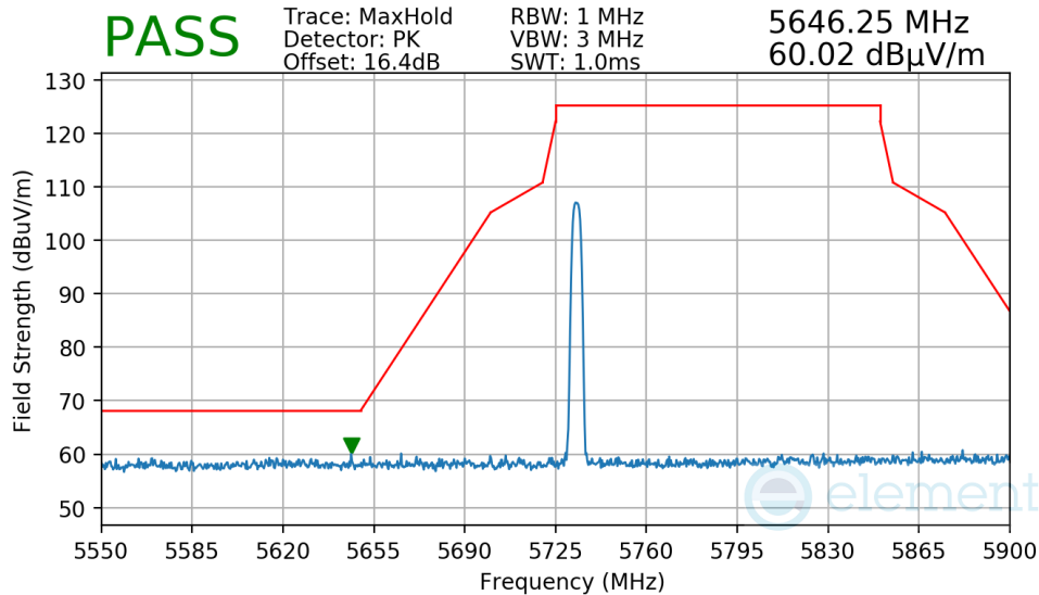
Plot 7-208. Radiated Lower Band Edge Measurement Antenna 2a
