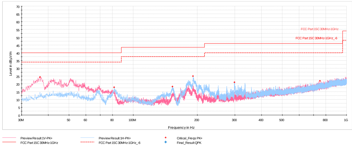
Plot 7-214. Radiated Spurious Emissions Below 1GHz TxBF (HDR4, ePA – 5844MHz), with AC/DC Adapter
