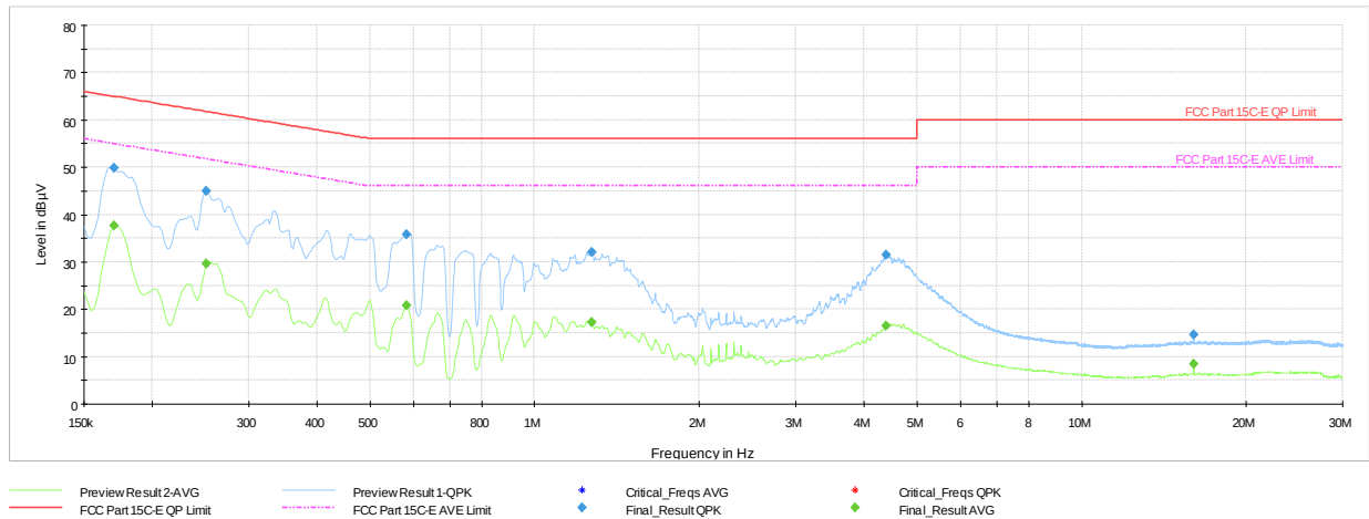
Plot 7-218. AC Line Conducted Plot TxBF (HDR4, ePA – 5844MHz) (N) with AC/DC Adapter
