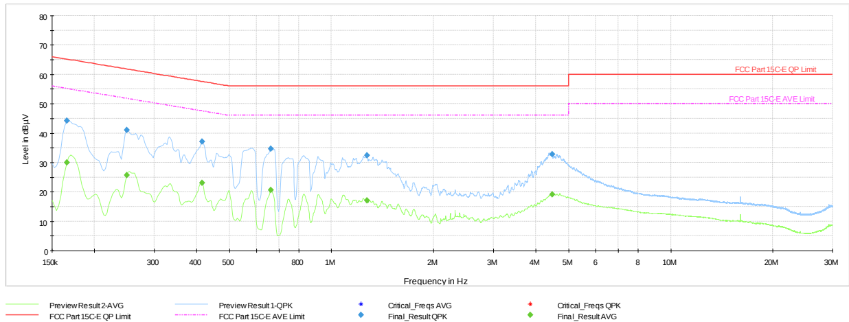
Plot 7-217. AC Line Conducted Plot TxBF (HDR4, ePA – 5844MHz) (L1) with AC/DC Adapter
