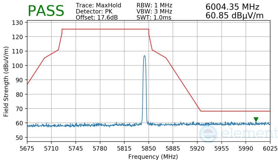
Plot 7-209. Radiated Upper Band Edge Measurement Antenna 2a
