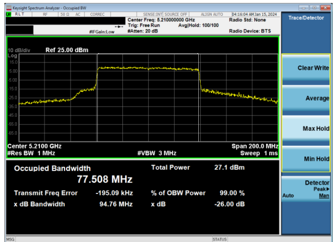
Plot 7-28. 26dB BW & 99% OBW Antenna WF5b (80MHz BW 802.11ax(SU) – Ch. 42, MCS4)
