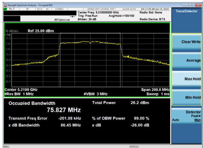
Plot 7-27. 26dB BW & 99% OBW Antenna WF5b (80MHz BW 802.11ac – Ch. 42, MCS4)
