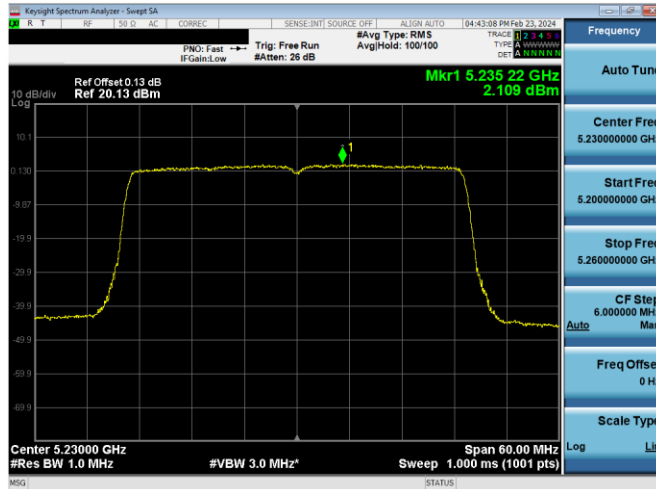
Plot 7-750. ISED SDM Primary PSD Antenna 4a (40MHz BW 11ax(SU) – Ch.46, MCS2)
