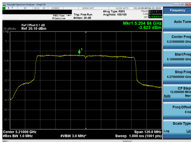
Plot 7-784. PSD CDD Diversity Antenna 2a (80MHz BW 802.11ax(SU) – Ch. 42, MCS2)
