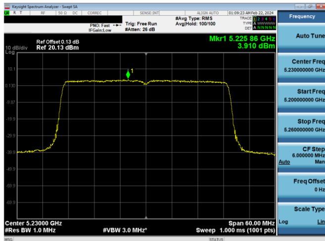
Plot 7-782. PSD CDD Diversity Antenna 2a (40MHz BW 802.11ax(SU) – Ch. 46, MCS2)
