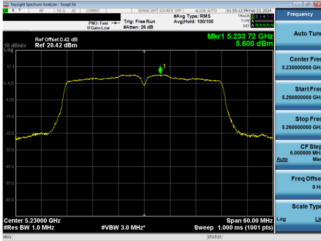
Plot 7-803. PSD CDD Diversity Antenna 2a (40MHz BW 802.11n – Ch. 46, MCS12)
