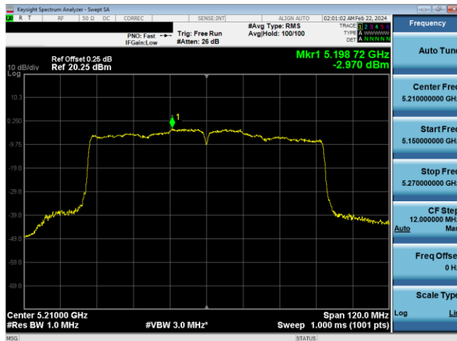
Plot 7-805. PSD CDD Diversity Antenna 2a (80MHz BW 802.11ac – Ch. 42, MCS4)
