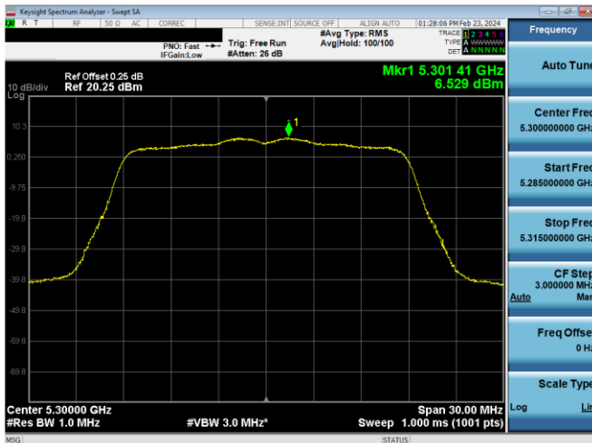
Plot 7-787. PSD CDD Diversity Antenna 2a (20MHz BW 802.11n – Ch. 60, MCS10)
