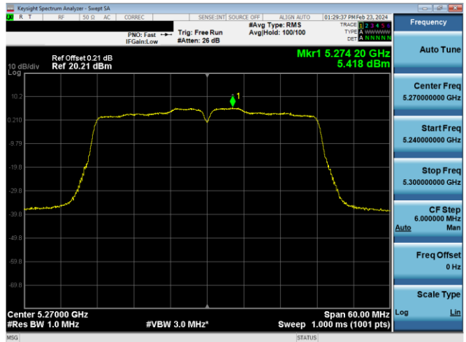
Plot 7-789. PSD CDD Diversity Antenna 2a (40MHz BW 802.11n – Ch. 54, MCS10)
