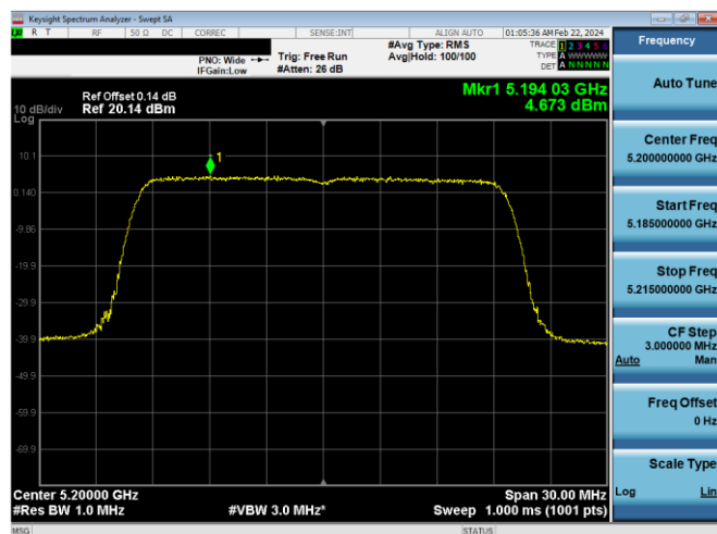
Plot 7-780. PSD CDD Diversity Antenna 2a (20MHz BW 802.11ax(SU) – Ch. 40, MCS2)
