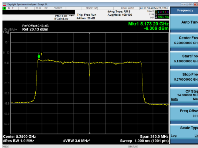
Plot 7-786. PSD CDD Diversity Antenna 2a (160MHz BW 802.11ax(SU) – Ch. 50, MCS2)
