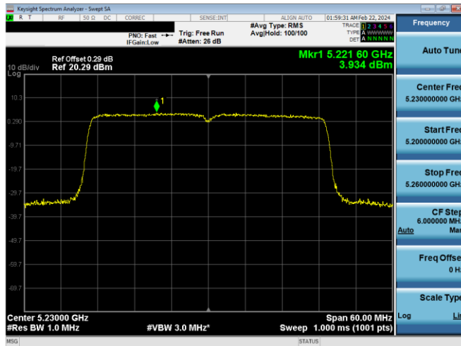
Plot 7-804. PSD CDD Diversity Antenna 2a (40MHz BW 802.11ax(SU) – Ch. 46, MCS4)
