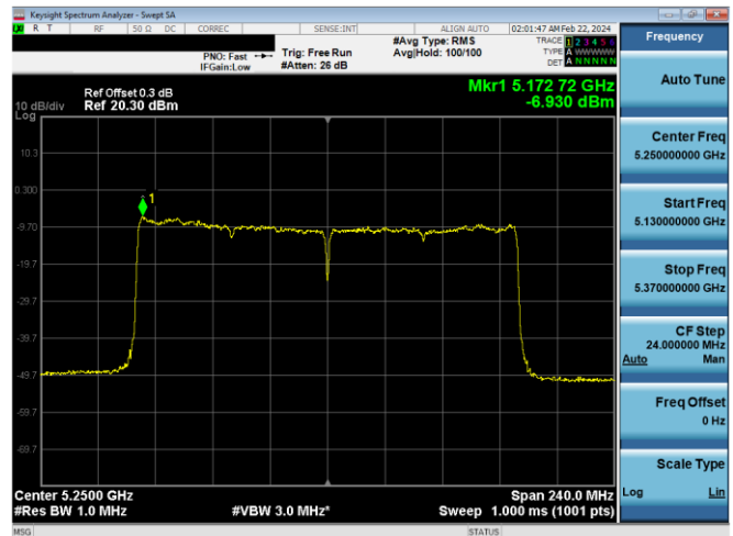
Plot 7-808. PSD CDD Diversity Antenna 2a (160MHz BW 802.11ax(SU) – Ch. 50, MCS4)
