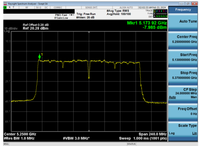
Plot 7-807. PSD CDD Diversity Antenna 2a (160MHz BW 802.11ac – Ch. 50, MCS4)
