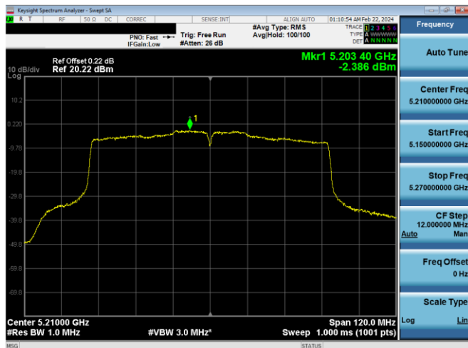
Plot 7-783. PSD CDD Diversity Antenna 2a (80MHz BW 802.11ac – Ch. 42, MCS2)
