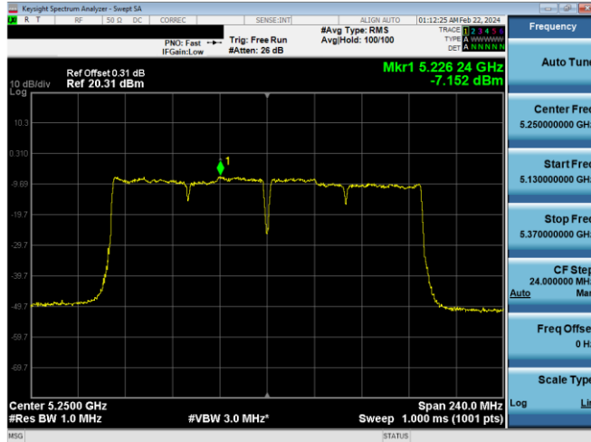
Plot 7-785. PSD CDD Diversity Antenna 2a (160MHz BW 802.11ac – Ch. 50, MCS2)
