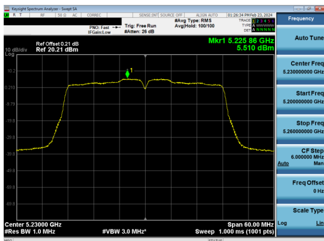
Plot 7-781. PSD CDD Diversity Antenna 2a (40MHz BW 802.11n – Ch. 46, MCS10)
