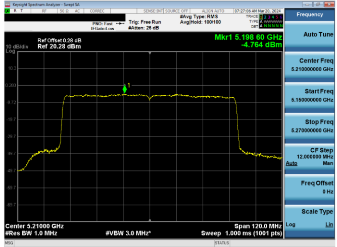
Plot 7-806. PSD CDD Diversity Antenna 2a (80MHz BW 802.11ax(SU) – Ch. 42, MCS4)
