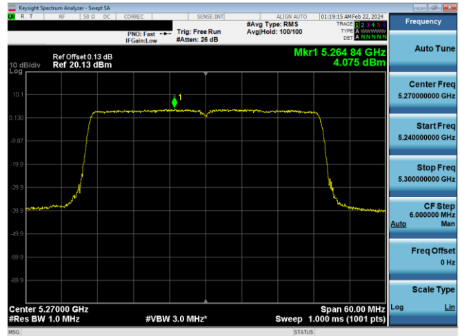
Plot 7-790. PSD CDD Diversity Antenna 2a (40MHz BW 802.11ax(SU) – Ch. 54, MCS2)
