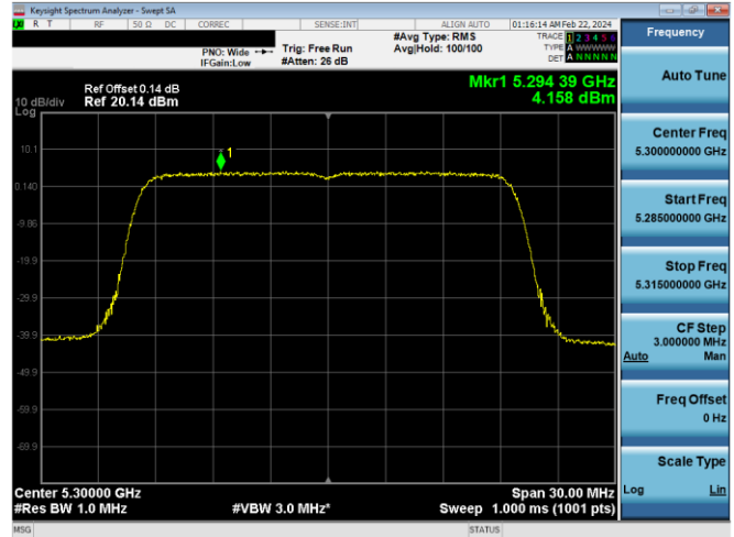
Plot 7-788. PSD CDD Diversity Antenna 2a (20MHz BW 802.11ax(SU) – Ch. 60, MCS2)
