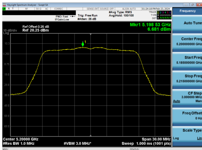
Plot 7-779. PSD CDD Diversity Antenna 2a (20MHz BW 802.11n – Ch. 40, MCS10)
