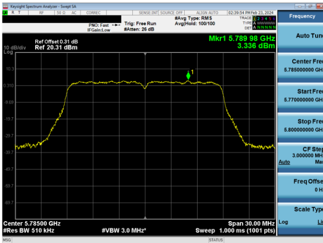
Plot 7-870. PSD CDD Diversity Antenna 2a (20MHz BW 802.11n – Ch. 157, MCS15)
