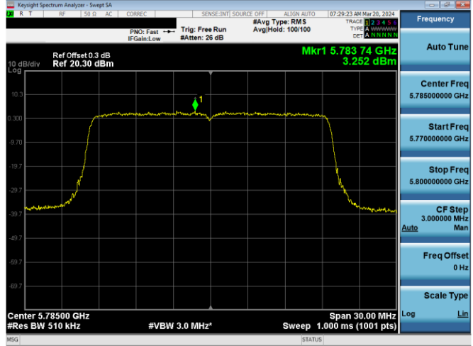
Plot 7-860. PSD CDD Diversity Antenna 2a (20MHz BW 802.11ax(SU) – Ch. 157, MCS4)
