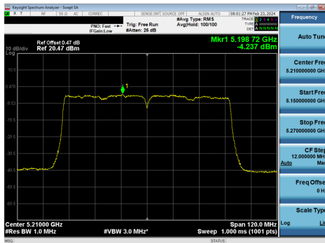
Plot 7-901. ISPD PSD CDD Diversity Antenna 2a (80MHz BW 11ac - Ch.42, MCS9)
