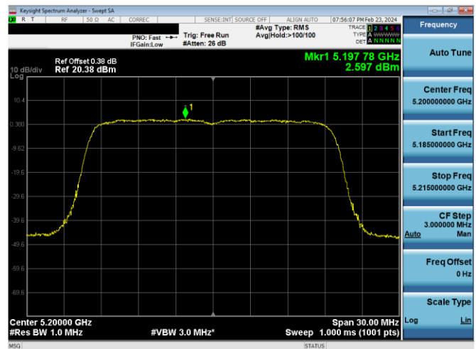
Plot 7-898. ISED PSD CDD Diversity Antenna 2a (20MHz BW 11ac(SU) – Ch.40, MCS11)
