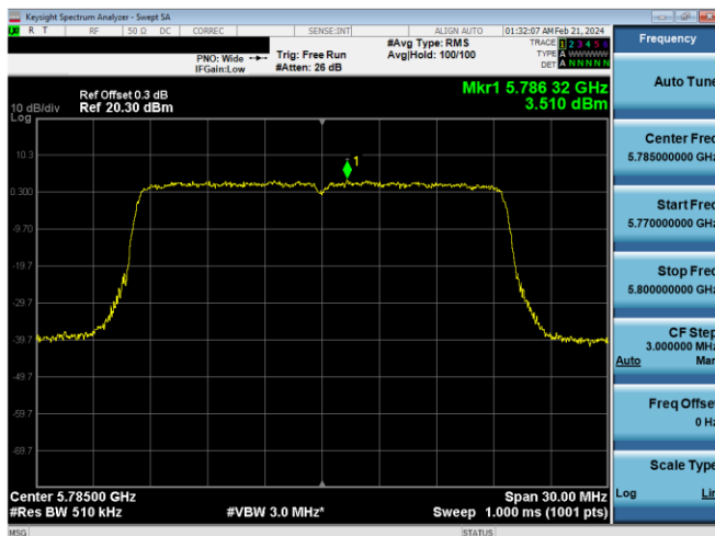
Plot 7-859. PSD CDD Diversity Antenna WF5b (20MHz BW 802.11ax(SU) – Ch. 157, MCS4)
