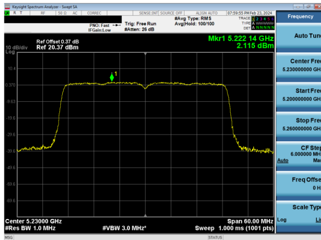
Plot 7-900. ISPD PSD SDM Diversity Antenna 2a (40MHz BW 11ax(SU) - Ch.46, MCS11)
