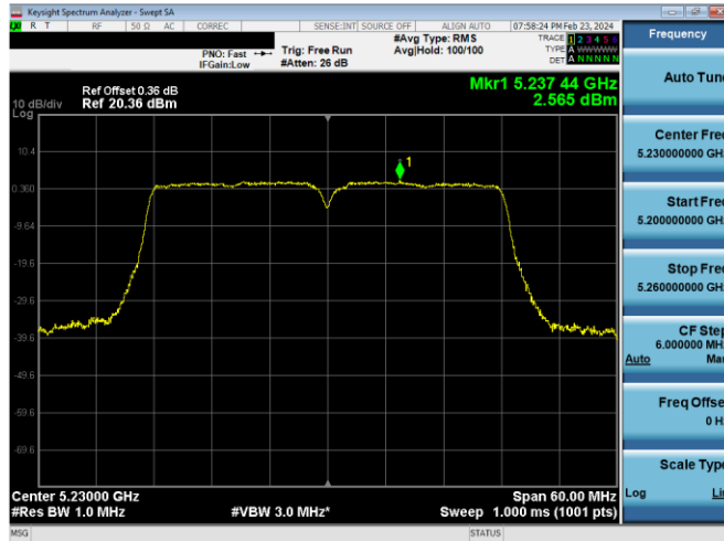
Plot 7-899. ISPD PSD SDM Diversity Antenna 2a (40MHz BW 11n - Ch.46, MCS15)
