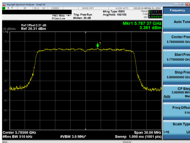
Plot 7-871. PSD CDD Diversity Antenna WF5b (20MHz BW 802.11ax(SU) – Ch. 157, MCS11)
