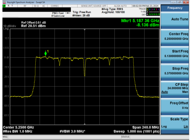
Plot 7-903. ISPD PSD CDD Diversity Antenna 2a (160MHz BW 11ac - Ch.50, MCS9)
