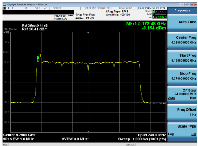
Plot 7-904. ISPD PSD CDD Diversity Antenna 2a (160MHz BW 11ax (SU) - Ch.50, MCS11)
