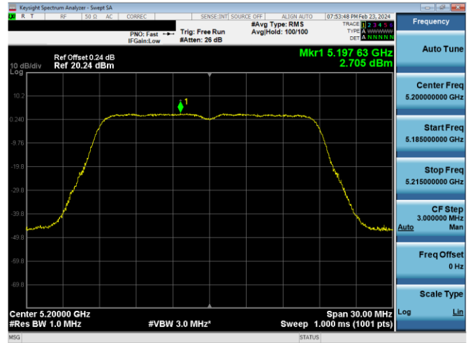
Plot 7-897. ISED PSD CDD Diversity Antenna 2a (20MHz BW 11n – Ch.40, MCS15)
