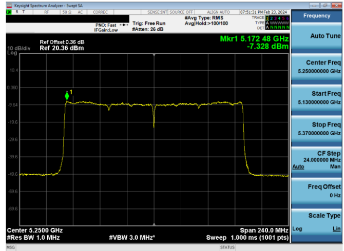
Plot 7-896. ISED CDD Diversity Antenna 2a (160MHz BW 11ac (SU) – Ch.50, MCS4)
