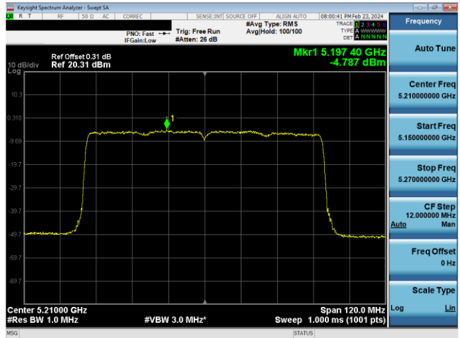
Plot 7-902. ISPD PSD CDD Diversity Antenna 2a (80MHz BW 11ax (SU) - Ch.42, MCS11)
