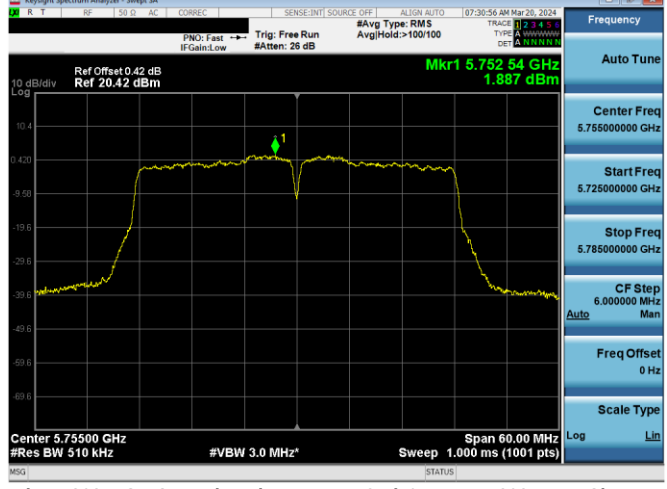
Plot 7-862. PSD CDD Diversity Antenna 2a (40MHz BW 802.11n – Ch. 151, MCS12)
