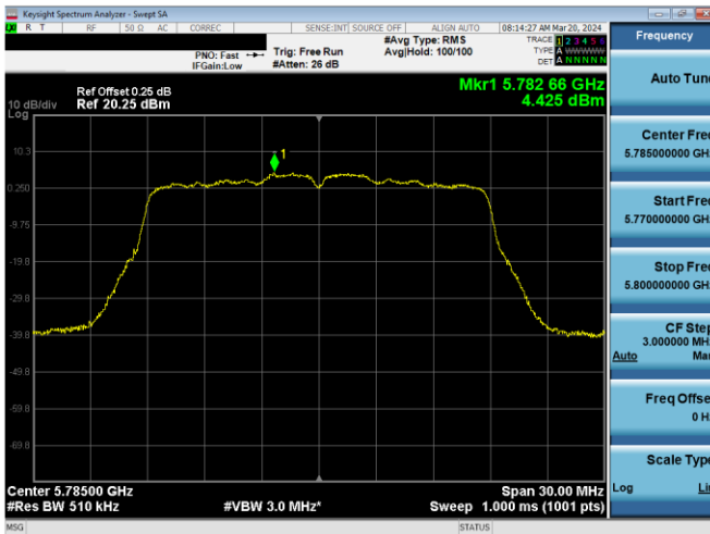
Plot 7-858. PSD CDD Diversity Antenna 2a (20MHz BW 802.11n – Ch. 157, MCS12)
