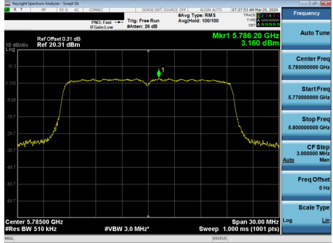
Plot 7-872. PSD CDD Diversity Antenna 2a (20MHz BW 802.11ax(SU) – Ch. 157, MCS11)
