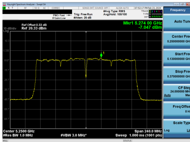
Plot 7-895. ISED PSD CDD Diversity Antenna 2a (160MHz BW 11ac – Ch.50, MCS4)
