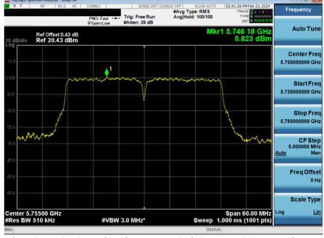
Plot 7-874. PSD CDD Diversity Antenna 2a (40MHz BW 802.11n – Ch. 151, MCS15)
