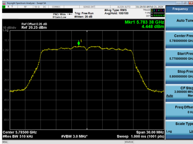
Plot 7-857. PSD CDD Diversity Antenna WF5b (20MHz BW 802.11n – Ch. 157, MCS12)
