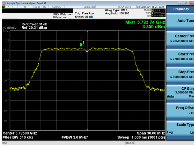
Plot 7-869. PSD CDD Diversity Antenna WF5b (20MHz BW 802.11n – Ch. 157, MCS15)
