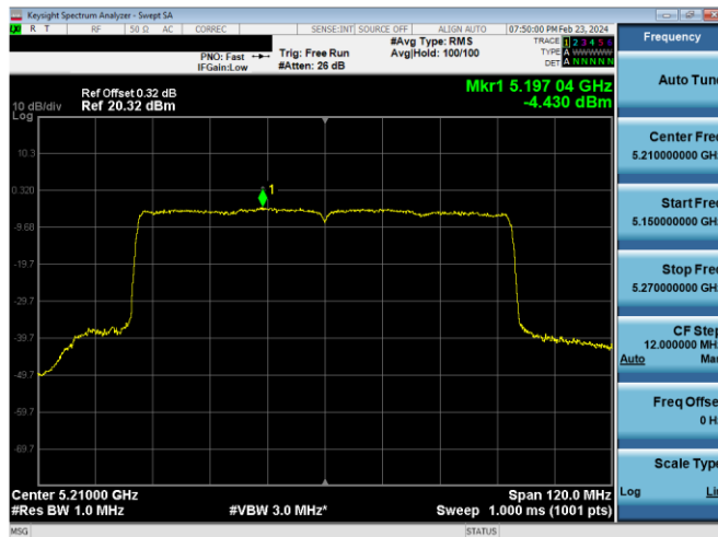
Plot 7-894. ISED PSD CDD Diversity Antenna 2a (80MHz BW 11ac (SU) – Ch.42, MCS4)
