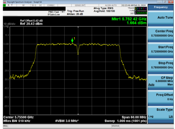
Plot 7-873. PSD CDD Diversity Antenna WF5b (40MHz BW 802.11n – Ch. 151, MCS15)
