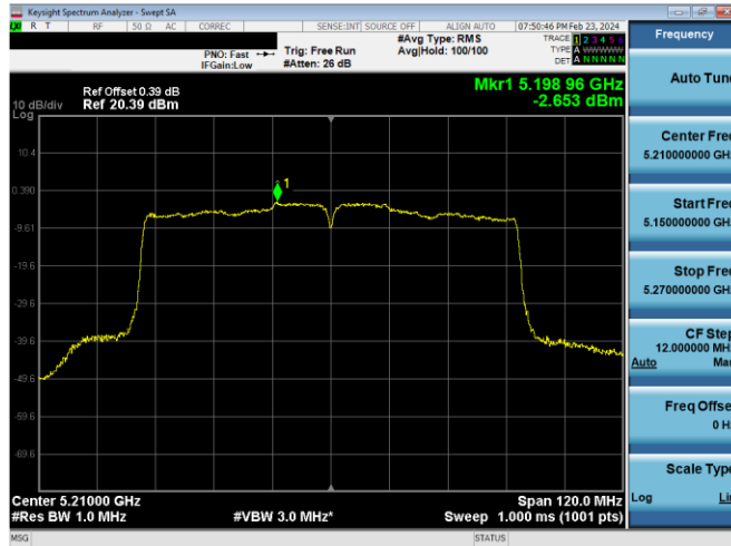
Plot 7-893. ISED PSD CDD Diversity Antenna 2a (80MHz BW 11ac – Ch.42, MCS4)
