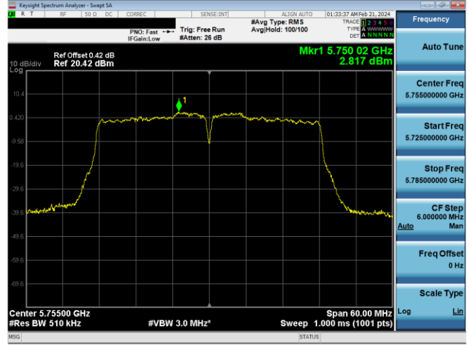
Plot 7-861. PSD CDD Diversity Antenna WF5b (40MHz BW 802.11n – Ch. 151, MCS12)
