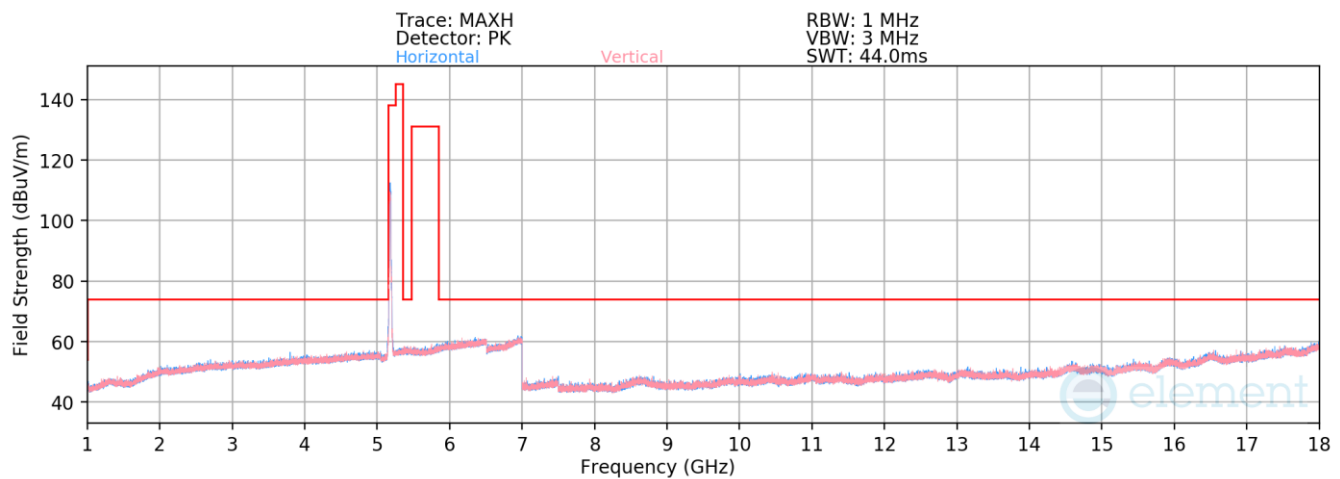
Plot 7-929. Radiated Spurious Emissions above 1GHz Antenna 4a (802.11n – Ch. 36)
