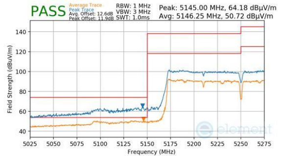
Plot 7-1209. ANTENNA WF5B (PEAK & AVERAGE, CH.50, 802.11AC, MCS9)
