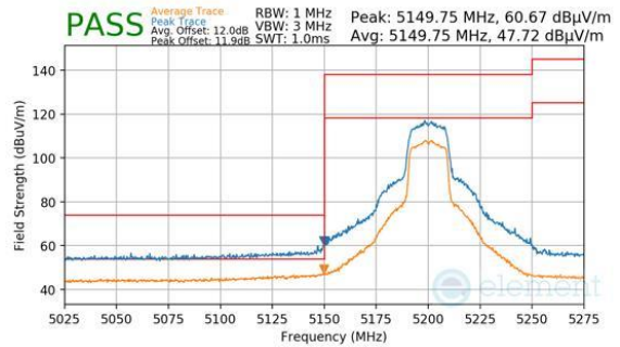
Plot 7-1046. ANTENNA WF5B (PEAK & AVERAGE, CH.40, 802.11N, MCS2)
