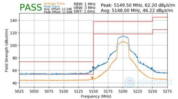
Plot 7-1233. ANTENNA 4A (PEAK & AVERAGE, CH.40, 802.11N, MCS4)
