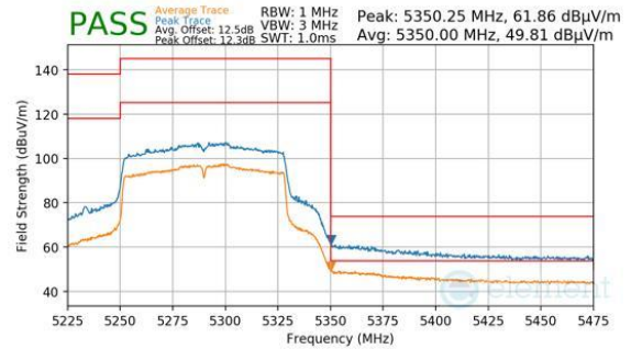
Plot 7-1166. ANTENNA WF5B (PEAK & AVERAGE, CH.58, 802.11AC, MCS2)
