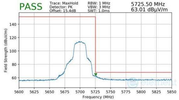
Plot 7-1064. ANTENNA WF5B (PEAK, CH.140, 802.11N, MCS2)
