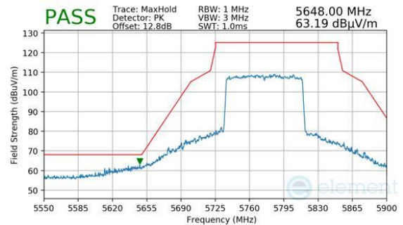
Plot 7-1203. ANTENNA WF5B (PEAK, CH.155, 802.11AX(SU), MCS11)
