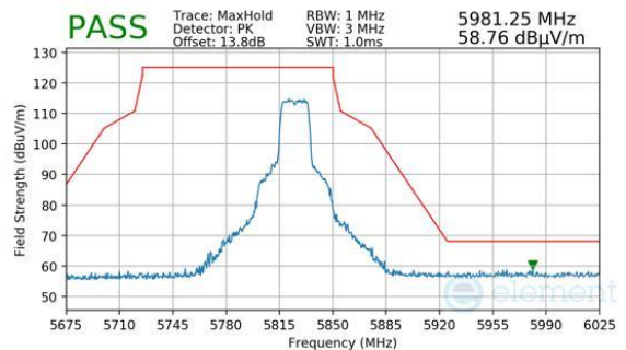
Plot 7-1072. ANTENNA WF5B (PEAK, CH.165, 802.11N, MCS7)
