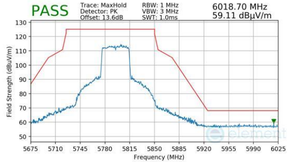
Plot 7-1161. ANTENNA WF5B (PEAK, CH.159, 802.11AX(SU), MCS4)
