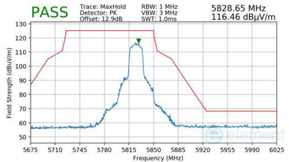
Plot 7-1071. ANTENNA WF5B (PEAK, CH.165, 802.11N, MCS4)
