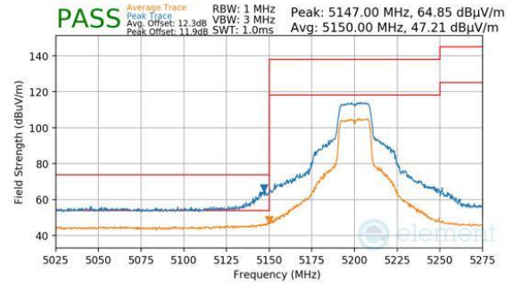
Plot 7-1234. ANTENNA 4A (PEAK & AVERAGE, CH.40, 802.11N, MCS7)
