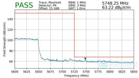
Plot 7-1226. ANTENNA WF5B (PEAK, CH.114, 802.11AX(SU), MCS4)
