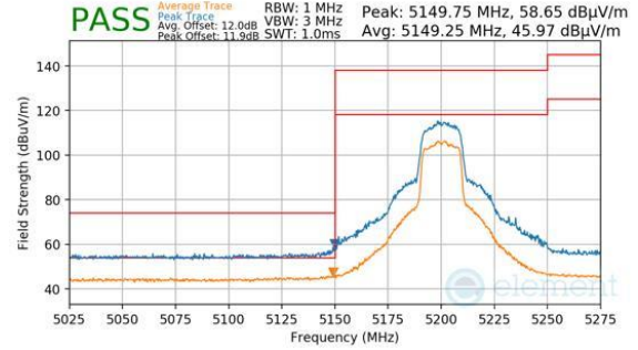
Plot 7-1232. ANTENNA 4A (PEAK & AVERAGE, CH.40, 802.11N, MCS2)
