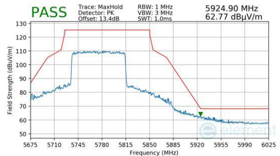
Plot 7-1204. ANTENNA WF5B (PEAK, CH.155, 802.11AX(SU), MCS11)
