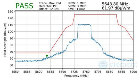
Plot 7-1341. ANTENNA 4A (PEAK, CH.151, 802.11AX(SU), MCS11)
