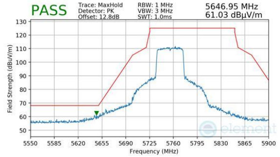
Plot 7-1340. ANTENNA 4A (PEAK, CH.151, 802.11AX(SU), MCS4)
