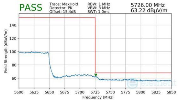
Plot 7-1410. ANTENNA 4A (PEAK, CH.114, 802.11AX(SU), MCS11)
