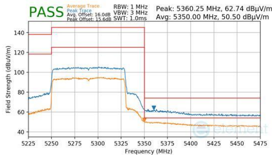
Plot 7-1370. ANTENNA 4A (PEAK & AVERAGE, CH.58, 802.11AX(SU), MCS4)
