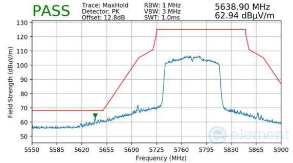
Plot 7-1360. ANTENNA 4A (PEAK, CH.155, 802.11AC, MCS2)
