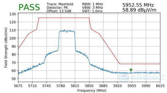
Plot 7-1342. ANTENNA 4A (PEAK, CH.159, 802.11AX(SU), MCS2)
