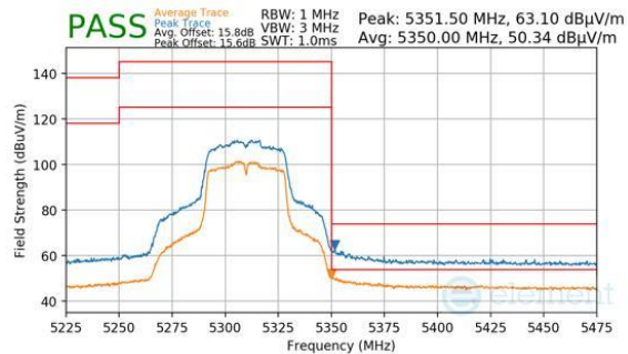
Plot 7-1298. ANTENNA 4A (PEAK & AVERAGE, CH.62, 802.11N, MCS2)
