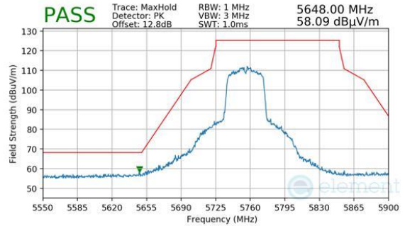
Plot 7-1310. ANTENNA 4A (PEAK, CH.151, 802.11N, MCS2)
