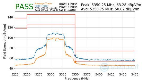
Plot 7-1299. ANTENNA 4A (PEAK & AVERAGE, CH.62, 802.11N, MCS4)
