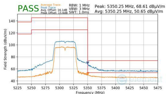
Plot 7-1300. ANTENNA 4A (PEAK & AVERAGE, CH.62, 802.11N, MCS7)
