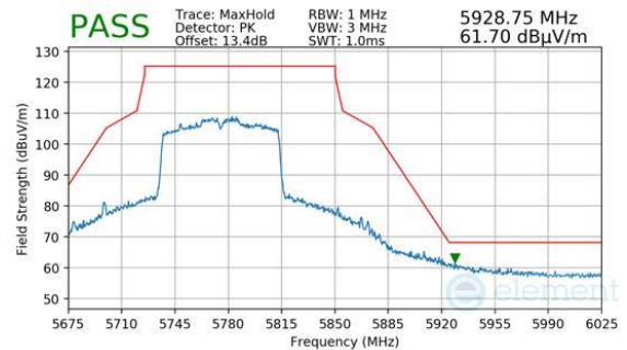
Plot 7-1361. ANTENNA 4A (PEAK, CH.155, 802.11AC, MCS2)
