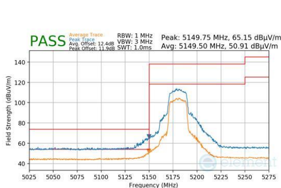
Plot 7-1789. CDD DIVERSITY DIVERSITY (PEAK & AVERAGE, CH.36, 802.11N, MCS12)
