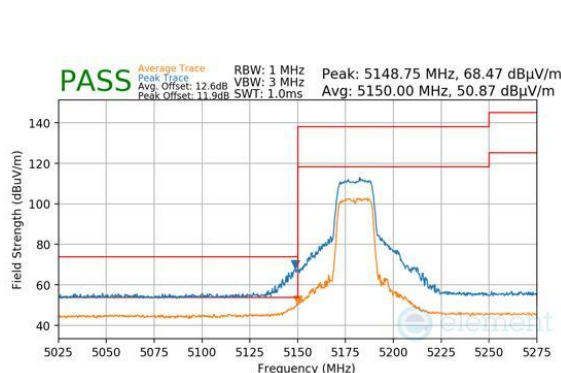
Plot 7-1790. CDD DIVERSITY DIVERSITY (PEAK & AVERAGE, CH.36, 802.11N, MCS15)
