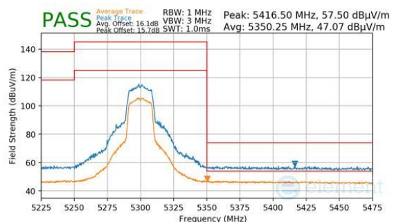
Plot 7-1793. CDD DIVERSITY DIVERSITY (PEAK & AVERAGE, CH.60, 802.11N, MCS12)
