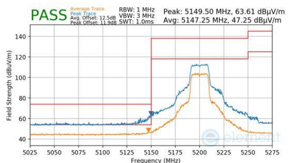
Plot 7-1792. CDD DIVERSITY DIVERSITY (PEAK & AVERAGE, CH.40, 802.11N, MCS15)
