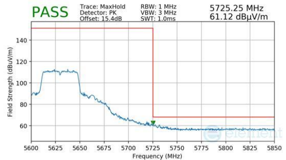
Plot 7-1864. CDD DIVERSITY DIVERSITY (PEAK, CH.126, 802.11N, MCS15)
