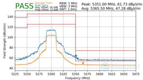
Plot 7-1821. CDD DIVERSITY DIVERSITY (PEAK & AVERAGE, CH.60, 802.11AX(SU), MCS11)
