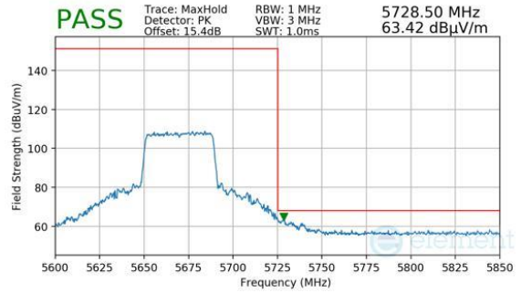
Plot 7-1899. CDD DIVERSITY DIVERSITY (PEAK, CH.134, 802.11AX(SU), MCS11)
