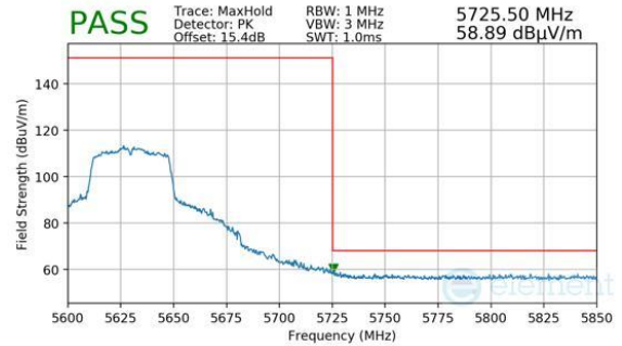
Plot 7-1863. CDD DIVERSITY DIVERSITY (PEAK, CH.126, 802.11N, MCS12)
