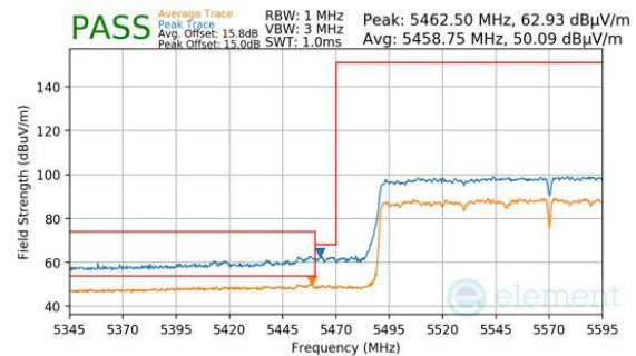
Plot 7-1970. CDD DIVERSITY DIVERSITY (PEAK & AVERAGE, CH.114, 802.11AX(SU), MCS11)
