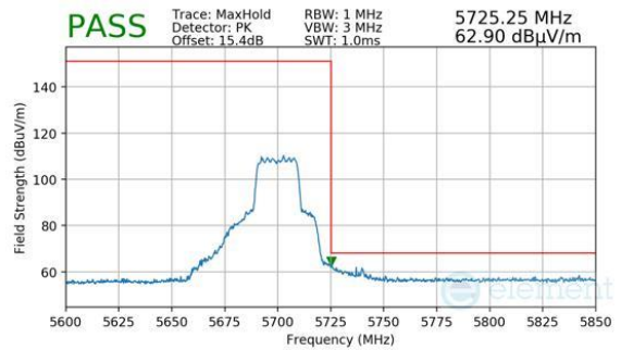
Plot 7-1834. CDD DIVERSITY DIVERSITY (PEAK, CH.140, 802.11AX(SU), MCS4)
