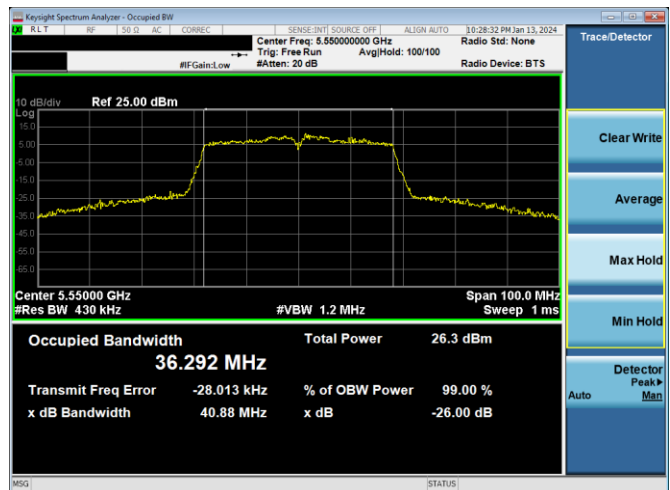
Plot 7-170. 26dB BW & 99% OBW Antenna 2a (40MHz BW 802.11n – Ch. 110, MCS4)
