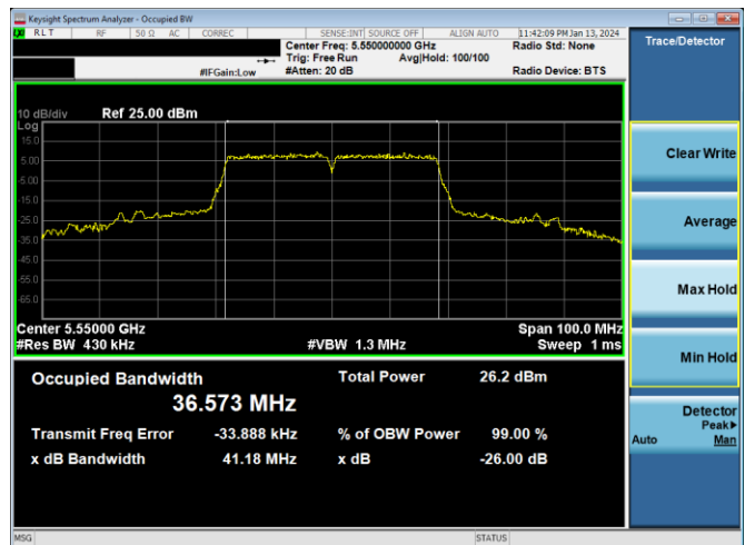
Plot 7-192. 26dB BW & 99% OBW Antenna 2a (40MHz BW 802.11n – Ch. 110) , MCS7)
