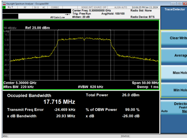
Plot 7-162. 26dB BW & 99% OBW Antenna 2a (20MHz BW 802.11n – Ch. 60, MCS4)
