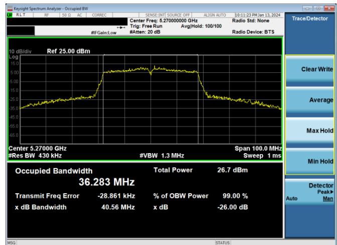
Plot 7-164. 26dB BW & 99% OBW Antenna 2a (40MHz BW 802.11n – Ch. 54, MCS4)
