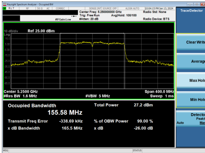
Plot 7-160. 26dB BW & 99% OBW Antenna 2a (160MHz BW 802.11ac – Ch. 50, MCS4)
