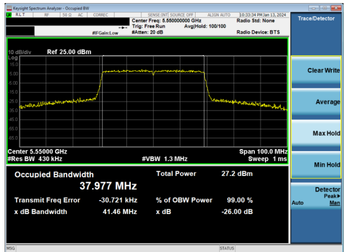
Plot 7-171. 26dB BW & 99% OBW Antenna 2a (40MHz BW 802.11ax(SU) – Ch. 110, MCS4)
