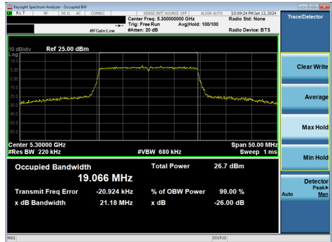
Plot 7-163. 26dB BW & 99% OBW Antenna 2a (20MHz BW 802.11ax(SU) – Ch. 60, MCS4)
