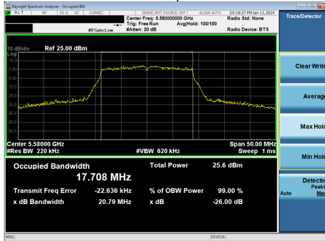
Plot 7-168. 26dB BW & 99% OBW Antenna 2a (20MHz BW 802.11n – Ch. 116, MCS4)
