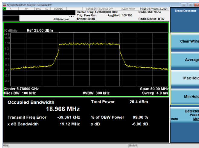
Plot 7-223. 6dB BW & 99% OBW Antenna 4a (20MHz BW 802.11ax(SU) – Ch. 157, MCS4)
