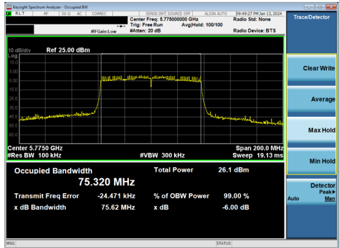
Plot 7-238. 6dB BW & 99% OBW Antenna 2a (80MHz BW 802.11ac – Ch. 155, MCS2)
