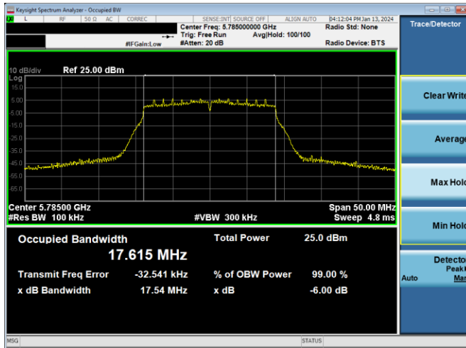
Plot 7-216. 6dB BW & 99% OBW Antenna 4a (20MHz BW 802.11n – Ch. 157, MCS2)
