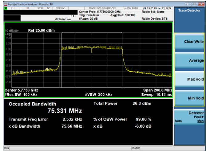
Plot 7-220. 6dB BW & 99% OBW Antenna 4a (80MHz BW 802.11ac – Ch. 155, MCS2)
