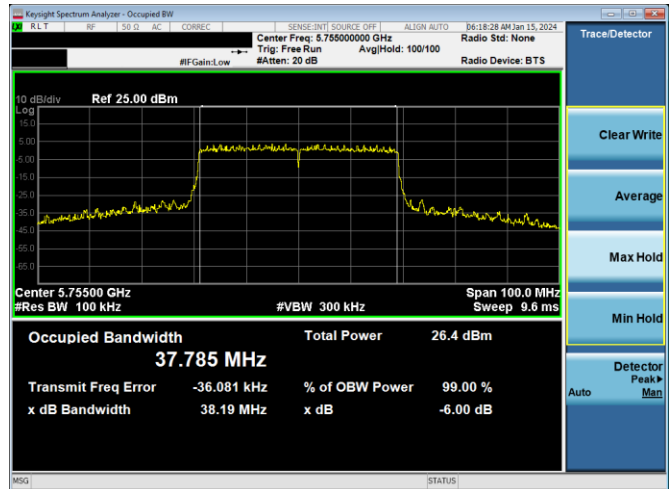
Plot 7-213. 6dB BW & 99% OBW Antenna WF5b (40MHz BW 802.11ax(SU) – Ch. 151, MCS11)
