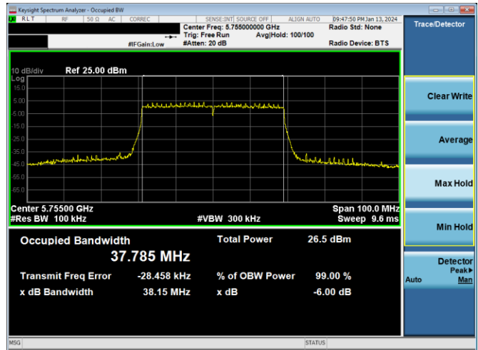
Plot 7-237. 6dB BW & 99% OBW Antenna 2a (40MHz BW 802.11ax(SU) – Ch. 151, MCS2)
