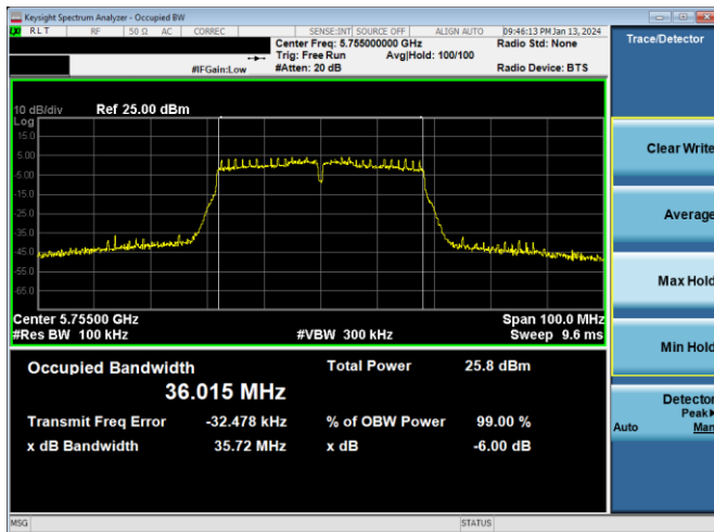
Plot 7-236. 6dB BW & 99% OBW Antenna 2a (40MHz BW 802.11n – Ch. 151, MCS2)
