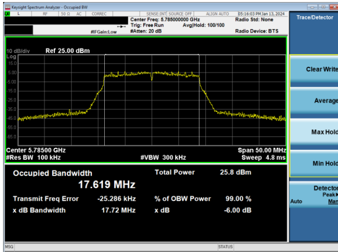
Plot 7-222. 6dB BW & 99% OBW Antenna 4a (20MHz BW 802.11n – Ch. 157, MCS4)
