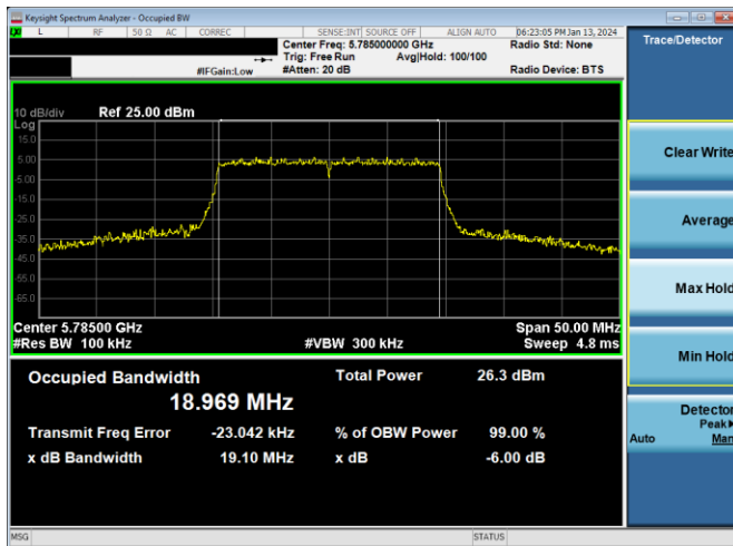
Plot 7-229. 6dB BW & 99% OBW Antenna 4a (20MHz BW 802.11ax(SU) – Ch. 157, MCS11)
