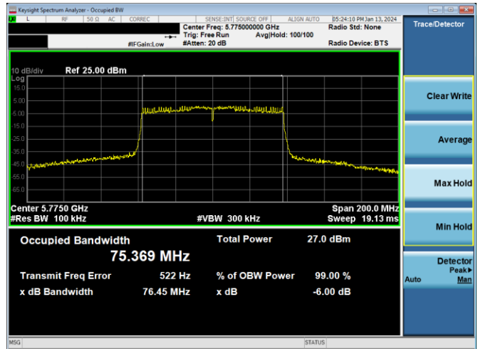
Plot 7-226. 6dB BW & 99% OBW Antenna 4a (80MHz BW 802.11ac – Ch. 155, MCS4)
