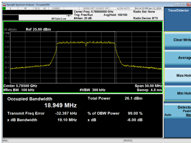
Plot 7-217. 6dB BW & 99% OBW Antenna 4a (20MHz BW 802.11ax(SU) – Ch. 157, MCS2)
