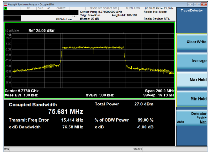
Plot 7-232. 6dB BW & 99% OBW Antenna 4a (80MHz BW 802.11ac – Ch. 155, MCS9)
