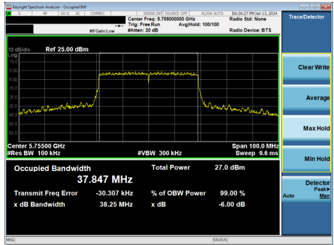
Plot 7-231. 6dB BW & 99% OBW Antenna 4a (40MHz BW 802.11ax(SU) – Ch. 151, MCS11)
