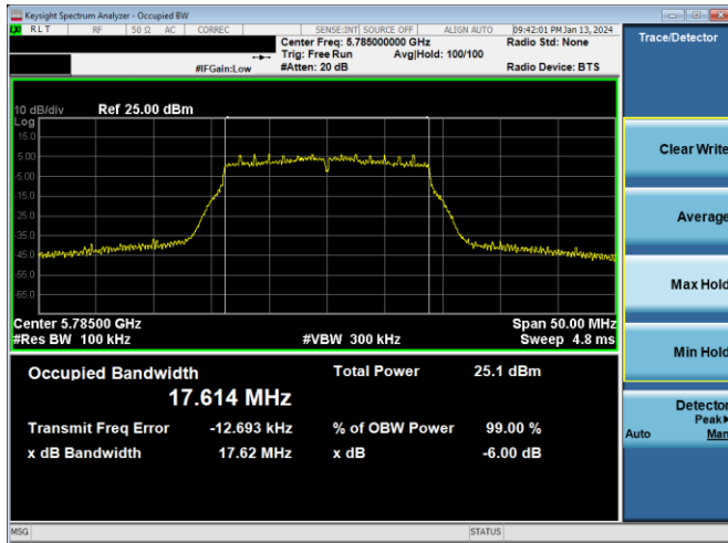
Plot 7-234. 6dB BW & 99% OBW Antenna 2a (20MHz BW 802.11n – Ch. 157, MCS2)
