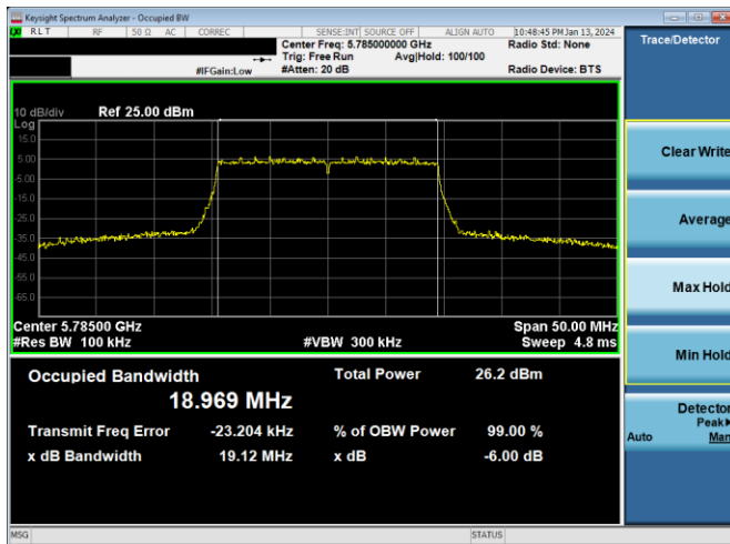
Plot 7-241. 6dB BW & 99% OBW Antenna 2a (20MHz BW 802.11ax(SU) – Ch. 157, MCS4)
