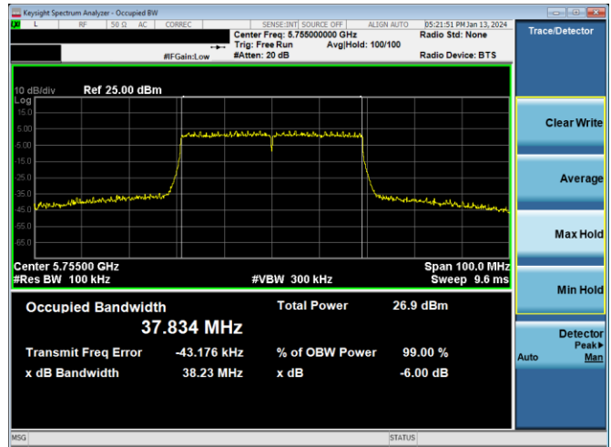
Plot 7-225. 6dB BW & 99% OBW Antenna 4a (40MHz BW 802.11ax(SU) – Ch. 151, MCS4)
