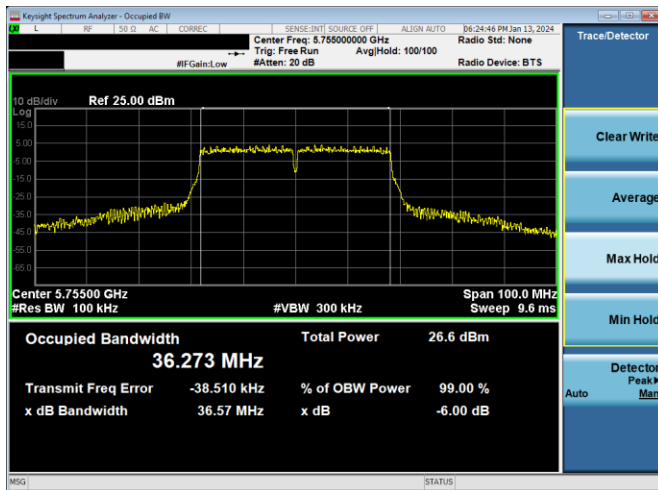
Plot 7-230. 6dB BW & 99% OBW Antenna 4a (40MHz BW 802.11n – Ch. 151, MCS7)
