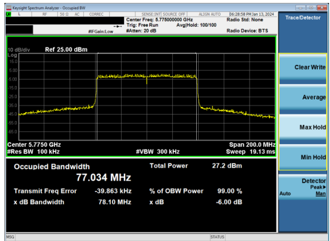
Plot 7-233. 6dB BW & 99% OBW Antenna 4a (80MHz BW 802.11ax(SU) – Ch. 155, MCS11)
