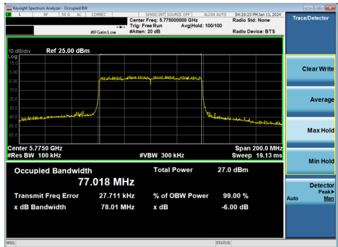
Plot 7-221. 6dB BW & 99% OBW Antenna 4a (80MHz BW 802.11ax(SU) – Ch. 155, MCS2)
