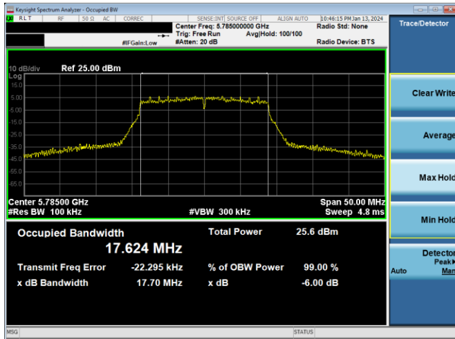
Plot 7-240. 6dB BW & 99% OBW Antenna 2a (20MHz BW 802.11n – Ch. 157, MCS4)
