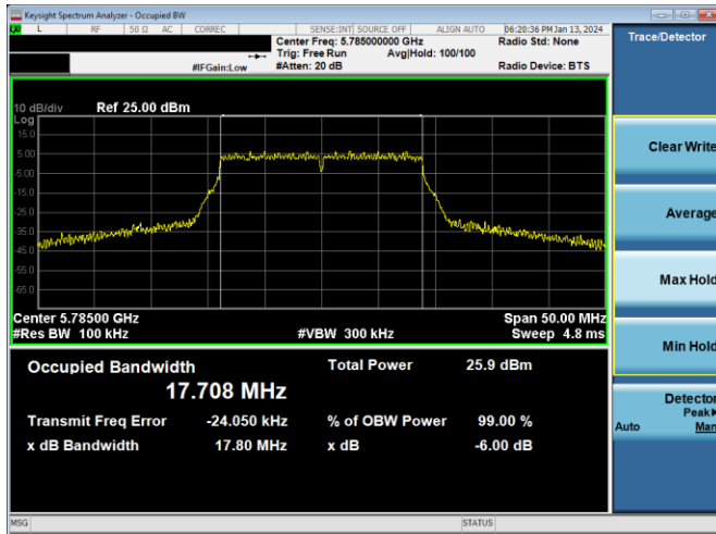
Plot 7-228. 6dB BW & 99% OBW Antenna 4a (20MHz BW 802.11n – Ch. 157, MCS7)
