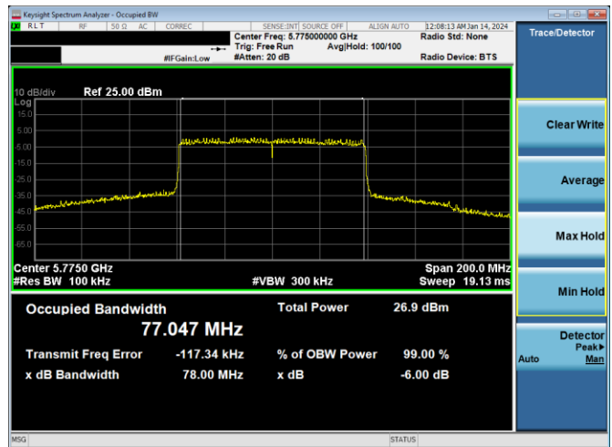
Plot 7-251. 6dB BW & 99% OBW Antenna 2a (80MHz BW 802.11ax(SU) – Ch. 155, MCS11)
