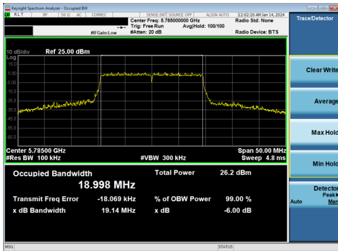
Plot 7-247. 6dB BW & 99% OBW Antenna 2a (20MHz BW 802.11ax(SU) – Ch. 157, MCS11)
