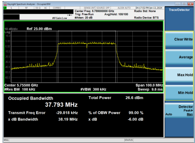
Plot 7-219. 6dB BW & 99% OBW Antenna 4a (40MHz BW 802.11ax(SU) – Ch. 151, MCS2)
