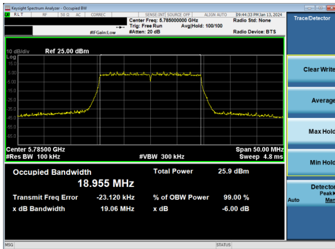
Plot 7-235. 6dB BW & 99% OBW Antenna 2a (20MHz BW 802.11ax(SU) – Ch. 157, MCS2)
