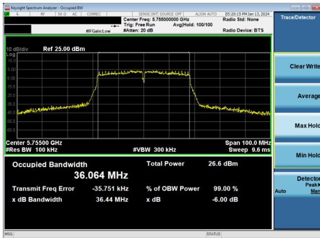
Plot 7-224. 6dB BW & 99% OBW Antenna 4a (40MHz BW 802.11n – Ch. 151, MCS4)
