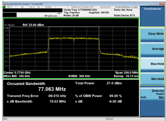
Plot 7-245. 6dB BW & 99% OBW Antenna 2a (80MHz BW 802.11ax(SU) – Ch. 155, MCS4)
