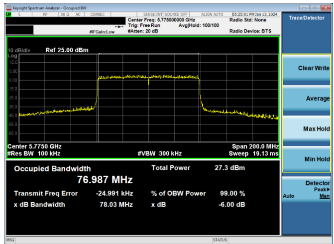
Plot 7-227. 6dB BW & 99% OBW Antenna 4a (80MHz BW 802.11ax(SU) – Ch. 155, MCS4)
