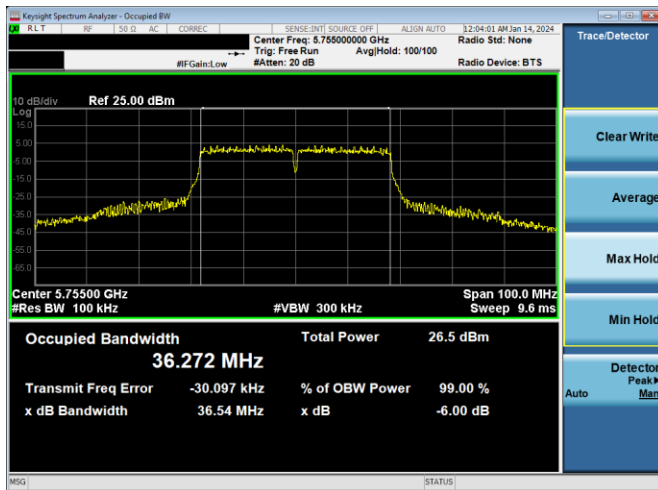
Plot 7-248. 6dB BW & 99% OBW Antenna 2a (40MHz BW 802.11n – Ch. 151, MCS7)
