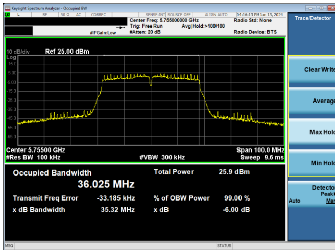
Plot 7-218. 6dB BW & 99% OBW Antenna 4a (40MHz BW 802.11n – Ch. 151, MCS2)
