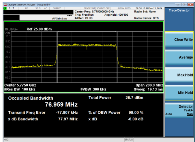
Plot 7-239. 6dB BW & 99% OBW Antenna 2a (80MHz BW 802.11ax(SU) – Ch. 155, MCS2)
