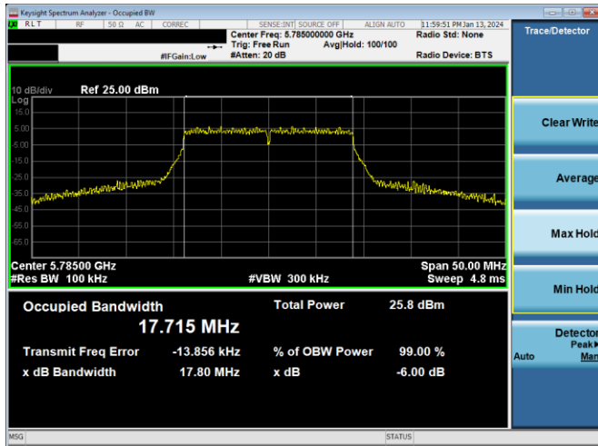
Plot 7-246. 6dB BW & 99% OBW Antenna 2a (20MHz BW 802.11n – Ch. 157, MCS7)
