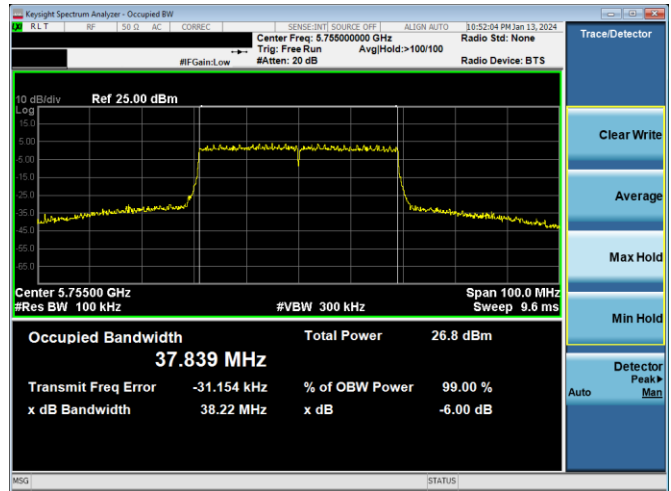
Plot 7-243. 6dB BW & 99% OBW Antenna 2a (40MHz BW 802.11ax(SU) – Ch. 151, MCS4)
