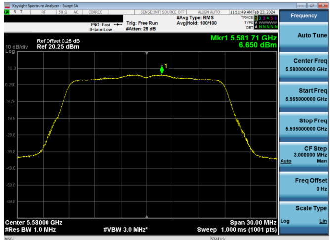
Plot 7-604. PSD CDD Primary Antenna 4a (20MHz BW 802.11n - Ch. 116, MCS10)
