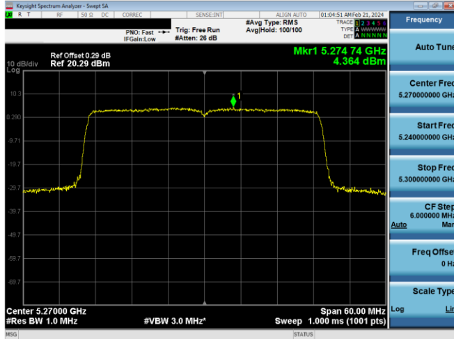
Plot 7-641. PSD CDD Primary Antenna WF5b (40MHz BW 802.11ax(SU) – Ch. 54, MCS4)
