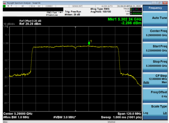
Plot 7-645. PSD CDD Primary Antenna WF5b (80MHz BW 802.11ax(SU) – Ch. 58, MCS4)
