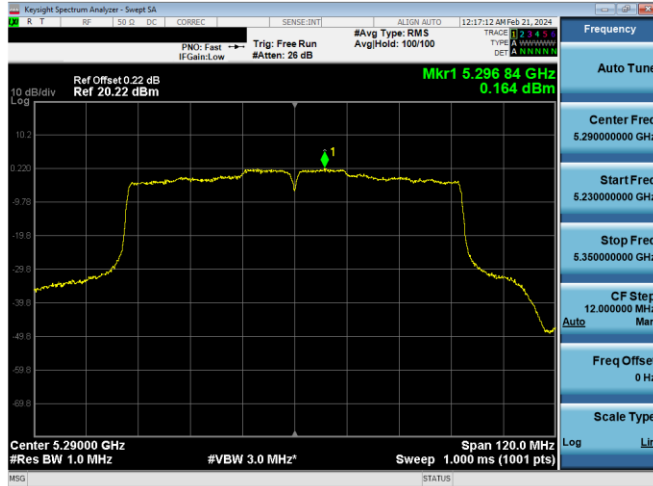
Plot 7-599. PSD CDD Primary Antenna WF5b (80MHz BW 802.11ac - Ch. 58, MCS2)
