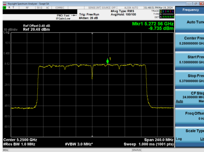
Plot 7-678. PSD CDD Primary Antenna 4a (160MHz BW 802.11ax(SU) – Ch. 50, MCS11)
