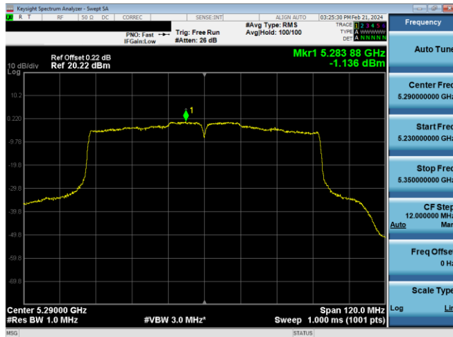
Plot 7-600. PSD CDD Primary Antenna 4a (80MHz BW 802.11ac - Ch. 58, MCS2)
