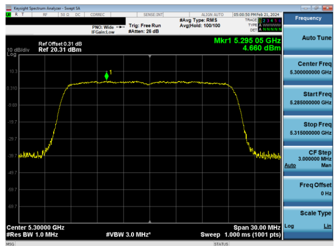
Plot 7-682. PSD CDD Primary Antenna 4a (20MHz BW 802.11ax(SU) – Ch. 60, MCS11)
