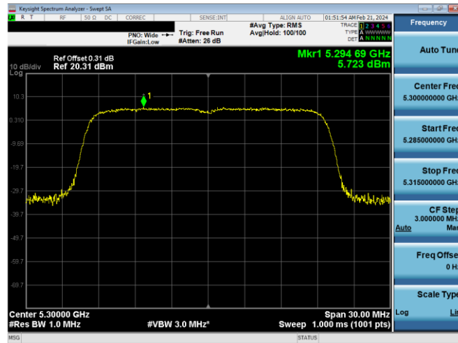
Plot 7-679. PSD CDD Primary Antenna WF5b (20MHz BW 802.11n – Ch. 60, MCS15)
