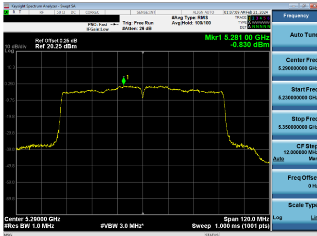
Plot 7-643. PSD CDD Primary Antenna WF5b (80MHz BW 802.11ac – Ch. 58, MCS4)
