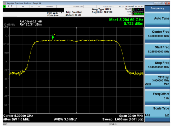
Plot 7-681. PSD CDD Primary Antenna WF5b (20MHz BW 802.11ax(SU) – Ch. 60, MCS11)
