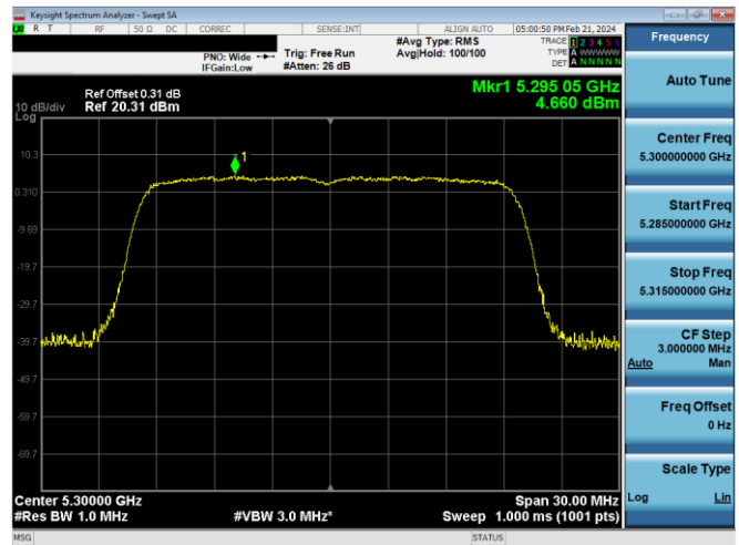
Plot 7-680. PSD CDD Primary Antenna 4a (20MHz BW 802.11n – Ch. 60, MCS15)
