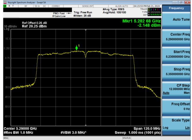
Plot 7-644. PSD CDD Primary Antenna 4a (80MHz BW 802.11ac – Ch. 58, MCS4)
