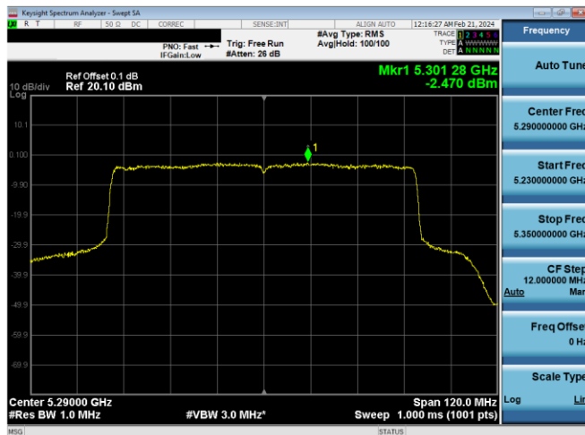
Plot 7-601. PSD CDD Primary Antenna WF5b (80MHz BW 802.11ax(SU) - Ch. 58, MCS2)
