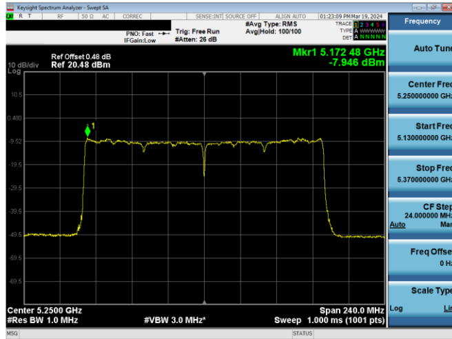
Plot 7-677. PSD CDD Primary Antenna WF5b (160MHz BW 802.11ax(SU) – Ch. 50, MCS11)
