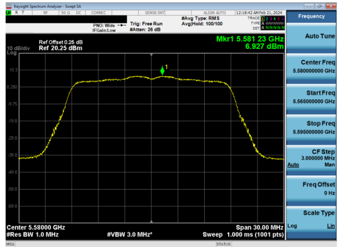
Plot 7-603. PSD CDD Primary Antenna WF5b (20MHz BW 802.11n - Ch. 116, MCS10)
