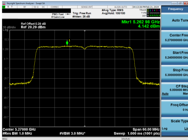
Plot 7-642. PSD CDD Primary Antenna 4a (40MHz BW 802.11ax(SU) – Ch. 54, MCS4)
