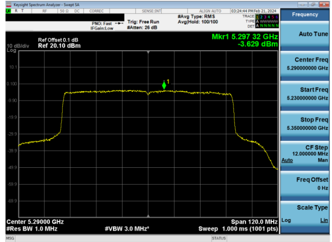
Plot 7-602. PSD CDD Primary Antenna 4a (80MHz BW 802.11ax(SU) - Ch. 58, MCS2)
