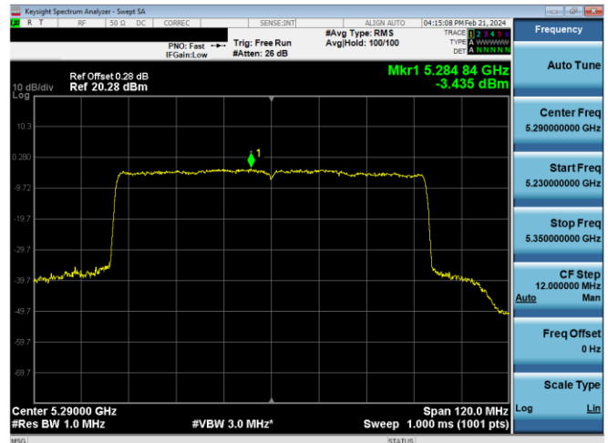
Plot 7-646. PSD CDD Primary Antenna 4a (80MHz BW 802.11ax(SU) – Ch. 58, MCS4)
