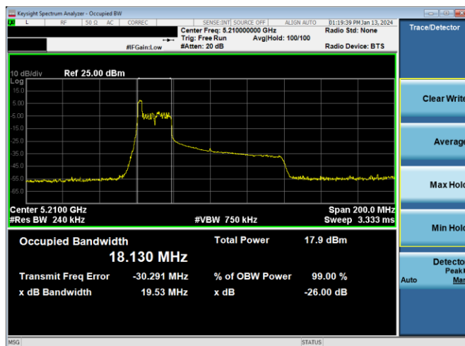
Plot 7-53. 26dB BW & 99% OBW Antenna 4a (80MHz BW 11ax Index 0 – RU26 – Ch.42)
