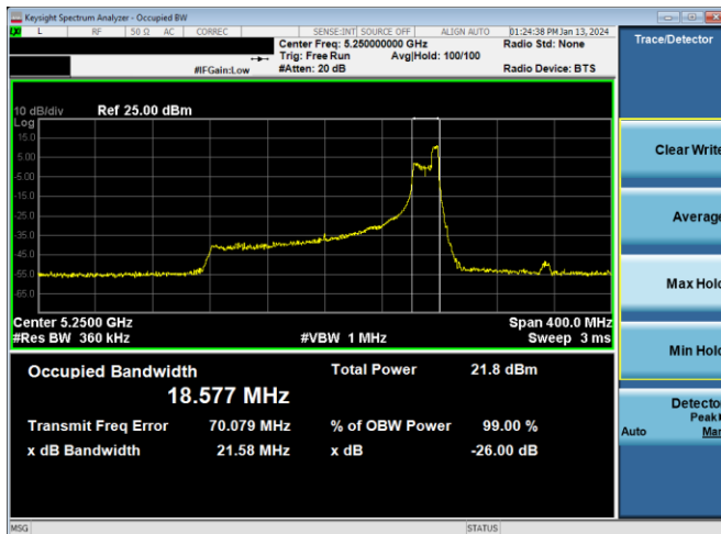
Plot 7-59. 26dB BW & 99% OBW Antenna 4a (160MHz BW 11ax Index 52 – RU52 – Ch.50 (U))
