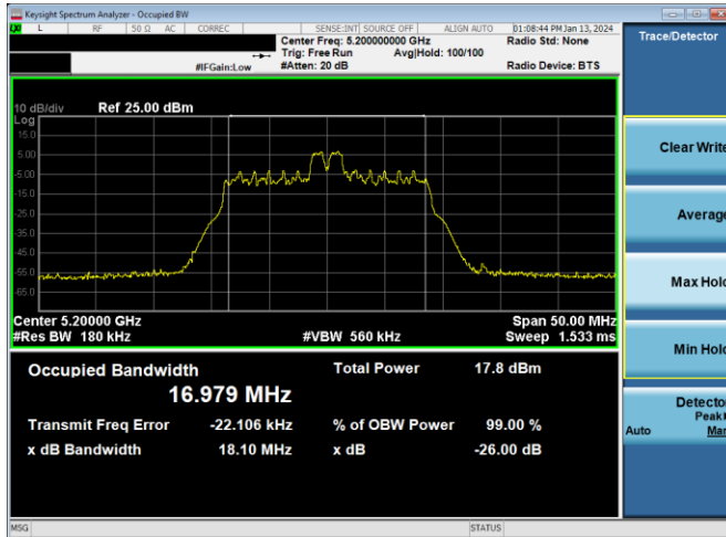
Plot 7-46. 26dB BW & 99% OBW Antenna 4a (20MHz BW 11ax Index 4 – RU26 – Ch.40)
