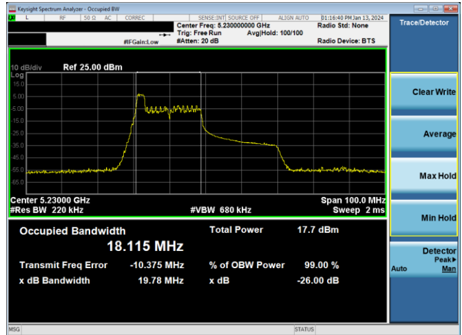
Plot 7-49. 26dB BW & 99% OBW Antenna 4a (40MHz BW 11ax Index 0 – RU26 – Ch.46)
