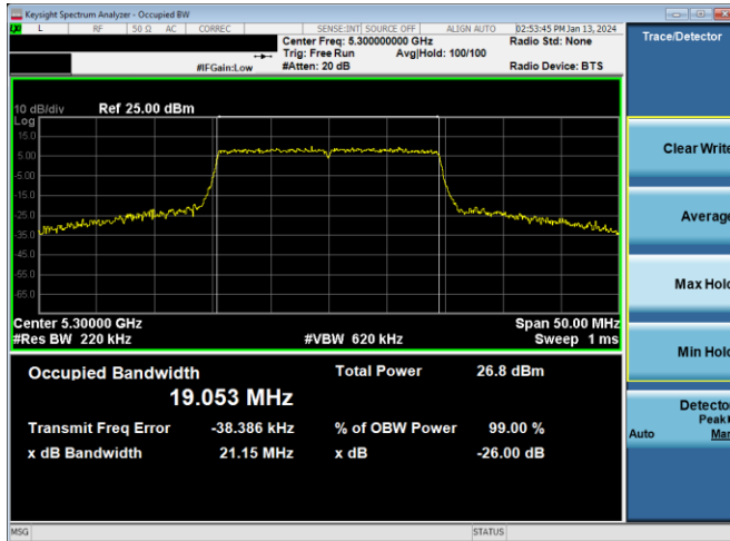
Plot 7-64. 26dB BW & 99% OBW Antenna 4a (20MHz BW 11ax - RU242 - Ch.60)
