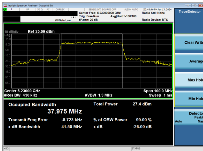
Plot 7-52. 26dB BW & 99% OBW Antenna 4a (40MHz BW 11ax – RU484 – Ch.46)
