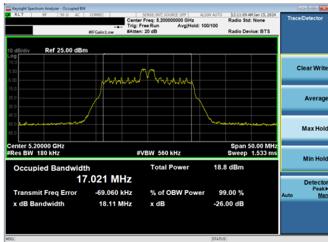
Plot 7-2. 26dB BW & 99% OBW Antenna WF5B (20MHz BW 11ax Index 4 – RU26 – Ch.40)
