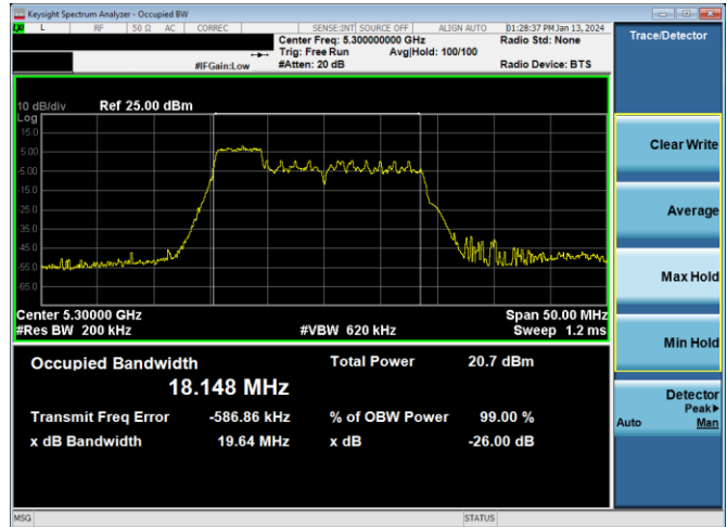
Plot 7-61. 26dB BW & 99% OBW Antenna 4a (20MHz BW 11ax Index 37 – RU52 – Ch.60)
