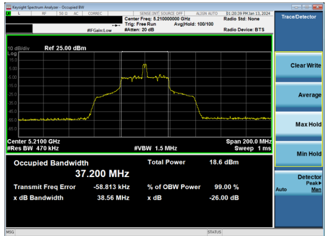
Plot 7-54. 26dB BW & 99% OBW Antenna 4a (80MHz BW 11ax Index 18 – RU26 – Ch.42)
