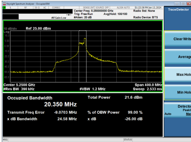
Plot 7-58. 26dB BW & 99% OBW Antenna 4a (160MHz BW 11ax Index 52 – RU52 – Ch.50 (L))
