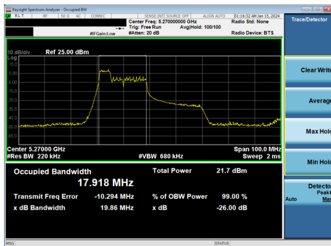
Plot 7-21. 26dB BW & 99% OBW Antenna WF5B (40MHz BW 11ax Index 37 – RU52 – Ch.54)
