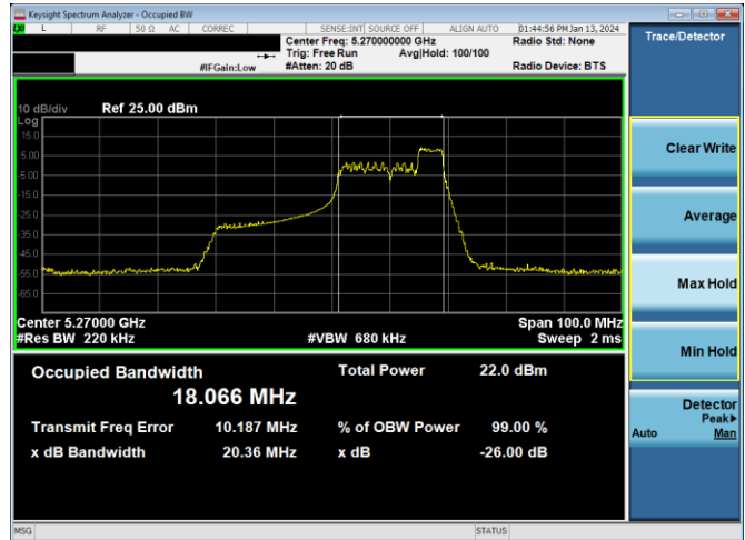
Plot 7-67. 26dB BW & 99% OBW Antenna 4a (40MHz BW 11ax Index 44 - RU52 - Ch.54)
