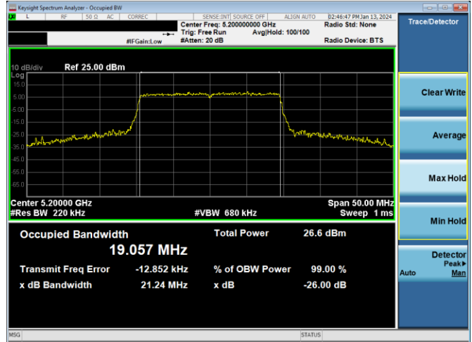
Plot 7-48. 26dB BW & 99% OBW Antenna 4a (20MHz BW 11ax – RU242 – Ch.40)
