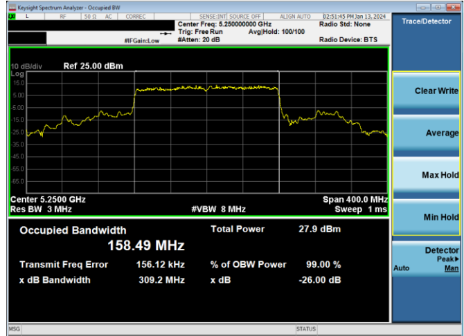
Plot 7-60. 26dB BW & 99% OBW Antenna 4a (160MHz BW 11ax – RU996x2 – Ch.50)
