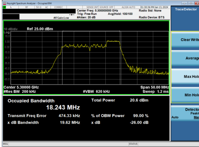
Plot 7-63. 26dB BW & 99% OBW Antenna 4a (20MHz BW 11ax Index 40 - RU52 - Ch.60)
