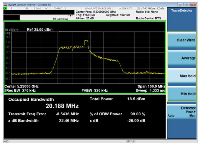
Plot 7-50. 26dB BW & 99% OBW Antenna 4a (40MHz BW 11ax Index 8 – RU26 – Ch.46)
