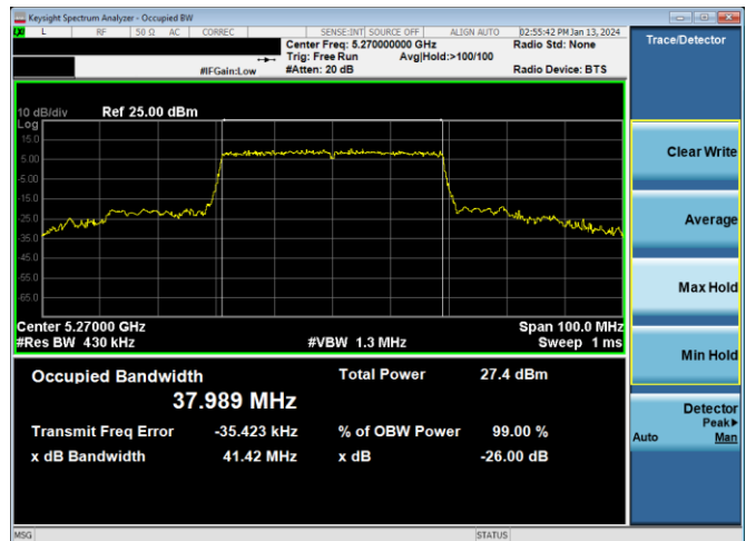
Plot 7-68. 26dB BW & 99% OBW Antenna 4a (40MHz BW 11ax - RU484 - Ch.54)
