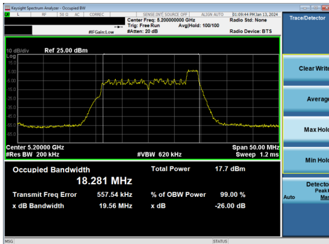
Plot 7-47. 26dB BW & 99% OBW Antenna 4a (20MHz BW 11ax Index 8 – RU26 – Ch.40)
