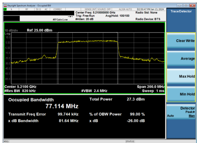
Plot 7-56. 26dB BW & 99% OBW Antenna 4a (80MHz BW 11ax – RU996 – Ch.42)
