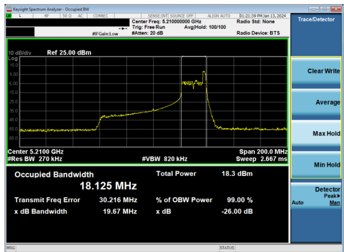
Plot 7-55. 26dB BW & 99% OBW Antenna 4a (80MHz BW 11ax Index 36 – RU26 – Ch.42)
