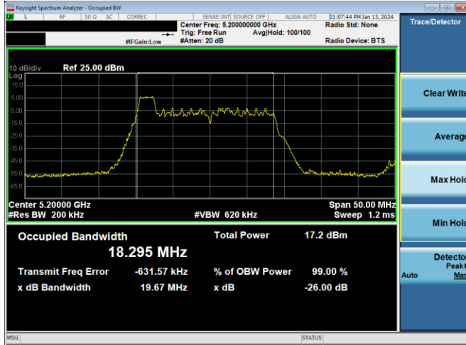
Plot 7-45. 26dB BW & 99% OBW Antenna 4a (20MHz BW 11ax Index 0 – RU26 – Ch.40)
