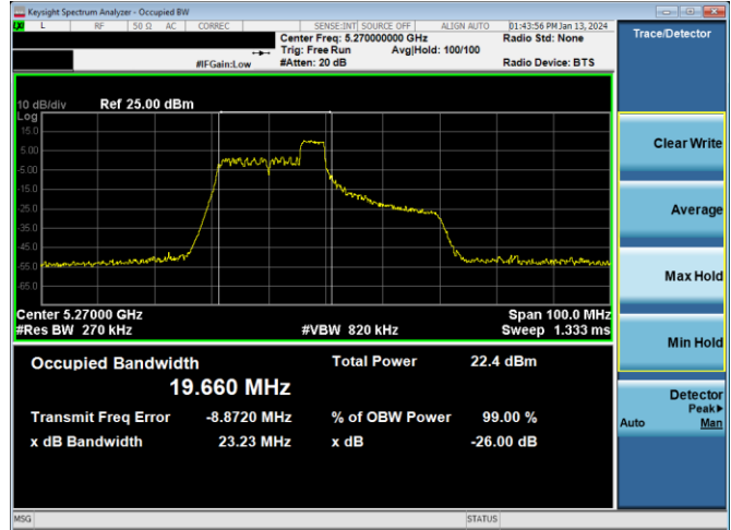
Plot 7-66. 26dB BW & 99% OBW Antenna 4a (40MHz BW 11ax Index 40 - RU52 - Ch.54)
