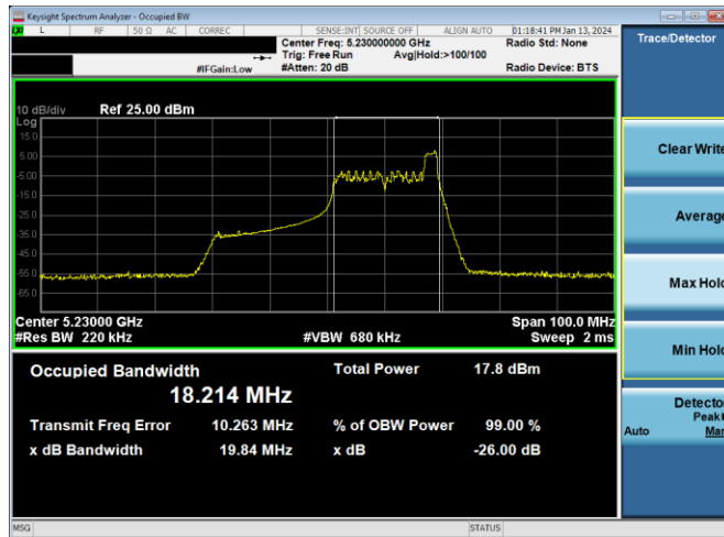
Plot 7-51. 26dB BW & 99% OBW Antenna 4a (40MHz BW 11ax Index 17 – RU26 – Ch.46)
