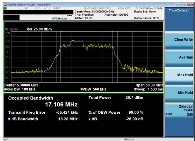
Plot 7-62. 26dB BW & 99% OBW Antenna 4a (20MHz BW 11ax Index 38 – RU52 – Ch.60)
