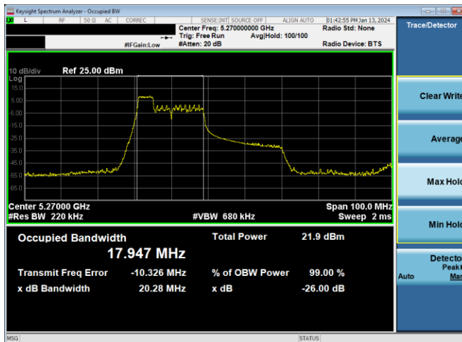
Plot 7-65. 26dB BW & 99% OBW Antenna 4a (40MHz BW 11ax Index 37 - RU52 - Ch.54)
